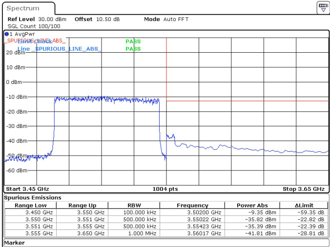
70MHz_30kHz_3515MHz_DFT-s-OFDM QPSK_RB180@0 -35.39 dBm
