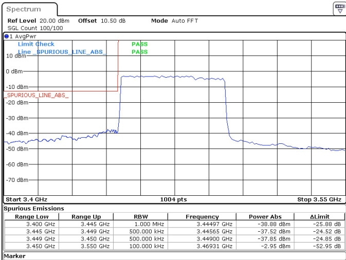
50MHz_30kHz_3475MHz_DFT-s-OFDM QPSK_RB128@0 -37.52 dBm
