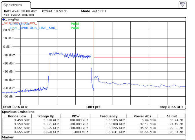
50MHz_30kHz_3525MHz_DFT-s-OFDM QPSK_RB128@0 -35.55 dBm
