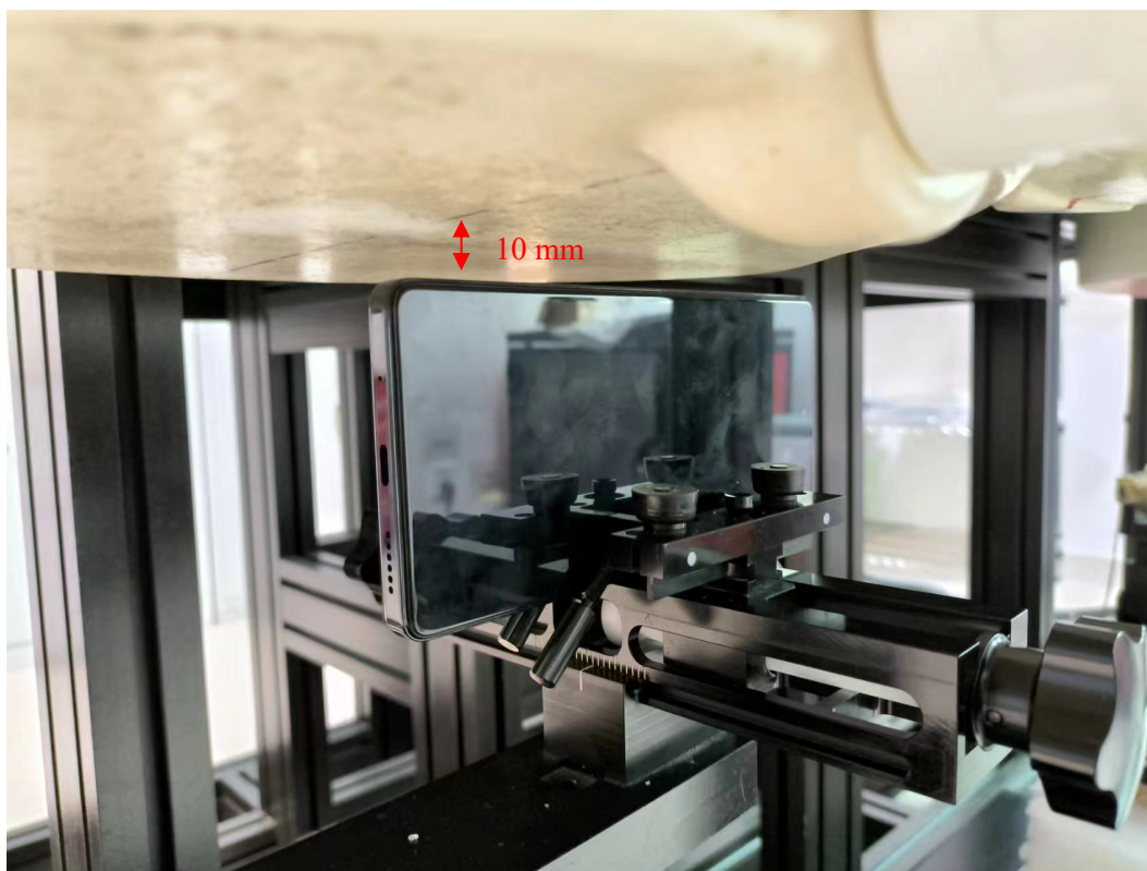
Body Right Setup Photo (10 mm)
