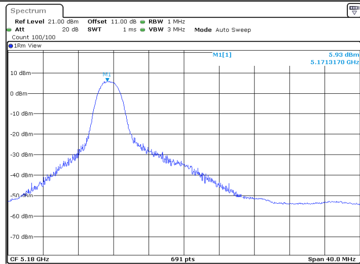
11AX20MIMO_Chain0_5180_26Tone_RU0
