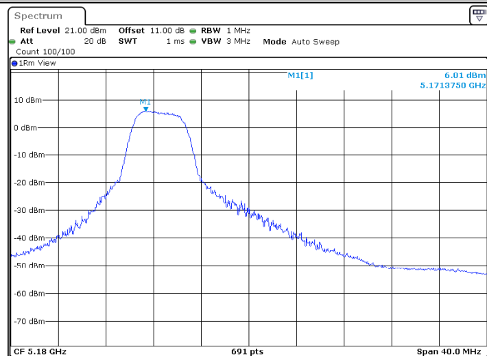
11AX20MIMO_Chain0_5180_52Tone_RU37
