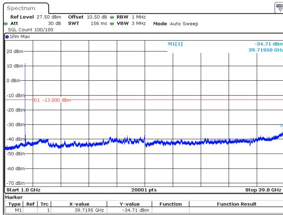
50MHz_15kHz_3840MHz_DFT-s-OFDM QPSK_RB1@0&amp;-34.71 dBm
