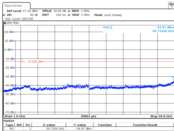
50MHz_30kHz_3725MHz_DFT-s-OFDM QPSK_RB1@0&amp;-34.97 dBm
