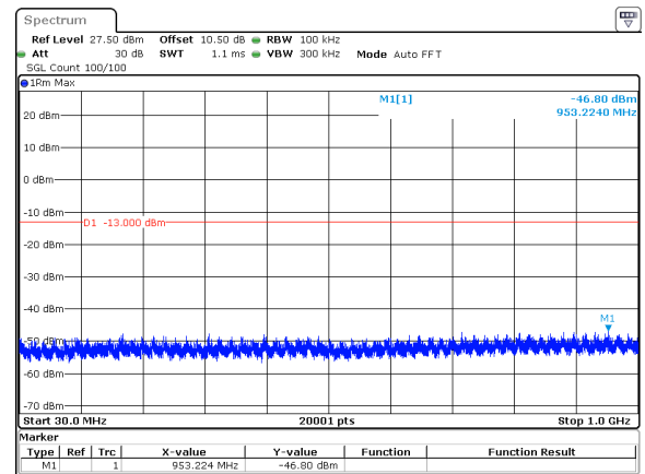
50MHz_30kHz_3725MHz_DFT-s-OFDM QPSK_RB1@0&amp;-46.80 dBm
