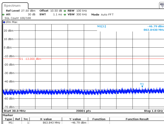
10MHz_30kHz_3545MHz_DFT-s-OFDM QPSK_RB24@0&amp;-46.79 dBm
