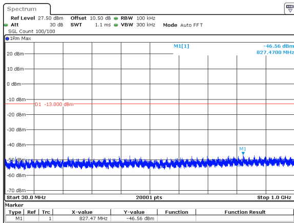
50MHz_30kHz_3955MHz_DFT-s-OFDM QPSK_RB1@132&amp;-46.56 dBm
