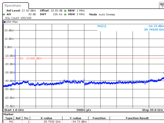
40MHz_15kHz_3840MHz_DFT-s-OFDM QPSK_RB216@0&amp;-34.73 dBm
