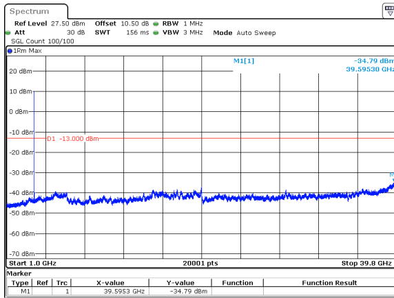
70MHz_30kHz_3735MHz_DFT-s-OFDM QPSK_RB1@0&amp;-34.79 dBm
