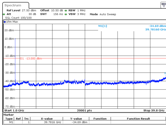
40MHz_30kHz_3840MHz_DFT-s-OFDM QPSK_RB1@0&amp;-34.69 dBm
