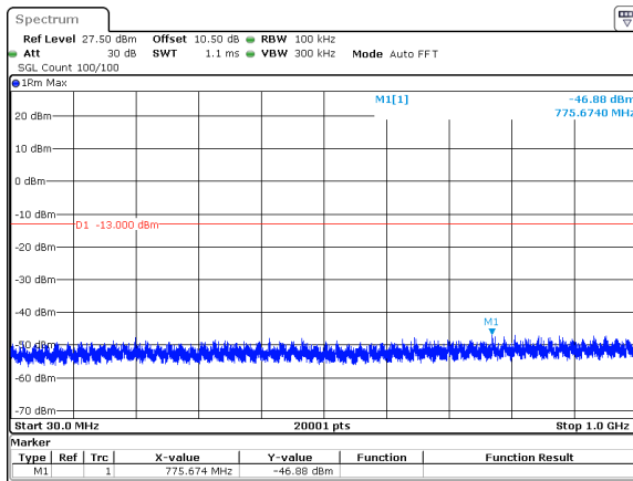
50MHz_30kHz_3840MHz_DFT-s-OFDM QPSK_RB1@132&amp;-46.88 dBm
