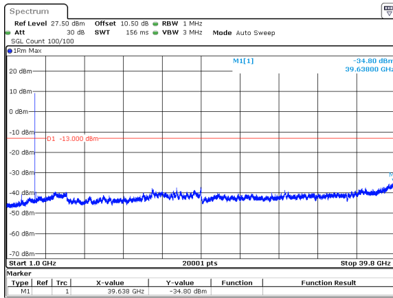
70MHz_30kHz_3840MHz_DFT-s-OFDM QPSK_RB1@0&amp;-34.80 dBm
