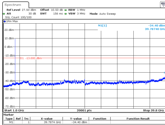
90MHz_30kHz_3840MHz_DFT-s-OFDM QPSK_RB1@0&amp;-34.40 dBm
