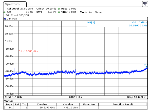
60MHz_30kHz_3730MHz_DFT-s-OFDM QPSK_RB1@0&amp;-35.10 dBm
