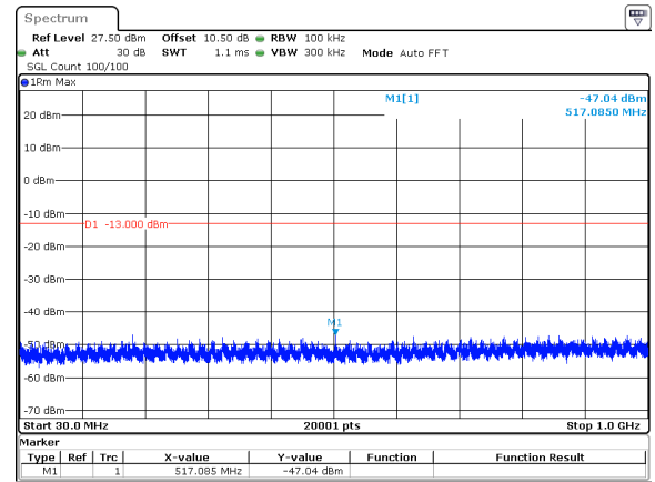
50MHz_15kHz_3725MHz_DFT-s-OFDM QPSK_RB1@0&amp;-47.04 dBm
