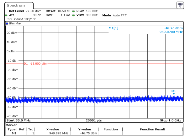
70MHz_30kHz_3840MHz_DFT-s-OFDM QPSK_RB1@188&amp;-46.75 dBm
