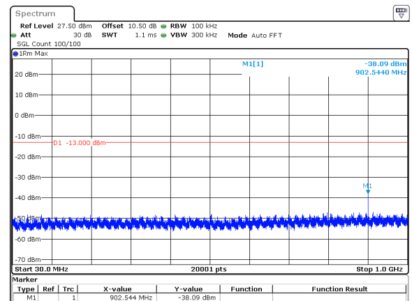
50MHz_15kHz_3840MHz_DFT-s-OFDM QPSK_RB270@0&amp;-38.09 dBm
