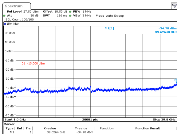
50MHz_30kHz_3725MHz_DFT-s-OFDM QPSK_RB1@132&amp;-34.78 dBm
