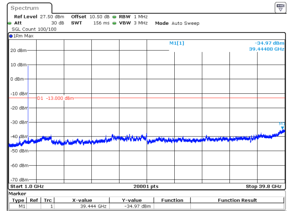
80MHz_30kHz_3740MHz_DFT-s-OFDM QPSK_RB1@0&amp;-34.97 dBm
