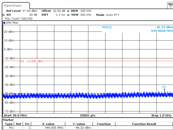
100MHz_30kHz_3840MHz_DFT-s-OFDM QPSK_RB1@272&amp;-46.22 dBm
