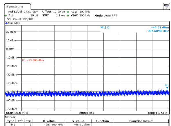
50MHz_15kHz_3955MHz_DFT-s-OFDM QPSK_RB270@0&amp;-46.51 dBm
