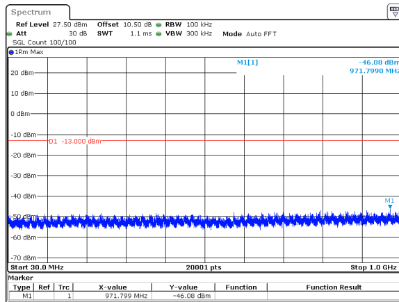
90MHz_30kHz_3840MHz_DFT-s-OFDM QPSK_RB1@244&amp;-46.08 dBm
