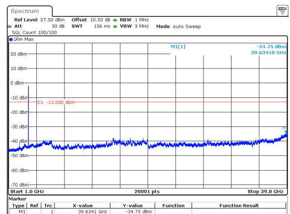
50MHz_30kHz_3725MHz_DFT-s-OFDM QPSK_RB128@0&amp;-34.75 dBm
