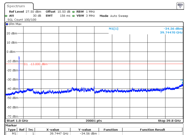
70MHz_30kHz_3945MHz_DFT-s-OFDM QPSK_RB180@0&amp;-34.56 dBm
