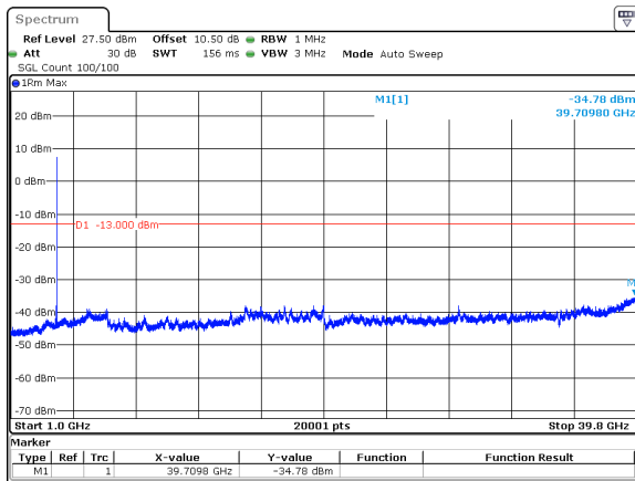
60MHz_30kHz_3840MHz_DFT-s-OFDM QPSK_RB1@161&amp;-34.78 dBm
