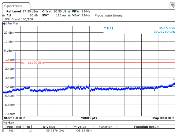
30MHz_15kHz_3715MHz_DFT-s-OFDM QPSK_RB160@0&amp;-35.15 dBm
