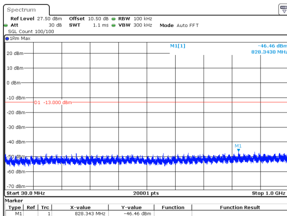
30MHz_15kHz_3965MHz_DFT-s-OFDM QPSK_RB160@0&amp;-46.46 dBm
