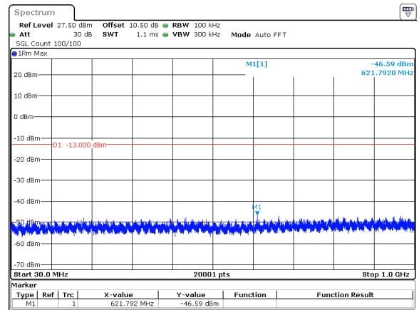
60MHz_30kHz_3730MHz_DFT-s-OFDM QPSK_RB1@161&amp;-46.59 dBm
