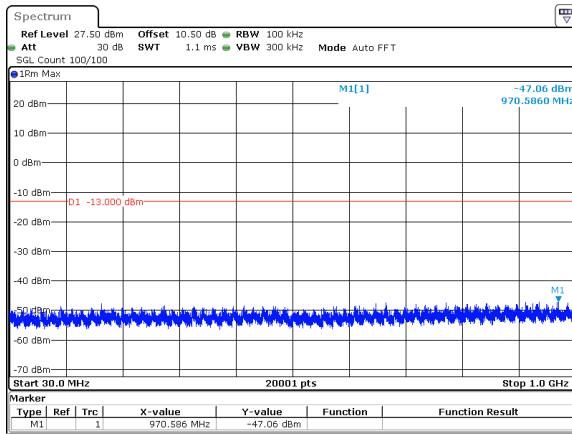
50MHz_30kHz_3840MHz_DFT-s-OFDM QPSK_RB1@0&amp;-47.06 dBm
