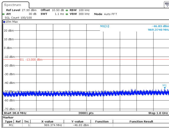
50MHz_15kHz_3955MHz_DFT-s-OFDM QPSK_RB1@0&amp;-46.83 dBm
