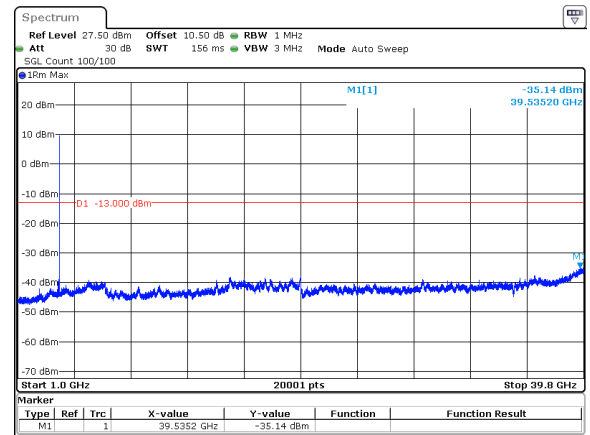
50MHz_30kHz_3840MHz_DFT-s-OFDM QPSK_RB1@132&amp;-35.14 dBm
