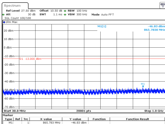
30MHz_15kHz_3840MHz_DFT-s-OFDM QPSK_RB160@0&amp;-46.83 dBm
