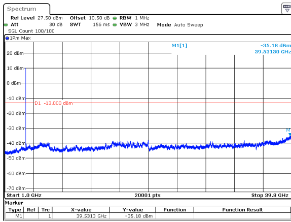
100MHz_30kHz_3840MHz_DFT-s-OFDM QPSK_RB1@0&amp;-35.18 dBm
