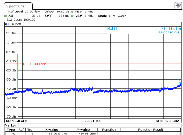
60MHz_30kHz_3730MHz_DFT-s-OFDM QPSK_RB162@0&amp;-34.81 dBm
