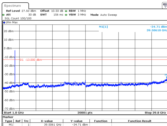
50MHz_15kHz_3840MHz_DFT-s-OFDM QPSK_RB270@0&amp;-34.71 dBm
