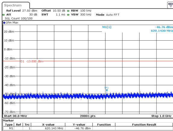
70MHz_30kHz_3945MHz_DFT-s-OFDM QPSK_RB1@188&amp;-46.76 dBm
