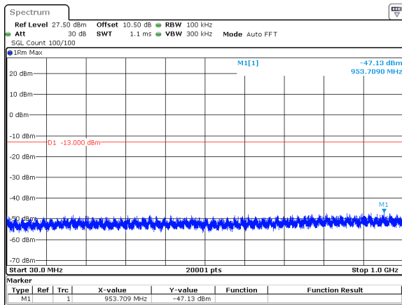
80MHz_30kHz_3840MHz_DFT-s-OFDM QPSK_RB1@216&amp;-47.13 dBm
