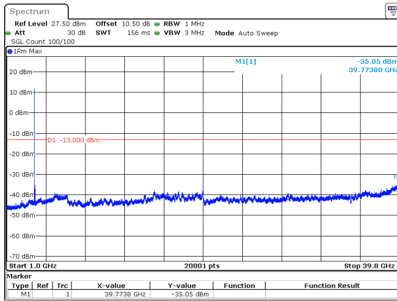
50MHz_15kHz_3725MHz_DFT-s-OFDM QPSK_RB1@0&amp;-35.05 dBm
