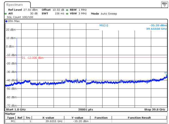
50MHz_30kHz_3840MHz_DFT-s-OFDM QPSK_RB1@0&amp;-35.20 dBm
