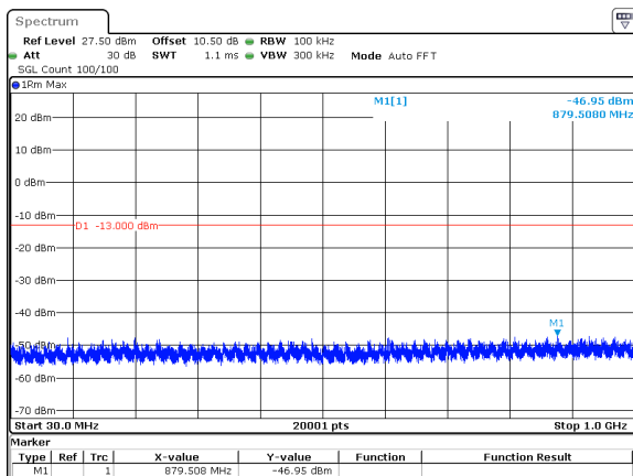
70MHz_30kHz_3945MHz_DFT-s-OFDM QPSK_RB180@0&amp;-46.95 dBm
