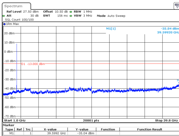
50MHz_15kHz_3955MHz_DFT-s-OFDM QPSK_RB1@269&amp;-35.04 dBm
