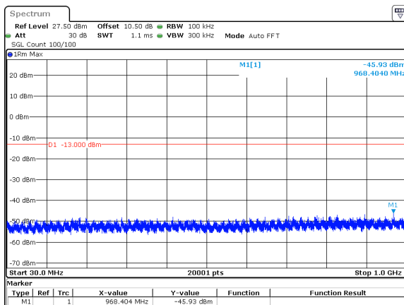
40MHz_30kHz_3720MHz_DFT-s-OFDM QPSK_RB100@0&amp;-45.93 dBm
