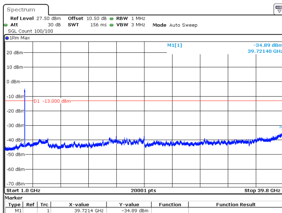
80MHz_30kHz_3740MHz_DFT-s-OFDM QPSK_RB216@0&amp;-34.89 dBm
