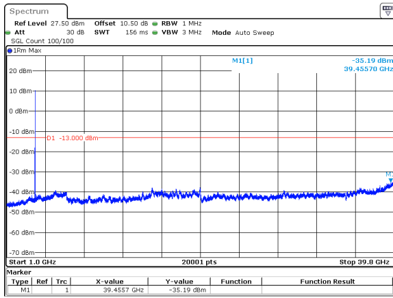
30MHz_15kHz_3840MHz_DFT-s-OFDM QPSK_RB1@0&amp;-35.19 dBm
