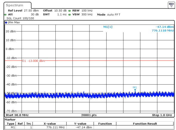
60MHz_30kHz_3840MHz_DFT-s-OFDM QPSK_RB1@161&amp;-47.14 dBm
