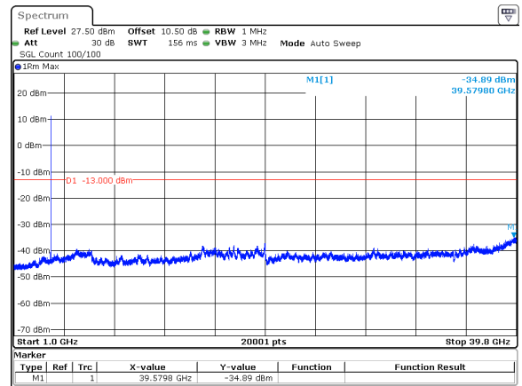
30MHz_15kHz_3840MHz_DFT-s-OFDM QPSK_RB1@159&amp;-34.89 dBm
