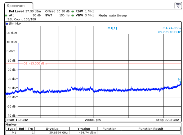
100MHz_30kHz_3840MHz_DFT-s-OFDM QPSK_RB1@272&amp;-34.74 dBm
