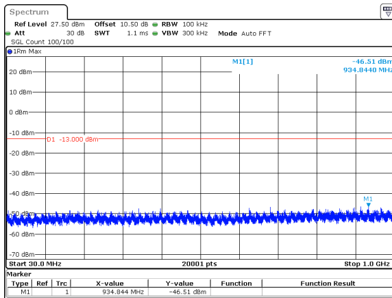
10MHz_30kHz_3545MHz_DFT-s-OFDM QPSK_RB1@23&amp;-46.51 dBm
