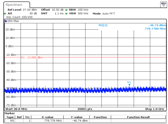
30MHz_15kHz_3840MHz_DFT-s-OFDM QPSK_RB1@0&amp;-46.74 dBm
