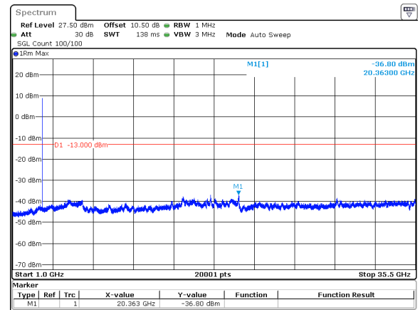
10MHz_30kHz_3545MHz_DFT-s-OFDM QPSK_RB1@23&amp;-36.80 dBm
