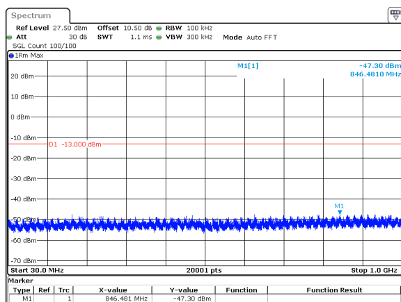
50MHz_30kHz_3725MHz_DFT-s-OFDM QPSK_RB128@0&amp;-47.30 dBm
