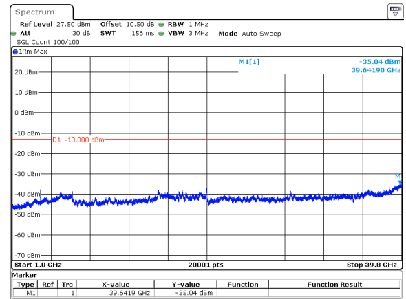
40MHz_15kHz_3840MHz_DFT-s-OFDM QPSK_RB1@215&amp;-35.04 dBm
