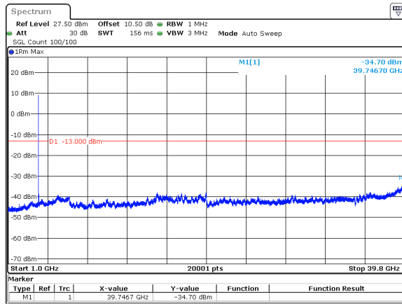
40MHz_15kHz_3960MHz_DFT-s-OFDM QPSK_RB1@0&amp;-34.70 dBm
