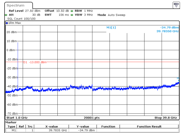
70MHz_30kHz_3735MHz_DFT-s-OFDM QPSK_RB1@188&amp;-34.79 dBm
