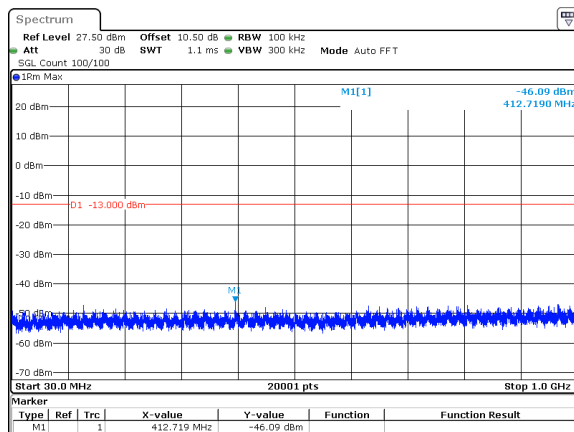
90MHz_30kHz_3840MHz_DFT-s-OFDM QPSK_RB243@0&amp;-46.09 dBm
