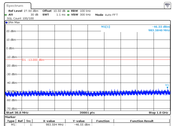
40MHz_15kHz_3840MHz_DFT-s-OFDM QPSK_RB216@0&amp;-46.55 dBm
