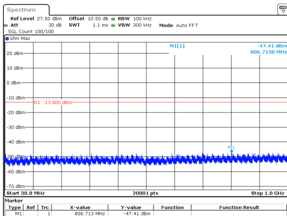
50MHz_30kHz_3955MHz_DFT-s-OFDM QPSK_RB128@0&amp;-47.41 dBm
