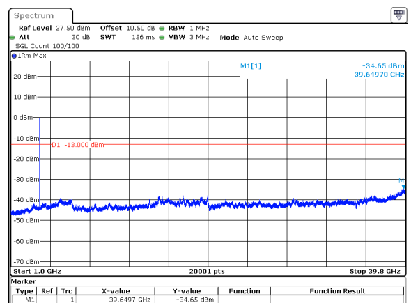
40MHz_30kHz_3840MHz_DFT-s-OFDM QPSK_RB100@0&amp;-34.65 dBm
