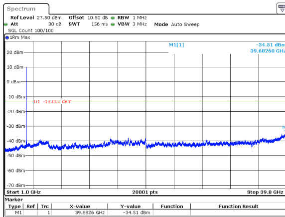
30MHz_15kHz_3965MHz_DFT-s-OFDM QPSK_RB1@159&amp;-34.51 dBm
