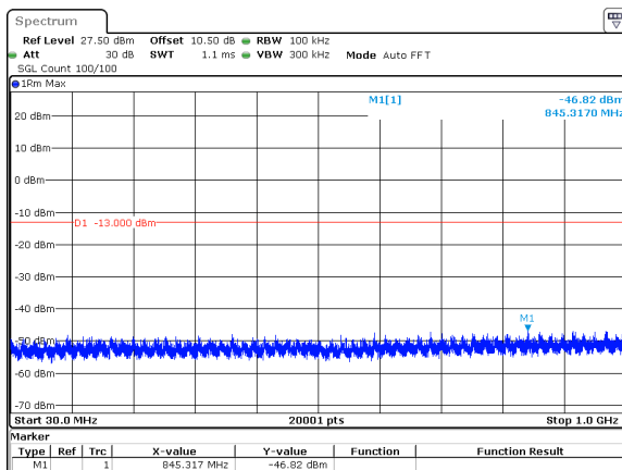
70MHz_30kHz_3735MHz_DFT-s-OFDM QPSK_RB180@0&amp;-46.82 dBm
