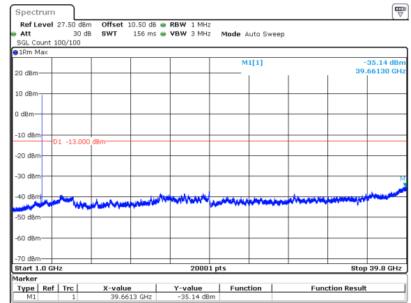
90MHz_30kHz_3840MHz_DFT-s-OFDM QPSK_RB1@244&amp;-35.14 dBm
