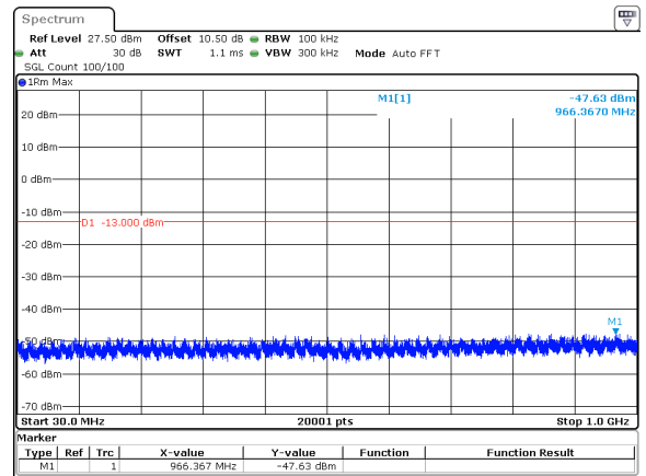
90MHz_30kHz_3935MHz_DFT-s-OFDM QPSK_RB1@244&amp;-47.63 dBm
