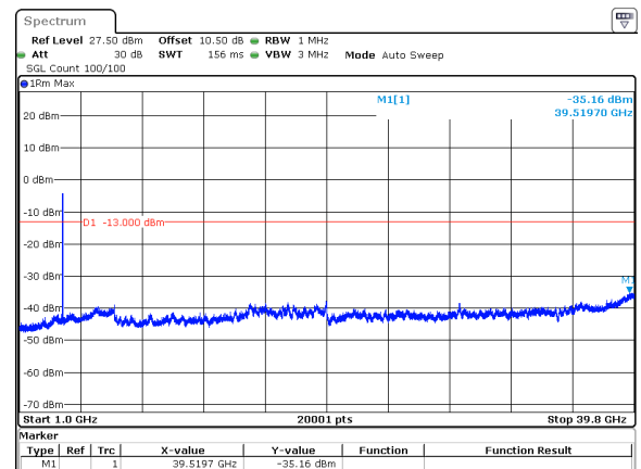
70MHz_30kHz_3735MHz_DFT-s-OFDM QPSK_RB180@0&amp;-35.16 dBm
