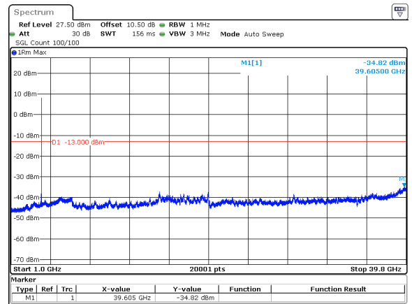
50MHz_30kHz_3955MHz_DFT-s-OFDM QPSK_RB1@132&amp;-34.82 dBm
