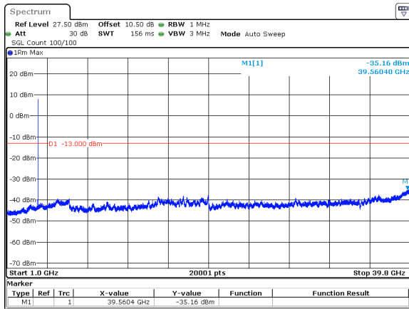
100MHz_30kHz_3930MHz_DFT-s-OFDM QPSK_RB1@272&amp;-35.16 dBm
