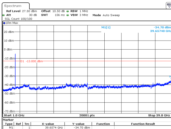
70MHz_30kHz_3840MHz_DFT-s-OFDM QPSK_RB180@0&amp;-34.70 dBm
