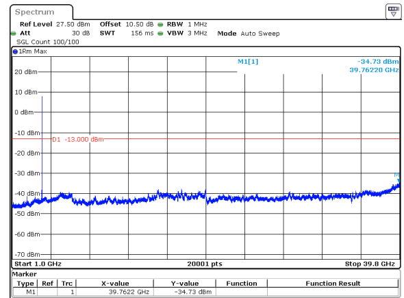
40MHz_30kHz_3960MHz_DFT-s-OFDM QPSK_RB1@105&amp;-34.73 dBm
