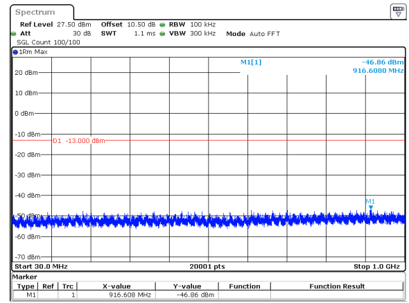
100MHz_30kHz_3840MHz_DFT-s-OFDM QPSK_RB1@0&amp;-46.86 dBm
