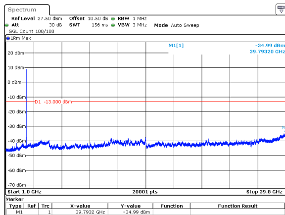
40MHz_30kHz_3840MHz_DFT-s-OFDM QPSK_RB1@105&amp;-34.99 dBm
