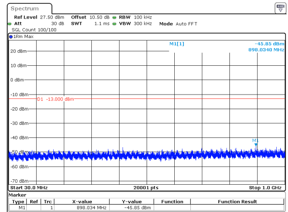
30MHz_15kHz_3715MHz_DFT-s-OFDM QPSK_RB1@159&amp;-45.85 dBm
