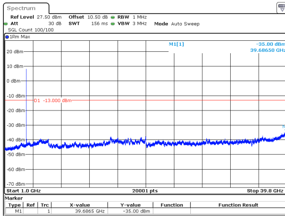
30MHz_15kHz_3965MHz_DFT-s-OFDM QPSK_RB1@0&amp;-35.00 dBm
