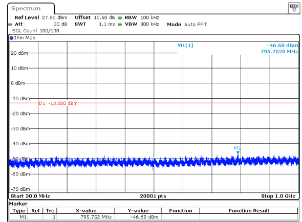
50MHz_15kHz_3840MHz_DFT-s-OFDM QPSK_RB1@0&amp;-46.68 dBm
