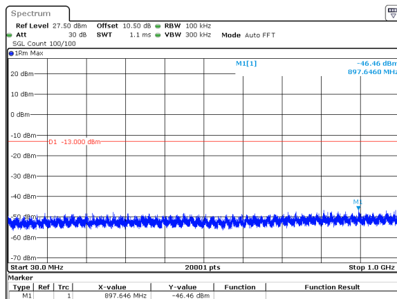
40MHz_15kHz_3960MHz_DFT-s-OFDM QPSK_RB216@0&amp;-46.46 dBm
