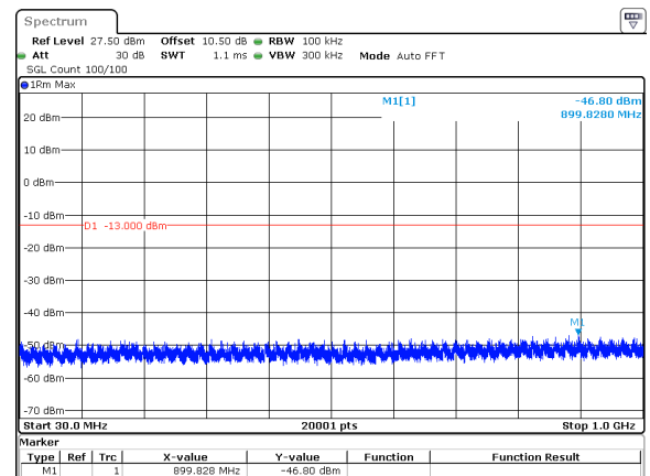
30MHz_15kHz_3715MHz_DFT-s-OFDM QPSK_RB160@0&amp;-46.80 dBm
