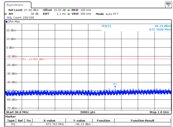
40MHz_15kHz_3840MHz_DFT-s-OFDM QPSK_RB1@0&amp;-46.13 dBm
