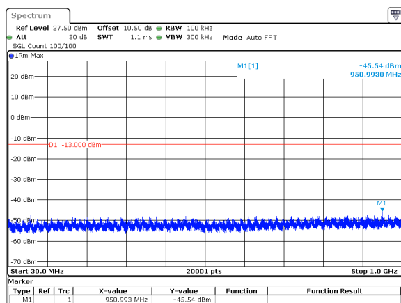
40MHz_30kHz_3840MHz_DFT-s-OFDM QPSK_RB100@0&amp;-45.54 dBm
