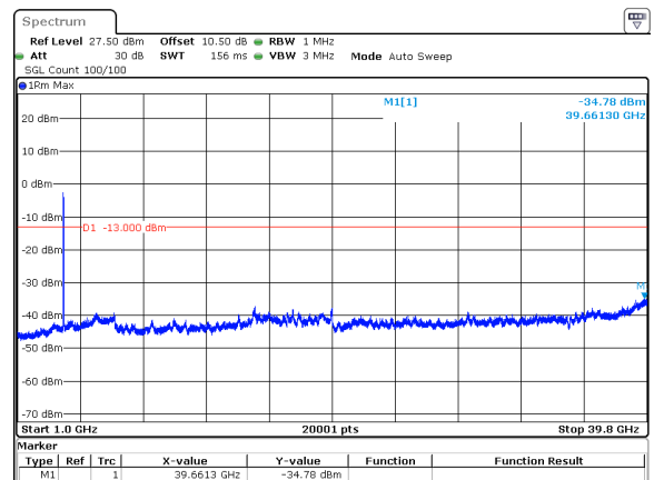
60MHz_30kHz_3840MHz_DFT-s-OFDM QPSK_RB162@0&amp;-34.78 dBm
