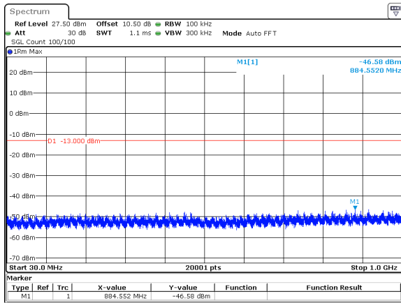
70MHz_30kHz_3945MHz_DFT-s-OFDM QPSK_RB1@0&amp;-46.58 dBm
