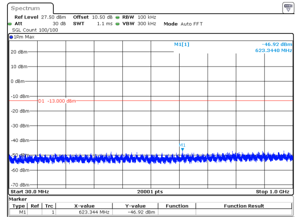
70MHz_30kHz_3735MHz_DFT-s-OFDM QPSK_RB1@0&amp;-46.92 dBm
