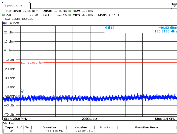
30MHz_15kHz_3840MHz_DFT-s-OFDM QPSK_RB1@159&amp;-46.82 dBm
