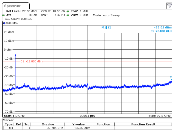
80MHz_30kHz_3840MHz_DFT-s-OFDM QPSK_RB216@0&amp;-35.02 dBm
