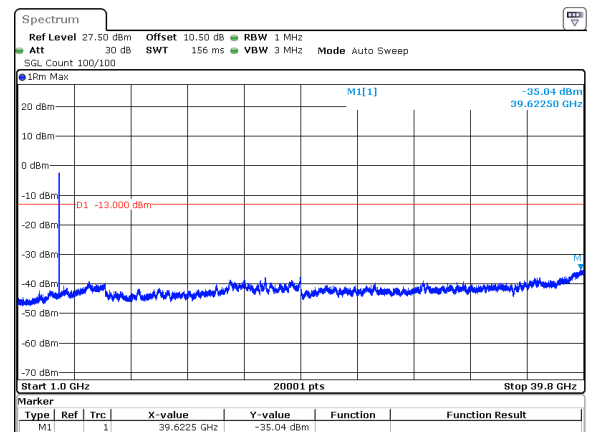
50MHz_30kHz_3840MHz_DFT-s-OFDM QPSK_RB128@0&amp;-35.04 dBm
