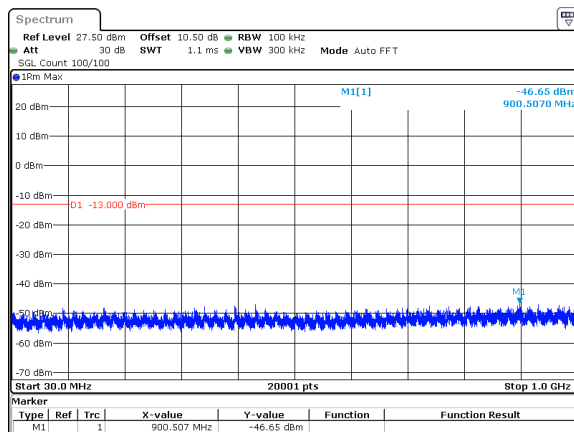
40MHz_15kHz_3720MHz_DFT-s-OFDM QPSK_RB216@0&amp;-46.65 dBm
