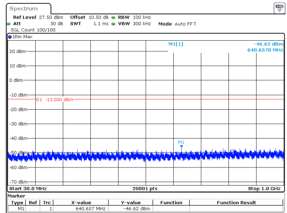
30MHz_15kHz_3965MHz_DFT-s-OFDM QPSK_RB1@159&amp;-46.62 dBm
