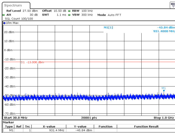
50MHz_15kHz_3840MHz_DFT-s-OFDM QPSK_RB1@269&amp;-45.84 dBm
