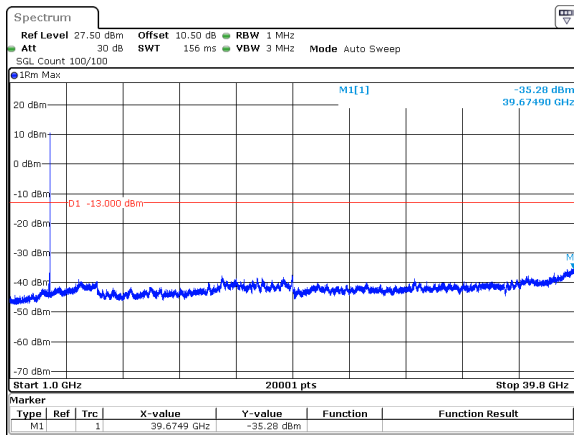
60MHz_30kHz_3730MHz_DFT-s-OFDM QPSK_RB1@161&amp;-35.28 dBm
