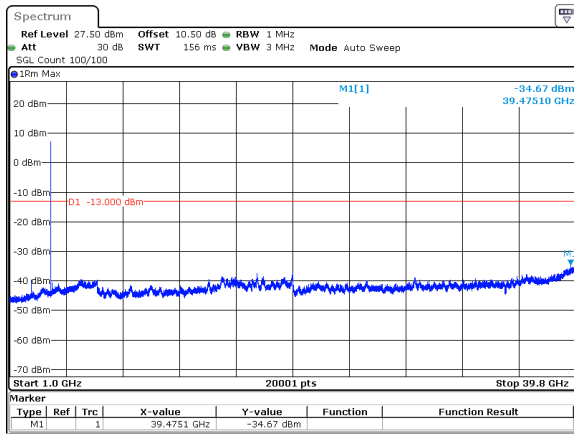
80MHz_30kHz_3840MHz_DFT-s-OFDM QPSK_RB1@0&amp;-34.67 dBm
