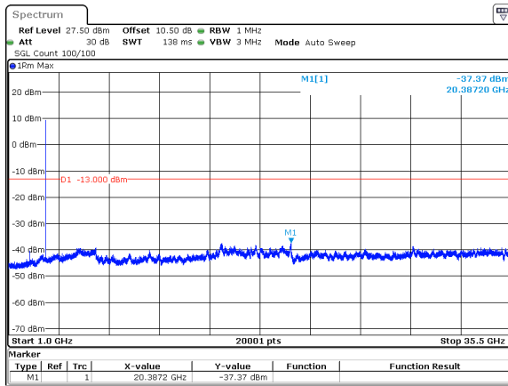
10MHz_30kHz_3545MHz_DFT-s-OFDM QPSK_RB1@0&amp;-37.37 dBm
