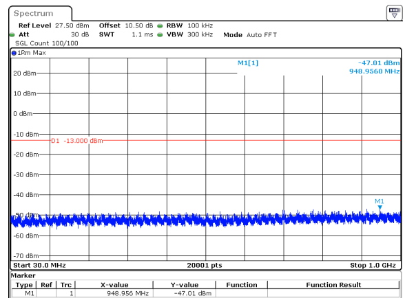
80MHz_30kHz_3840MHz_DFT-s-OFDM QPSK_RB216@0&amp;-47.01 dBm
