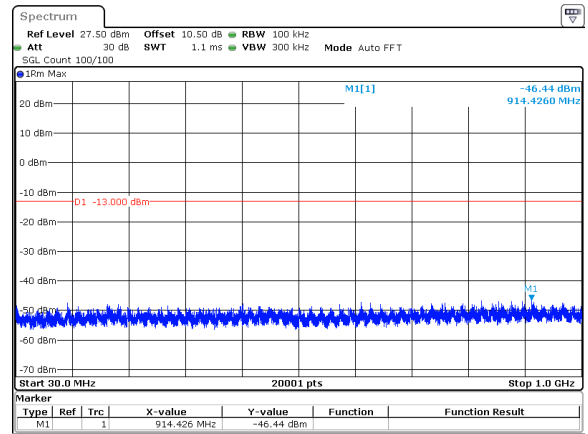
80MHz_30kHz_3840MHz_DFT-s-OFDM QPSK_RB1@0&amp;-46.44 dBm
