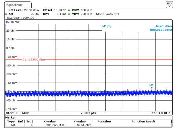
40MHz_15kHz_3720MHz_DFT-s-OFDM QPSK_RB1@0&amp;-46.61 dBm
