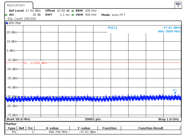
10MHz_30kHz_3545MHz_DFT-s-OFDM QPSK_RB1@0&amp;-47.01 dBm
