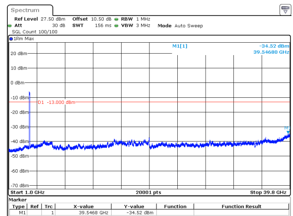
100MHz_30kHz_3840MHz_DFT-s-OFDM QPSK_RB270@0&amp;-34.52 dBm
