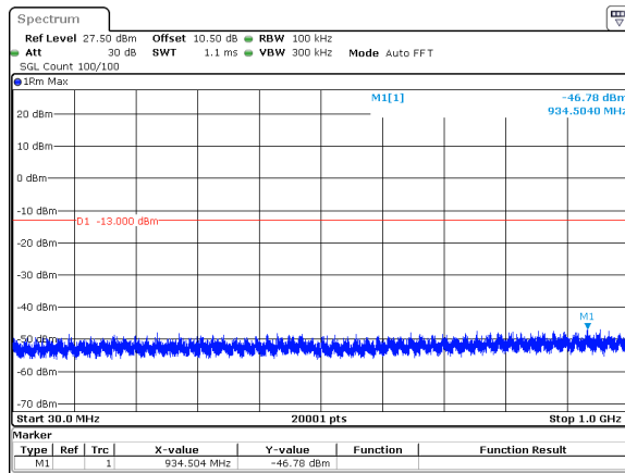
40MHz_15kHz_3840MHz_DFT-s-OFDM QPSK_RB1@215&amp;-46.78 dBm
