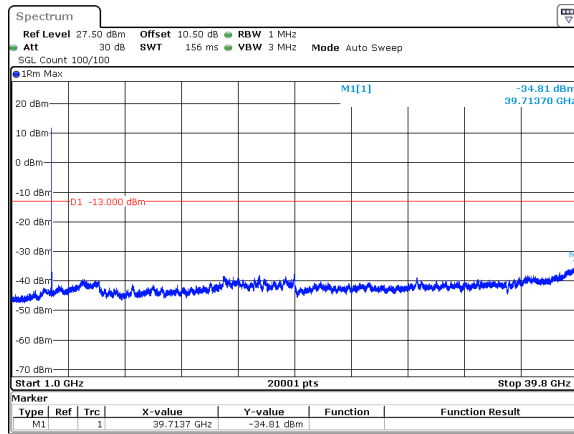
40MHz_15kHz_3720MHz_DFT-s-OFDM QPSK_RB1@0&amp;-34.81 dBm
