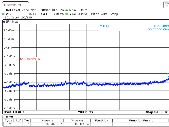
60MHz_30kHz_3840MHz_DFT-s-OFDM QPSK_RB1@0&amp;-34.58 dBm
