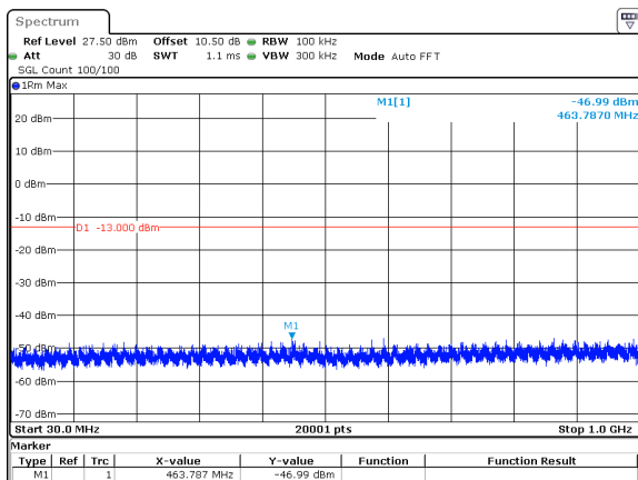
60MHz_30kHz_3840MHz_DFT-s-OFDM QPSK_RB162@0&amp;-46.99 dBm
