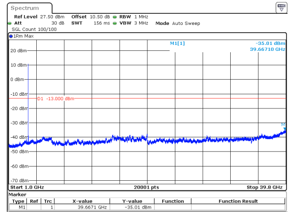
30MHz_15kHz_3715MHz_DFT-s-OFDM QPSK_RB1@0&amp;-35.01 dBm
