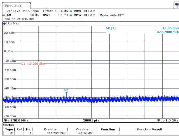
40MHz_30kHz_3720MHz_DFT-s-OFDM QPSK_RB1@105&amp;-45.96 dBm
