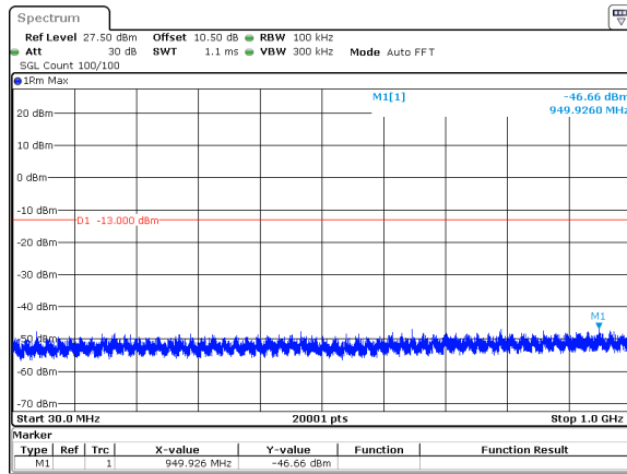
10MHz_30kHz_3500MHz_DFT-s-OFDM QPSK_RB1@0&amp;-46.66 dBm
