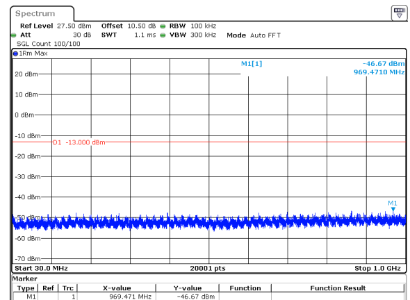
70MHz_30kHz_3840MHz_DFT-s-OFDM QPSK_RB180@0&amp;-46.67 dBm
