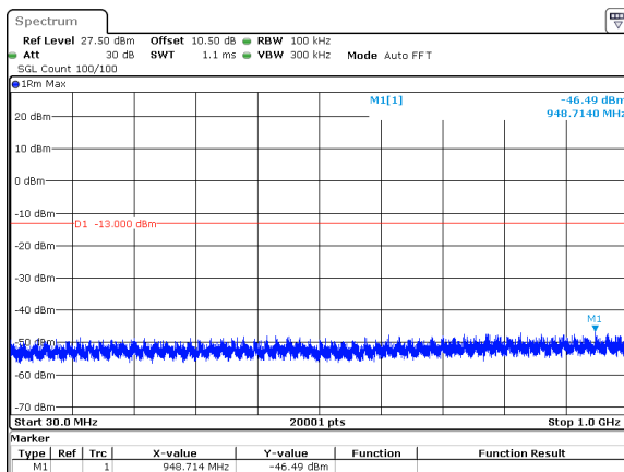
50MHz_30kHz_3840MHz_DFT-s-OFDM QPSK_RB128@0&amp;-46.49 dBm
