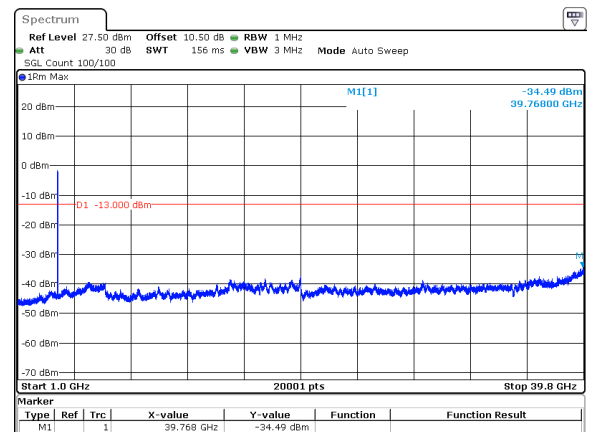
50MHz_15kHz_3725MHz_DFT-s-OFDM QPSK_RB270@0&amp;-34.49 dBm
