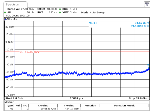
50MHz_15kHz_3725MHz_DFT-s-OFDM QPSK_RB1@269&amp;-34.57 dBm
