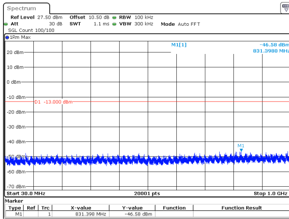
30MHz_15kHz_3715MHz_DFT-s-OFDM QPSK_RB1@0&amp;-46.58 dBm
