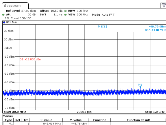
60MHz_30kHz_3730MHz_DFT-s-OFDM QPSK_RB162@0&amp;-46.76 dBm
