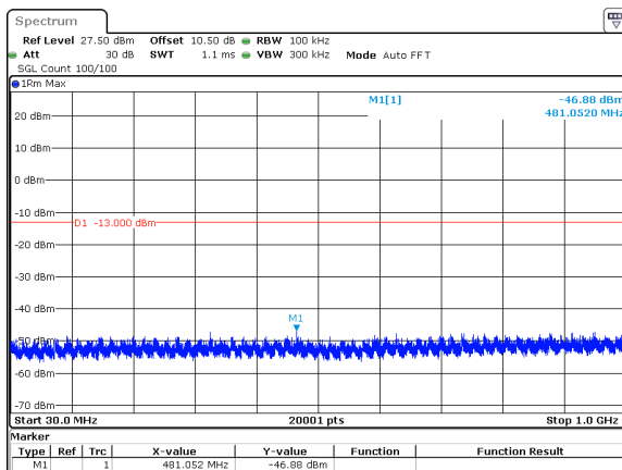
50MHz_15kHz_3725MHz_DFT-s-OFDM QPSK_RB270@0&amp;-46.88 dBm
