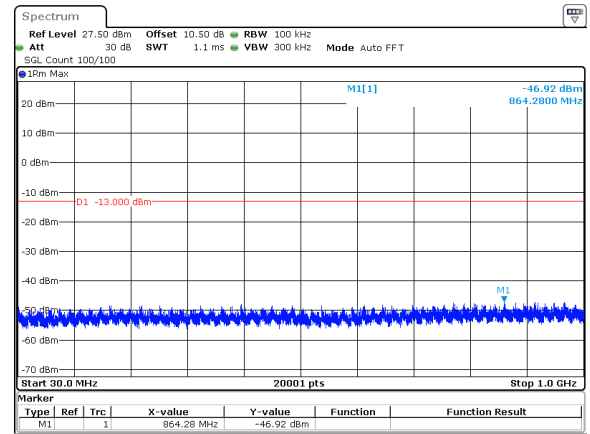
90MHz_30kHz_3840MHz_DFT-s-OFDM QPSK_RB1@0&amp;-46.92 dBm
