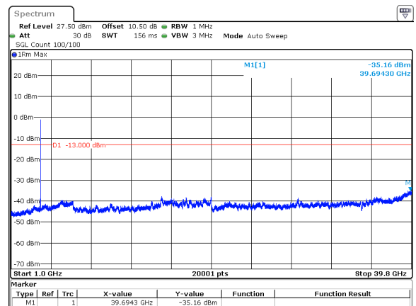
30MHz_15kHz_3840MHz_DFT-s-OFDM QPSK_RB160@0&amp;-35.16 dBm
