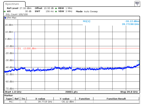
50MHz_15kHz_3955MHz_DFT-s-OFDM QPSK_RB1@0&amp;-35.12 dBm
