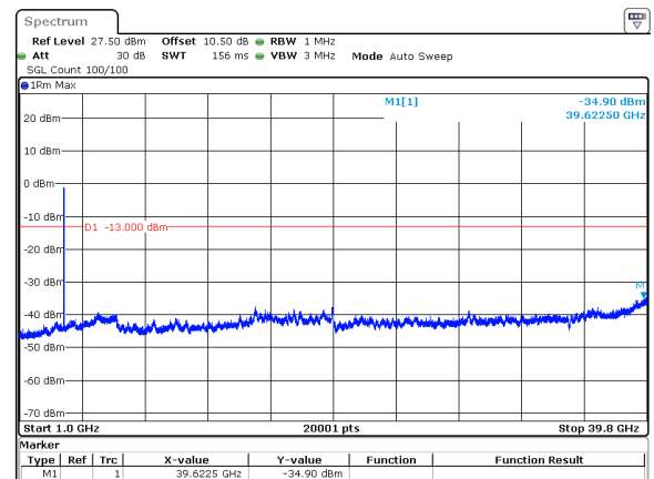
40MHz_15kHz_3720MHz_DFT-s-OFDM QPSK_RB216@0&amp;-34.90 dBm
