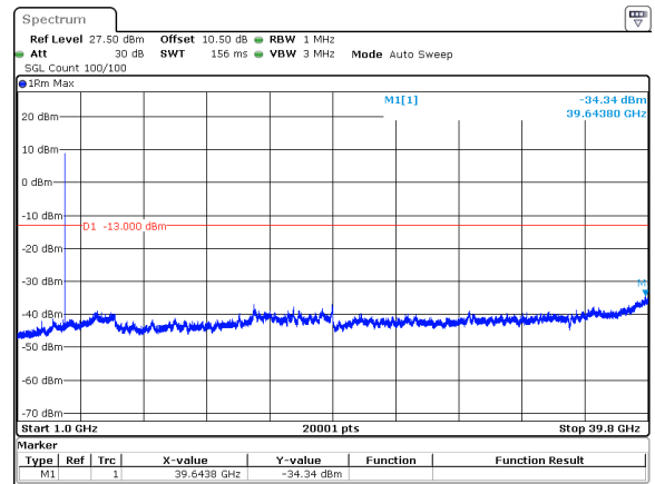
80MHz_30kHz_3840MHz_DFT-s-OFDM QPSK_RB1@216&amp;-34.34 dBm
