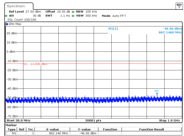
50MHz_15kHz_3955MHz_DFT-s-OFDM QPSK_RB1@269&amp;-46.56 dBm
