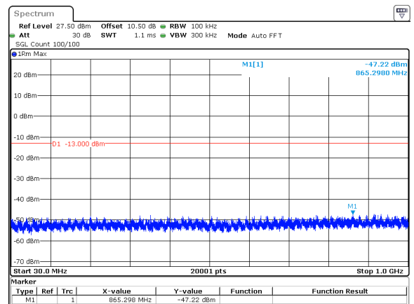
40MHz_30kHz_3840MHz_DFT-s-OFDM QPSK_RB1@105&amp;-47.22 dBm
