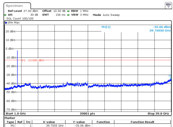
30MHz_15kHz_3965MHz_DFT-s-OFDM QPSK_RB160@0&amp;-35.06 dBm
