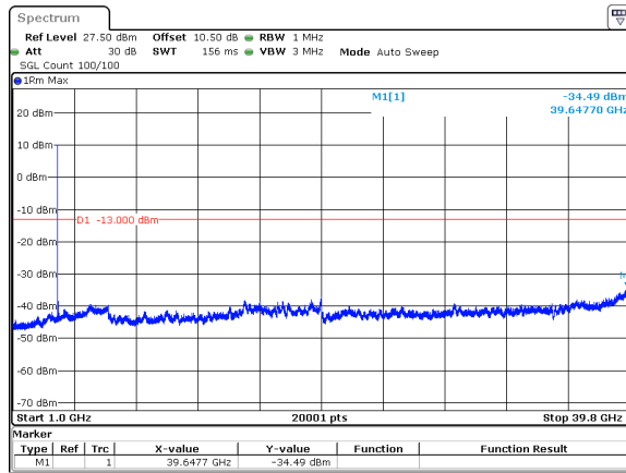
40MHz_15kHz_3840MHz_DFT-s-OFDM QPSK_RB1@0&amp;-34.49 dBm
