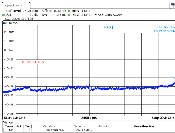
70MHz_30kHz_3840MHz_DFT-s-OFDM QPSK_RB1@188&amp;-34.90 dBm
