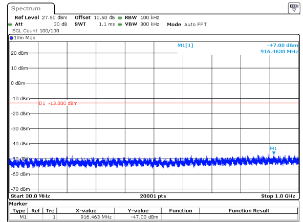
100MHz_30kHz_3930MHz_DFT-s-OFDM QPSK_RB1@272&amp;-47.00 dBm
