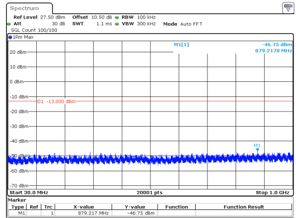
60MHz_30kHz_3840MHz_DFT-s-OFDM QPSK_RB1@0&amp;-46.75 dBm
