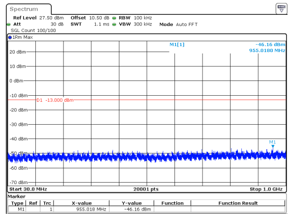
40MHz_30kHz_3840MHz_DFT-s-OFDM QPSK_RB1@0&amp;-46.16 dBm
