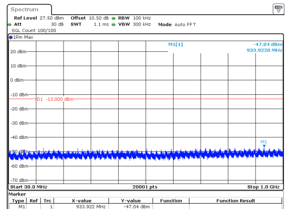
80MHz_30kHz_3740MHz_DFT-s-OFDM QPSK_RB216@0&amp;-47.04 dBm
