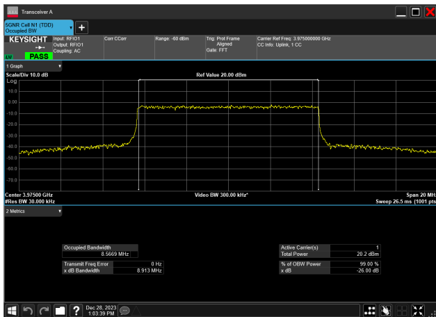
10MHz_30kHz_3975MHz_CP-OFDM 16 QAM_RB24@0 8.567 MHz
