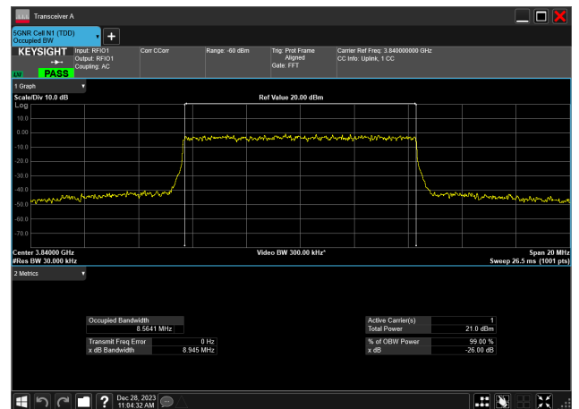
10MHz_30kHz_3840MHz_DFT-s-OFDM 64 QAM_RB24@0 8.564 MHz
