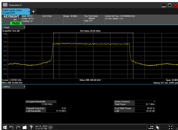
15MHz_15kHz_3707.5MHz_DFT-s-OFDM PI/2 BPSK_RB75@0 13.995 MHz
