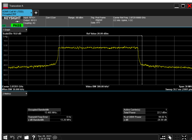
15MHz_30kHz_3972.5MHz_DFT-s-OFDM QPSK_RB36@0 13.465 MHz
