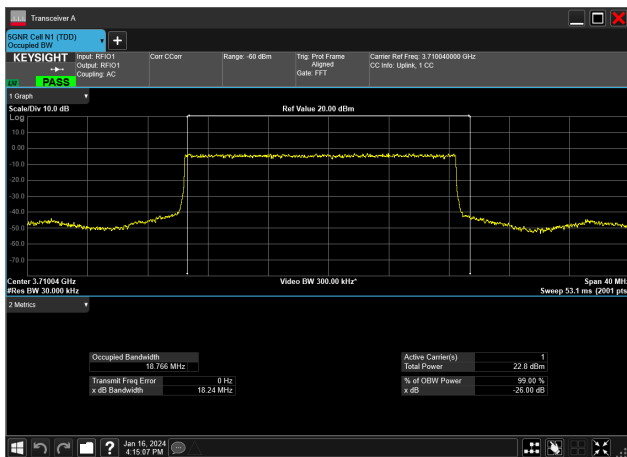
20MHz_15kHz_3710MHz_DFT-s-OFDM PI/2 BPSK_RB100@0 18.766 MHz
