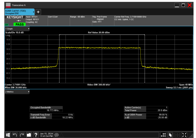
20MHz_15kHz_3710MHz_DFT-s-OFDM 64 QAM_RB100@0 18.773 MHz
