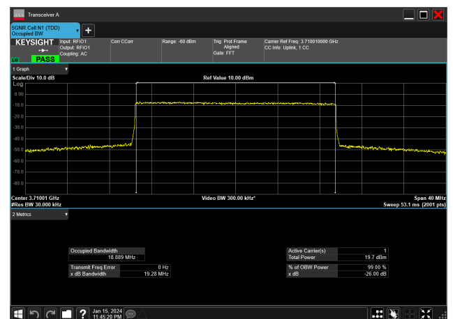
20MHz_15kHz_3710MHz_CP-OFDM 64 QAM_RB106@0 18.889 MHz
