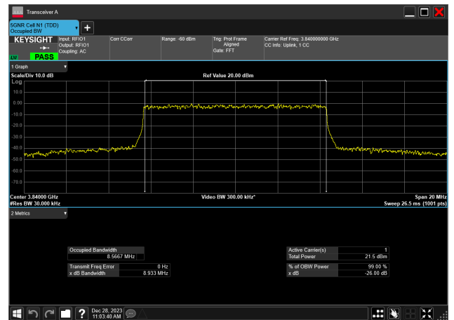
10MHz_30kHz_3840MHz_DFT-s-OFDM 16 QAM_RB24@0 8.567 MHz
