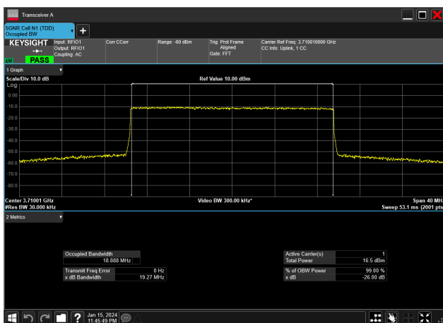
20MHz_15kHz_3710MHz_CP-OFDM 256 QAM_RB106@0 18.888 MHz
