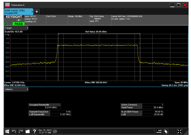
10MHz_15kHz_3975MHz_DFT-s-OFDM 64 QAM_RB50@0 9.214 MHz
