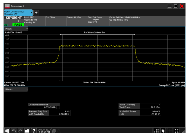
10MHz_30kHz_3840MHz_CP-OFDM 64 QAM_RB24@0 8.570 MHz
