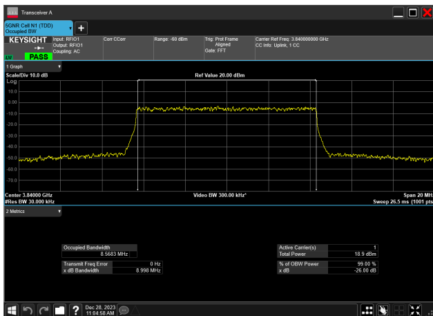
10MHz_30kHz_3840MHz_DFT-s-OFDM 256 QAM_RB24@0 8.568 MHz
