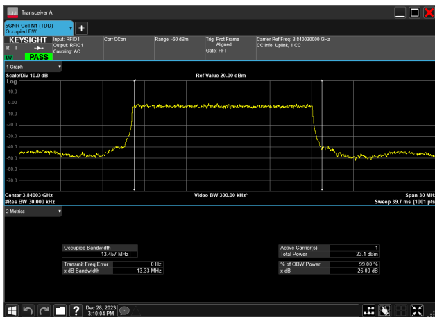
15MHz_30kHz_3840MHz_DFT-s-OFDM PI/2 BPSK_RB36@0 13.457 MHz
