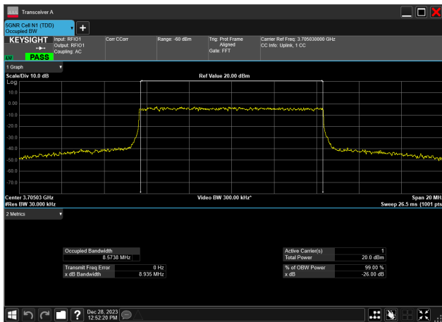
10MHz_30kHz_3705MHz_CP-OFDM 64 QAM_RB24@0 8.574 MHz
