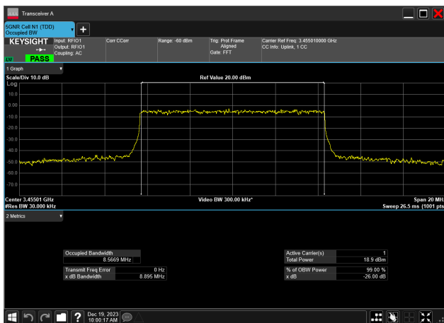
10MHz_30kHz_3455MHz_DFT-s-OFDM 256 QAM_RB24@0 8.567 MHz
