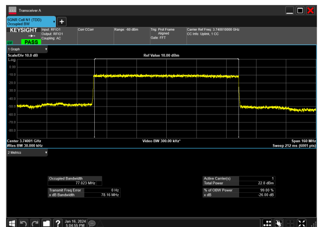
80MHz_30kHz_3740MHz_DFT-s-OFDM QPSK_RB216@0 77.023 MHz
