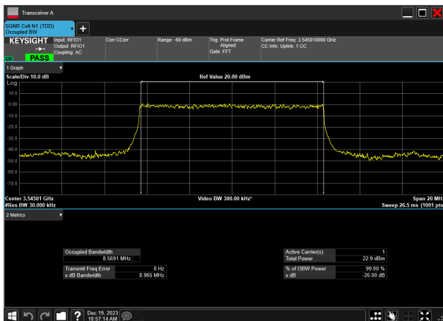
10MHz_30kHz_3545MHz_DFT-s-OFDM PI/2 BPSK_RB24@0 8.569 MHz
