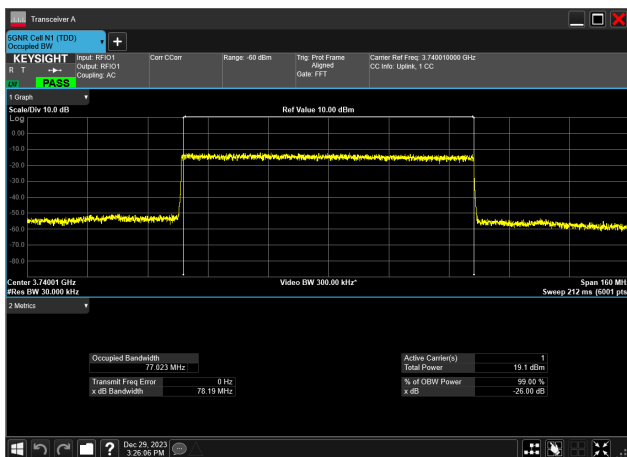
80MHz_30kHz_3740MHz_DFT-s-OFDM 256 QAM_RB216@0 77.023 MHz
