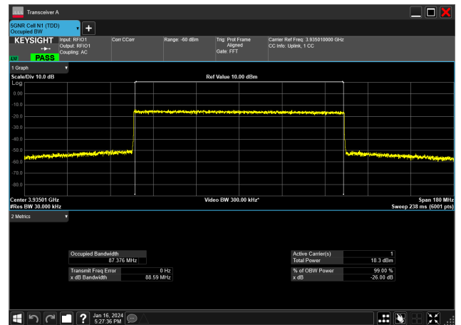
90MHz_30kHz_3935MHz_CP-OFDM 256 QAM_RB245@0 87.376 MHz
