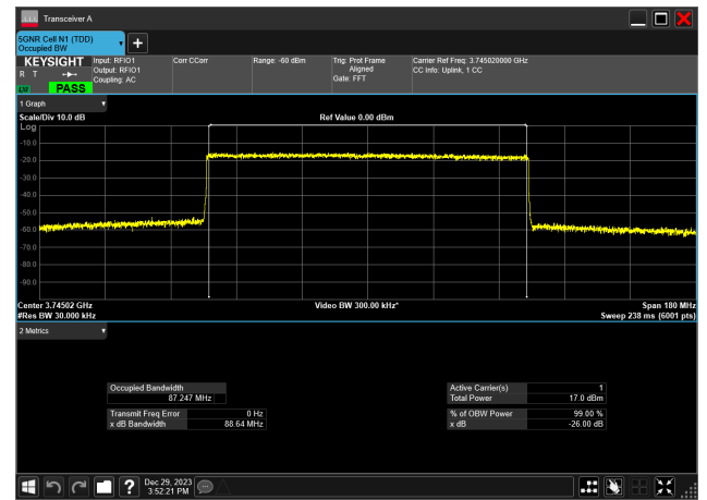
90MHz_30kHz_3745MHz_CP-OFDM 256 QAM_RB245@0 87.247 MHz
