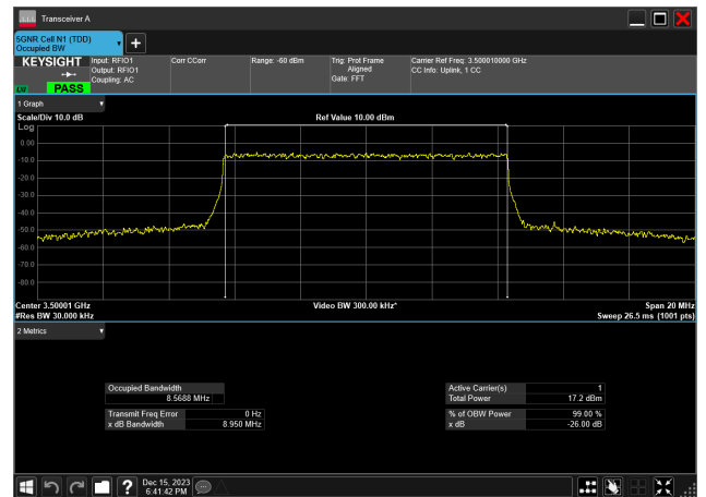
10MHz_30kHz_3500MHz_CP-OFDM 256 QAM_RB24@0 8.569 MHz
