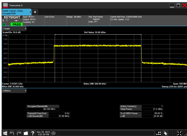
90MHz_30kHz_3935MHz_DFT-s-OFDM 16 QAM_RB243@0 86.546 MHz
