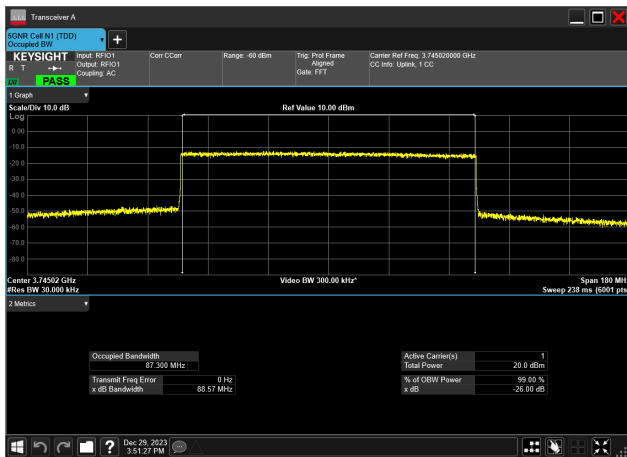
90MHz_30kHz_3745MHz_CP-OFDM 64 QAM_RB245@0 87.300 MHz
