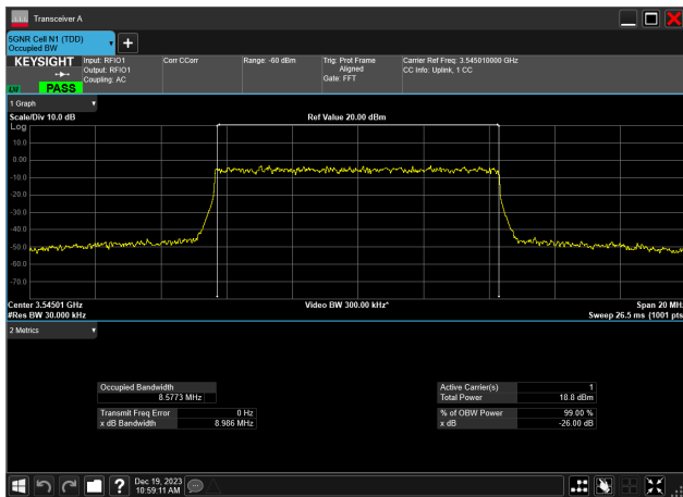
10MHz_30kHz_3545MHz_DFT-s-OFDM 256 QAM_RB24@0 8.577 MHz
