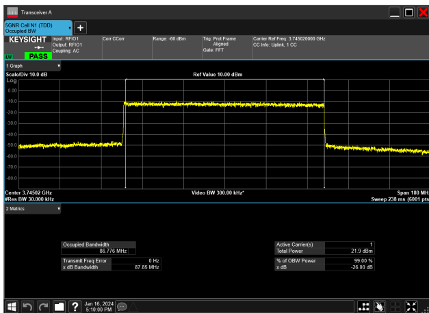
90MHz_30kHz_3745MHz_DFT-s-OFDM 16 QAM_RB243@0 86.776 MHz
