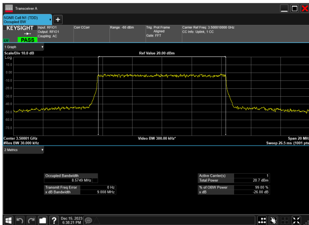
10MHz_30kHz_3500MHz_DFT-s-OFDM 64 QAM_RB24@0 8.575 MHz
