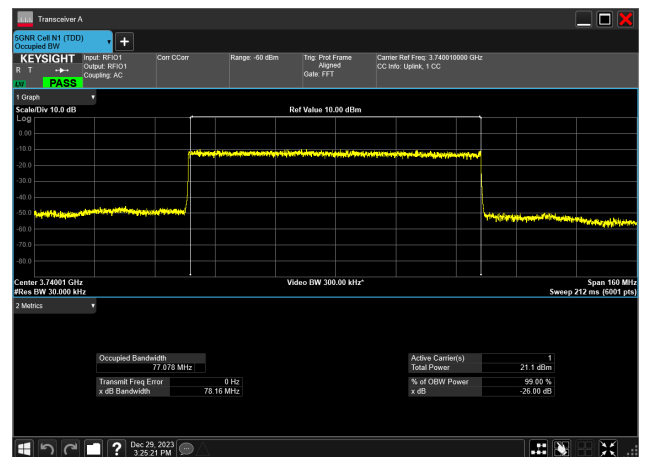
80MHz_30kHz_3740MHz_DFT-s-OFDM 64 QAM_RB216@0 77.078 MHz
