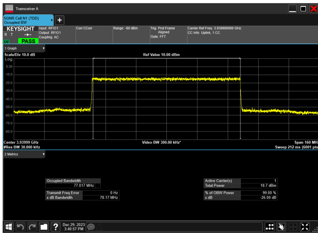
80MHz_30kHz_3940MHz_DFT-s-OFDM 256 QAM_RB216@0 77.017 MHz
