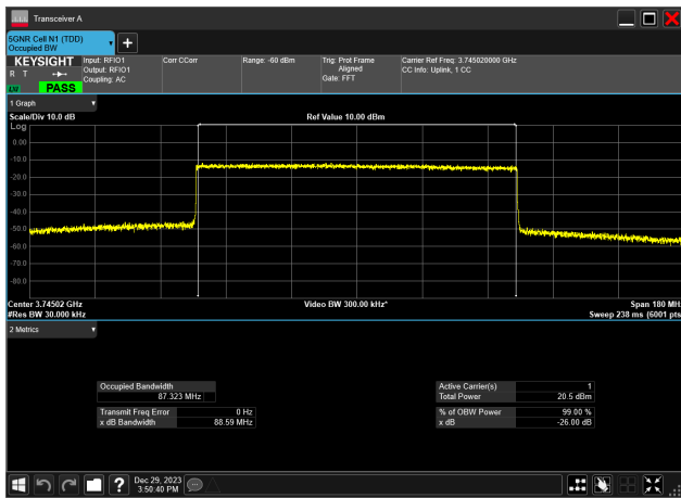
90MHz_30kHz_3745MHz_CP-OFDM 16 QAM_RB245@0 87.323 MHz
