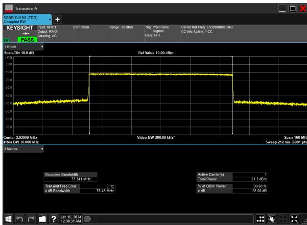
80MHz_30kHz_3940MHz_CP-OFDM QPSK_RB217@0 77.341 MHz
