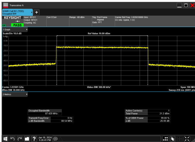
90MHz_30kHz_3935MHz_CP-OFDM 64 QAM_RB245@0 87.429 MHz
