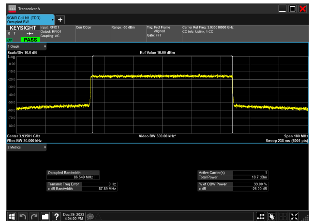
90MHz_30kHz_3935MHz_DFT-s-OFDM 256 QAM_RB243@0 86.549 MHz
