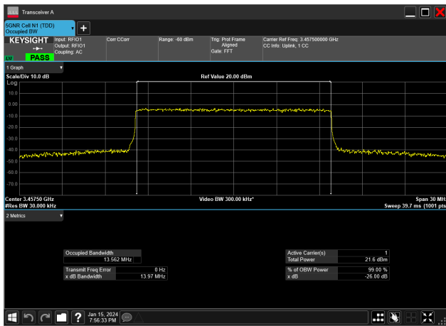
15MHz_30kHz_3457.5MHz_CP-OFDM 16 QAM_RB38@0 13.562 MHz
