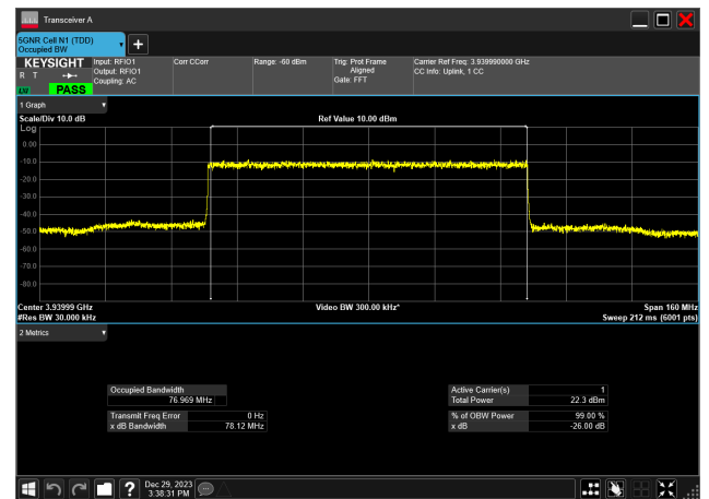
80MHz_30kHz_3940MHz_DFT-s-OFDM QPSK_RB216@0 76.969 MHz
