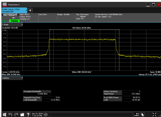
15MHz_30kHz_3457.5MHz_DFT-s-OFDM 16 QAM_RB36@0 13.460 MHz
