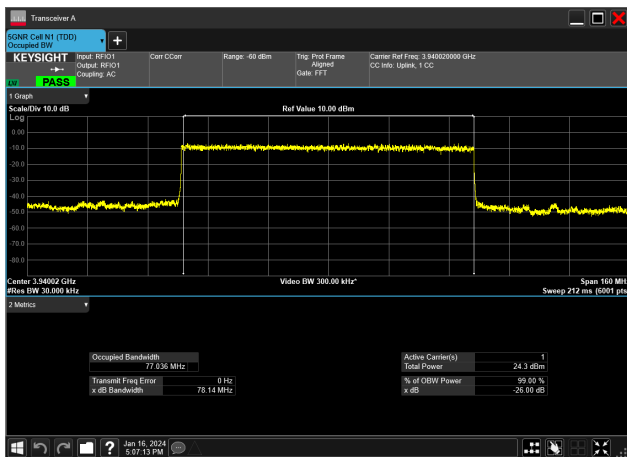
80MHz_30kHz_3940MHz_DFT-s-OFDM PI/2 BPSK_RB216@0 77.036 MHz
