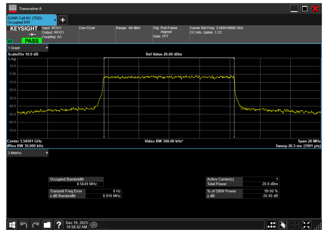
10MHz_30kHz_3545MHz_DFT-s-OFDM 64 QAM_RB24@0 8.565 MHz
