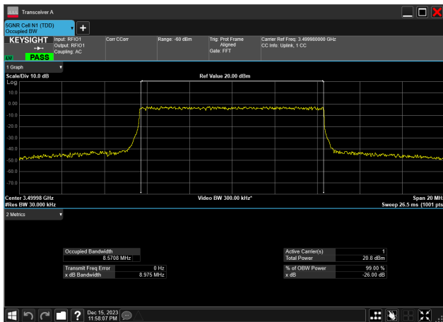
10MHz_30kHz_3500MHz_CP-OFDM 16 QAM_RB24@0 8.571 MHz
