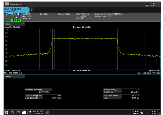
10MHz_30kHz_3545MHz_CP-OFDM 16 QAM_RB24@0 8.570 MHz
