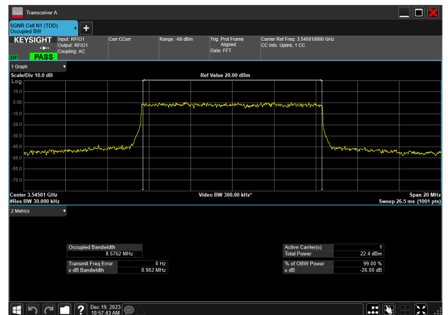
10MHz_30kHz_3545MHz_DFT-s-OFDM QPSK_RB24@0 8.576 MHz
