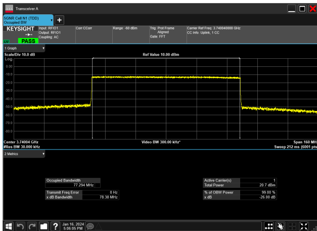
80MHz_30kHz_3740MHz_CP-OFDM QPSK_RB217@0 77.294 MHz
