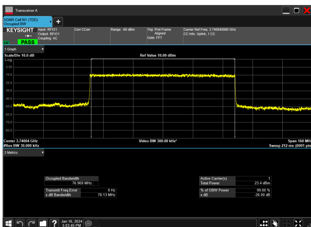
80MHz_30kHz_3740MHz_DFT-s-OFDM PI/2 BPSK_RB216@0 76.969 MHz
