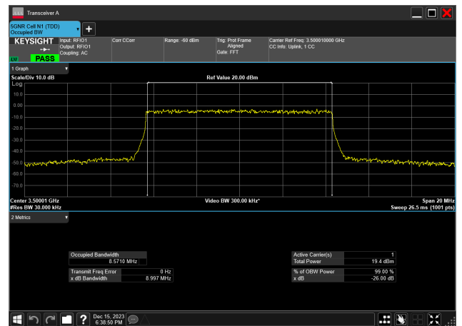
10MHz_30kHz_3500MHz_DFT-s-OFDM 256 QAM_RB24@0 8.571 MHz
