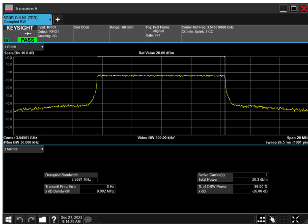
10MHz_30kHz_3545MHz_CP-OFDM QPSK_RB24@0 8.568 MHz
