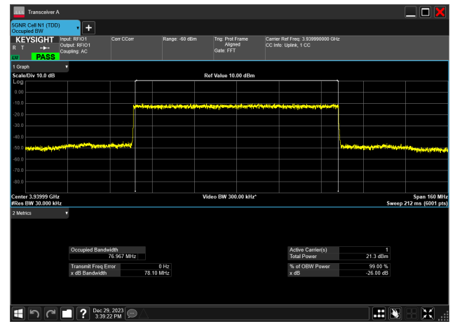
80MHz_30kHz_3940MHz_DFT-s-OFDM 16 QAM_RB216@0 76.967 MHz
