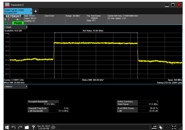
80MHz_30kHz_3740MHz_DFT-s-OFDM 16 QAM_RB216@0 77.015 MHz
