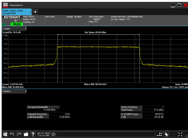
15MHz_30kHz_3457.5MHz_CP-OFDM 64 QAM_RB38@0 13.569 MHz
