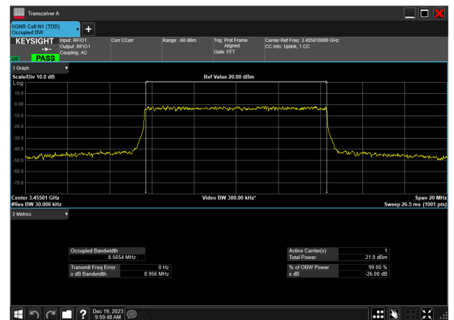
10MHz_30kHz_3455MHz_DFT-s-OFDM 64 QAM_RB24@0 8.565 MHz
