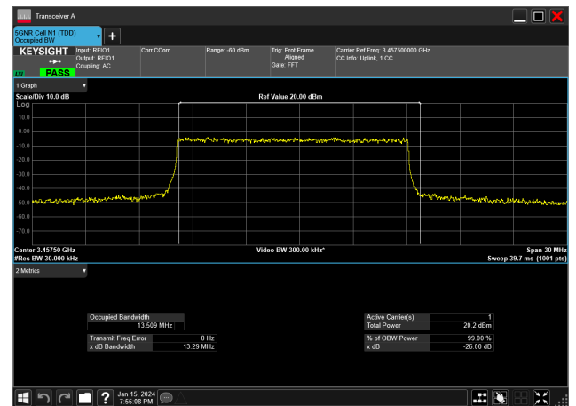
15MHz_30kHz_3457.5MHz_DFT-s-OFDM 256 QAM_RB36@0 13.509 MHz
