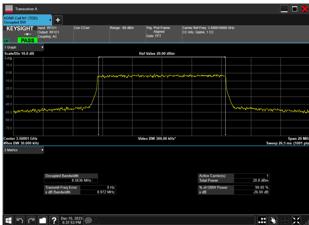
10MHz_30kHz_3500MHz_DFT-s-OFDM 16 QAM_RB24@0 8.564 MHz
