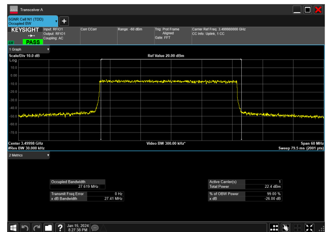
30MHz_30kHz_3500MHz_DFT-s-OFDM 64 QAM_RB75@0 27.619 MHz
