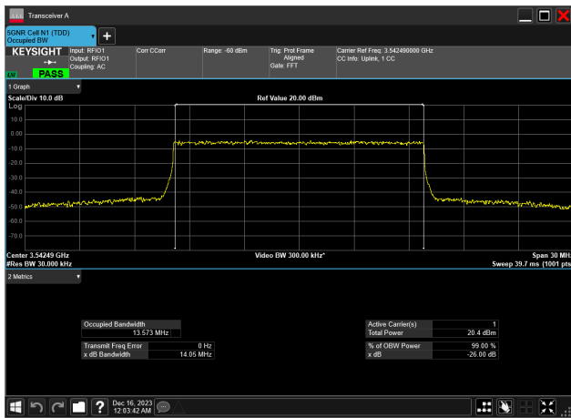
15MHz_30kHz_3542.5MHz_CP-OFDM 16 QAM_RB38@0 13.573 MHz
