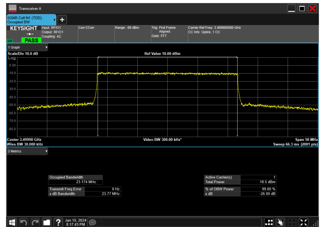
25MHz_30kHz_3500MHz_CP-OFDM 256 QAM_RB65@0 23.174 MHz
