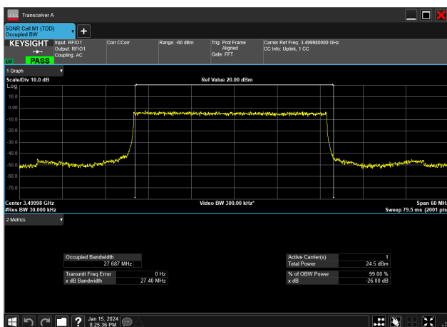
30MHz_30kHz_3500MHz_DFT-s-OFDM PI/2 BPSK_RB75@0 27.687 MHz
