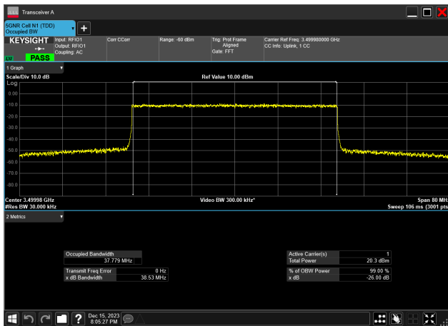
40MHz_30kHz_3500MHz_CP-OFDM 64 QAM_RB106@0 37.779 MHz
