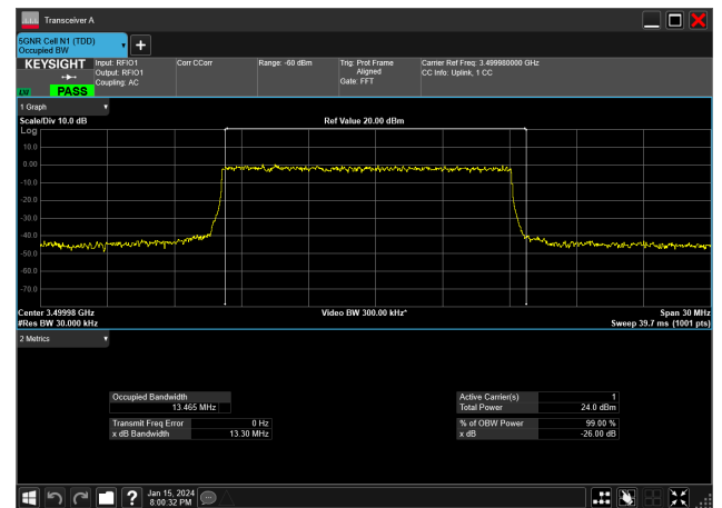
15MHz_30kHz_3500MHz_DFT-s-OFDM QPSK_RB36@0 13.465 MHz
