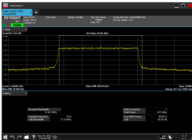
15MHz_30kHz_3542.5MHz_DFT-s-OFDM 16 QAM_RB36@0 13.451 MHz
