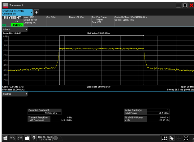
15MHz_30kHz_3542.5MHz_CP-OFDM 64 QAM_RB38@0 13.565 MHz
