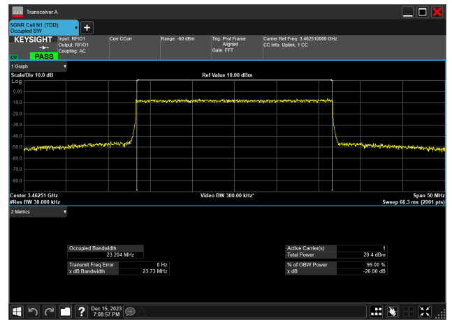
25MHz_30kHz_3462.5MHz_CP-OFDM 16 QAM_RB65@0 23.204 MHz
