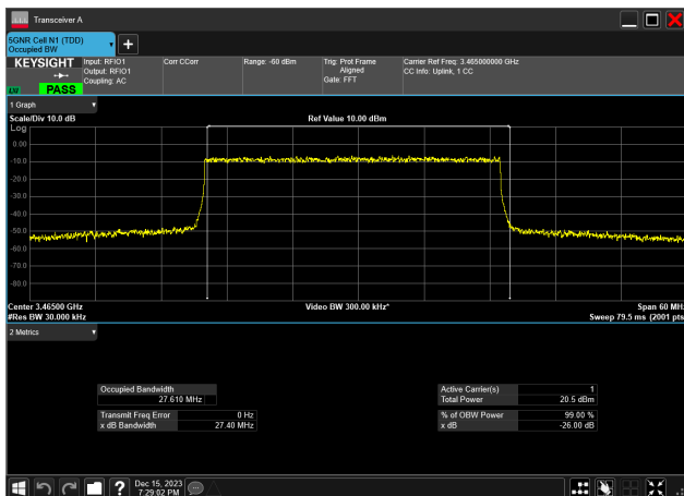
30MHz_30kHz_3465MHz_DFT-s-OFDM 16 QAM_RB75@0 27.610 MHz
