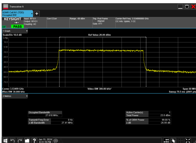
30MHz_30kHz_3535MHz_DFT-s-OFDM 16 QAM_RB75@ 27.618 MHz
