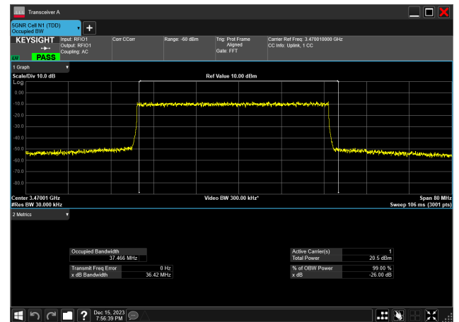
40MHz_30kHz_3470MHz_DFT-s-OFDM 16 QAM_RB100@0 37.466 MHz
