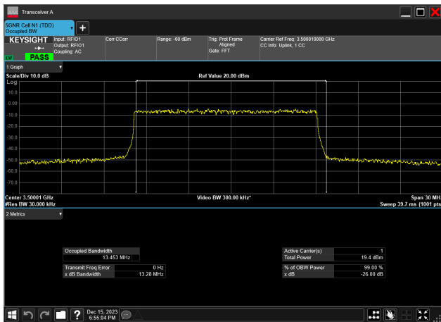
15MHz_30kHz_3500MHz_DFT-s-OFDM 256 QAM_RB36@0 13.453 MHz
