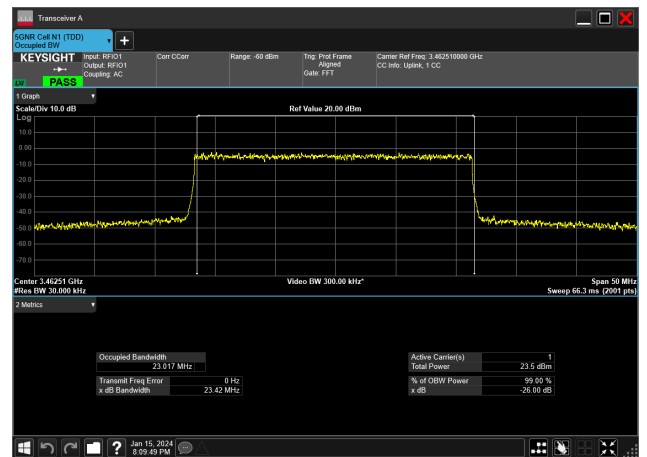
25MHz_30kHz_3462.5MHz_DFT-s-OFDM_QPSK_RB64@0 23.017 MHz
