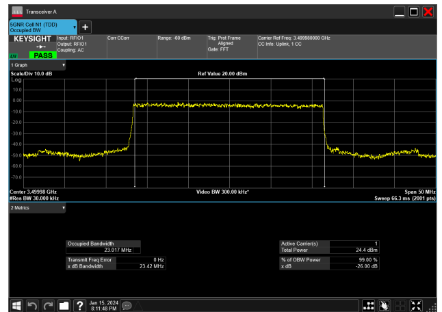
25MHz_30kHz_3500MHz_DFT-s-OFDM PI/2 BPSK_RB64@0 23.017 MHz
