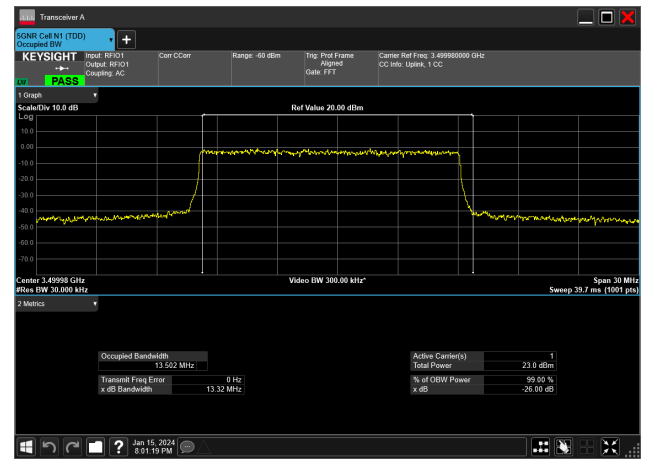
15MHz_30kHz_3500MHz_DFT-s-OFDM 16 QAM_RB36@0 13.502 MHz
