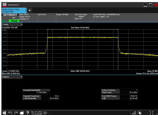
30MHz_30kHz_3535MHz_CP-OFDM 64 QAM_RB78@ 27.804 MHz
