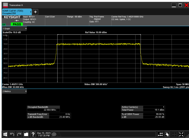
25MHz_30kHz_3462.5MHz_DFT-s-OFDM_256_QAM_RB64@0 22.904 MHz
