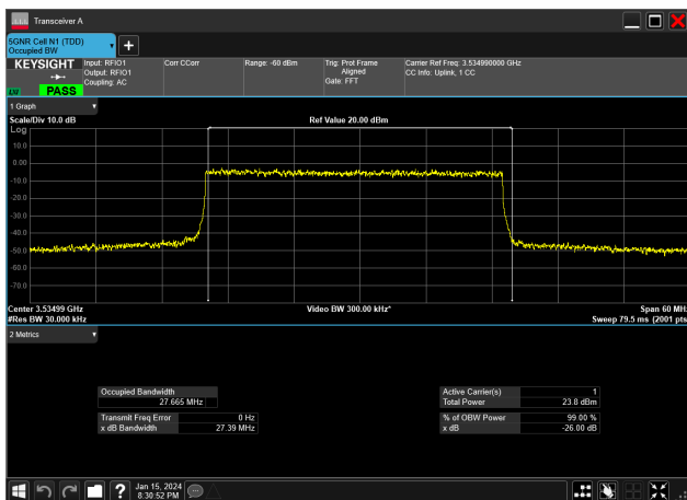
30MHz_30kHz_3535MHz_DFT-s-OFDM QPSK_RB75@0 27.665 MHz
