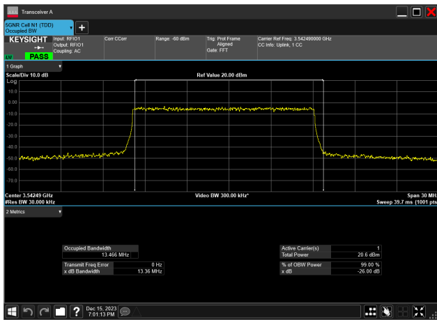
15MHz_30kHz_3542.5MHz_DFT-s-OFDM 64 QAM_RB36@0 13.466 MHz
