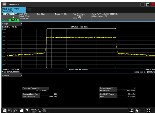
25MHz_30kHz_3462.5MHz_CP-OFDM 256 QAM_RB65@0 23.164 MHz
