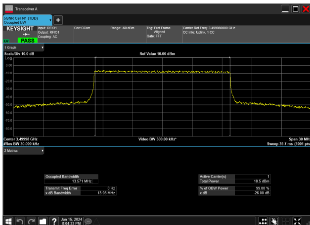
15MHz_30kHz_3500MHz_CP-OFDM 256 QAM_RB38@0 13.571 MHz
