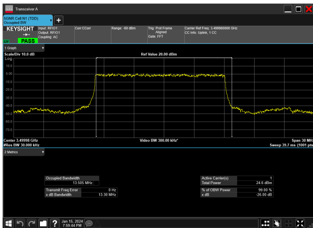
15MHz_30kHz_3500MHz_DFT-s-OFDM PI/2 BPSK_RB36@0 13.505 MHz
