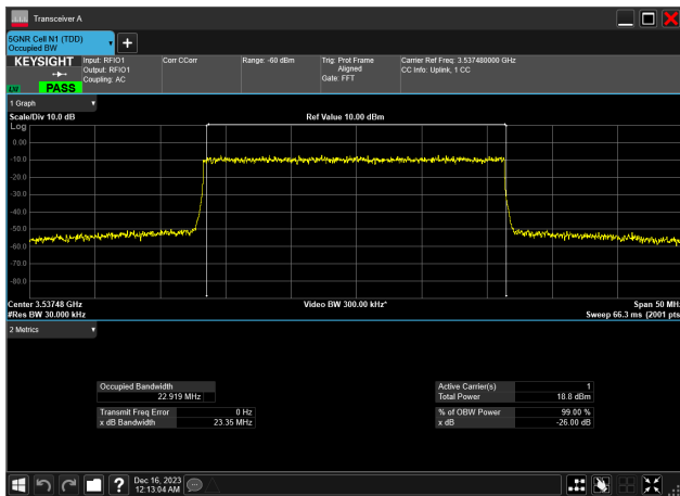
25MHz_30kHz_3537.5MHz_DFT-s-OFDM 256 QAM_RB64@0 22.919 MHz
