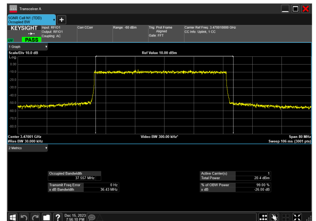
40MHz_30kHz_3470MHz_DFT-s-OFDM QPSK_RB100@0 37.557 MHz
