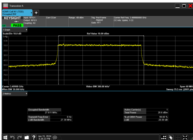
30MHz_30kHz_3500MHz_DFT-s-OFDM 256 QAM_RB75@0 27.611 MHz
