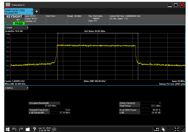
30MHz_30kHz_3500MHz_DFT-s-OFDM 16 QAM_RB75@0 27.629 MHz
