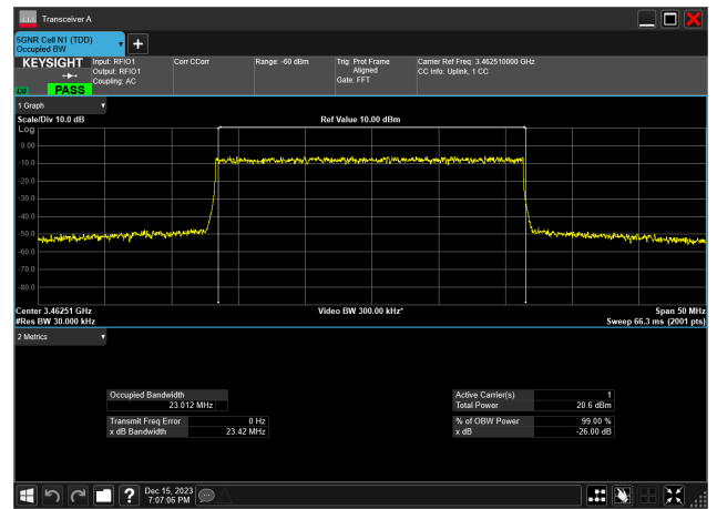
25MHz_30kHz_3462.5MHz_DFT-s-OFDM_64_QAM_RB64@0 23.012 MHz
