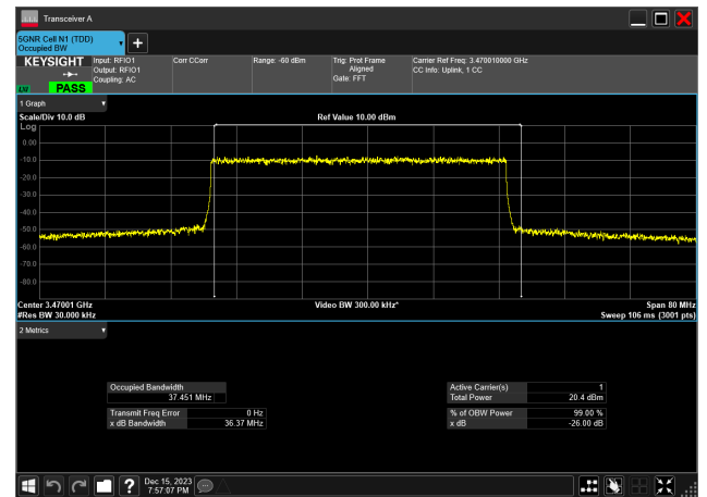
40MHz_30kHz_3470MHz_DFT-s-OFDM 64 QAM_RB100@0 37.451 MHz
