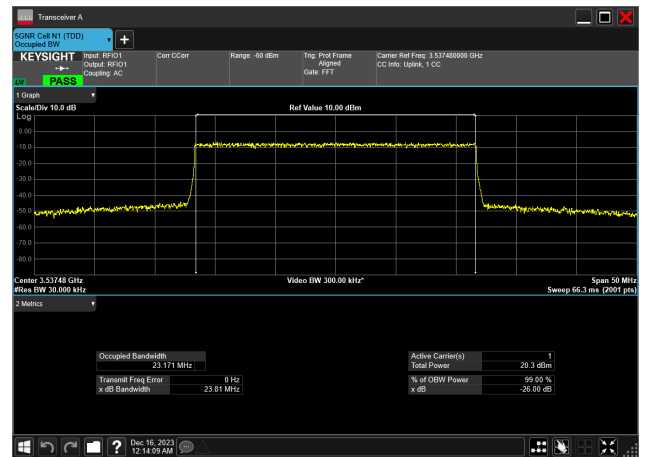
25MHz_30kHz_3537.5MHz_CP-OFDM 16 QAM_RB65@0 23.171 MHz
