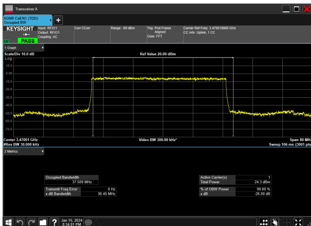
40MHz_30kHz_3470MHz_DFT-s-OFDM PI/2 BPSK_RB100@0 37.509 MHz
