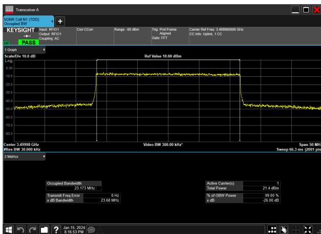
25MHz_30kHz_3500MHz_CP-OFDM 64 QAM_RB65@0 23.173 MHz
