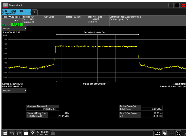
25MHz_30kHz_3537.5MHz_DFT-s-OFDM PI/2 BPSK_RB64@0 23.061 MHz
