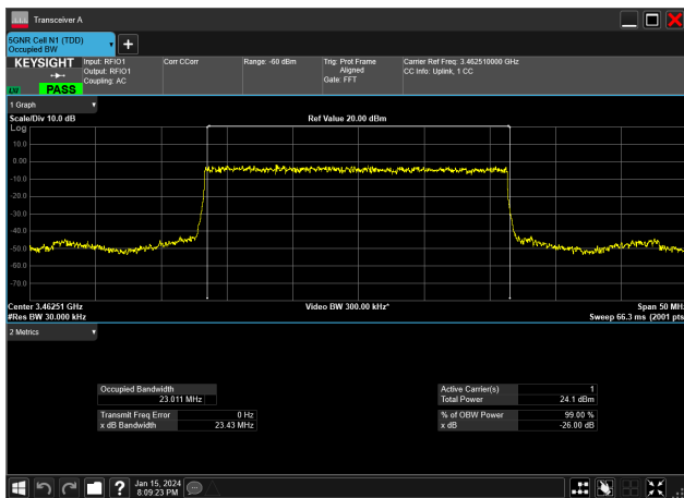
25MHz_30kHz_3462.5MHz_DFT-s-OFDM_PI/2_BPSK_RB64@0 23.011 MHz
