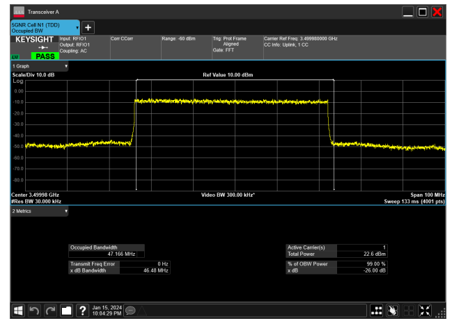
50MHz_30kHz_3500MHz_DFT-s-OFDM 64 QAM_RB128@0 47.166 MHz
