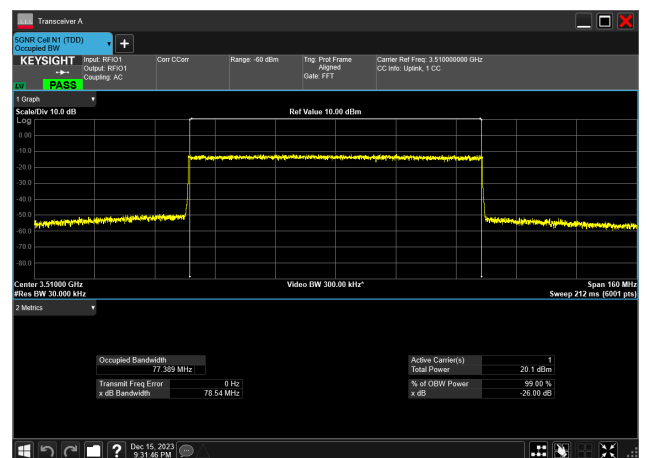
80MHz_30kHz_3510MHz_CP-OFDM 64 QAM_RB217@0 77.389 MHz
