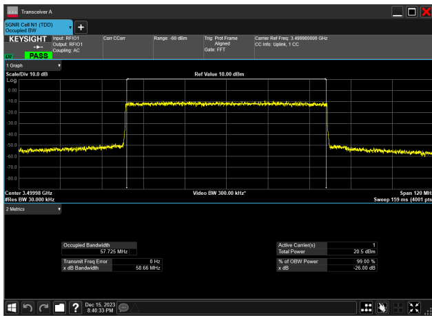
60MHz_30kHz_3500MHz_DFT-s-OFDM 64 QAM_RB162@0 57.725 MHz
