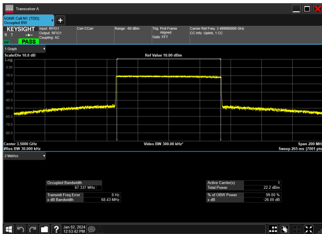
70MHz_30kHz_3500MHz_CP-OFDM QPSK_RB189@0 67.337 MHz
