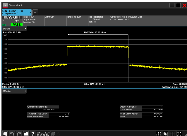
70MHz_30kHz_3500MHz_CP-OFDM 256 QAM_RB189@0 67.337 MHz
