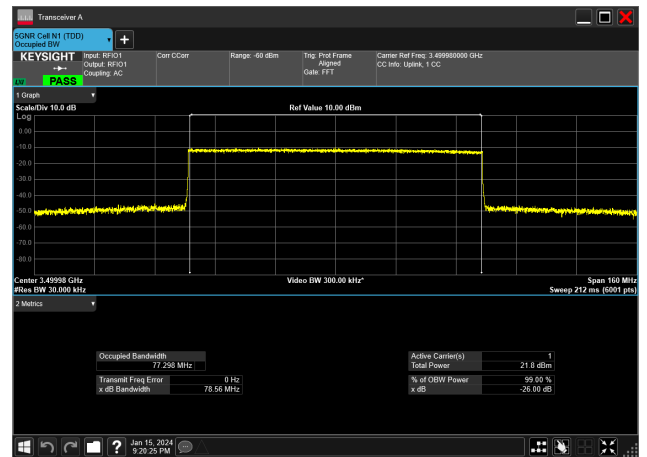
80MHz_30kHz_3500MHz_CP-OFDM QPSK_RB217@0 77.298 MHz
