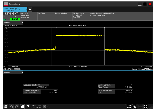
70MHz_30kHz_3500MHz_CP-OFDM 16 QAM_RB189@0 67.329 MHz
