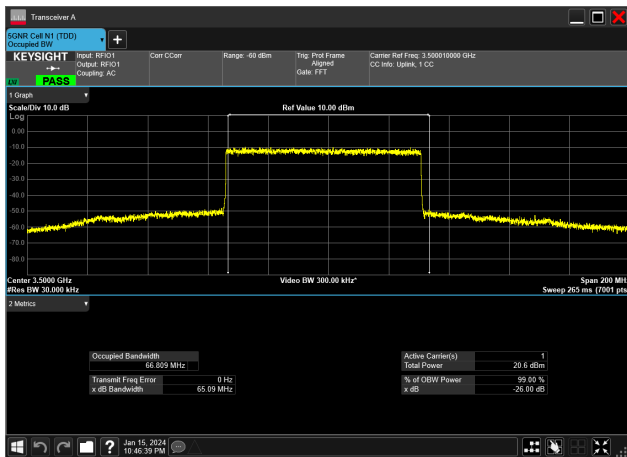
70MHz_30kHz_3500MHz_DFT-s-OFDM 256 QAM_RB180@0 66.809 MHz
