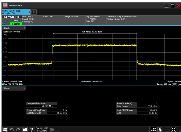
80MHz_30kHz_3490MHz_DFT-s-OFDM 256 QAM_RB216@0 76.982 MHz
