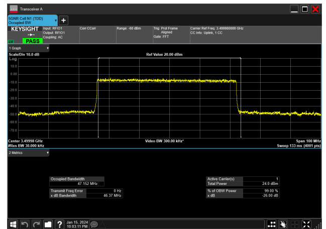
50MHz_30kHz_3500MHz_DFT-s-OFDM QPSK_RB128@0 47.152 MHz
