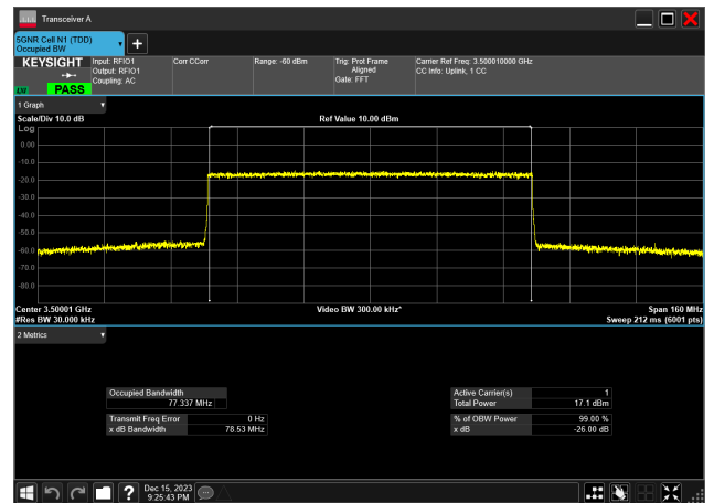
80MHz_30kHz_3500MHz_CP-OFDM 256 QAM_RB217@0 77.337 MHz
