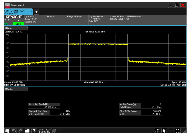
70MHz_30kHz_3500MHz_CP-OFDM 64 QAM_RB189@0 67.320 MHz
