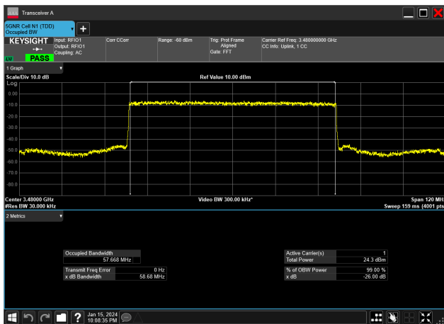
60MHz_30kHz_3480MHz_DFT-s-OFDM PI/2 BPSK_RB162@0 57.668 MHz
