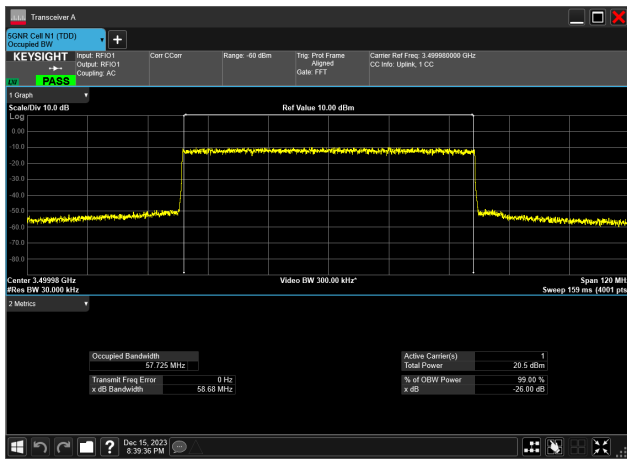
60MHz_30kHz_3500MHz_DFT-s-OFDM QPSK_RB162@0 57.725 MHz
