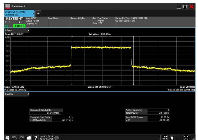
70MHz_30kHz_3485MHz_DFT-s-OFDM 256 QAM_RB180@0 66.918 MHz
