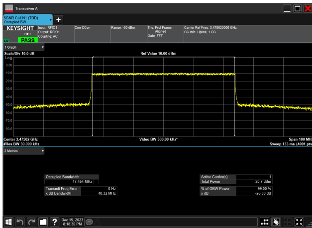
50MHz_30kHz_3475MHz_CP-OFDM 16 QAM_RB133@0 47.454 MHz
