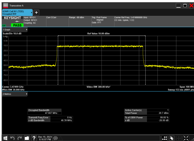
50MHz_30kHz_3475MHz_DFT-s-OFDM 16 QAM_RB128@0 47.007 MHz
