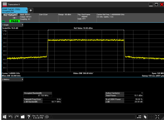
60MHz_30kHz_3480MHz_DFT-s-OFDM 256 QAM_RB162@0 57.750 MHz
