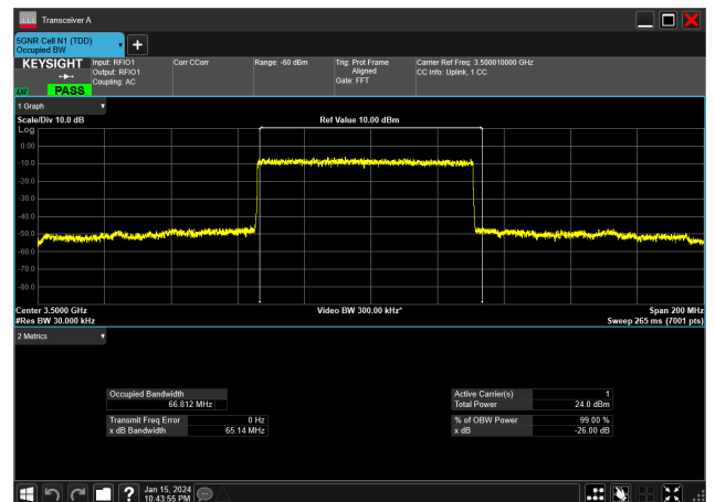
70MHz_30kHz_3500MHz_DFT-s-OFDM QPSK_RB180@0 66.812 MHz
