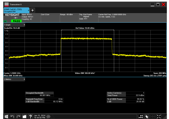
70MHz_30kHz_3500MHz_DFT-s-OFDM 16 QAM_RB180@0 66.881 MHz
