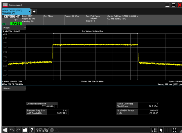
80MHz_30kHz_3500MHz_CP-OFDM 64 QAM_RB217@0 77.354 MHz
