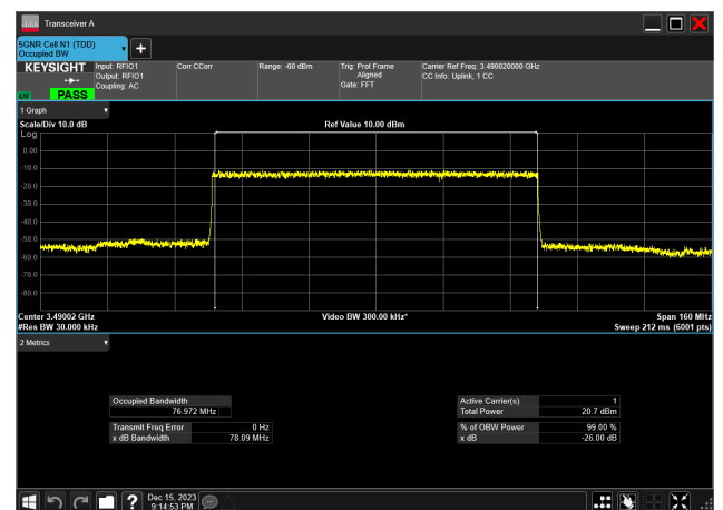
80MHz_30kHz_3490MHz_DFT-s-OFDM QPSK_RB216@0 76.972 MHz
