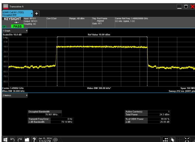
80MHz_30kHz_3490MHz_DFT-s-OFDM PI/2 BPSK_RB216@0 76.961 MHz
