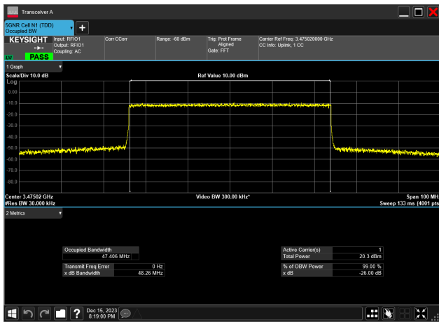
50MHz_30kHz_3475MHz_CP-OFDM 64 QAM_RB133@0 47.406 MHz
