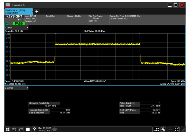
80MHz_30kHz_3490MHz_DFT-s-OFDM 16 QAM_RB216@0 77.014 MHz
