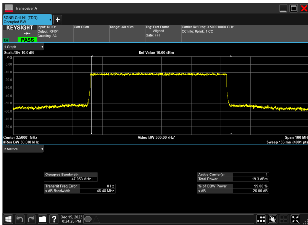
50MHz_30kHz_3500MHz_DFT-s-OFDM 256 QAM_RB128@0 47.053 MHz
