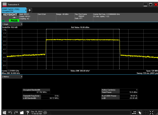
60MHz_30kHz_3520MHz_CP-OFDM 256 QAM_RB162@0 57.782 MHz
