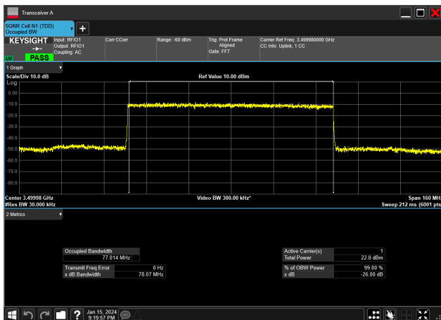
80MHz_30kHz_3500MHz_DFT-s-OFDM 16 QAM_RB216@0 77.014 MHz
