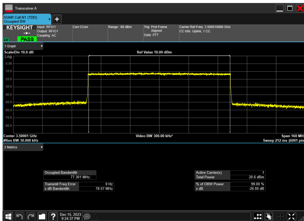
80MHz_30kHz_3500MHz_CP-OFDM 16 QAM_RB217@0 77.301 MHz
