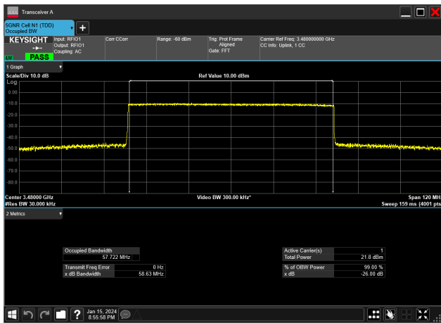
60MHz_30kHz_3480MHz_CP-OFDM QPSK_RB162@0 57.722 MHz
