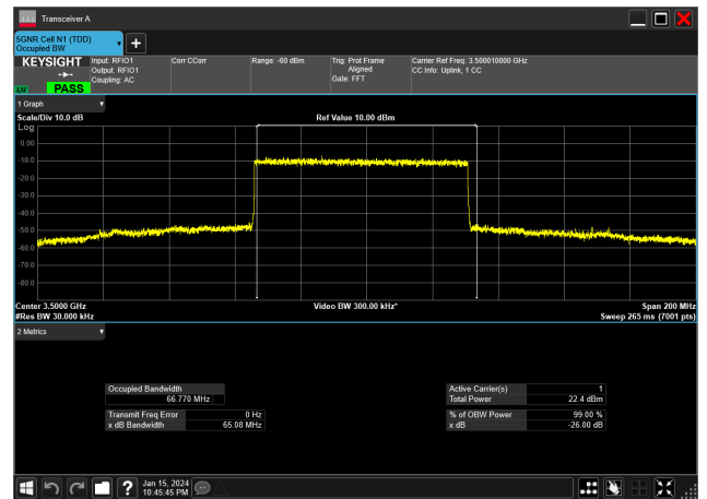
70MHz_30kHz_3500MHz_DFT-s-OFDM 64 QAM_RB180@0 66.770 MHz
