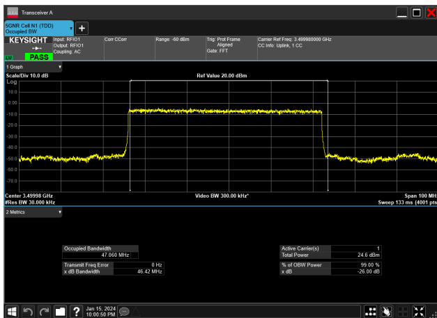
50MHz_30kHz_3500MHz_DFT-s-OFDM PI/2 BPSK_RB128@0 47.060 MHz
