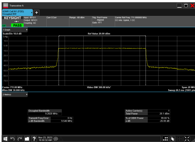
10MHz_15kHz_711MHz_CP-OFDM QPSK_RB52@0 9.282 MHz
