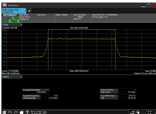
5MHz_15kHz_713.5MHz_DFT-s-OFDM 256 QAM_RB25@0 4.480 MHz
