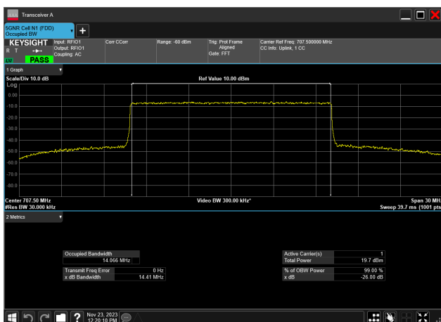
15MHz_15kHz_707.5MHz_CP-OFDM 64 QAM_RB79@0 14.066 MHz
