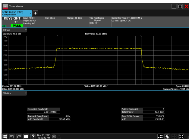
10MHz_15kHz_711MHz_CP-OFDM 64 QAM_RB52@0 9.284 MHz
