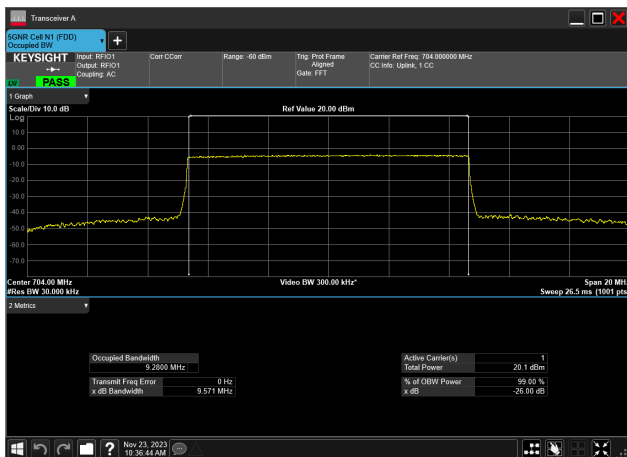
10MHz_15kHz_704MHz_CP-OFDM QPSK_RB52@0 9.280 MHz
