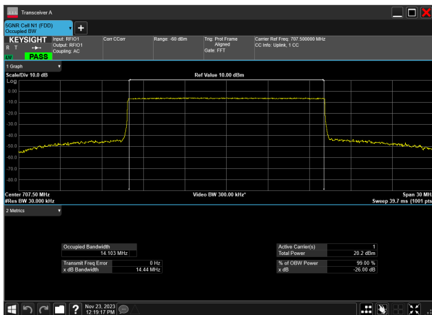
15MHz_15kHz_707.5MHz_CP-OFDM QPSK_RB79@0 14.103 MHz
