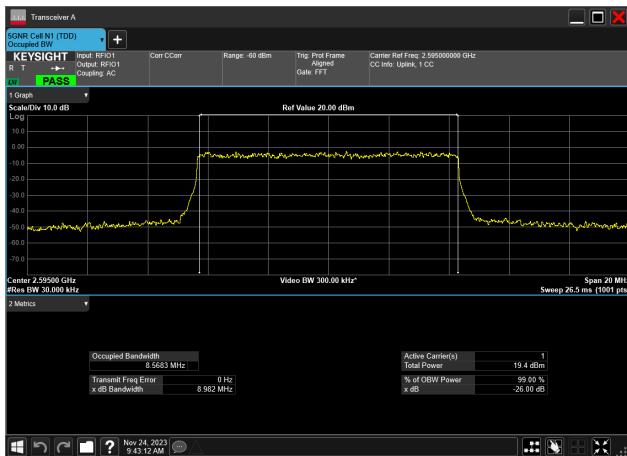
10MHz_30kHz_2595MHz_DFT-s-OFDM 64 QAM_RB24@0 8.568 MHz
