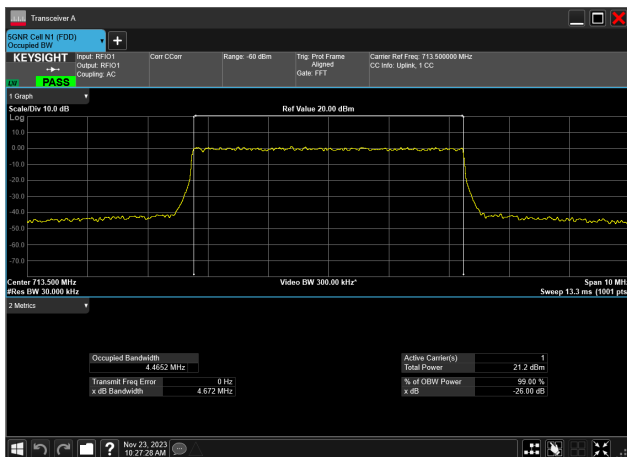
5MHz_15kHz_713.5MHz_DFT-s-OFDM 16 QAM_RB25@0 4.465 MHz
