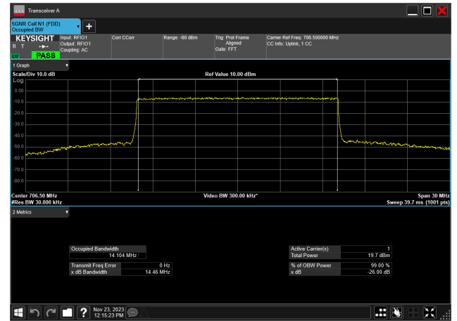
15MHz_15kHz_706.5MHz_CP-OFDM 64 QAM_RB79@0 14.104 MHz
