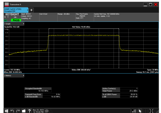
15MHz_15kHz_707.5MHz_CP-OFDM 16 QAM_RB79@0 14.103 MHz
