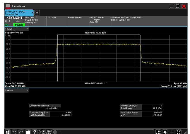
15MHz_15kHz_707.5MHz_CP-OFDM 256 QAM_RB79@0 14.103 MHz
