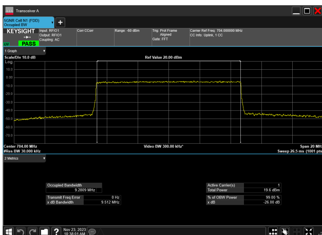
10MHz_15kHz_704MHz_CP-OFDM 64 QAM_RB52@0 9.281 MHz
