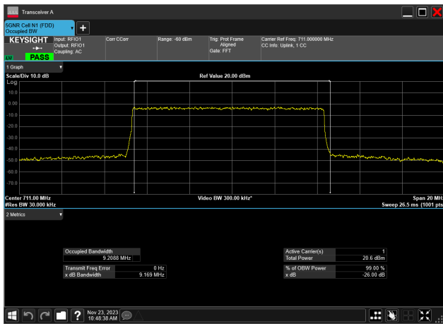
10MHz_15kHz_711MHz_DFT-s-OFDM 64 QAM_RB50@0 9.209 MHz
