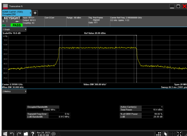
10MHz_30kHz_2595MHz_CP-OFDM 64 QAM_RB24@0 8.568 MHz
