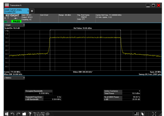
10MHz_15kHz_711MHz_CP-OFDM 256 QAM_RB52@0 9.260 MHz
