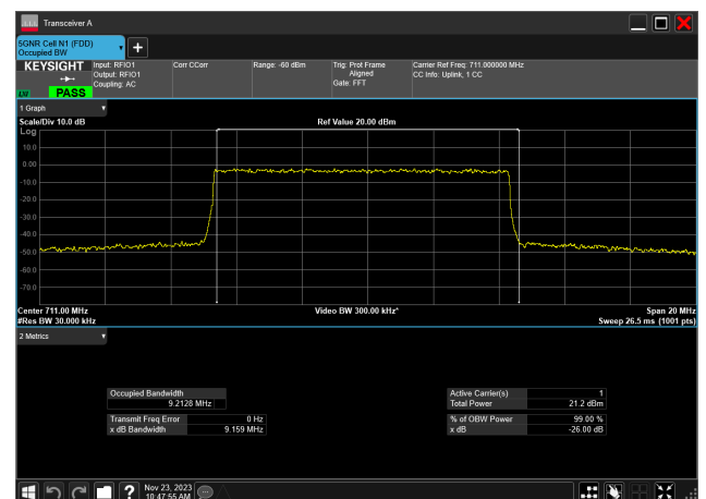
10MHz_15kHz_711MHz_DFT-s-OFDM 16 QAM_RB50@0 9.213 MHz
