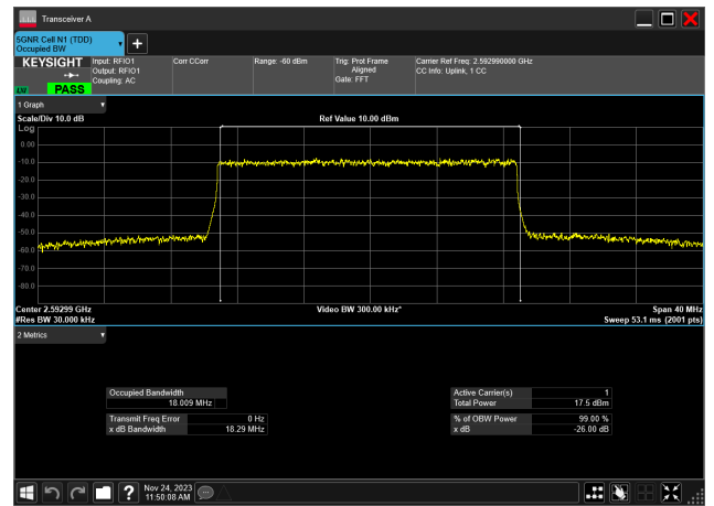
20MHz_30kHz_2592.99MHz_DFT-s-OFDM 256 QAM_RB50@0 18.009 MHz
