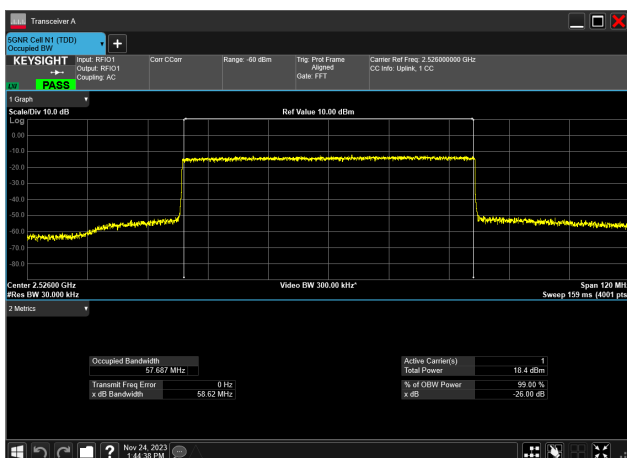
60MHz_30kHz_2526MHz_CP-OFDM 64 QAM_RB162@0 57.687 MHz
