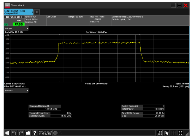
15MHz_30kHz_2682.48MHz_CP-OFDM 16 QAM_RB38@0 13.564 MHz
