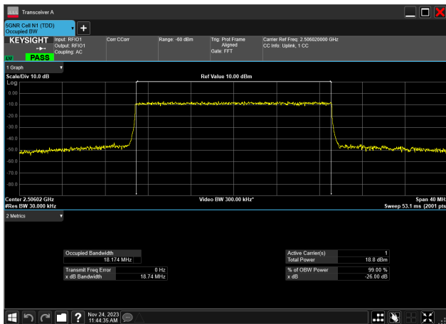
20MHz_30kHz_2506.02MHz_CP-OFDM 16 QAM_RB51@0 18.174 MHz
