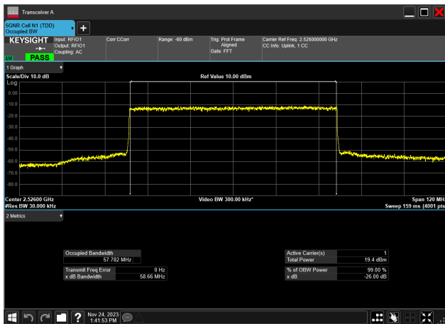
60MHz_30kHz_2526MHz_DFT-s-OFDM 64 QAM_RB162@0 57.782 MHz
