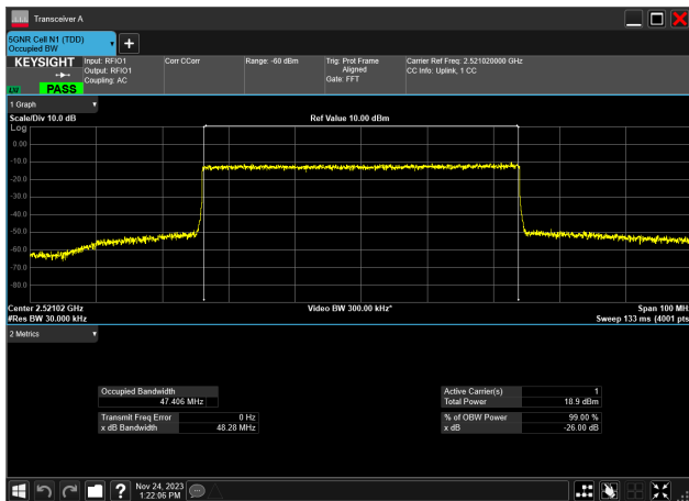
50MHz_30kHz_2521.02MHz_CP-OFDM 16 QAM_RB133@0 47.406 MHz
