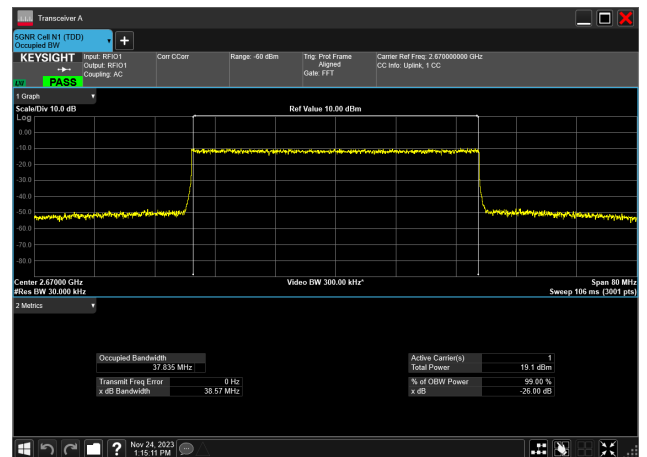
40MHz_30kHz_2670MHz_CP-OFDM 16 QAM_RB106@0 37.835 MHz
