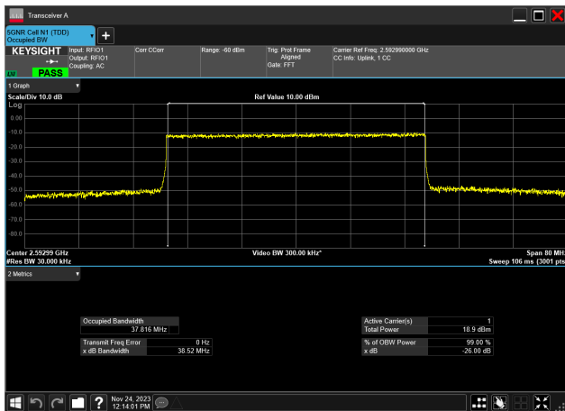
40MHz_30kHz_2592.99MHz_CP-OFDM 16 QAM_RB106@0 37.816 MHz
