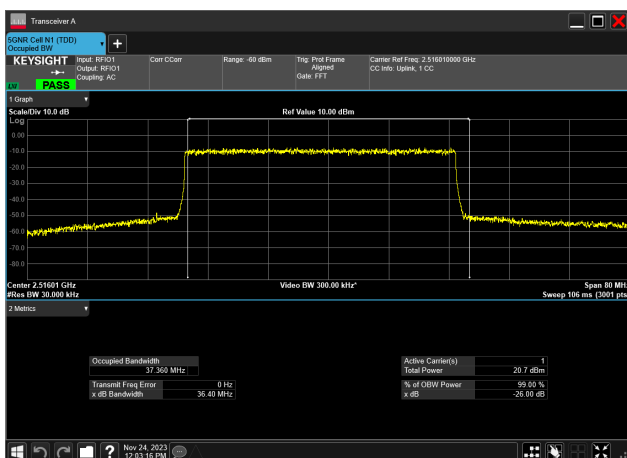
40MHz_30kHz_2516.01MHz_DFT-s-OFDM QPSK_RB100@0 37.360 MHz
