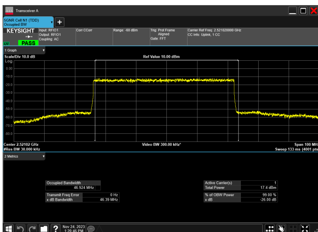
50MHz_30kHz_2521.02MHz_DFT-s-OFDM 256 QAM_RB128@0 46.924 MHz
