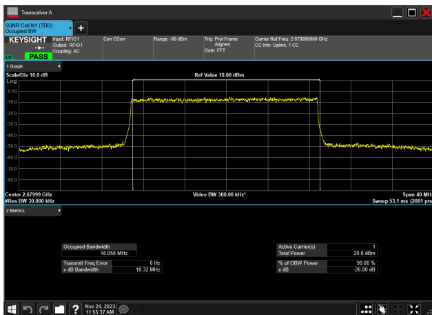
20MHz_30kHz_2679.99MHz_DFT-s-OFDM 16 QAM_RB50@0 18.050 MHz
