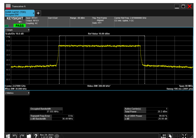
40MHz_30kHz_2670MHz_DFT-s-OFDM 16 QAM_RB100@0 37.555 MHz
