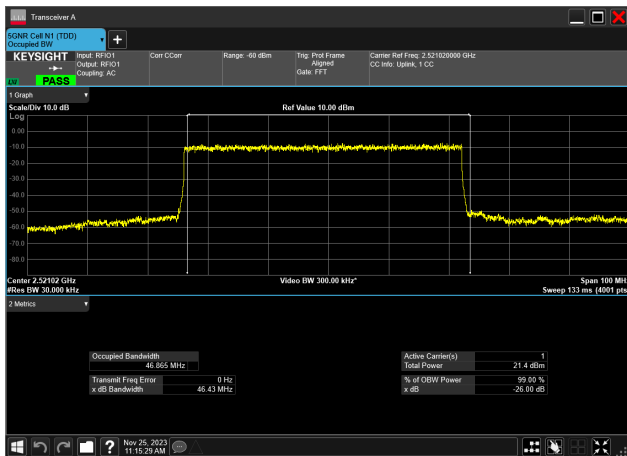
50MHz_30kHz_2521.02MHz_DFT-s-OFDM PI/2 BPSK_RB128@0 46.865 MHz
