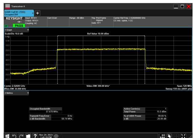
60MHz_30kHz_2526MHz_CP-OFDM 256 QAM_RB162@0 57.678 MHz
