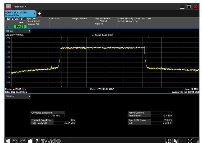
40MHz_30kHz_2516.01MHz_DFT-s-OFDM 16 QAM_RB100@0 37.351 MHz
