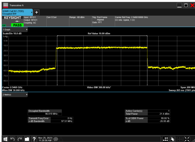
100MHz_30kHz_2546.01MHz_DFT-s-OFDM PI/2 BPSK_RB270@0 96.019 MHz
