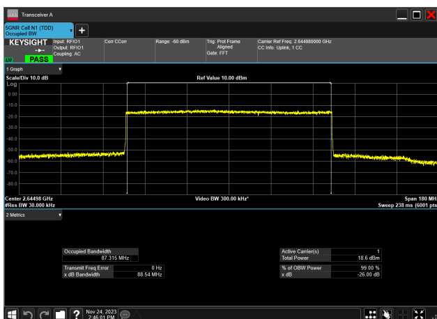
90MHz_30kHz_2644.98MHz_CP-OFDM 64 QAM_RB245@0 87.315 MHz
