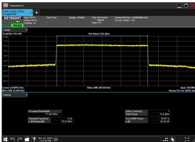
80MHz_30kHz_2649.99MHz_CP-OFDM 256 QAM_RB217@0 77.350 MHz
