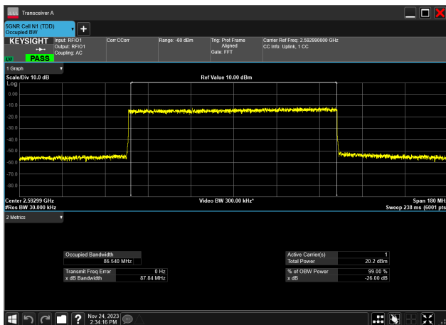
90MHz_30kHz_2592.99MHz_DFT-s-OFDM 16 QAM_RB243@0 86.540 MHz
