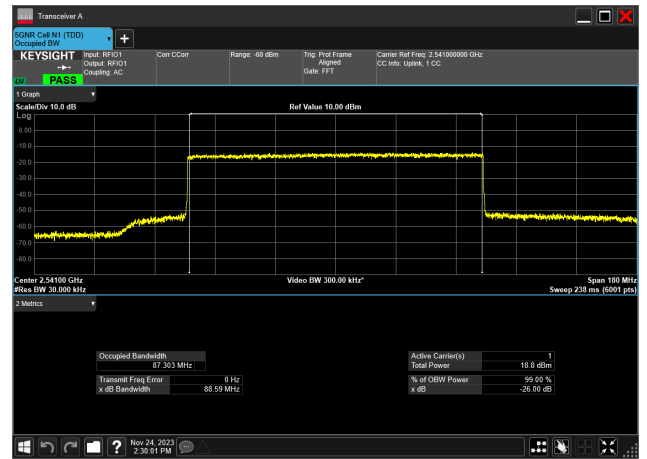
90MHz_30kHz_2541MHz_CP-OFDM 16 QAM_RB245@0 87.303 MHz
