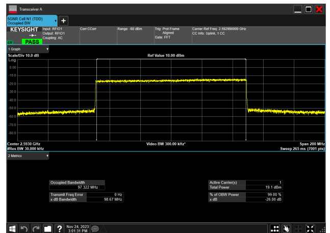
100MHz_30kHz_2592.99MHz_CP-OFDM 16 QAM_RB273@0 97.322 MHz
