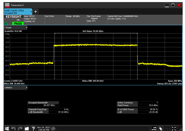
100MHz_30kHz_2640MHz_DFT-s-OFDM 64 QAM_RB270@0 96.007 MHz
