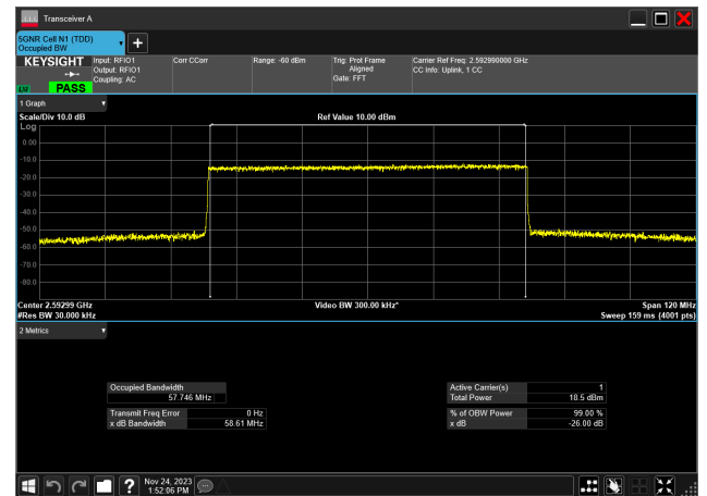
60MHz_30kHz_2592.99MHz_CP-OFDM 64 QAM_RB162@0 57.746 MHz
