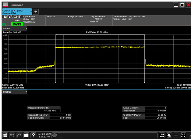
90MHz_30kHz_2541MHz_CP-OFDM QPSK_RB245@0 87.265 MHz
