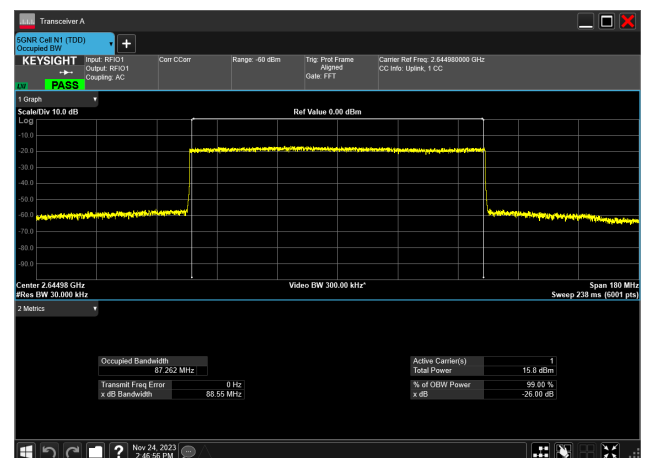
90MHz_30kHz_2644.98MHz_CP-OFDM 256 QAM_RB245@0 87.262 MHz
