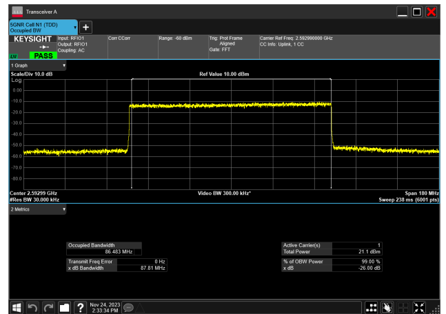
90MHz_30kHz_2592.99MHz_DFT-s-OFDM QPSK_RB243@0 86.483 MHz
