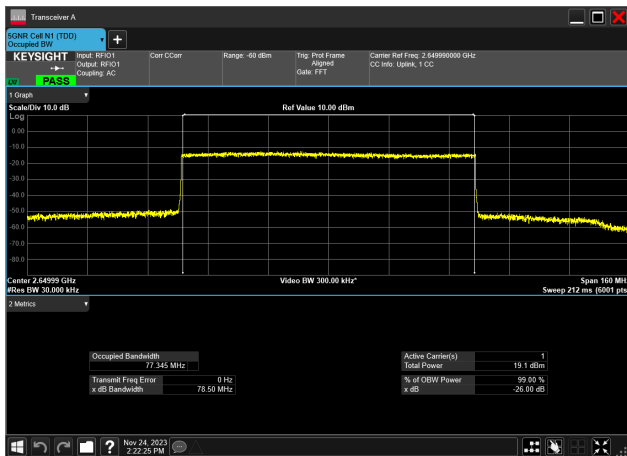
80MHz_30kHz_2649.99MHz_CP-OFDM 16 QAM_RB217@0 77.345 MHz
