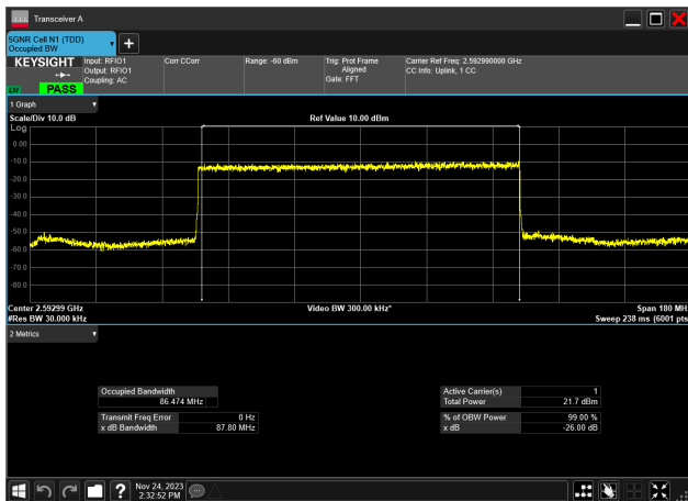
90MHz_30kHz_2592.99MHz_DFT-s-OFDM PI/2 BPSK_RB243@0 86.474 MHz
