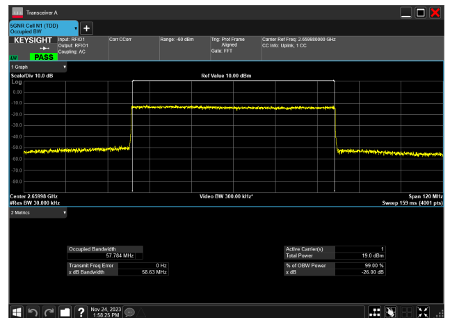
60MHz_30kHz_2659.98MHz_CP-OFDM 16 QAM_RB162@0 57.784 MHz
