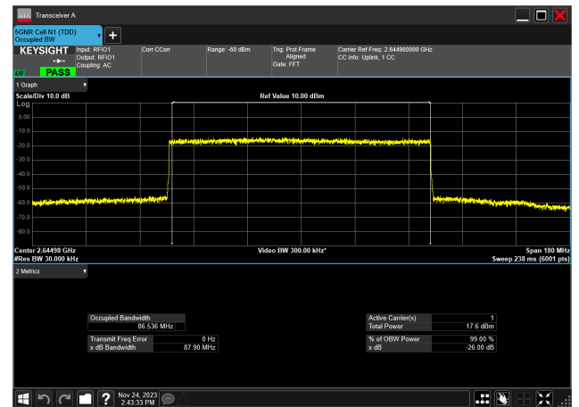
90MHz_30kHz_2644.98MHz_DFT-s-OFDM 256 QAM_RB243@0 86.536 MHz
