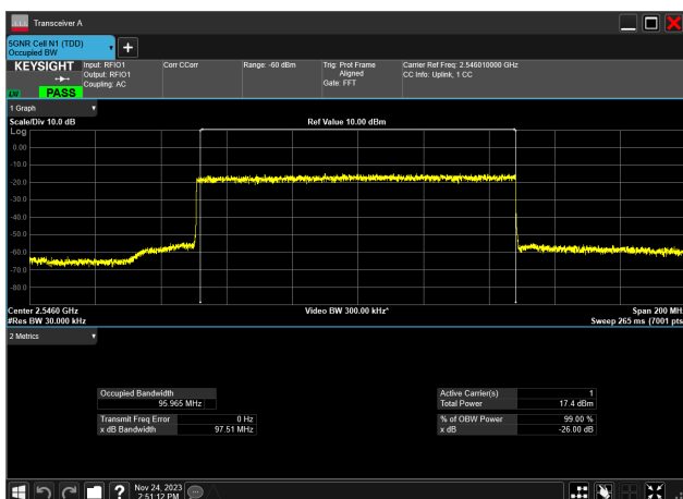
100MHz_30kHz_2546.01MHz_DFT-s-OFDM 256 QAM_RB270@0 95.965 MHz
