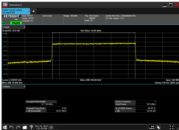
60MHz_30kHz_2592.99MHz_CP-OFDM 16 QAM_RB162@0 57.734 MHz
