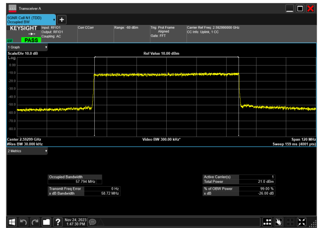
60MHz_30kHz_2592.99MHz_DFT-s-OFDM QPSK_RB162@0 57.794 MHz
