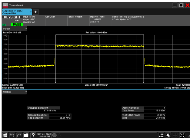
60MHz_30kHz_2659.98MHz_DFT-s-OFDM 64 QAM_RB162@0 57.841 MHz
