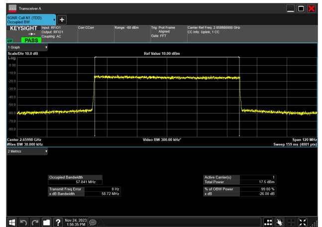
60MHz_30kHz_2659.98MHz_DFT-s-OFDM 256 QAM_RB162@0 57.841 MHz
