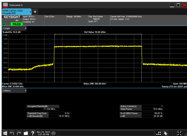
80MHz_30kHz_2536.02MHz_CP-OFDM 16 QAM_RB217@0 77.334 MHz
