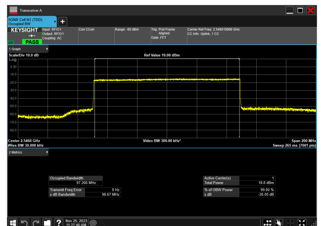
100MHz_30kHz_2546.01MHz_CP-OFDM QPSK_RB273@0 97.266 MHz
