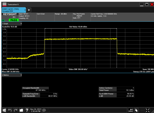
90MHz_30kHz_2541MHz_CP-OFDM 64 QAM_RB245@0 87.309 MHz
