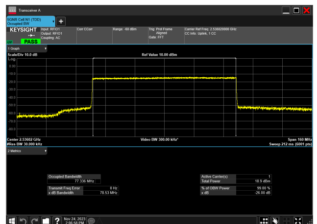
80MHz_30kHz_2536.02MHz_CP-OFDM QPSK_RB217@0 77.336 MHz
