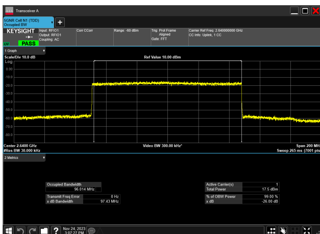
100MHz_30kHz_2640MHz_DFT-s-OFDM 256 QAM_RB270@0 96.014 MHz
