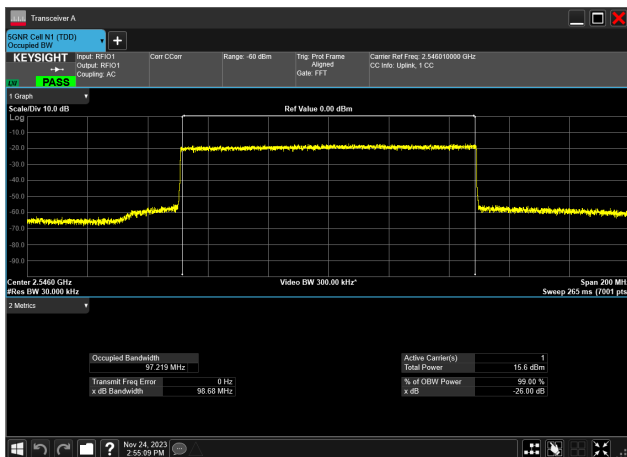
100MHz_30kHz_2546.01MHz_CP-OFDM 256 QAM_RB273@0 97.219 MHz
