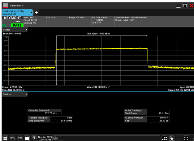
100MHz_30kHz_2592.99MHz_CP-OFDM QPSK_RB273@0 97.278 MHz
