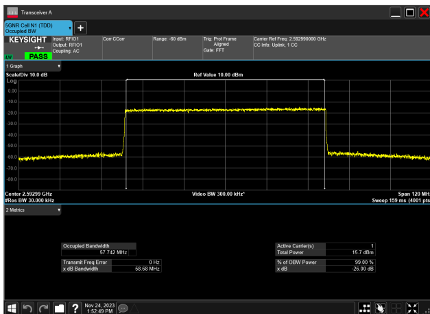
60MHz_30kHz_2592.99MHz_CP-OFDM 256 QAM_RB162@0 57.742 MHz
