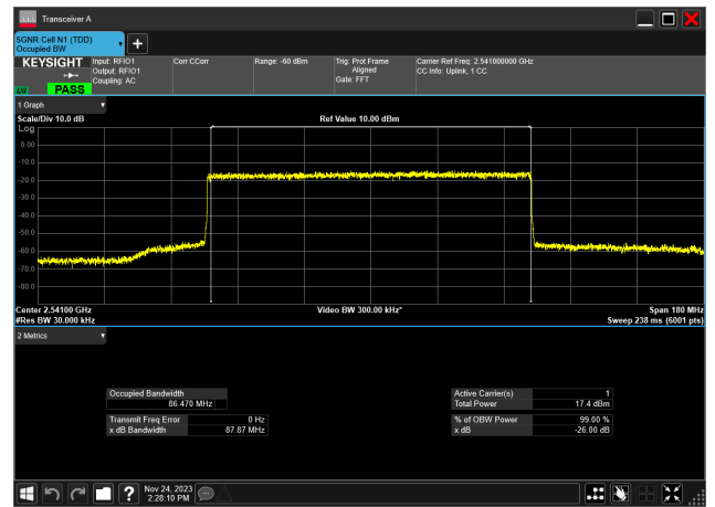
90MHz_30kHz_2541MHz_DFT-s-OFDM 256 QAM_RB243@0 86.470 MHz
