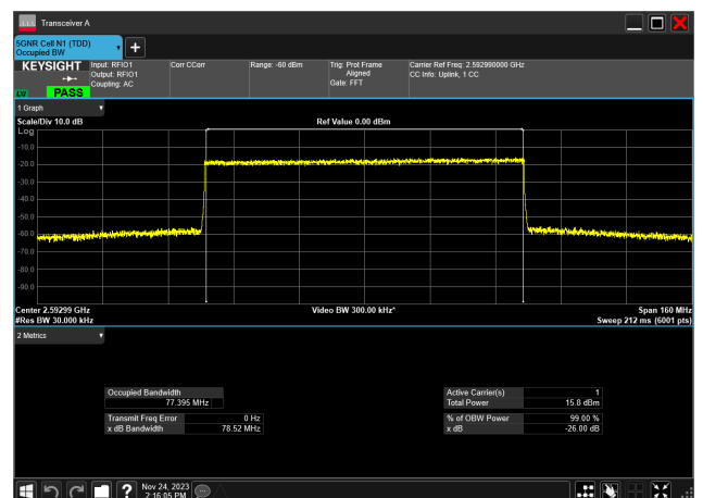
80MHz_30kHz_2592.99MHz_CP-OFDM 256 QAM_RB217@0 77.395 MHz
