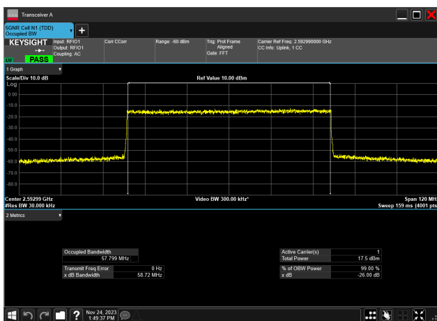
60MHz_30kHz_2592.99MHz_DFT-s-OFDM 256 QAM_RB162@0 57.799 MHz
