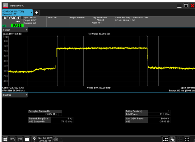
80MHz_30kHz_2536.02MHz_DFT-s-OFDM 16 QAM_RB216@0 76.877 MHz
