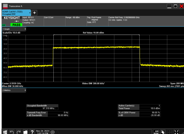
100MHz_30kHz_2592.99MHz_CP-OFDM 64 QAM_RB273@0 97.319 MHz
