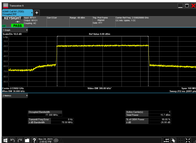
80MHz_30kHz_2536.02MHz_CP-OFDM 256 QAM_RB217@0 77.300 MHz
