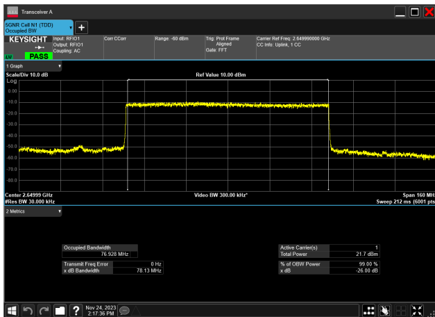
80MHz_30kHz_2649.99MHz_DFT-s-OFDM PI/2 BPSK_RB216@0 76.928 MHz
