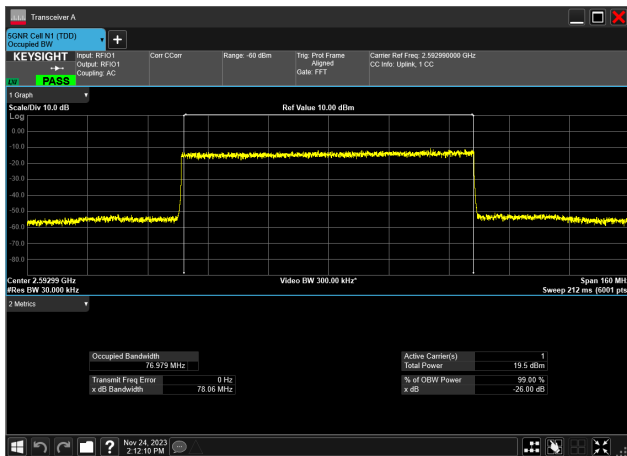
80MHz_30kHz_2592.99MHz_DFT-s-OFDM 64 QAM_RB216@0 76.979 MHz
