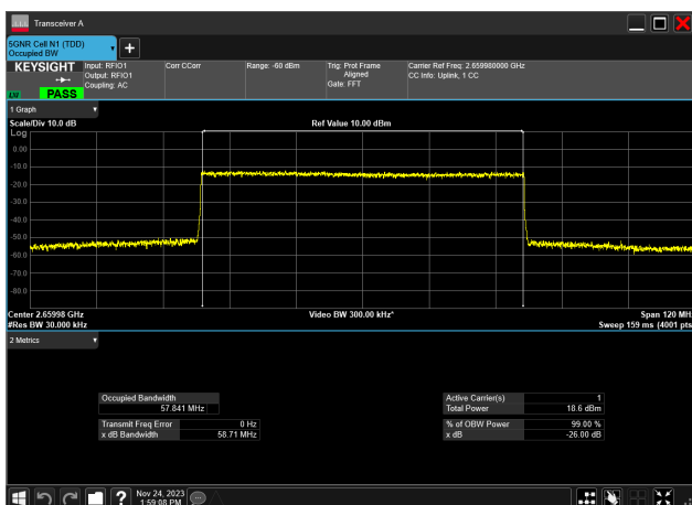
60MHz_30kHz_2659.98MHz_CP-OFDM 64 QAM_RB162@0 57.841 MHz
