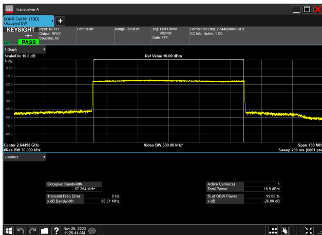
90MHz_30kHz_2644.98MHz_CP-OFDM QPSK_RB245@0 87.264 MHz
