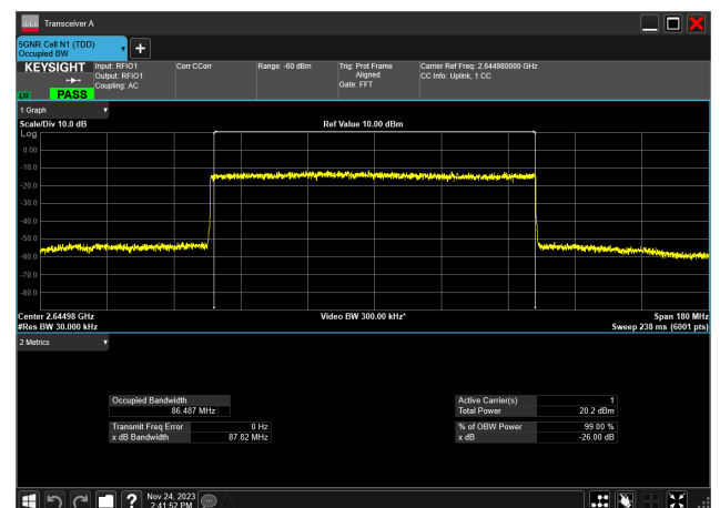
90MHz_30kHz_2644.98MHz_DFT-s-OFDM 16 QAM_RB243@0 86.487 MHz
