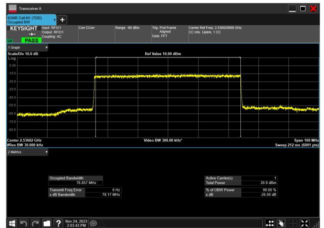
80MHz_30kHz_2536.02MHz_DFT-s-OFDM QPSK_RB216@0 76.857 MHz
