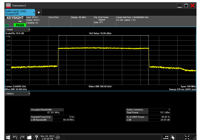
90MHz_30kHz_2644.98MHz_CP-OFDM 16 QAM_RB245@0 87.301 MHz
