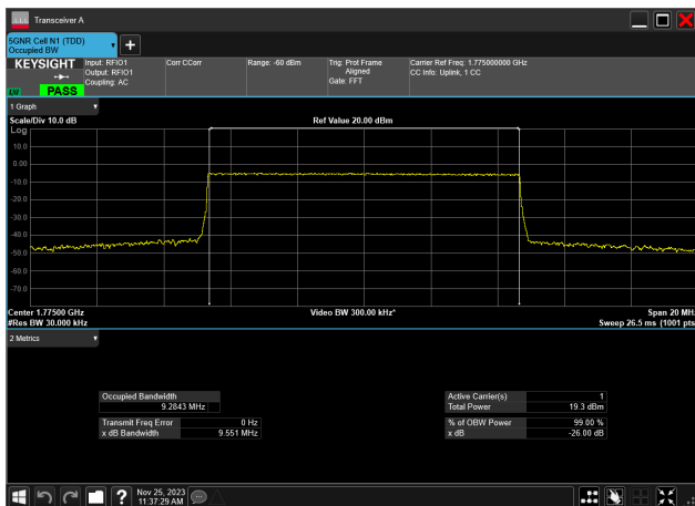
10MHz_15kHz_1775MHz_CP-OFDM QPSK_RB52@0 9.284 MHz
