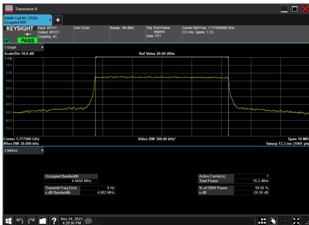
5MHz_15kHz_1777.5MHz_CP-OFDM 256 QAM_RB25@0 4.465 MHz
