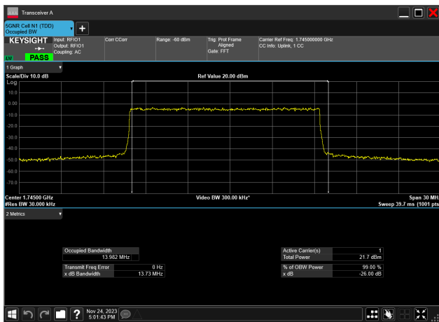
15MHz_15kHz_1745MHz_DFT-s-OFDM_QPSK_RB75@0 13.982 MHz
