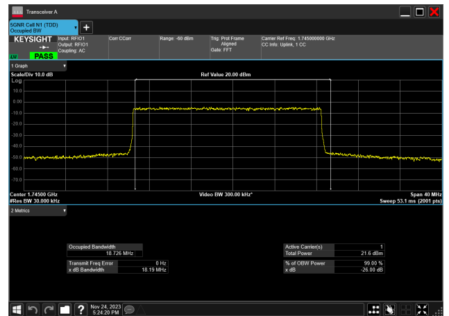
20MHz_15kHz_1745MHz_DFT-s-OFDM QPSK_RB100@0 18.726 MHz
