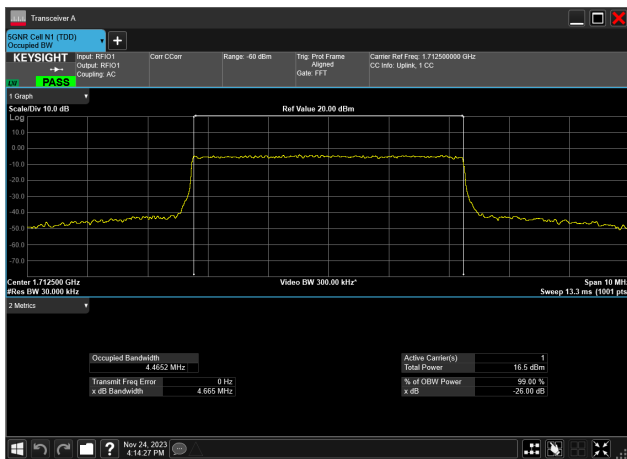
5MHz_15kHz_1712.5MHz_CP-OFDM 256 QAM_RB25@0 4.465 MHz
