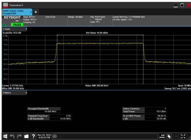
15MHz_15kHz_1717.5MHz_CP-OFDM_16_QAM_RB79@0 14.069 MHz
