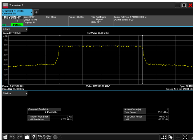
5MHz_15kHz_1712.5MHz_CP-OFDM 16 QAM_RB25@0 4.464 MHz
