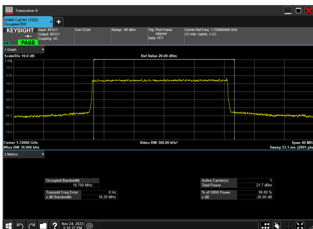
20MHz_15kHz_1720MHz_DFT-s-OFDM QPSK_RB100@0 18.700 MHz
