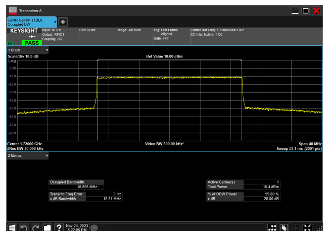
20MHz_15kHz_1720MHz_CP-OFDM 256 QAM_RB106@0 18.895 MHz
