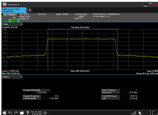
10MHz_15kHz_1745MHz_DFT-s-OFDM 16 QAM_RB50@0 9.209 MHz
