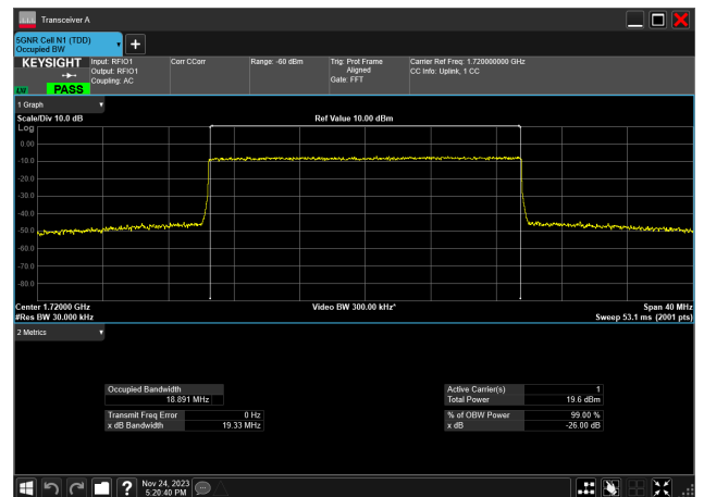
20MHz_15kHz_1720MHz_CP-OFDM 16 QAM_RB106@0 18.891 MHz
