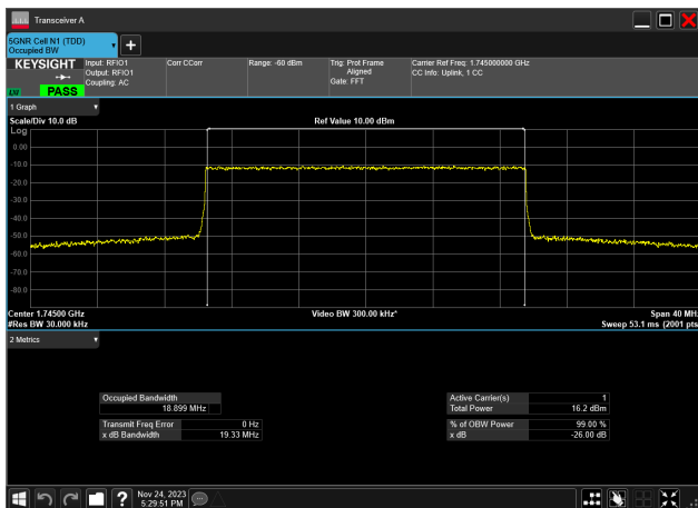
20MHz_15kHz_1745MHz_CP-OFDM 256 QAM_RB106@0 18.899 MHz
