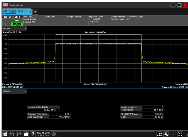
20MHz_15kHz_1745MHz_CP-OFDM 16 QAM_RB106@0 18.893 MHz
