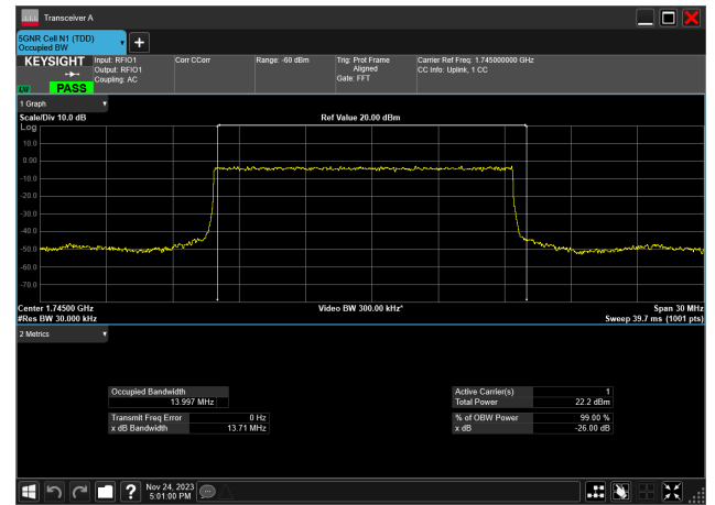
15MHz_15kHz_1745MHz_DFT-s-OFDM_PI/2_BPSK_RB75@0 13.997 MHz
