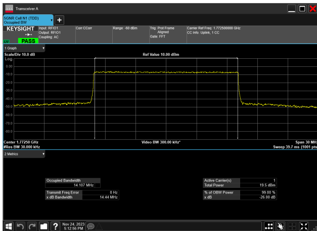
15MHz_15kHz_1772.5MHz_CP-OFDM 16 QAM_RB79@0 14.107 MHz
