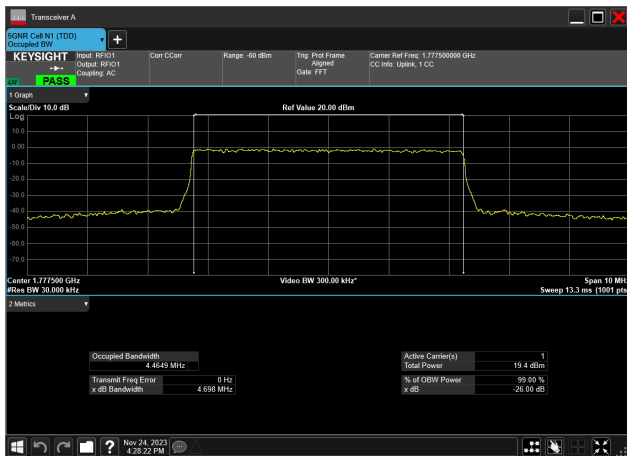
5MHz_15kHz_1777.5MHz_CP-OFDM 16 QAM_RB25@0 4.465 MHz
