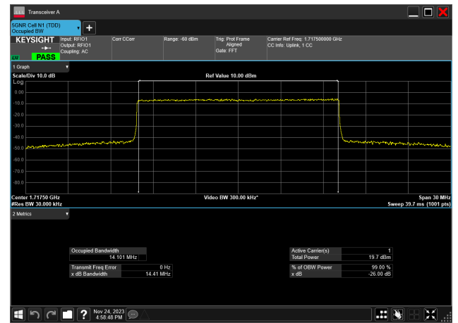
15MHz_15kHz_1717.5MHz_CP-OFDM_64_QAM_RB79@0 14.101 MHz
