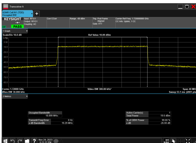
20MHz_15kHz_1720MHz_CP-OFDM 64 QAM_RB106@0 18.899 MHz
