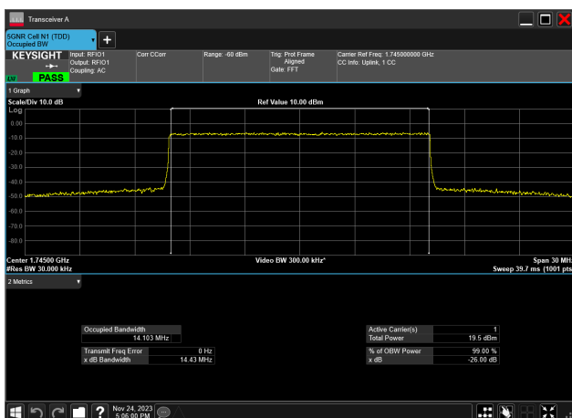
15MHz_15kHz_1745MHz_CP-OFDM 64 QAM_RB79@0 14.103 MHz
