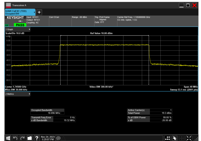
20MHz_15kHz_1745MHz_CP-OFDM 64 QAM_RB106@0 18.896 MHz
