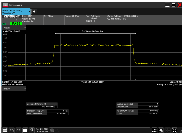
10MHz_15kHz_1715MHz_DFT-s-OFDM 64 QAM_RB50@0 9.217 MHz
