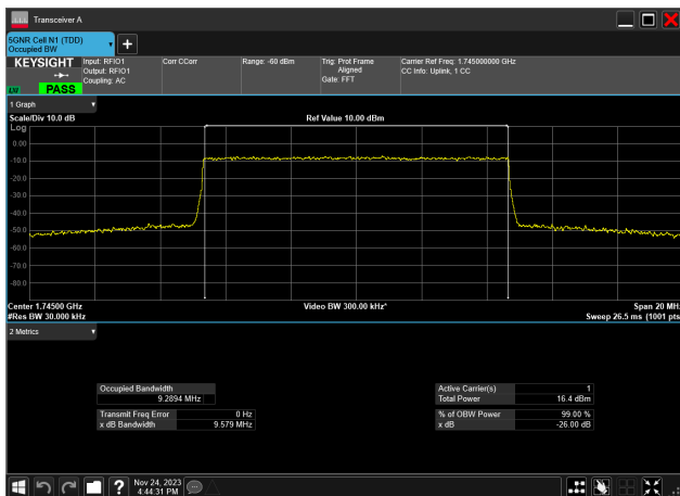
10MHz_15kHz_1745MHz_CP-OFDM 256 QAM_RB52@0 9.289 MHz
