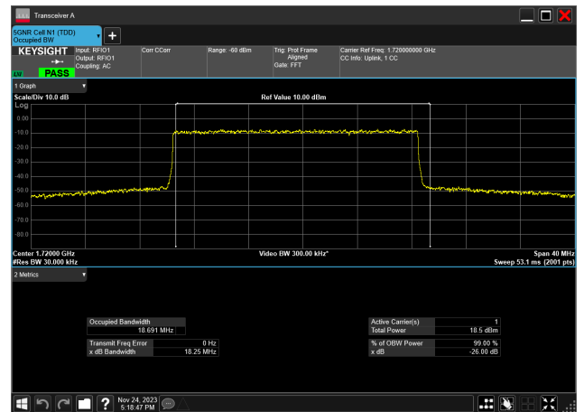
20MHz_15kHz_1720MHz_DFT-s-OFDM 256 QAM_RB100@0 18.691 MHz
