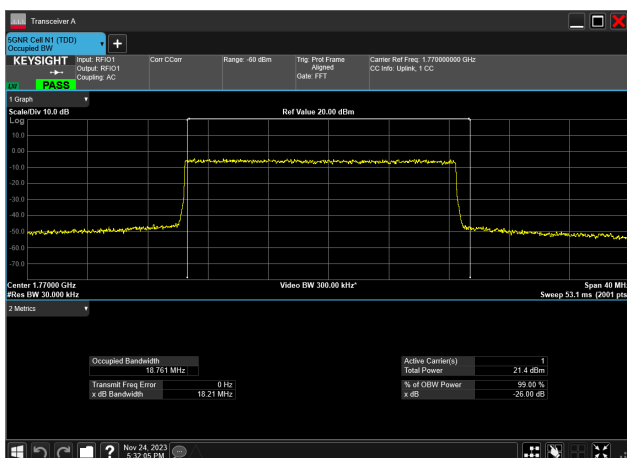
20MHz_15kHz_1770MHz_DFT-s-OFDM QPSK_RB100@0 18.761 MHz
