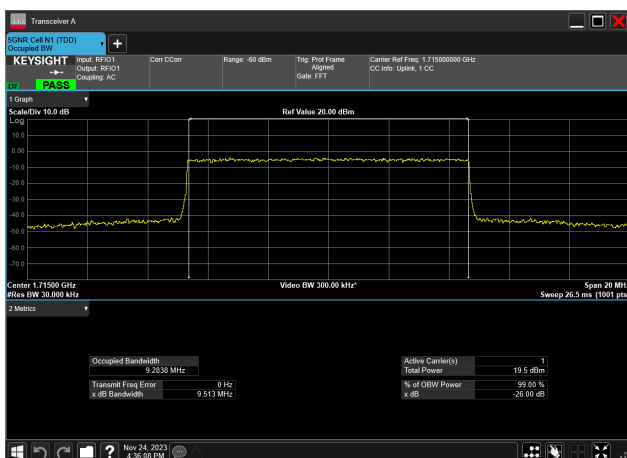
10MHz_15kHz_1715MHz_CP-OFDM 64 QAM_RB52@0 9.284 MHz
