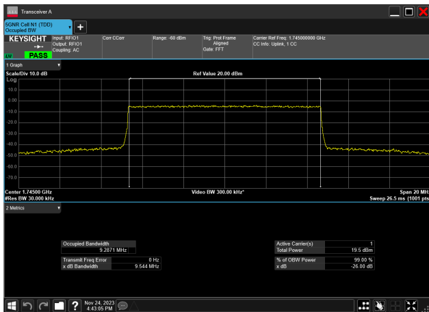
10MHz_15kHz_1745MHz_CP-OFDM 16 QAM_RB52@0 9.287 MHz
