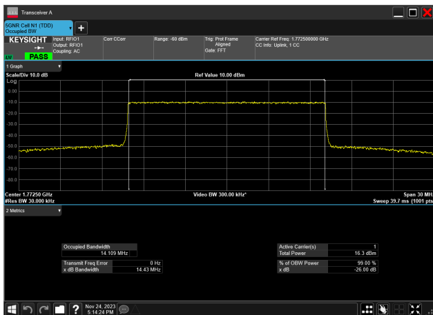
15MHz_15kHz_1772.5MHz_CP-OFDM 256 QAM_RB79@0 14.109 MHz
