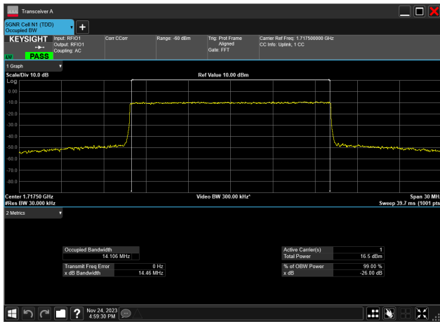
15MHz_15kHz_1717.5MHz_CP-OFDM_256_QAM_RB79@0 14.106 MHz
