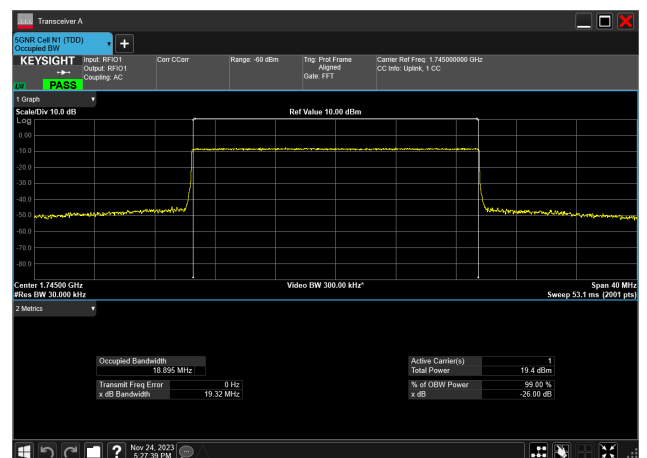
20MHz_15kHz_1745MHz_CP-OFDM QPSK_RB106@0 18.895 MHz
