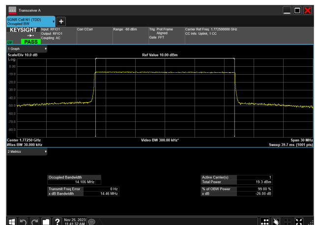
15MHz_15kHz_1772.5MHz_CP-OFDM QPSK_RB79@0 14.106 MHz
