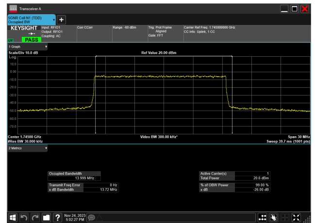
15MHz_15kHz_1745MHz_DFT-s-OFDM_16_QAM_RB75@0 13.999 MHz
