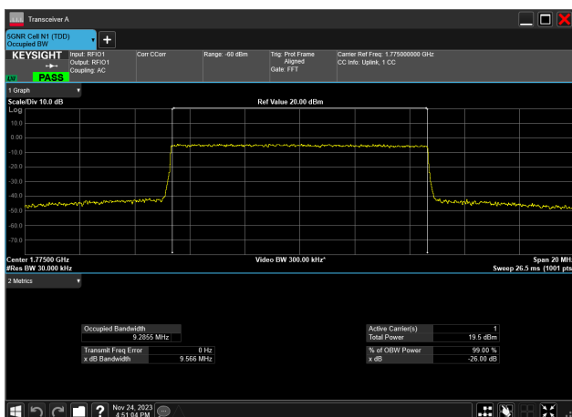
10MHz_15kHz_1775MHz_CP-OFDM 64 QAM_RB52@0 9.285 MHz
