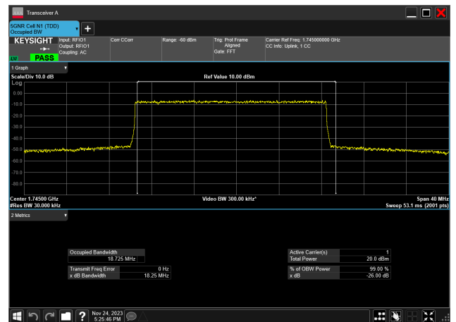
20MHz_15kHz_1745MHz_DFT-s-OFDM 64 QAM_RB100@0 18.725 MHz
