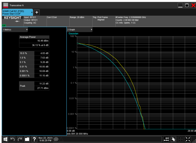
20MHz_15kHz_2535MHz_DFT-s-OFDM 64 QAM_RB100@0 9.20 dB
