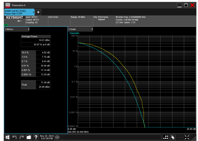
20MHz_15kHz_2535MHz_DFT-s-OFDM 256 QAM_RB100@0 9.43 dB
