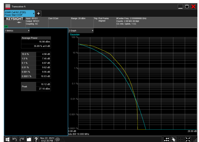
10MHz_15kHz_2535MHz_DFT-s-OFDM 16 QAM_RB50@0 8.87 dB
