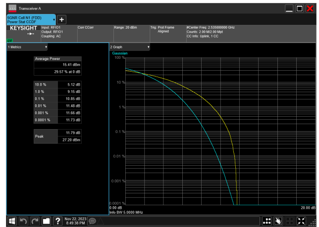
5MHz_15kHz_2535MHz_CP-OFDM 64 QAM_RB25@0 10.85 dB
