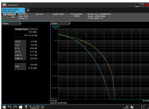
20MHz_15kHz_2535MHz_CP-OFDM 64 QAM_RB106@0 10.80 dB
