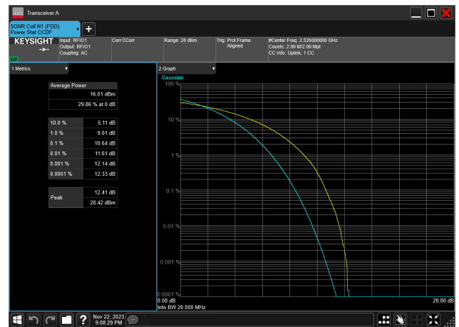
20MHz_15kHz_2535MHz_CP-OFDM 16 QAM_RB106@0 10.64 dB
