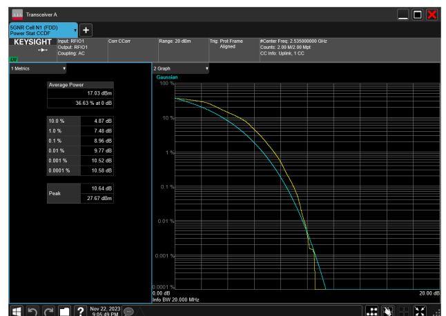
20MHz_15kHz_2535MHz_DFT-s-OFDM 16 QAM_RB100@0 8.96 dB
