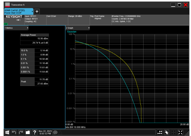
10MHz_15kHz_2535MHz_CP-OFDM 16 QAM_RB52@0 10.50 dB
