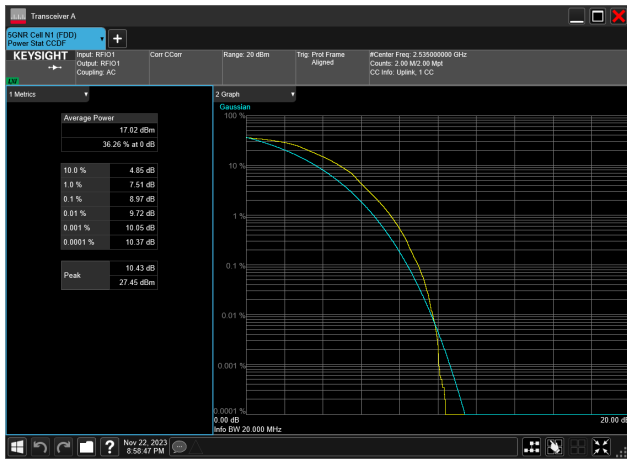
15MHz_15kHz_2535MHz_DFT-s-OFDM 16 QAM_RB75@0 8.97 dB
