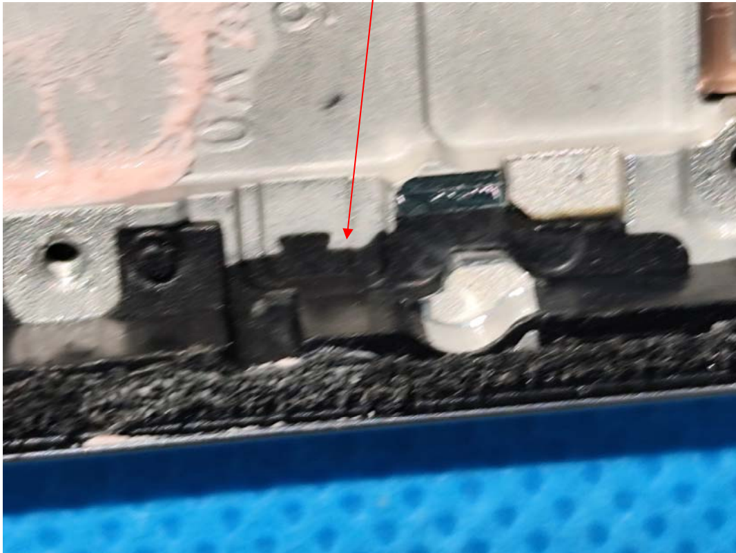
LTE B1/3 DL CA Antenna
