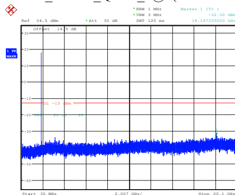
15MHz Middle QPSK_1@0(30MHz~20.1GHz)
