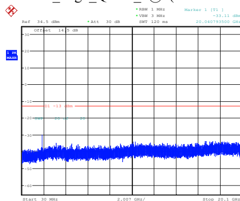
20MHz High QPSK 1@0(30MHz~20.1GHz)
