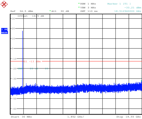
3MHz_Middle_QPSK_1@0(30MHz~18.55GHz)
