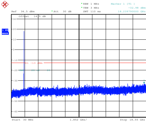
3MHz_High_QPSK_1@0(30MHz~18.55GHz)
