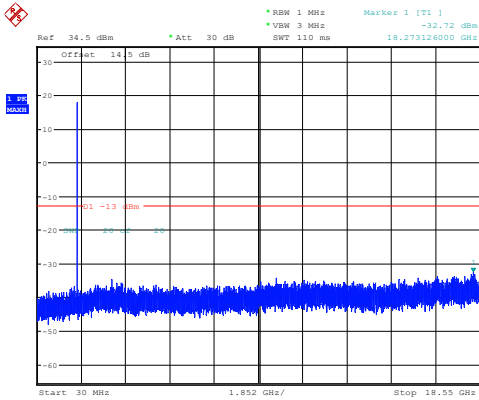
3MHz_Low_QPSK_1@0(30MHz~18.55GHz)
