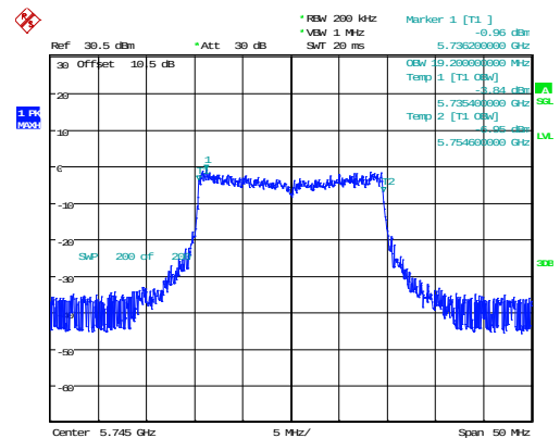
802.11ax20_5745MHz_RU_Full_Chain 1 19.200MHz
