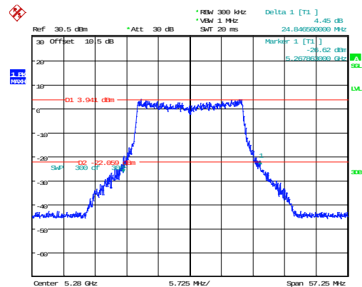
802.11ax20_5280MHz_RU_Full_Chain 0 24.847MHz
