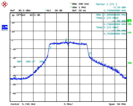
802.11a_5745MHz_Chain 1 17.300MHz
