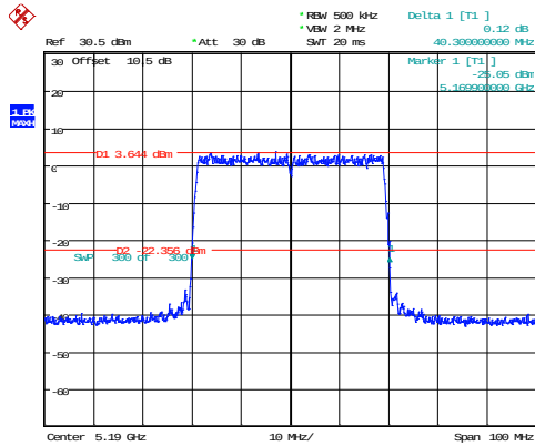
802.11ax40_5190MHz_RU_Full_Chain 1 40.300MHz
