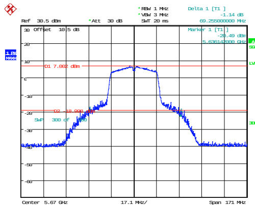
802.11n40_5670MHz_Chain 0 69.255MHz
