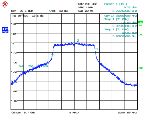
802.11a_5700MHz_Chain 1 17.350MHz
