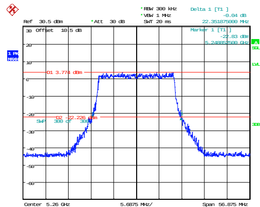
802.11ax20_5260MHz_RU_Full_Chain 1 22.352MHz
