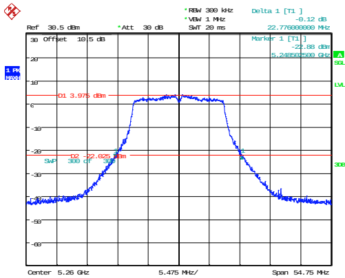
802.11a_5260MHz_Chain 1 22.776MHz
