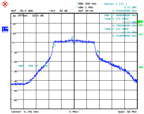
802.11a_5745MHz_Chain 0 17.400MHz
