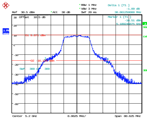
802.11a_5200MHz_Chain 1 38.861MHz
