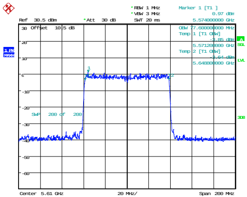
802.11ax80_5610MHz_RU_Full_Chain 1 77.600MHz
