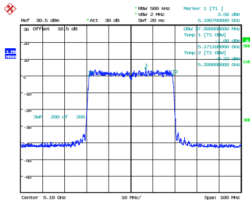
802.11ax40_5190MHz_RU_Full_Chain 1 37.900MHz
