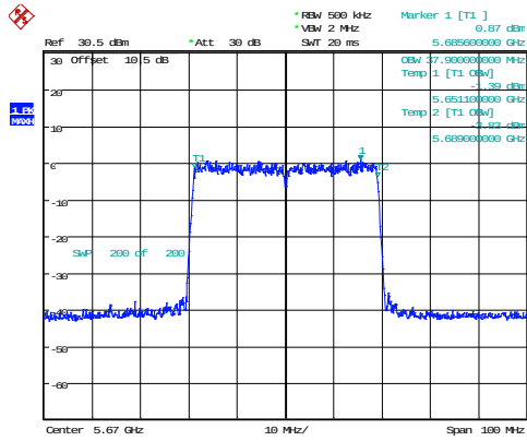
802.11ax40_5670MHz_RU_Full_Chain 1 37.900MHz
