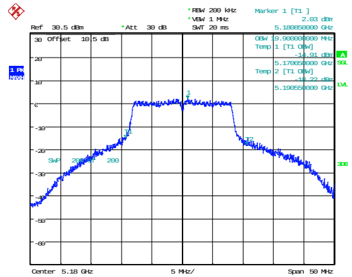
802.11a_5180MHz_Chain 1 19.900MHz
