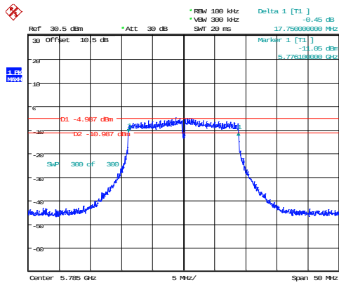
802.11n20_5785MHz_Chain 1 17.750MHz
