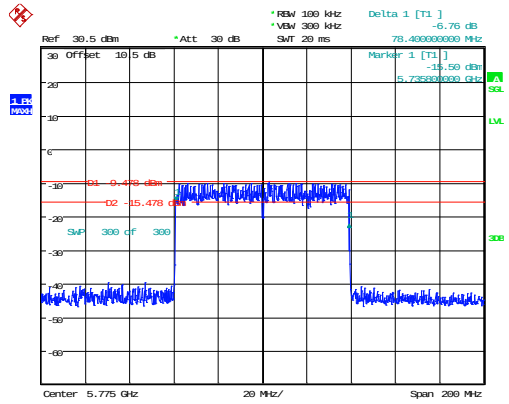
802.11ax80_5775MHz_RU_Full_Chain 1 78.400MHz
