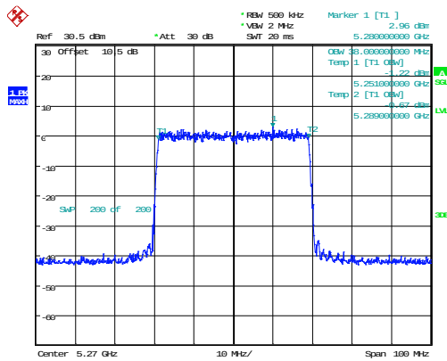
802.11ax40_5270MHz_RU_Full_Chain 0 38MHz
