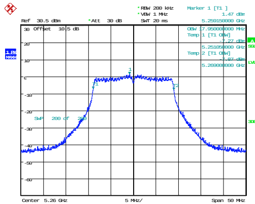
802.11n20_5260MHz_Chain 0 17.950MHz
