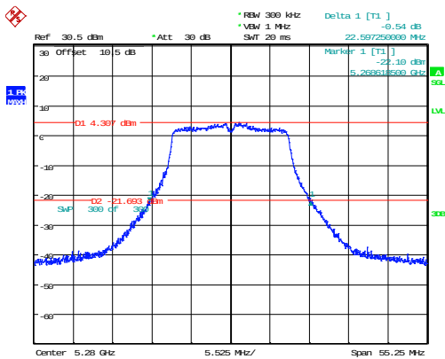
802.11a_5280MHz_Chain 1 22.597MHz
