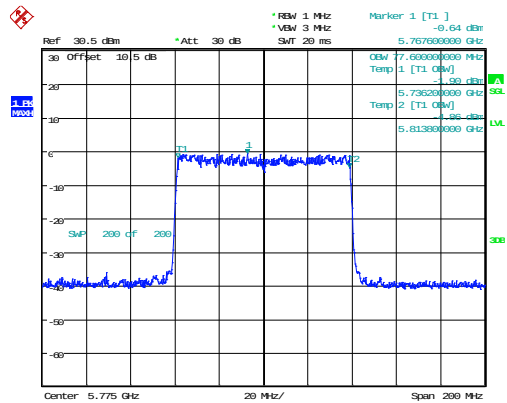
802.11ax80_5775MHz_RU_Full_Chain 1 77.600MHz
