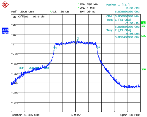
802.11a_5825MHz_Chain 0 16.850MHz
