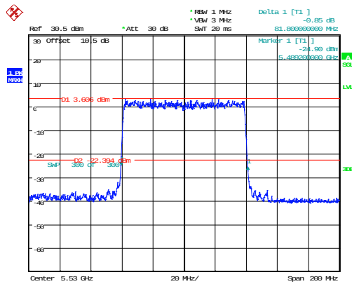
802.11ax80_5530MHz_RU_Full_Chain 0 81.800MHz
