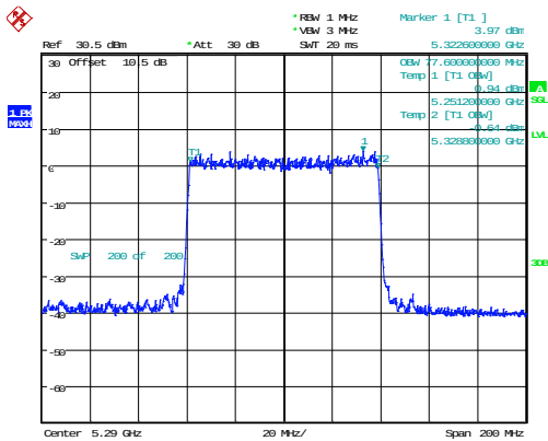
802.11ax80_5290MHz_RU_Full_Chain 1 77.600MHz
