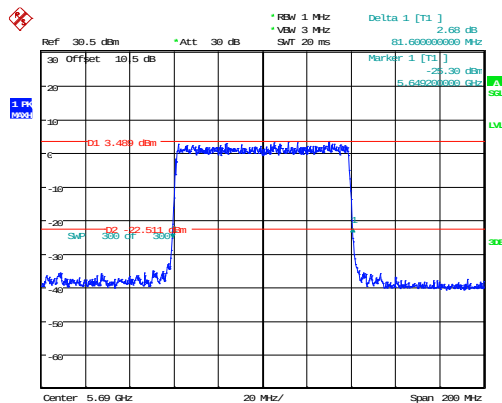
802.11ax80_5690MHz_RU_Full_Chain 0 81.600MHz
