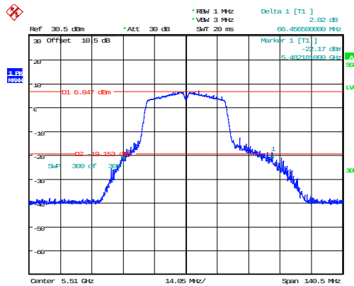
802.11n40_5510MHz_Chain 0 66.457MHz
