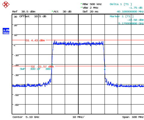
802.11ax40_5190MHz_RU_Full_Chain 0 40.100MHz
