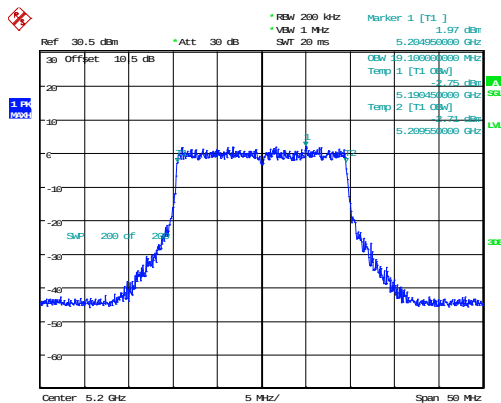
802.11ax20_5200MHz_RU_Full_Chain 1 19.100MHz
