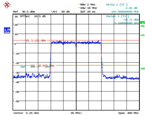
802.11ax160_5250MHz_RU_Full_Chain 1 164.400MHz
