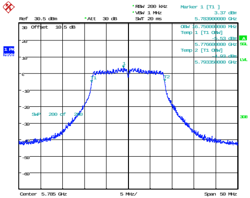
802.11a_5785MHz_Chain 0 16.750MHz
