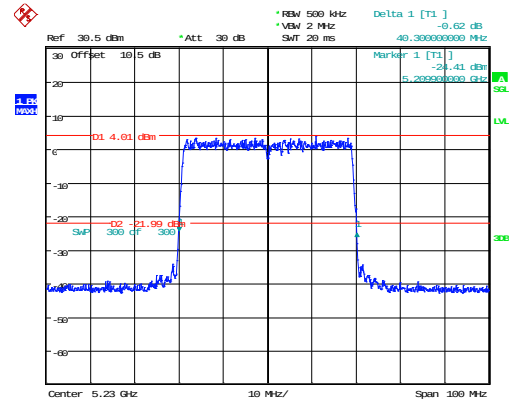
802.11ax40_5230MHz_RU_Full_Chain 1 40.300MHz
