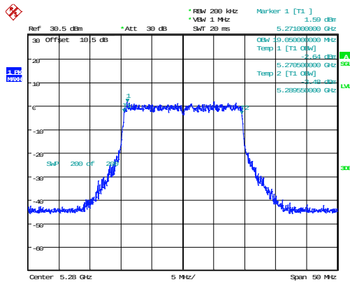
802.11ax20_5280MHz_RU_Full_Chain 1 19.050MHz
