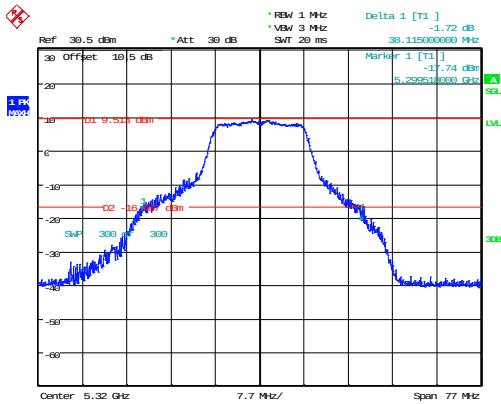
802.11a_5320MHz_Chain 0 38.115MHz
