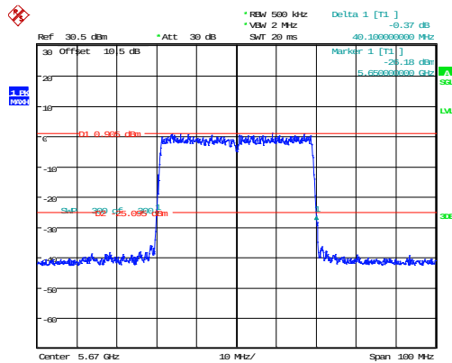
802.11ax40_5670MHz_RU_Full_Chain 1 40.100MHz
