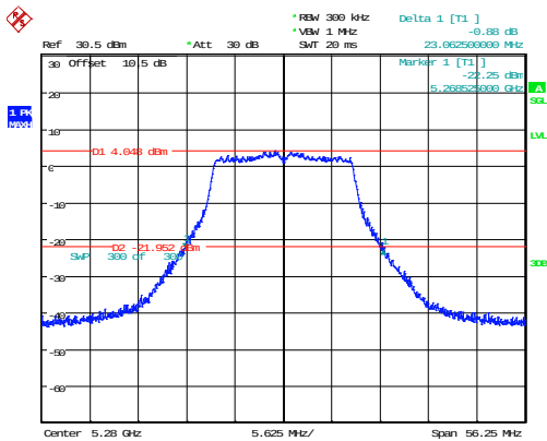
802.11a_5280MHz_Chain 0 23.063MHz
