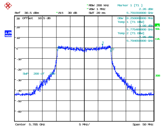
802.11ax20_5785MHz_RU_Full_Chain 0 19.250MHz
