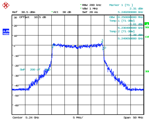
802.11ax20_5240MHz_RU_Full_Chain 0 19.250MHz
