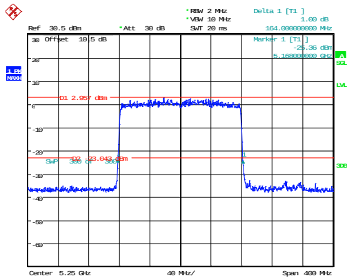
802.11ax160_5250MHz_RU_Full_Chain 0 164MHz
