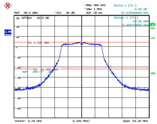
802.11a_5240MHz_Chain 1 22.677MHz
