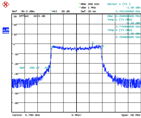
802.11ax20_5785MHz_RU_Full_Chain 1 19.200MHz
