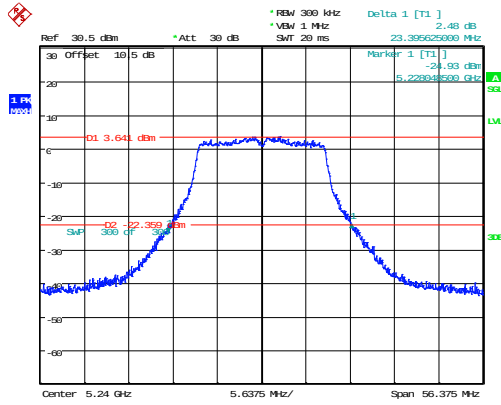
802.11a_5240MHz_Chain 0 23.396MHz
