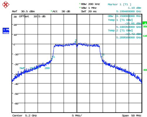
802.11n20_5200MHz_Chain 1 19.150MHz
