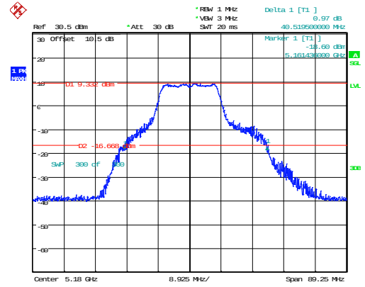
802.11a_5180MHz_Chain 1 40.520MHz
