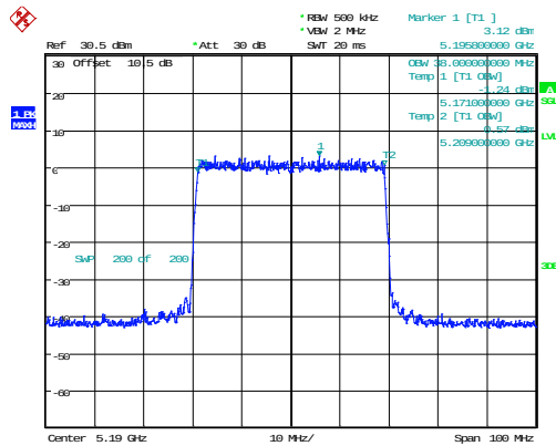
802.11ax40_5190MHz_RU_Full_Chain 0 38MHz
