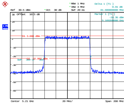
802.11ax80_5210MHz_RU_Full_Chain 0 81.600MHz
