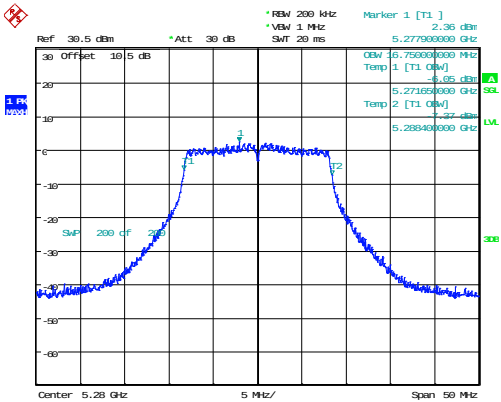
802.11a_5280MHz_Chain 0 16.750MHz
