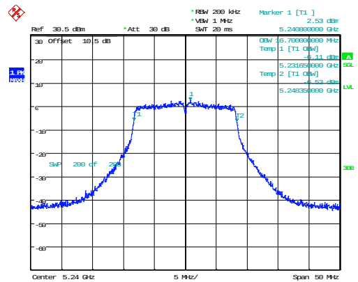
802.11a_5240MHz_Chain 1 16.700MHz
