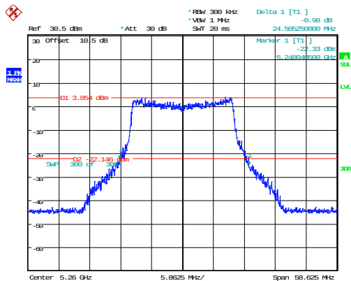
802.11ax20_5260MHz_RU_Full_Chain 0 24.505MHz
