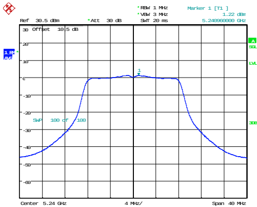
802.11a_5240MHz_Chain 1
