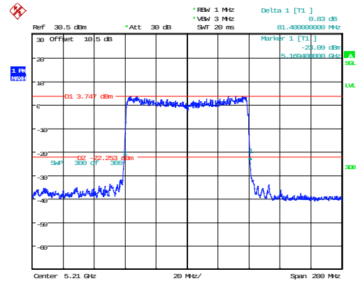
802.11ax80_5210MHz_RU_Full_Chain 1 81.400MHz
