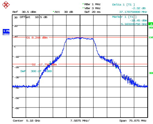
802.11a_5180MHz_Chain 0 37.179MHz
