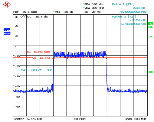
802.11ax80_5775MHz_RU_Full_Chain 0 78.400MHz
