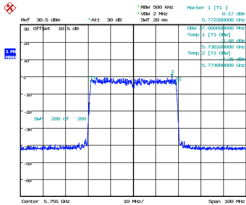
802.11ax40_5755MHz_RU_Full_Chain 1 37.900MHz
