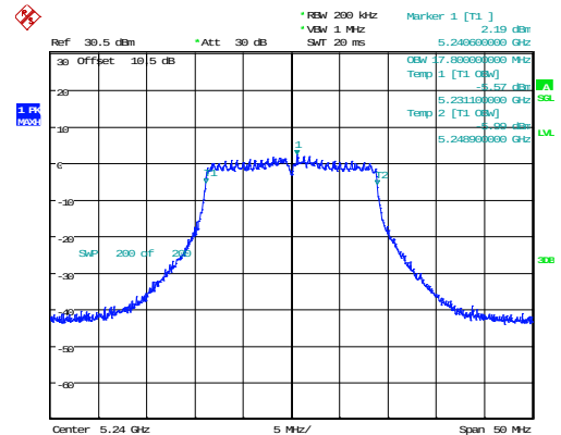
802.11n20_5240MHz_Chain 1 17.800MHz
