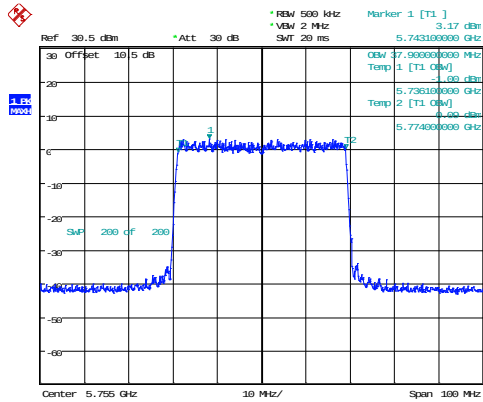
802.11ax40_5755MHz_RU_Full_Chain 0 37.900MHz
