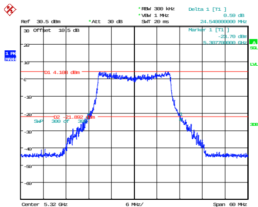
802.11ax20_5320MHz_RU_Full_Chain 0 24.540MHz
