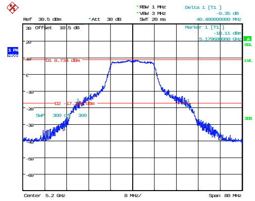
802.11a_5200MHz_Chain 0 40.480MHz
