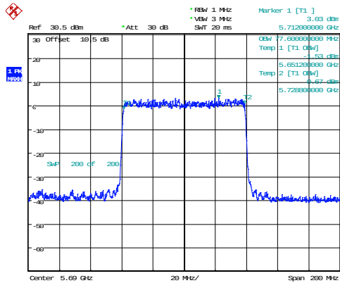
802.11ax80_5690MHz_RU_Full_Chain 0 77.600MHz
