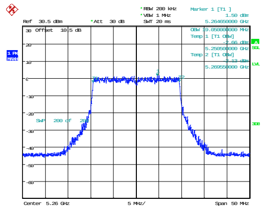
802.11ax20_5260MHz_RU_Full_Chain 1 19.050MHz
