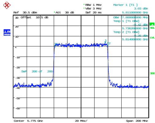
802.11ax80_5775MHz_RU_Full_Chain 0 77.800MHz
