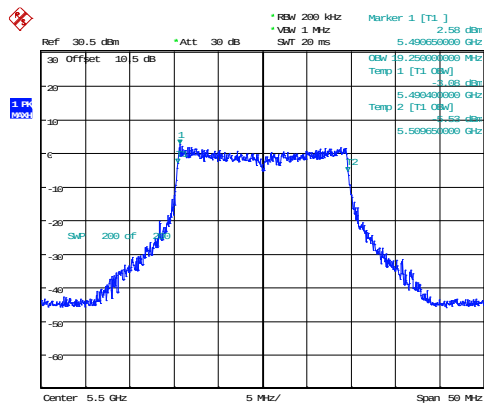
802.11ax20_5500MHz_RU_Full_Chain 0 19.250MHz
