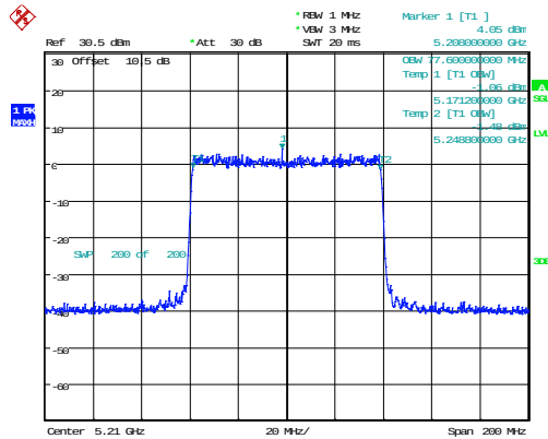
802.11ax80_5210MHz_RU_Full_Chain 0 77.600MHz
