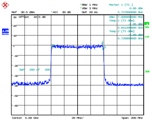
802.11ax80_5690MHz_RU_Full_Chain 1 77.600MHz
