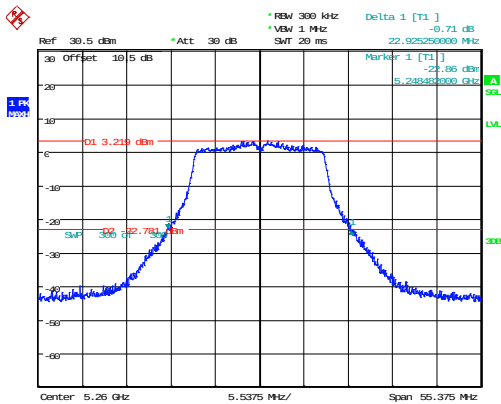
802.11a_5260MHz_Chain 0 22.925MHz
