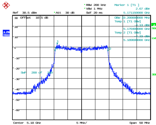
802.11ax20_5180MHz_RU_Full_Chain 0 19.200MHz
