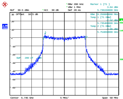
802.11ax20_5745MHz_RU_Full_Chain 0 19.250MHz
