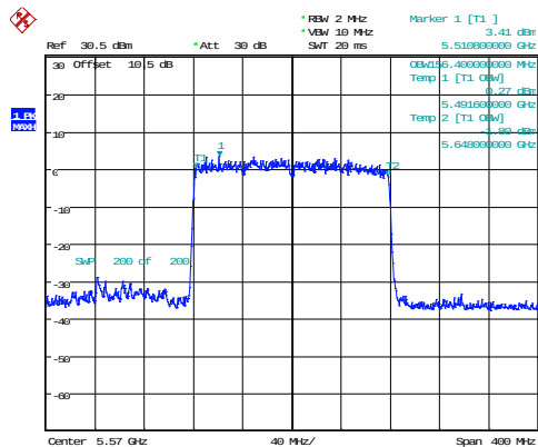
802.11ax160_5570MHz_RU_Full_Chain 0 156.400MHz
