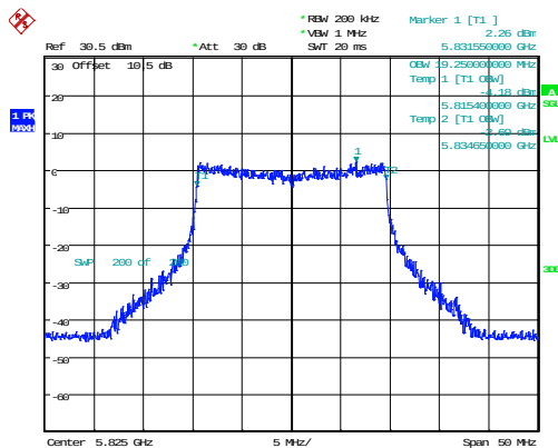
802.11ax20_5825MHz_RU_Full_Chain 0 19.250MHz
