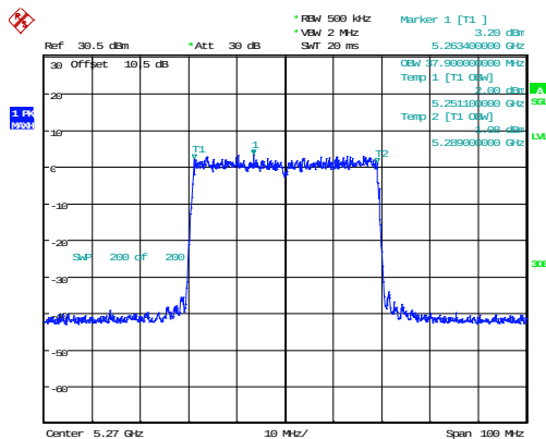
802.11ax40_5270MHz_RU_Full_Chain 1 37.900MHz
