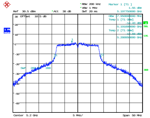
802.11a_5200MHz_Chain 0 17.950MHz
