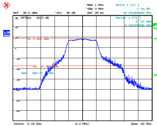
802.11n20_5180MHz_Chain 0 40.262MHz
