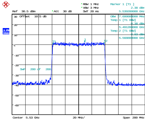
802.11ax80_5530MHz_RU_Full_Chain 0 77.600MHz
