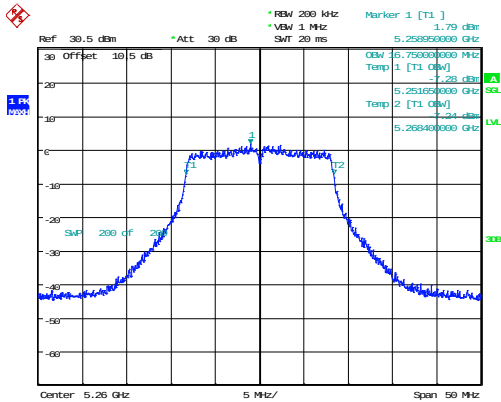
802.11a_5260MHz_Chain 0 16.750MHz
