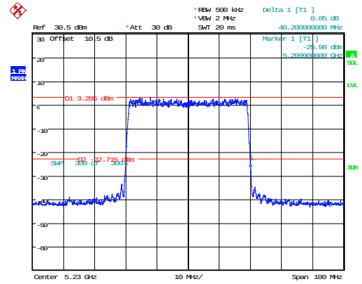
802.11ax40_5230MHz_RU_Full_Chain 0 40.200MHz
