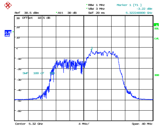
802.11ax20_5320MHz_RU_106/54_Chain 1
