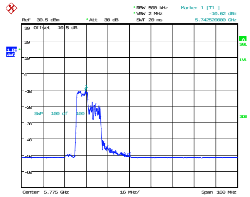
802.11ax80_5775MHz_RU_106/53_Chain 1
