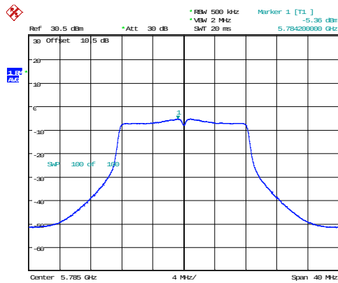
802.11a_5785MHz_Chain 1
