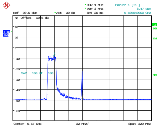
802.11ax160_5570MHz_RU_242/61_Chain 0
