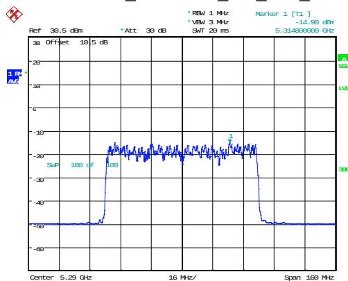
802.11ax80_5290MHz_RU_Full_Chain 0
