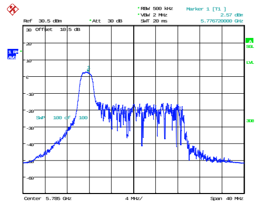
802.11ax20_5785MHz_RU_26/0_Chain 0
