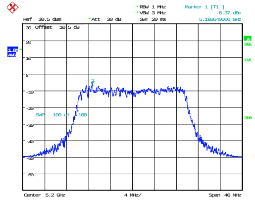
802.11ax20_5200MHz_RU_Full_Chain 0
