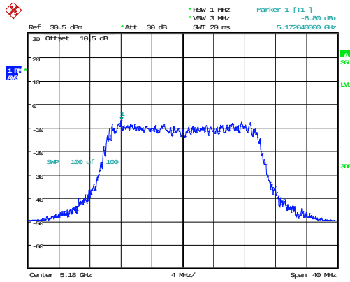
802.11ax20_5180MHz_RU_Full_Chain 0
