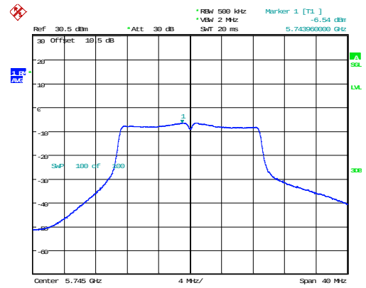
802.11n20_5745MHz_Chain 1
