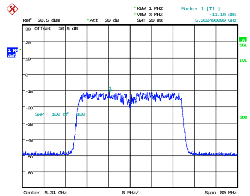
802.11ax40_5310MHz_RU_Full_Chain 1
