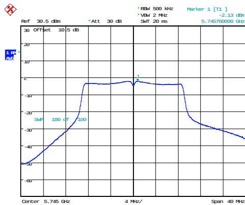
802.11n20_5745MHz_Chain 0
