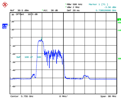
802.11ax40_5755MHz_RU_52/37_Chain 0
