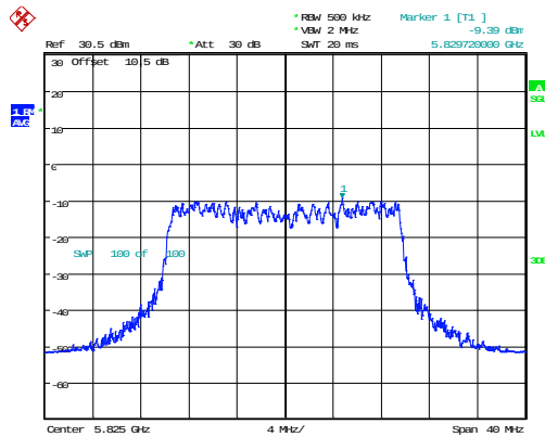
802.11ax20_5825MHz_RU_Full_Chain 0
