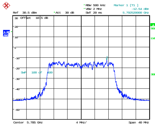
802.11ax20_5785MHz_RU_Full_Chain 1
