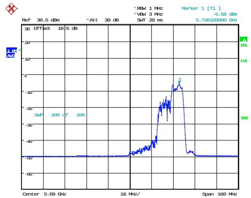
802.11ax80_5690MHz_RU_106/60_Chain 1
