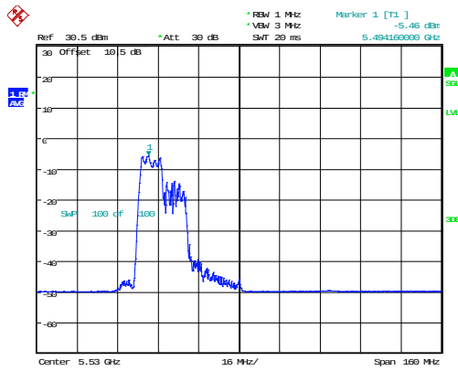
802.11ax80_5530MHz_RU_106/53_Chain 1
