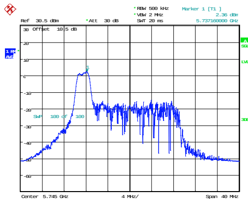
802.11ax20_5745MHz_RU_26/0_Chain 0
