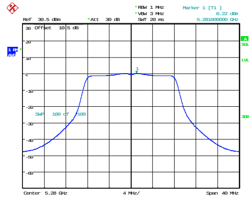
802.11a_5280MHz_Chain 0
