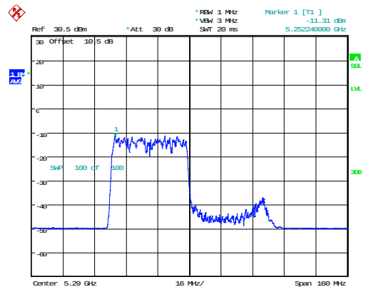
802.11ax80_5290MHz_RU_484/65_Chain 1
