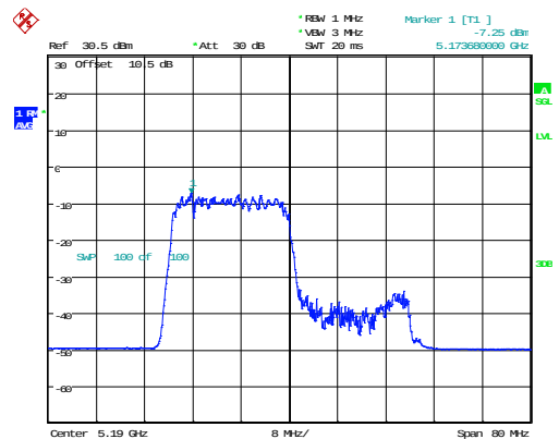
802.11ax40_5190MHz_RU_242/61_Chain 1
