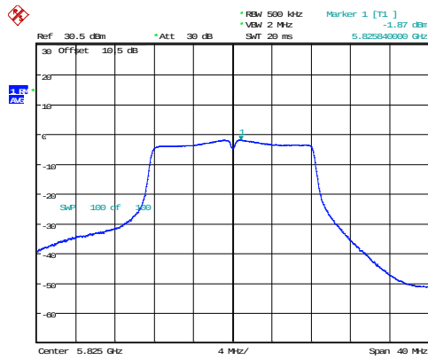
802.11a_5825MHz_Chain 0
