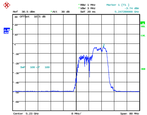
802.11ax40_5230MHz_RU_106/56_Chain 1
