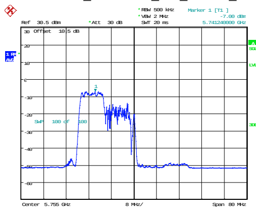
802.11ax40_5755MHz_RU_106/53_Chain 0
