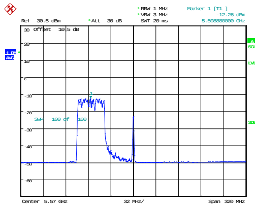
802.11ax160_5570MHz_RU_484/65_Chain 0
