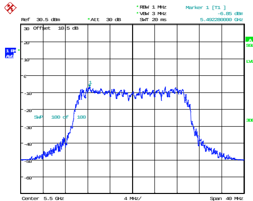
802.11ax20_5500MHz_RU_Full_Chain 0
