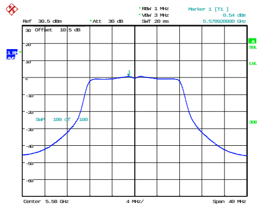
802.11a_5580MHz_Chain 0
