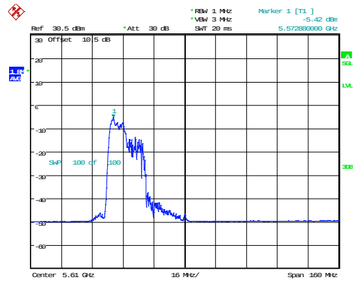
802.11ax80_5610MHz_RU_106/53_Chain 1
