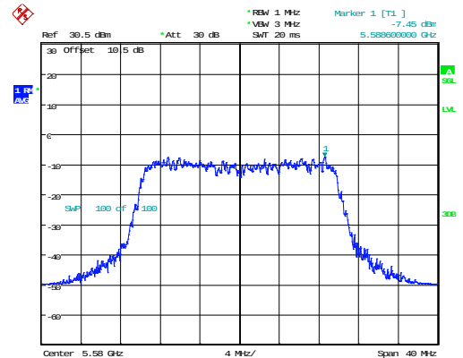
802.11ax20_5580MHz_RU_Full_Chain 0
