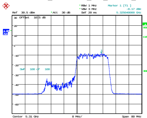
802.11ax40_5310MHz_RU_242/62_Chain 0
