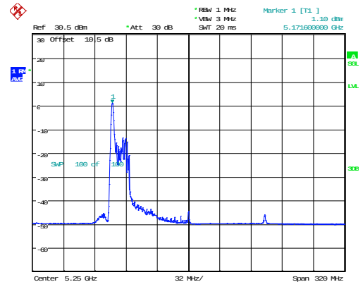
802.11ax160_5250MHz_RU_26/0_Chain 1
