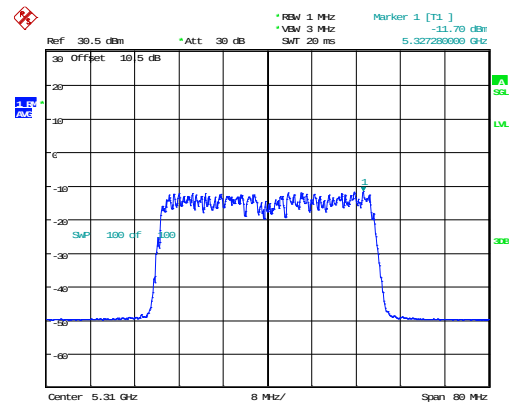
802.11ax40_5310MHz_RU_Full_Chain 0
