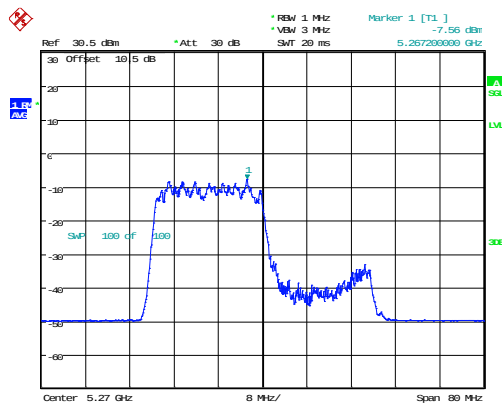
802.11ax40_5270MHz_RU_242/61_Chain 0
