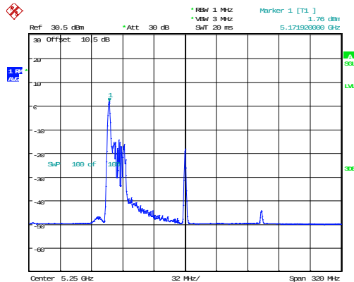
802.11ax160_5250MHz_RU_26/0_Chain 0
