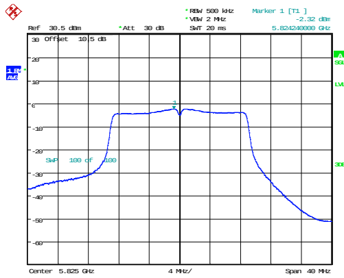
802.11n20_5825MHz_Chain 0
