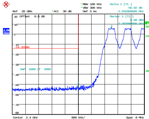
DH1_Hopping_Lower 56.92dB
