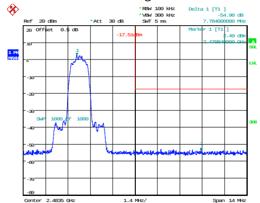
2DH1_High 54.90dB
