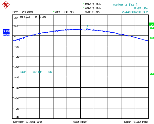
2DH1_Middle 6.02dBm
