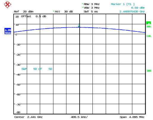
DH1_Middle 6.59dBm
