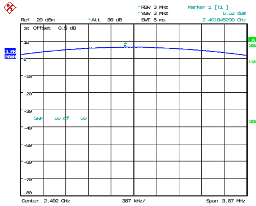
DH1_Low 6.52dBm
