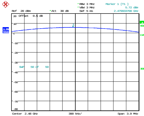
DH1_High 5.72dBm
