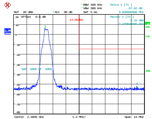
DH1_High 57.62dB
