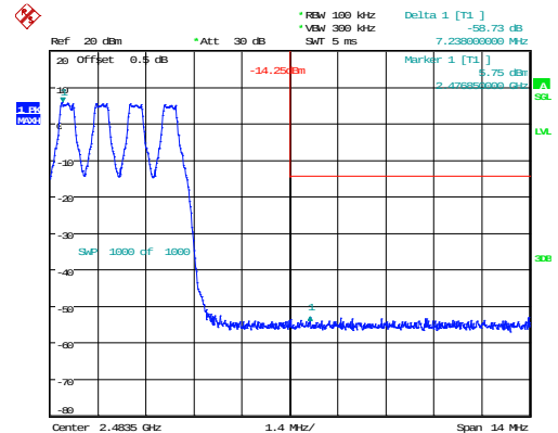
DH1_Hopping_Upper 58.73dB
