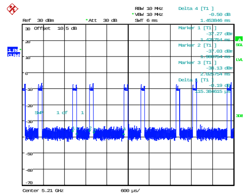
802.11ax80_5210MHz_RU_242/61_Chain 0 0.240ms,1.454ms
