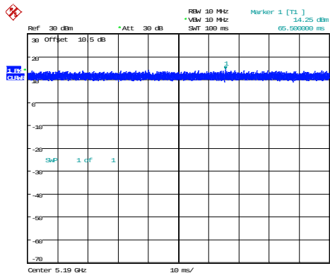
802.11n40_5190MHz_Chain 0 100ms,100ms
