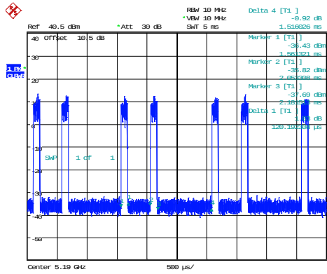
802.11ax40_5190MHz_RU_242/61_Chain 0 0.249ms,1.516ms
