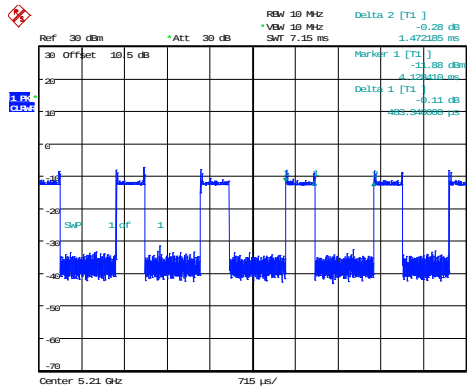
802.11ax80_5210MHz_RU_26/0_Chain 0 0.483ms,1.472ms
