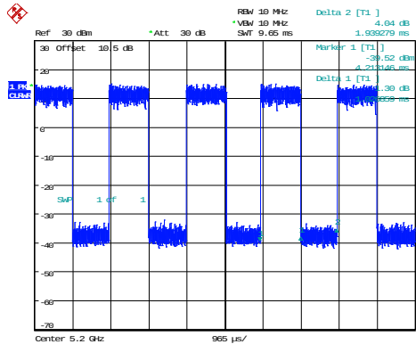
802.11ax20_5200MHz_RU_Full_Chain 0 1.027ms,1.939ms
