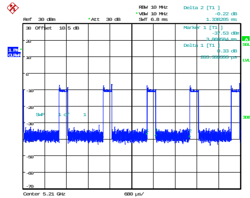
802.11ax80_5210MHz_RU_52/37_Chain 0 0.283ms,1.338ms
