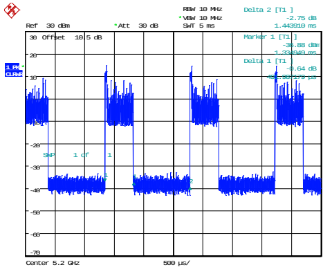
802.11ax20_5200MHz_RU_26/0_Chain 0 0.492ms,1.444ms
