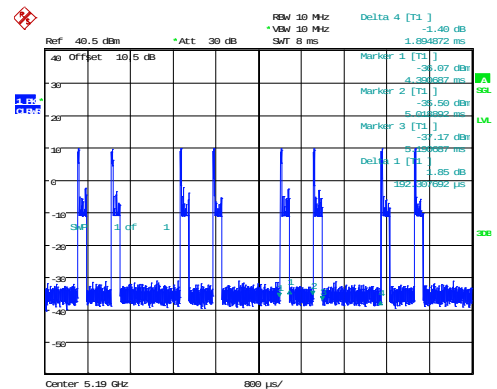
802.11ax40_5190MHz_RU_106/53_Chain 0 0.364ms,1.895ms
