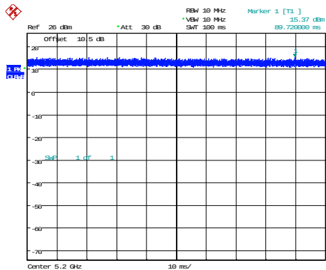
802.11a_5200MHz_Chain 0 100ms,100ms
