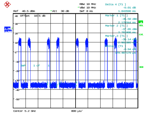
802.11ax20_5200MHz_RU_106/53_Chain 0 0.358ms,1.844ms
