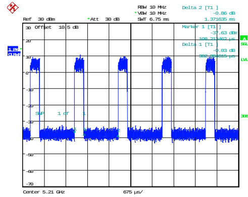
802.11ax80_5210MHz_RU_Full_Chain 0 0.303ms,1.372ms
