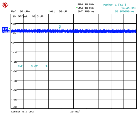
802.11n20_5200MHz_Chain 0 100ms,100ms
