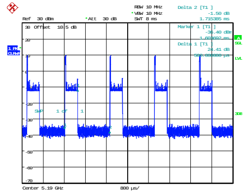
802.11ax40_5190MHz_RU_26/0_Chain 0 0.500ms,1.715ms
