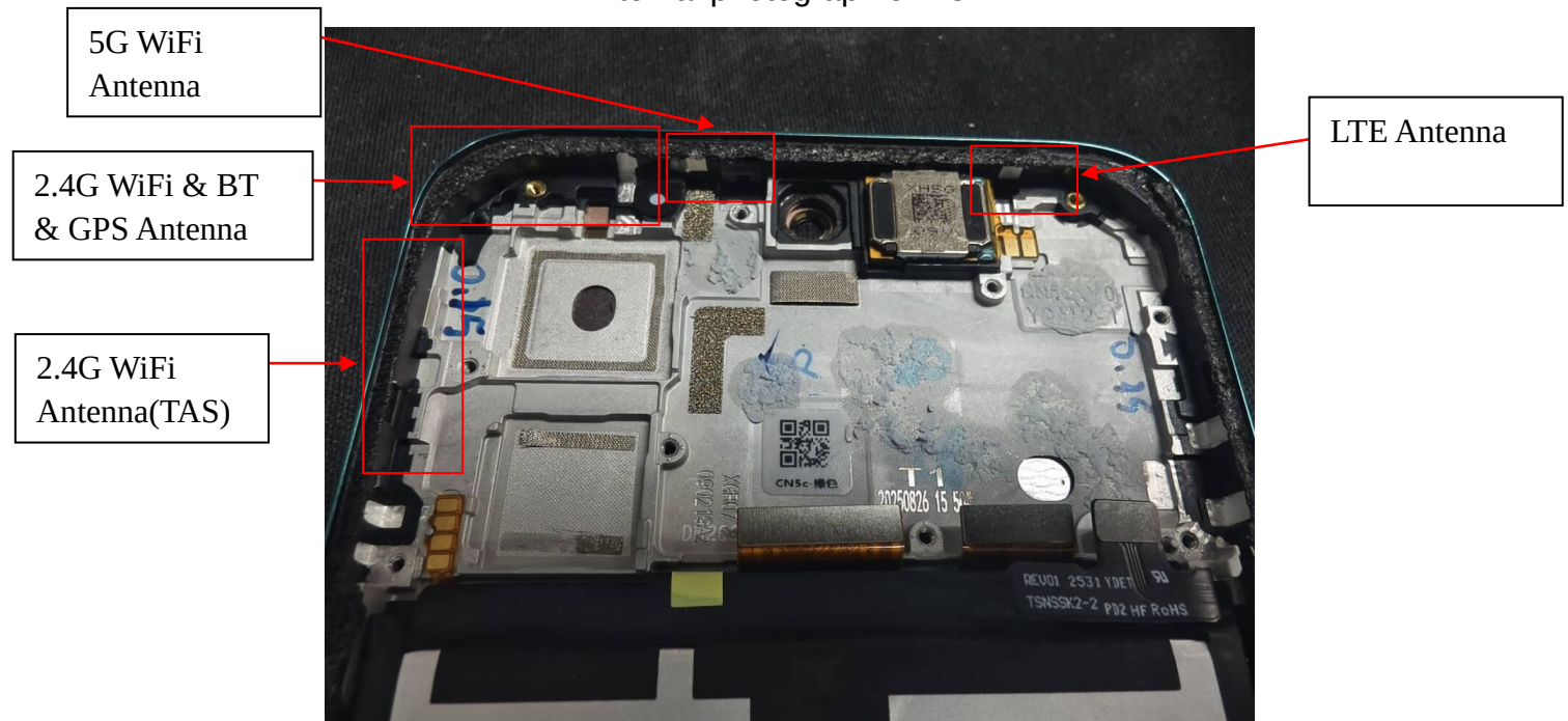
Internal photograph of EUT
