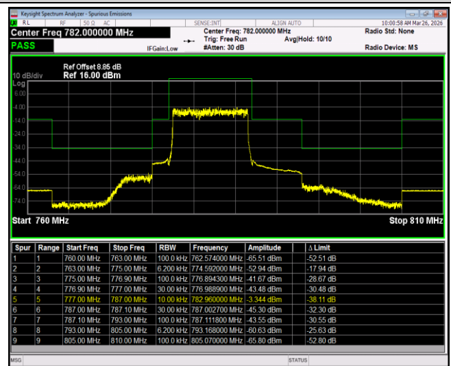
Band13-10MHz-64QAM-23230-1RB#49
