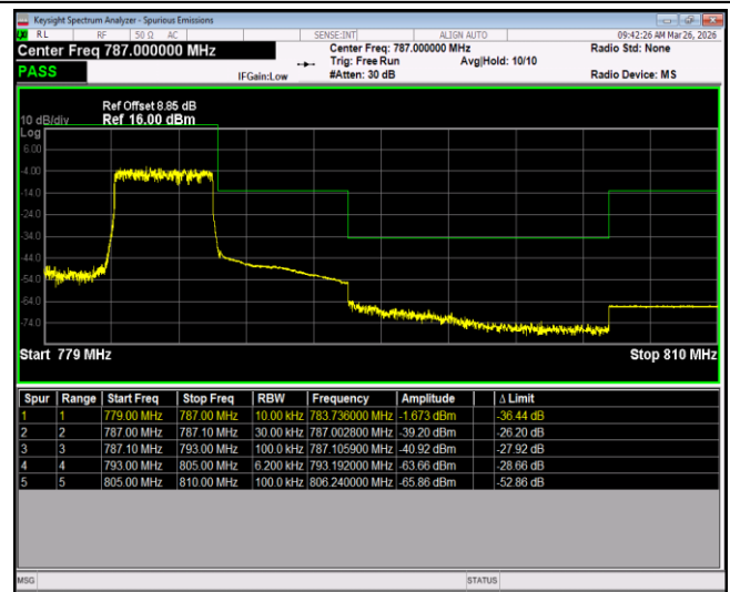
Band13-10MHz-QPSK-23230-1RB#49
