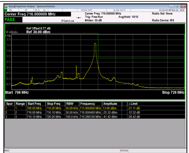
Band17-5MHz-64QAM-23755-1RB#0
