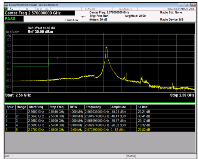
Band38-5MHz-QPSK-37775-25RB#0
