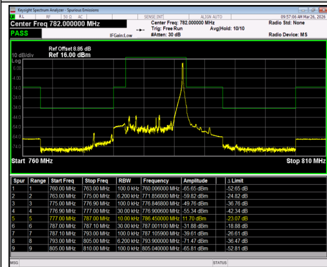
Band13-10MHz-64QAM-23230-1RB#0
