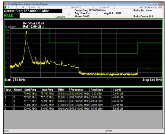
Band13-5MHz-64QAM-23255-25RB#0
