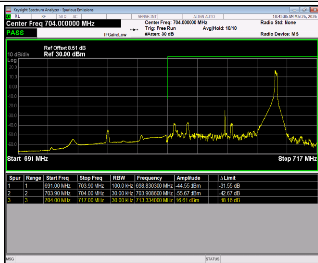
Band17-10MHz-64QAM-23800-1RB#0
