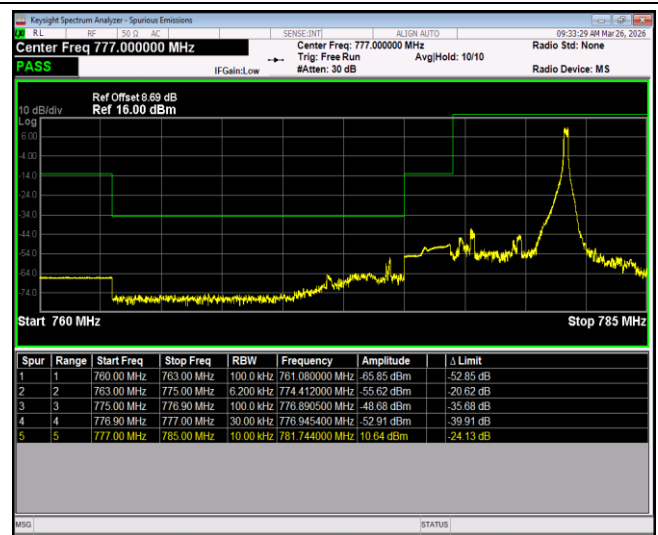
Band13-5MHz-64QAM-23255-1RB#0
