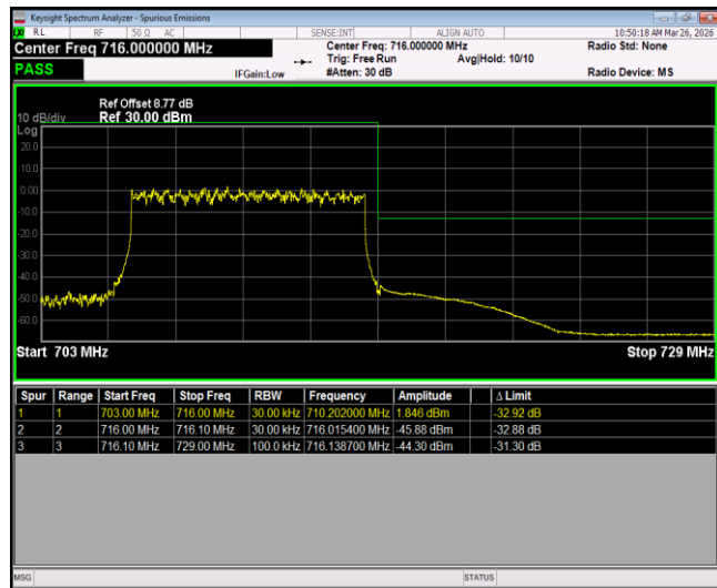
Band17-10MHz-64QAM-23780-1RB#49
