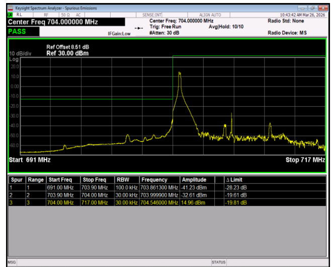
Band17-10MHz-64QAM-23780-50RB#0
