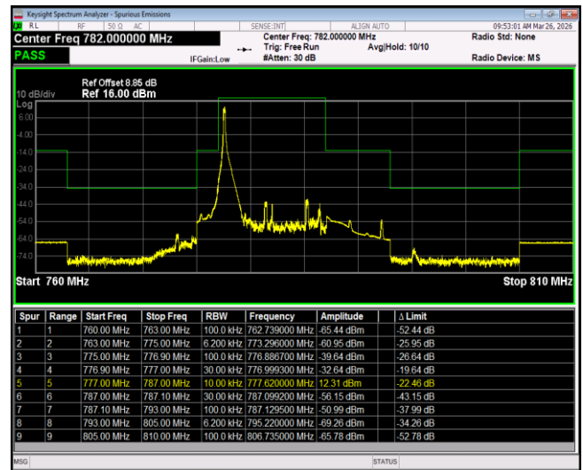
Band13-10MHz-16QAM-23230-50RB#0
