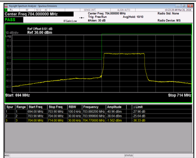
Band17-5MHz-64QAM-23825-1RB#24
