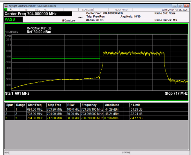
Band17-10MHz-64QAM-23800-1RB#49
