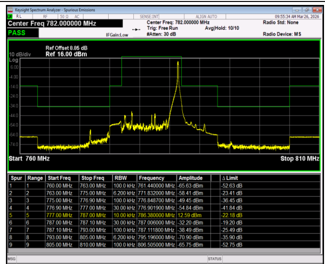
Band13-10MHz-16QAM-23230-1RB#0
