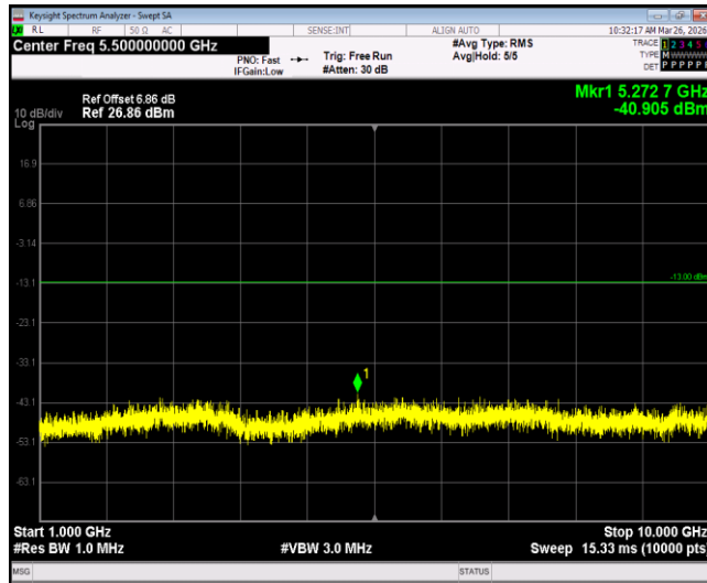
Band17-10MHz-QPSK-23780-1RB#0-Range2:1000~10000MHz
