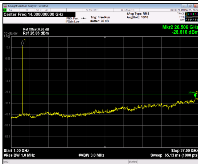
Band38-5MHz-64QAM-38000-1RB#0-Range2:1000~27000MHz
