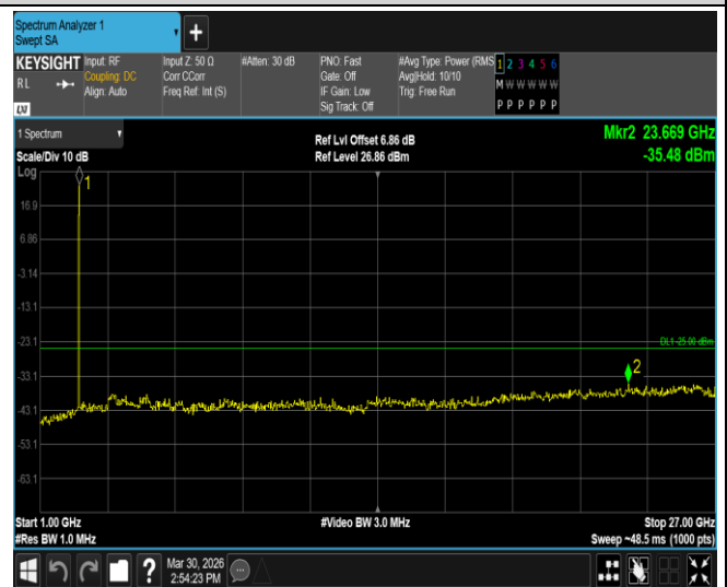
Band41-20MHz-64QAM-40620-1RB#0-Range2:1000~27000MHz
