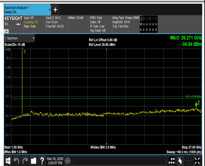
Band41-5MHz-64QAM-39675-1RB#0-Range2:1000~27000MHz
