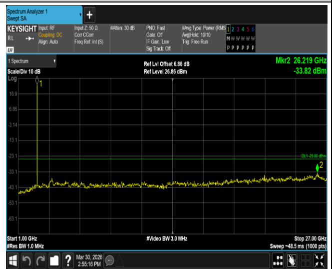
Band41-20MHz-64QAM-40620-1RB#0-Range2:1000~27000MHz
