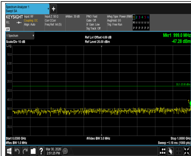
Band41-5MHz-16QAM-41565-1RB#0-Range1:30~1000MHz
