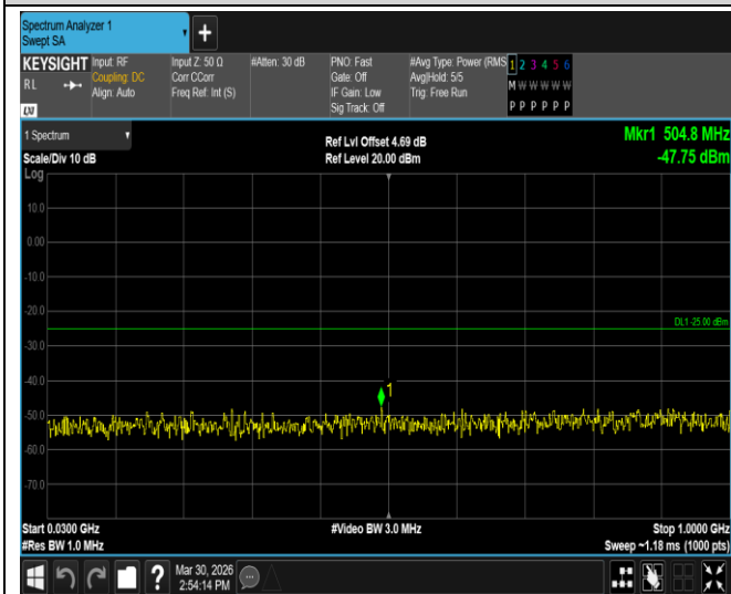
Band41-20MHz-64QAM-40620-1RB#0-Range1:30~1000MHz
