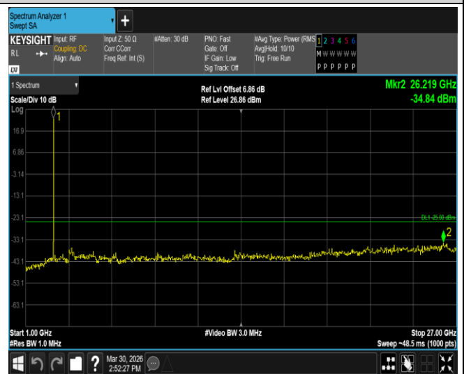
Band41-5MHz-64QAM-39675-1RB#0-Range2:1000~27000MHz
