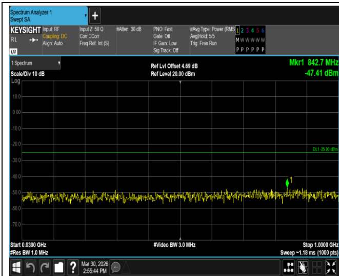
Band41-20MHz-64QAM-39750-1RB#0-Range1:30~1000MHz
