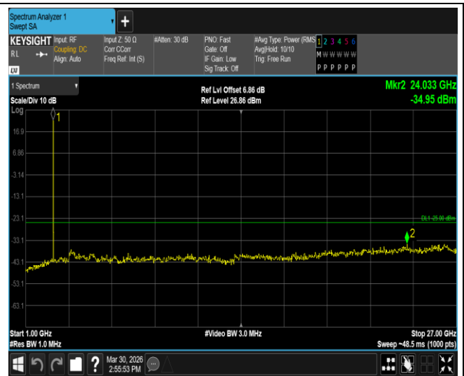
Band41-20MHz-64QAM-39750-1RB#0-Range2:1000~27000MHz
