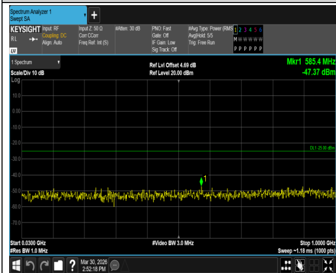
Band41-5MHz-64QAM-39675-1RB#0-Range1:30~1000MHz
