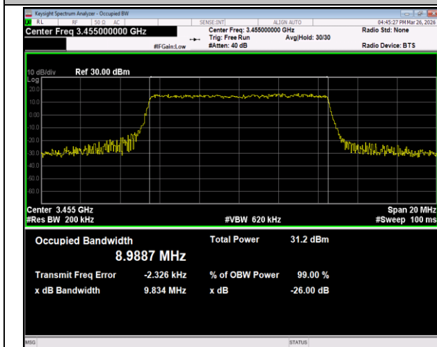
Band42(3450-3550)-10MHz-QPSK-42590-50RB#0-PASS
