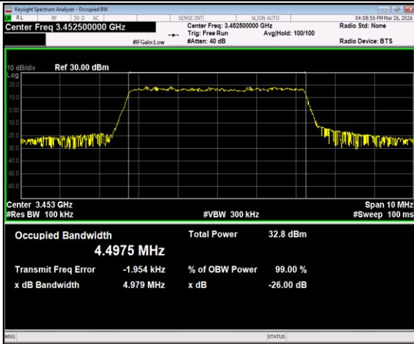
Band42(3450-3550)-5MHz-16QAM-42115-25RB#0-PASS
