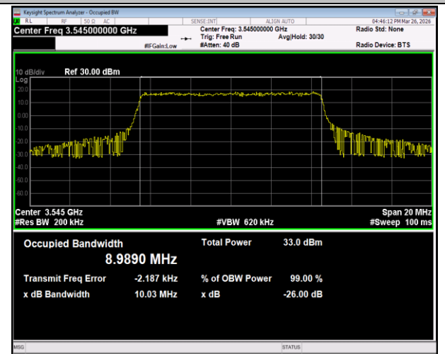
Band42(3450-3550)-10MHz-16QAM-43040-50RB#0-PASS
