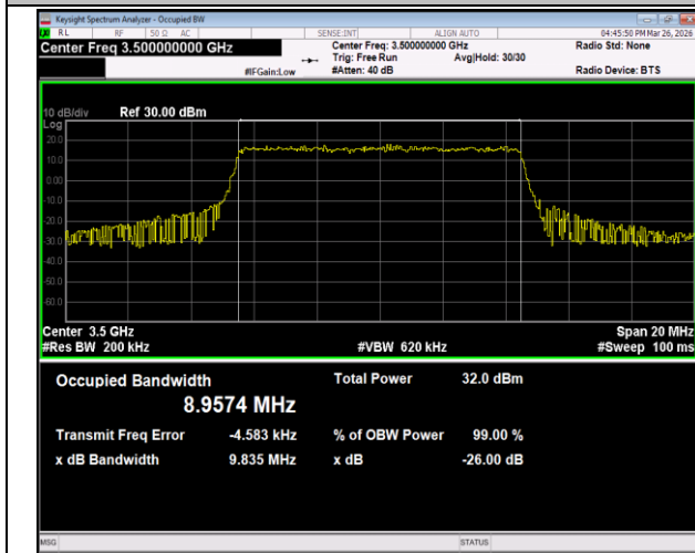
Band42(3450-3550)-10MHz-64QAM-43040-50RB#0-PASS
