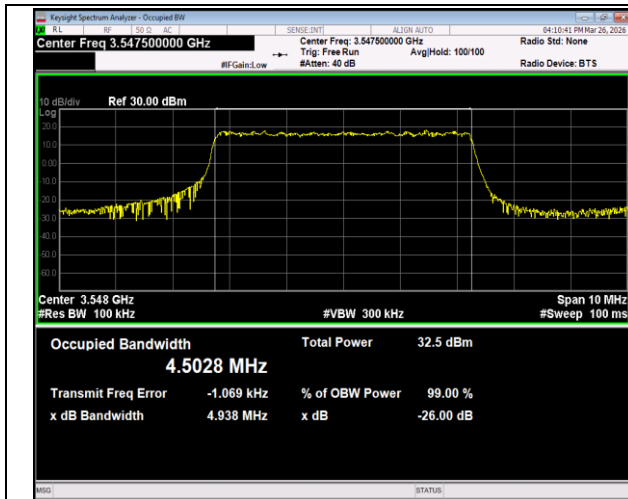
Band42(3450-3550)-5MHz-16QAM-43065-25RB#0-PASS
