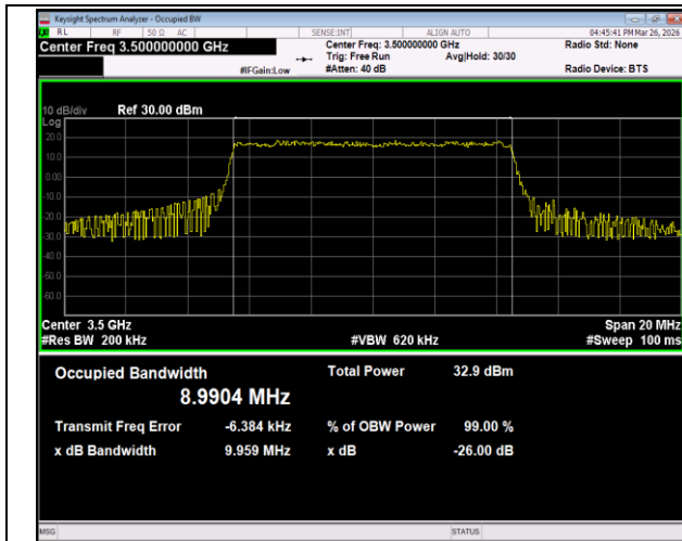
Band42(3450-3550)-10MHz-16QAM-42590-50RB#0-PASS
