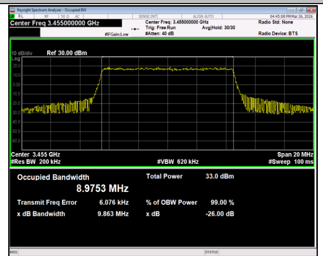
Band42(3450-3550)-10MHz-16QAM-42140-50RB#0-PASS
