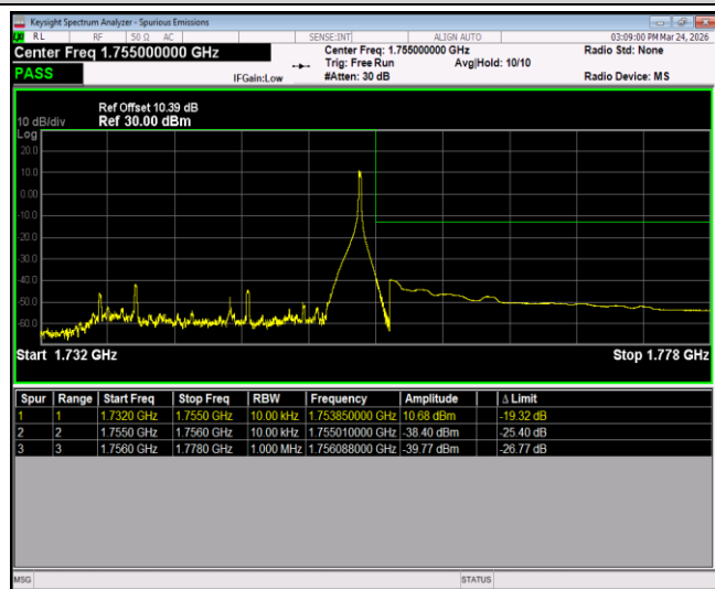
Band4-20MHz-16QAM-20050-1RB#0
