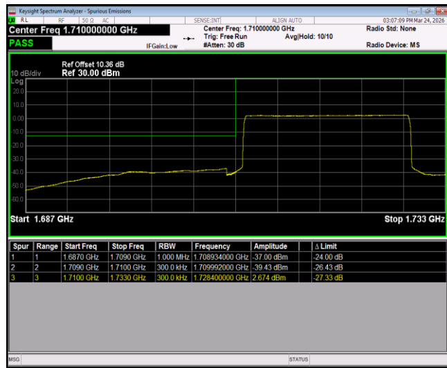
Band4-20MHz-16QAM-20300-1RB#99
