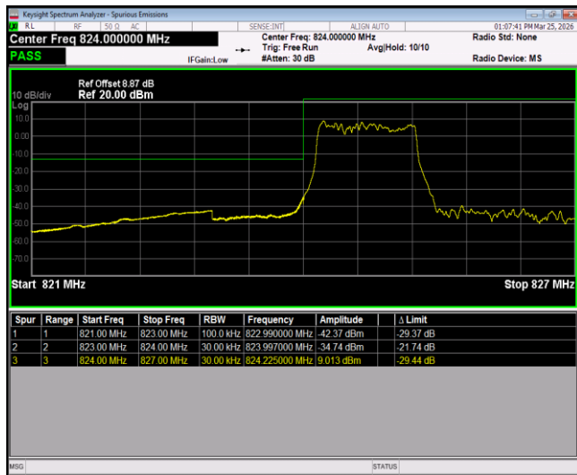
Band5-1.4MHz-64QAM-20643-1RB#5
