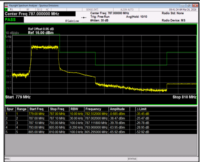
Band13-5MHz-64QAM-23205-1RB#24
