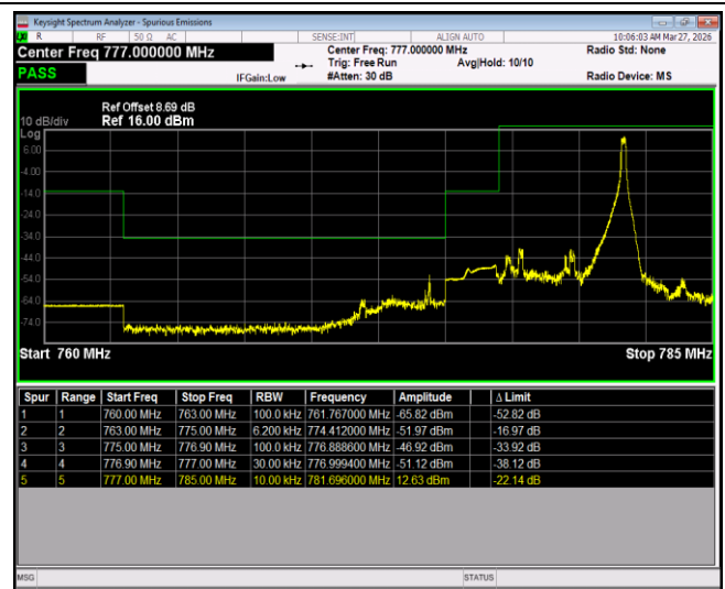
Band13-5MHz-16QAM-23255-1RB#0
