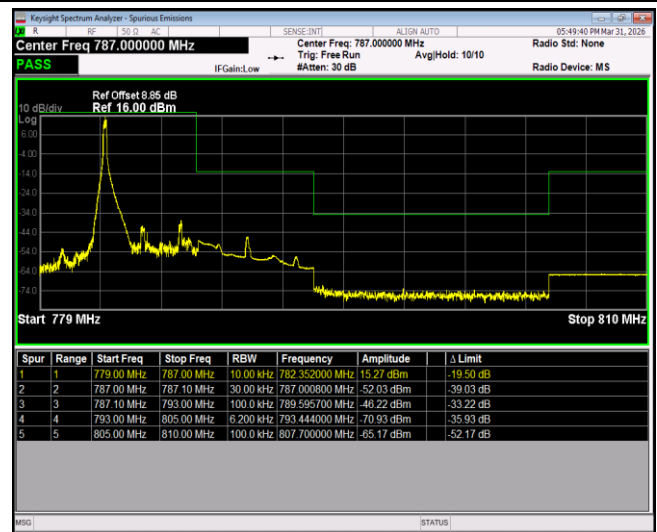
Band13-5MHz-QPSK-23255-25RB#0
