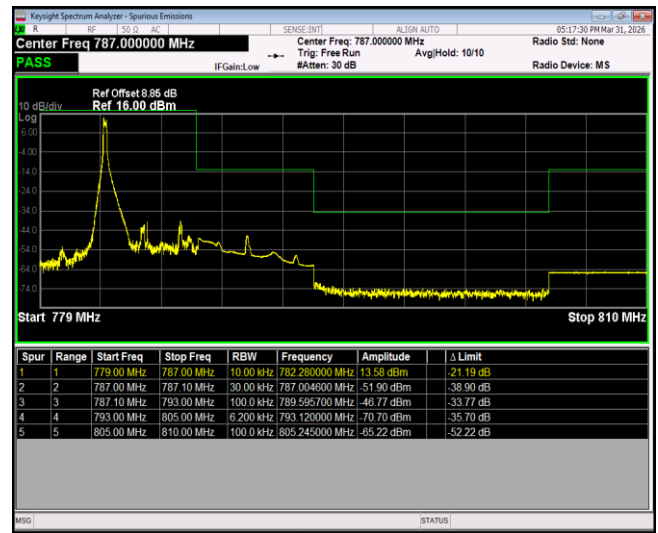
Band13-5MHz-16QAM-23255-25RB#0
