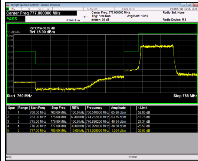
Band13-5MHz-16QAM-23255-1RB#24
