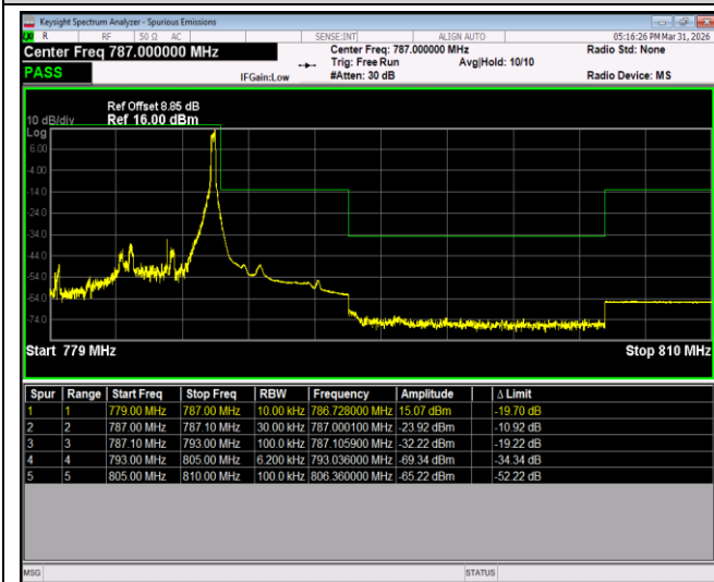
Band13-5MHz-16QAM-23205-1RB#0
