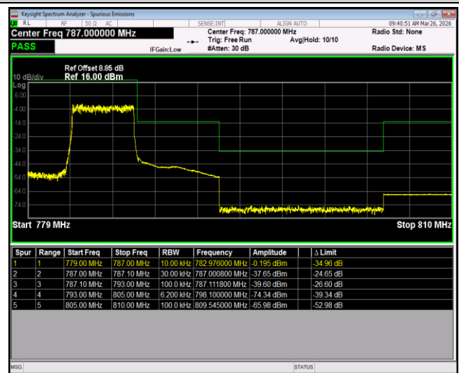
Band13-5MHz-16QAM-23205-1RB#24
