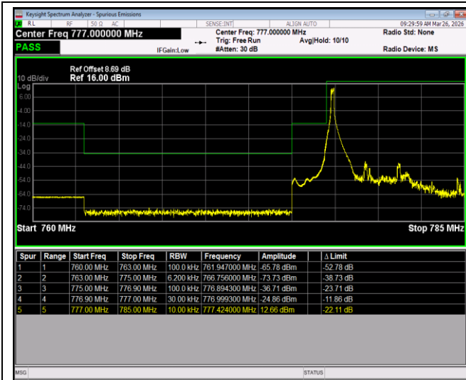
Band13-5MHz-QPSK-23205-25RB#0
