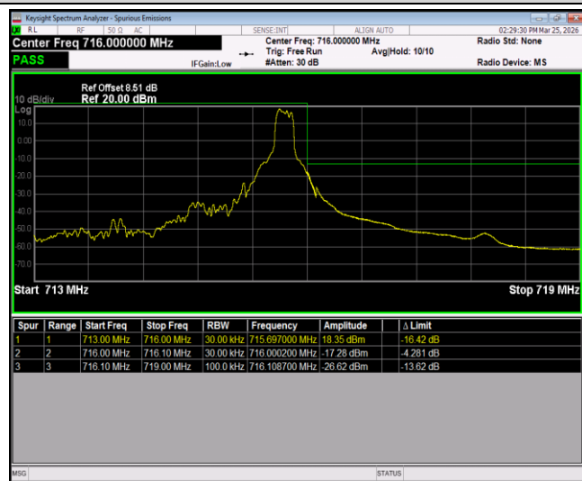
Band12-1.4MHz-16QAM-23017-1RB#0
