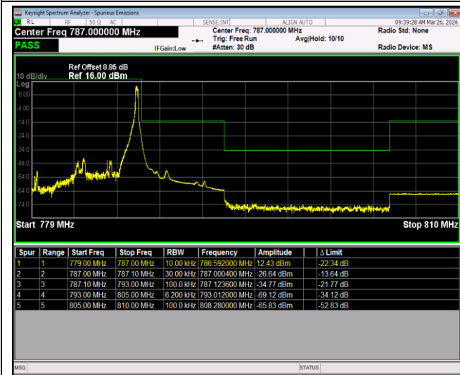
Band13-5MHz-64QAM-23205-1RB#0
