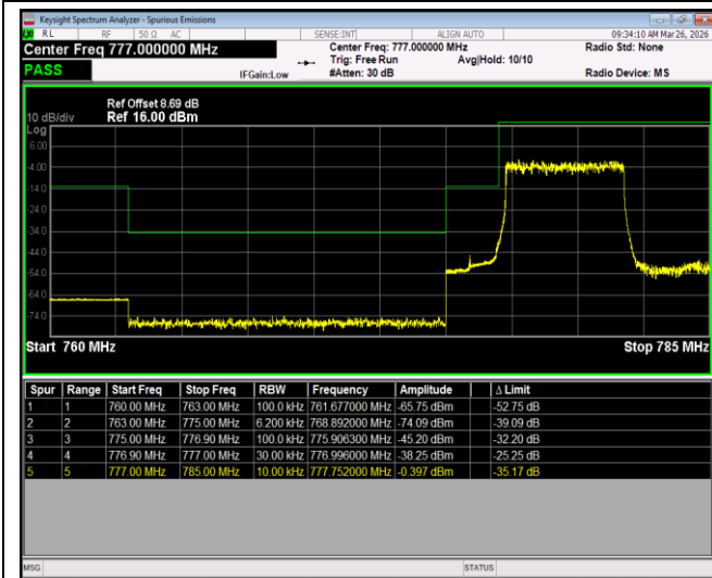
Band13-5MHz-QPSK-23255-1RB#24
