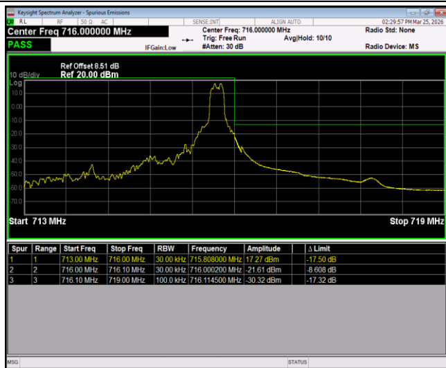
Band12-1.4MHz-64QAM-23017-1RB#0
