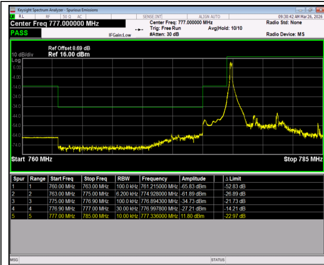
Band13-5MHz-16QAM-23205-25RB#0
