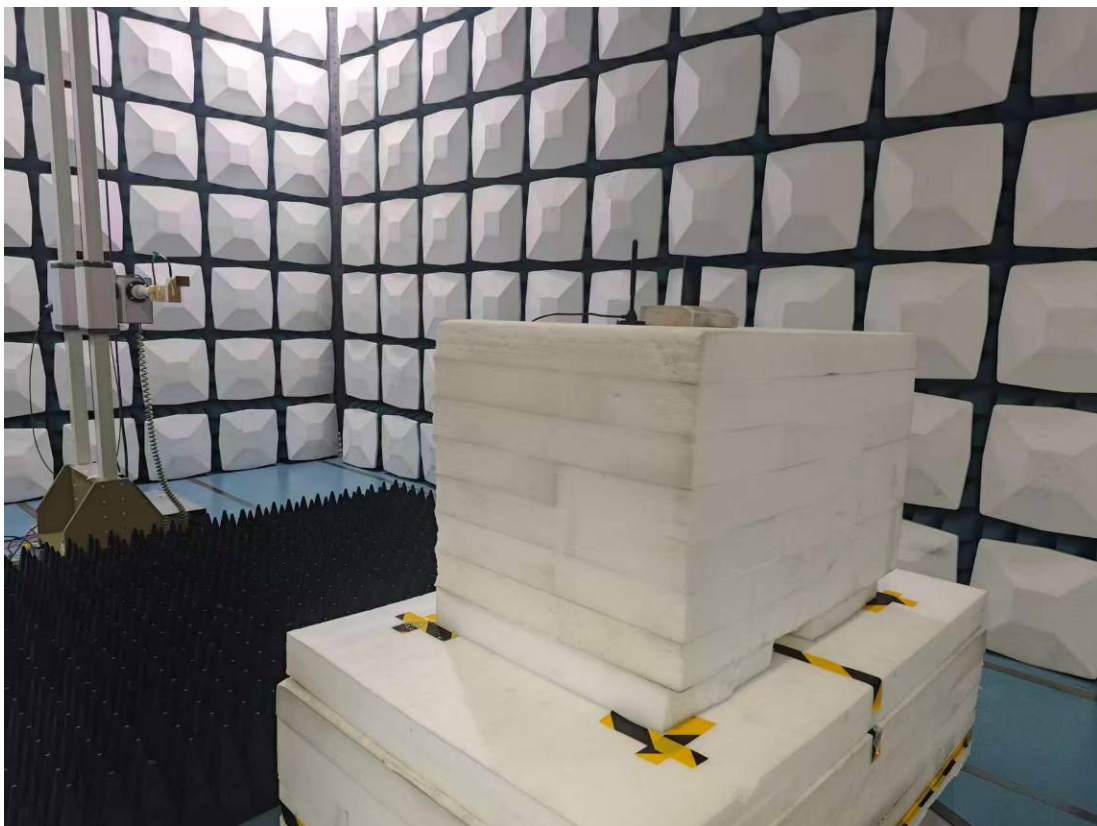
Radiated Emission 26.5-38GHz View
