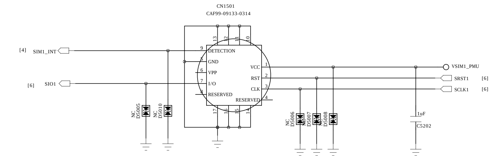
SIM1 SOCKET
