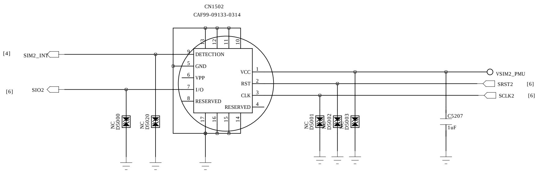
SIM2 SOCKET
