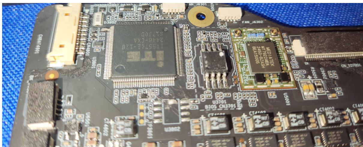
Internal photograph of EUT
