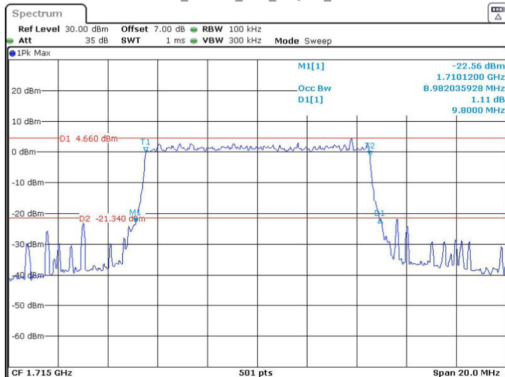
Band 66_10 MHz_Low_16QAM_RB50#0
