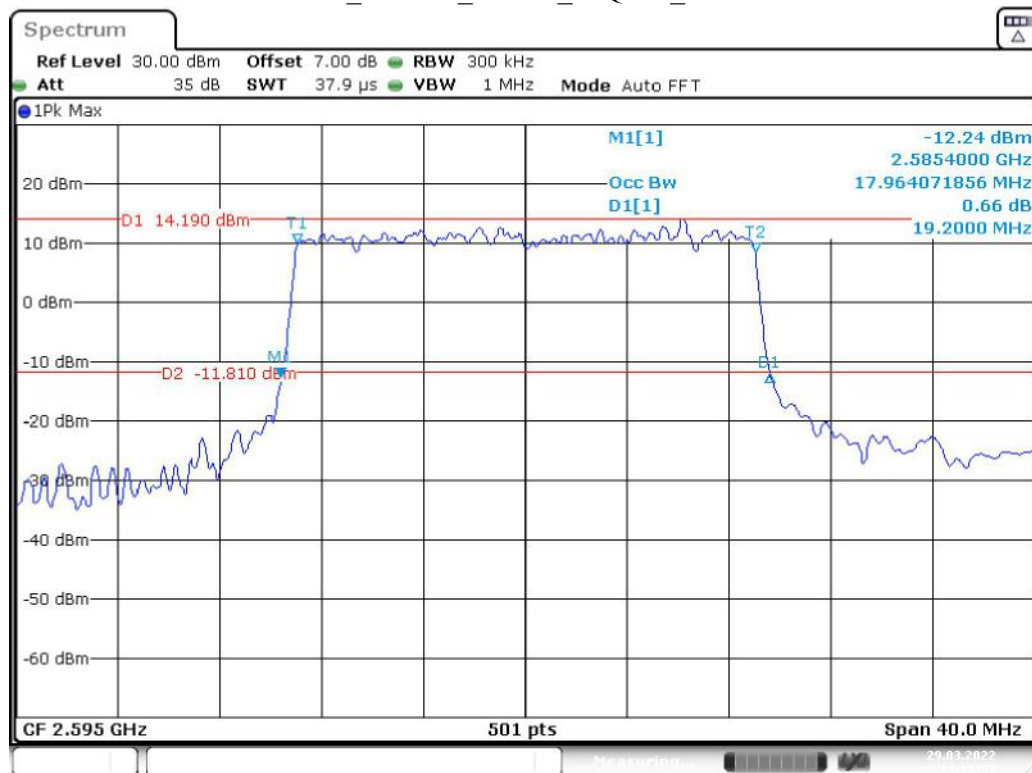
Band 41_20 MHz_Middle_16QAM_RB100#0
