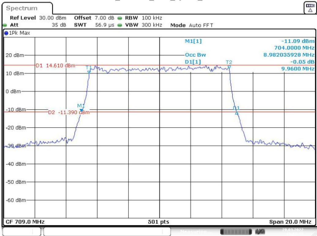
Band 17_10 MHz_Low_QPSK_RB50#0
