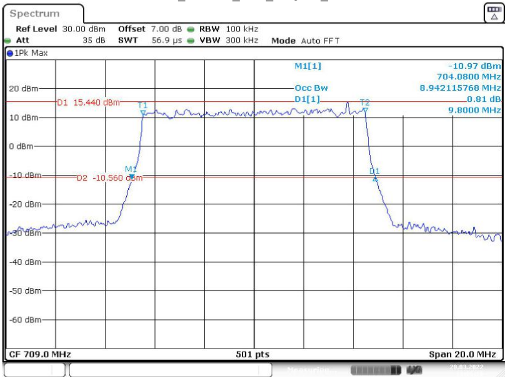
Band 17_10 MHz_Low_16QAM_RB50#0
