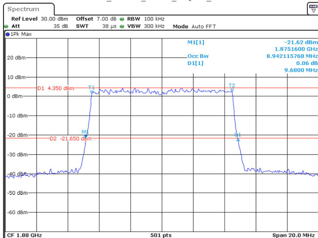
Band 2_10 MHz_Middle_16QAM_RB50#0
