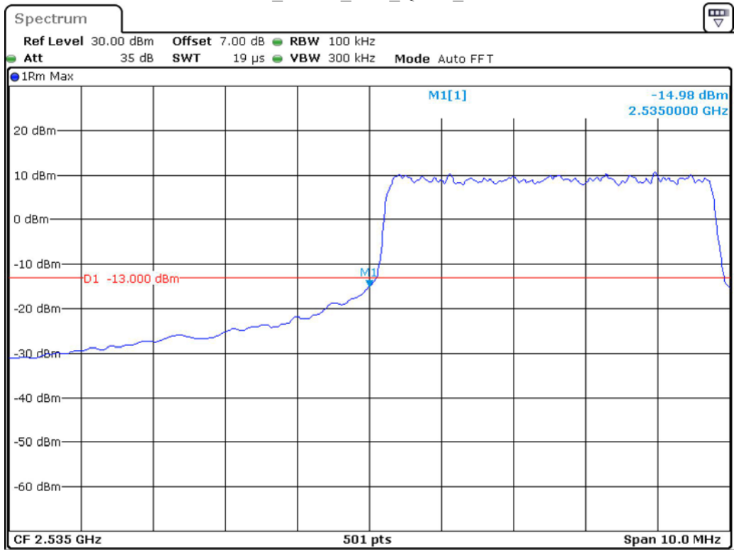
Band 41_5 MHz_Low_QPSK_RB25#0
