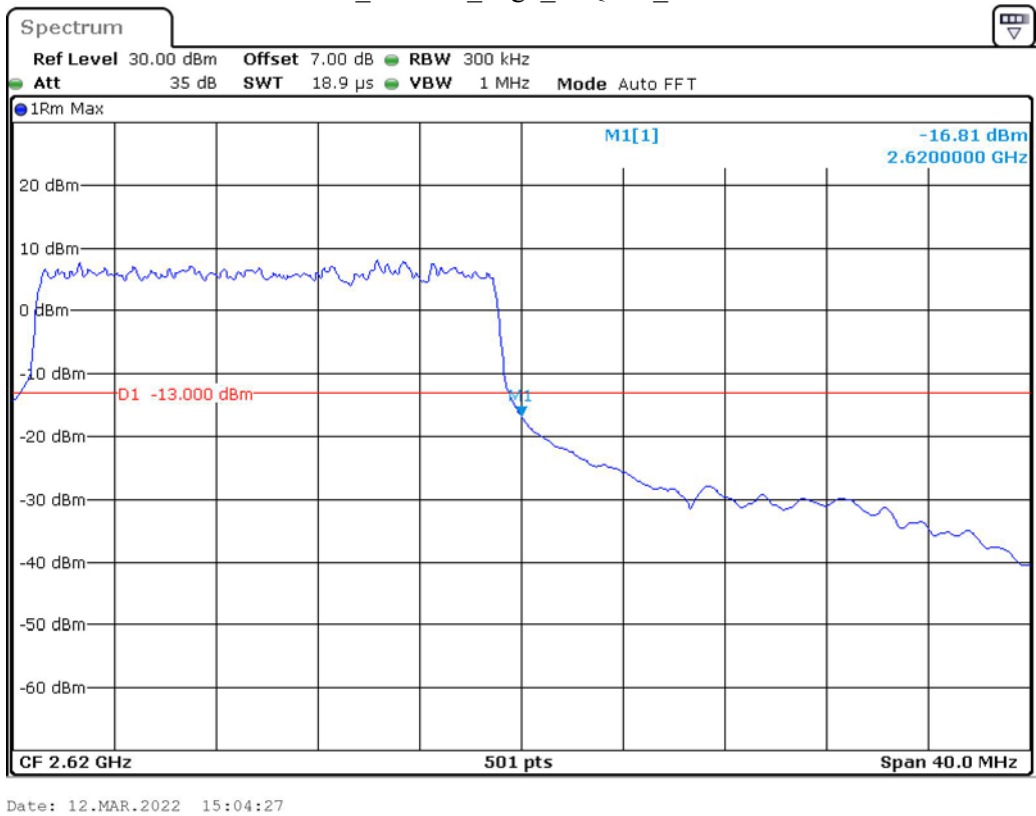
Band 38_20 MHz_High_16QAM_RB100#0
