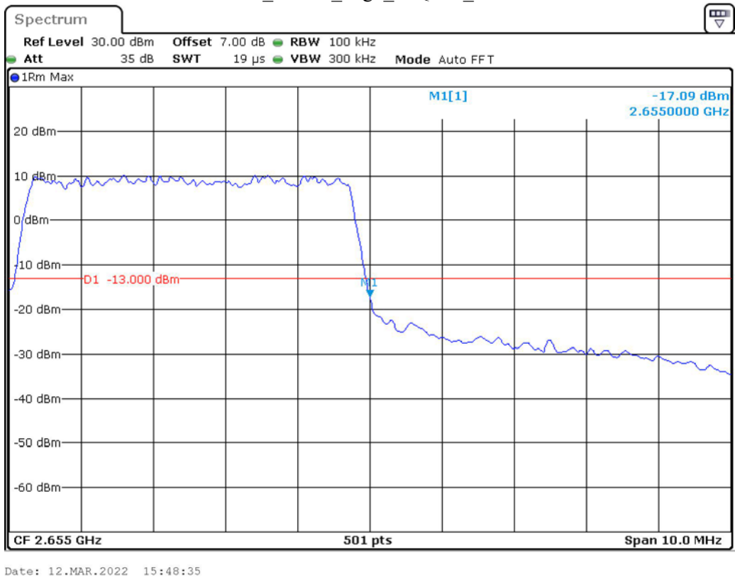
Band 41_5 MHz_High_16QAM_RB25#0
