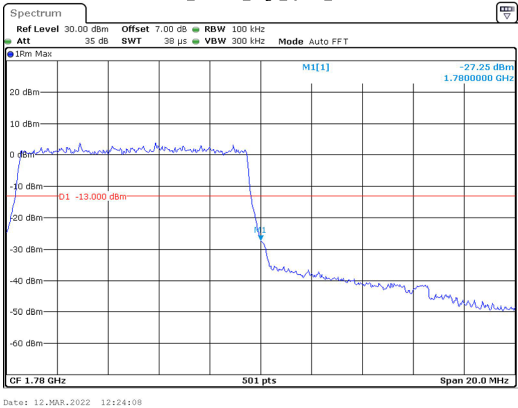
Band 66_10 MHz_High_QPSK_RB50#0
