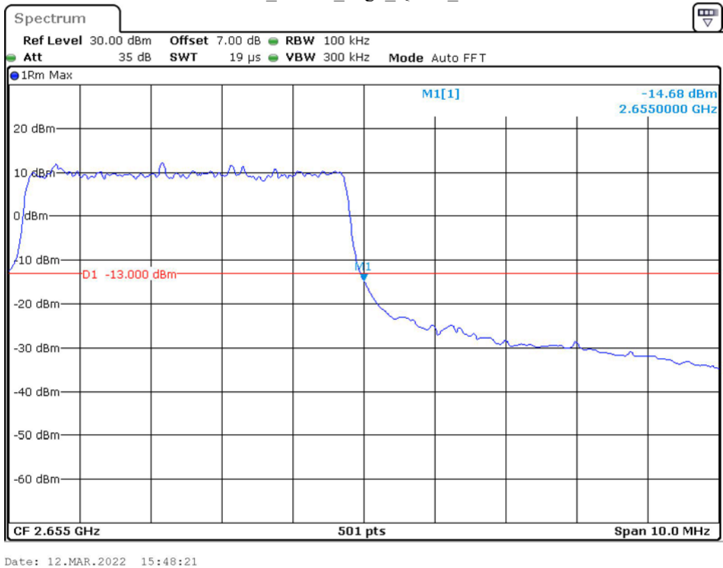
Band 41_5 MHz_High_QPSK_RB25#0
