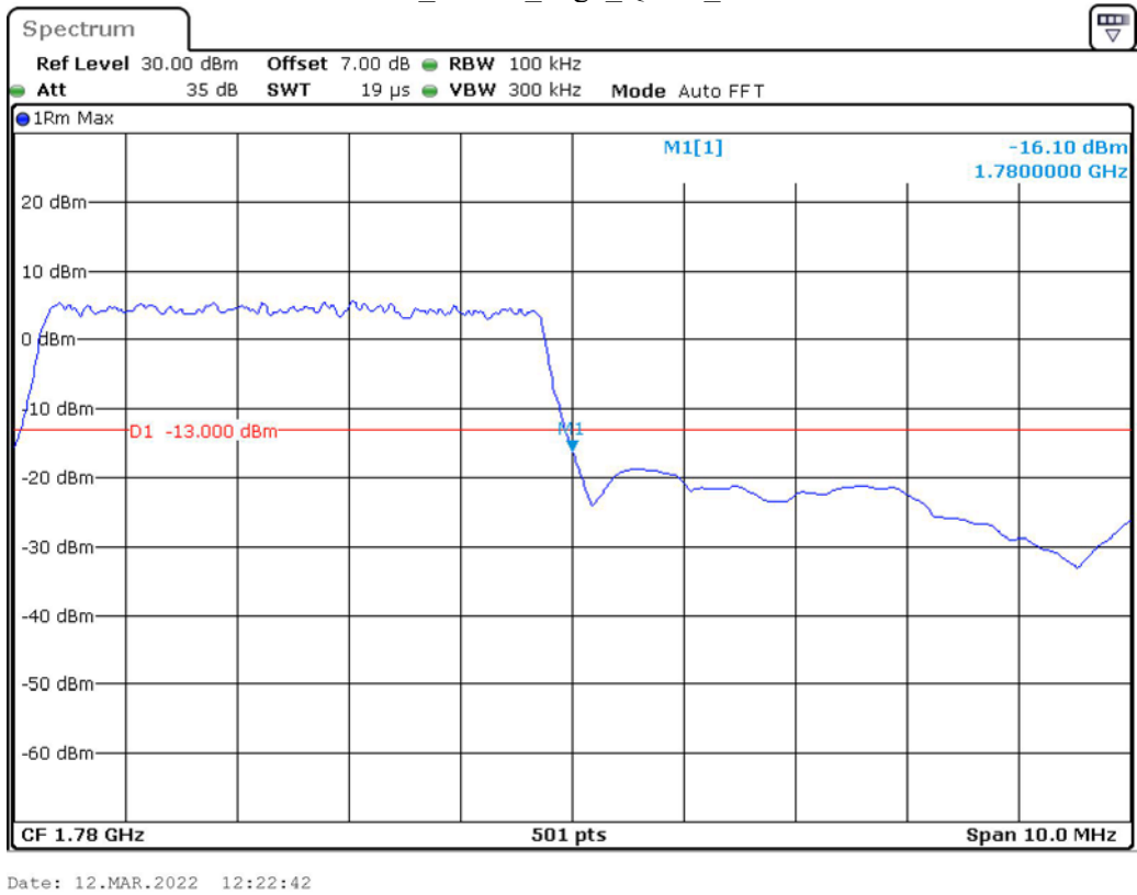
Band 66_5 MHz_High_QPSK_RB25#0
