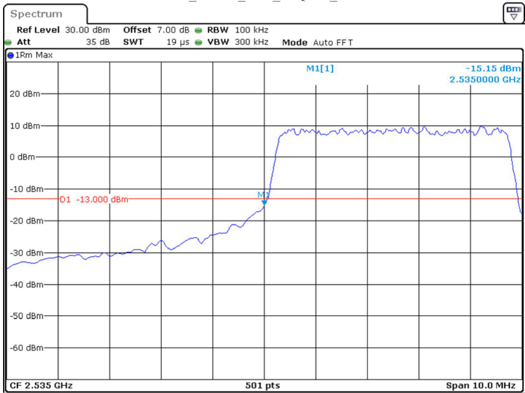
Band 41_5 MHz_Low_16QAM_RB25#0
