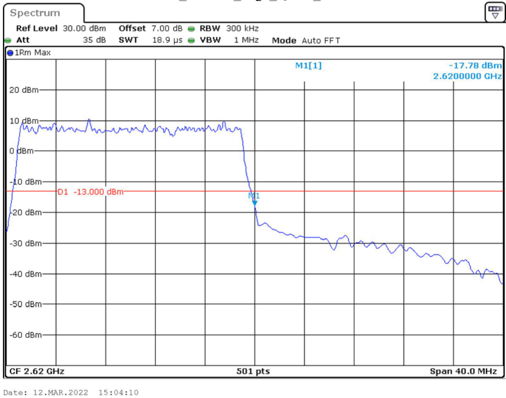
Band 38_20 MHz_High_QPSK_RB100#0
