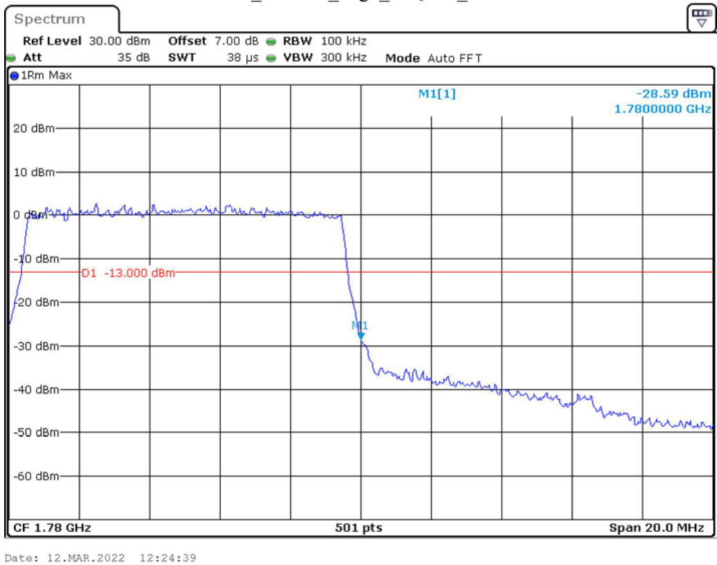
Band 66_10 MHz_High_16QAM_RB50#0
