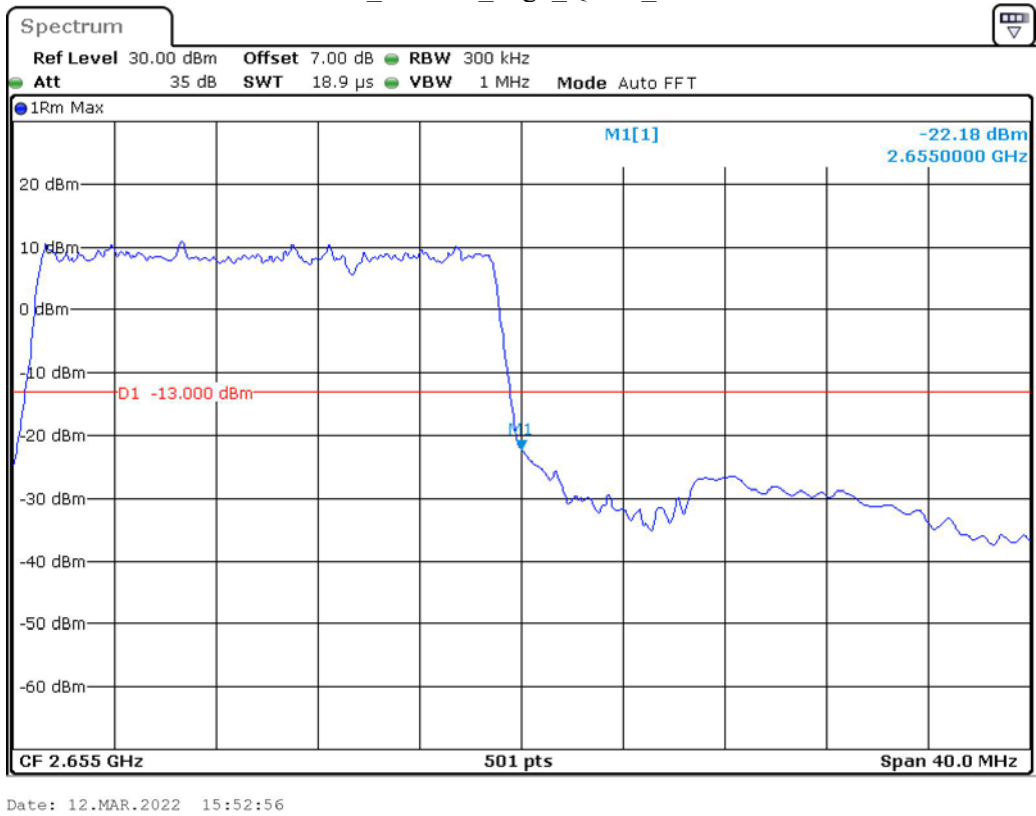
Band 41_20 MHz_High_QPSK_RB100#0
