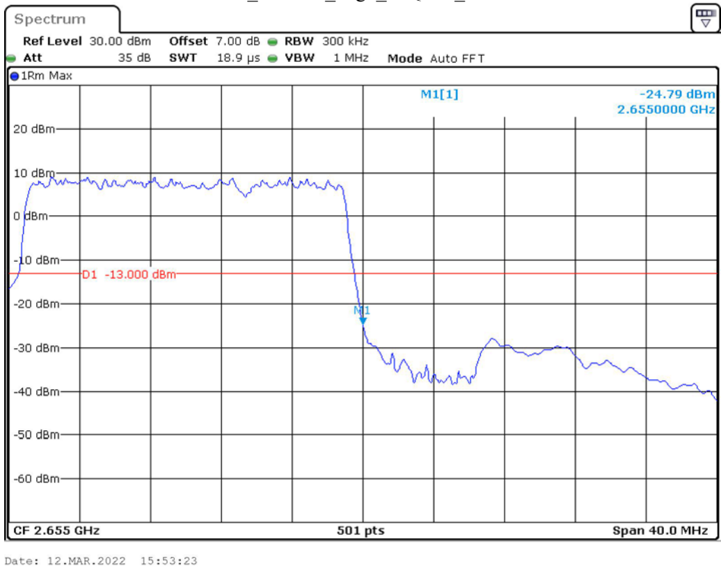
Band 41_20 MHz_High_16QAM_RB100#0
