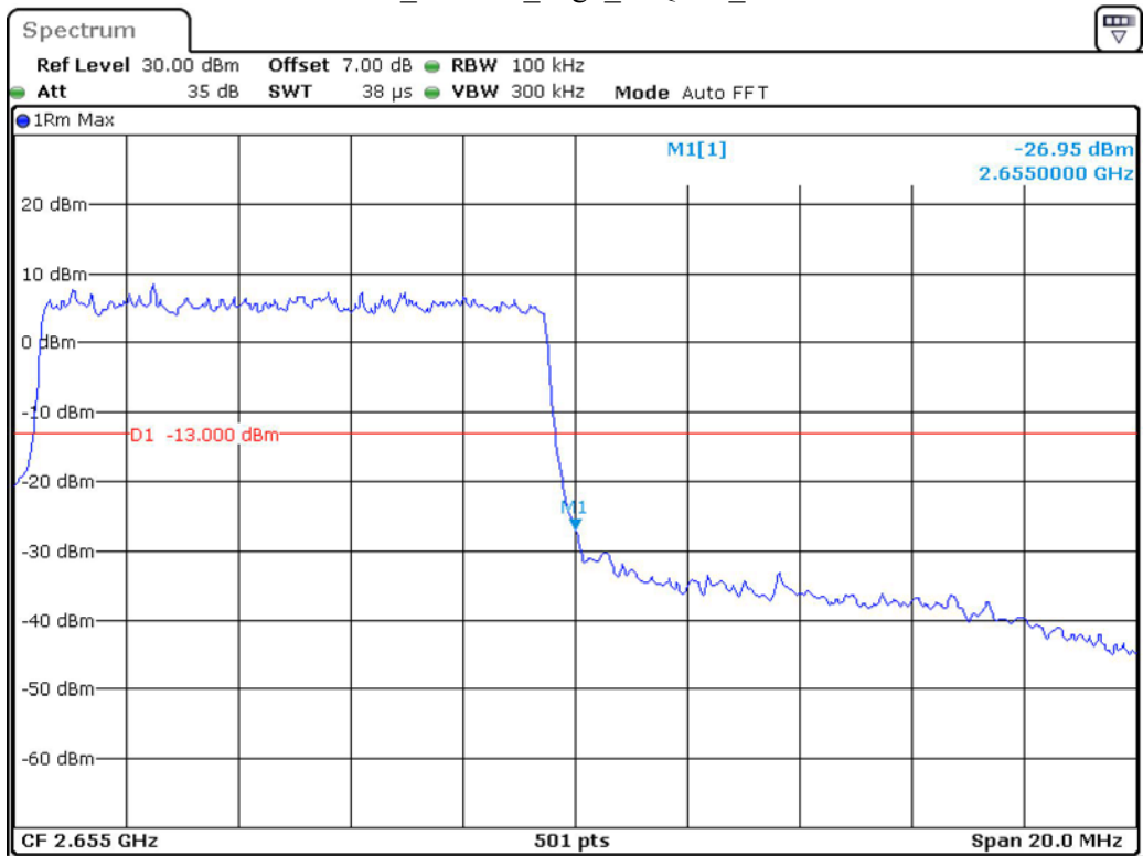
Band 41_10 MHz_High_16QAM_RB50#0
