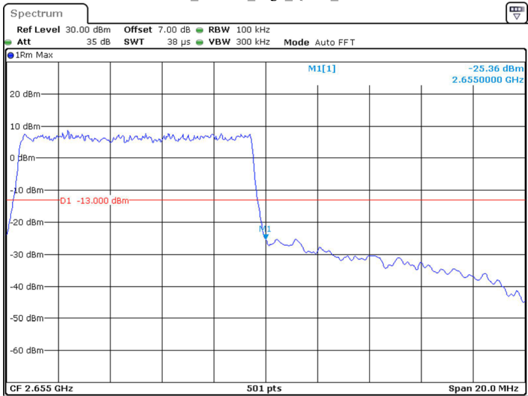
Band 41_10 MHz_High_QPSK_RB50#0
