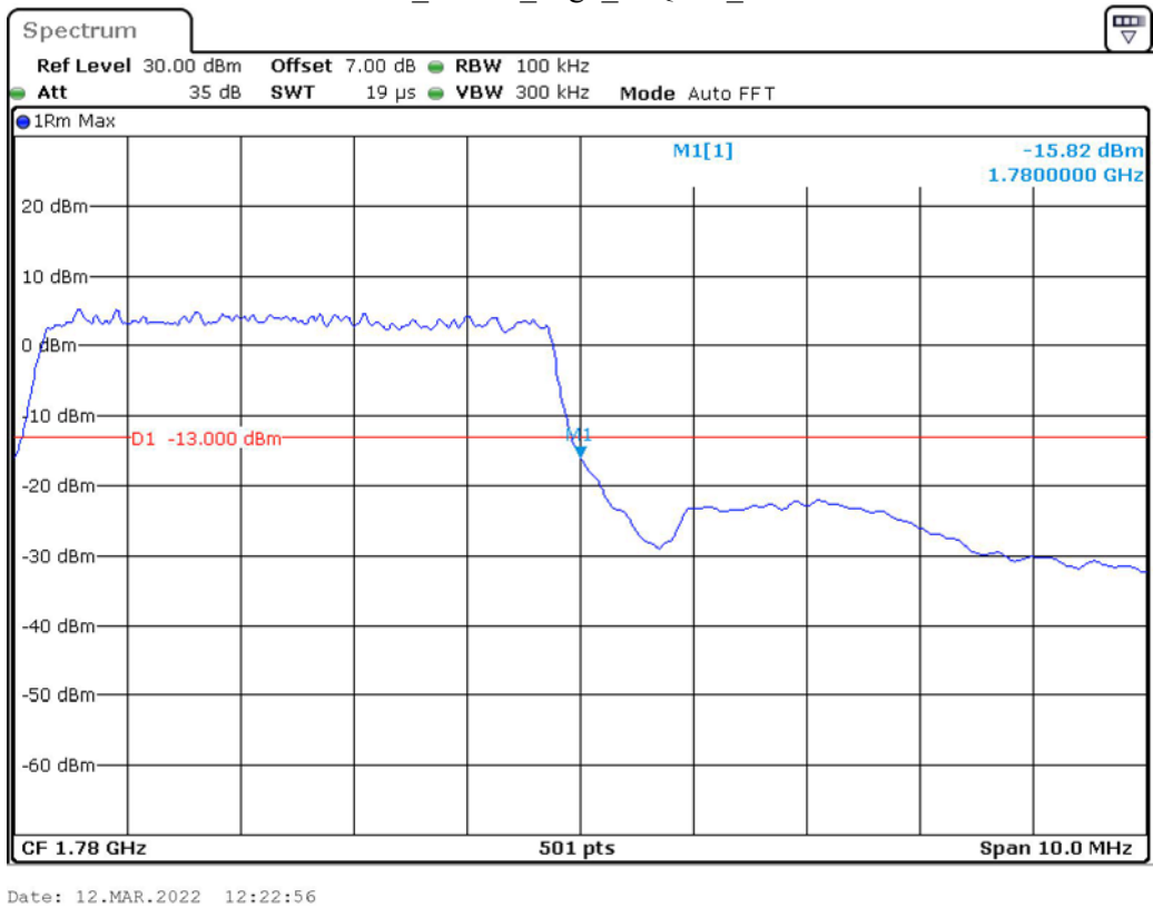
Band 66_5 MHz_High_16QAM_RB25#0
