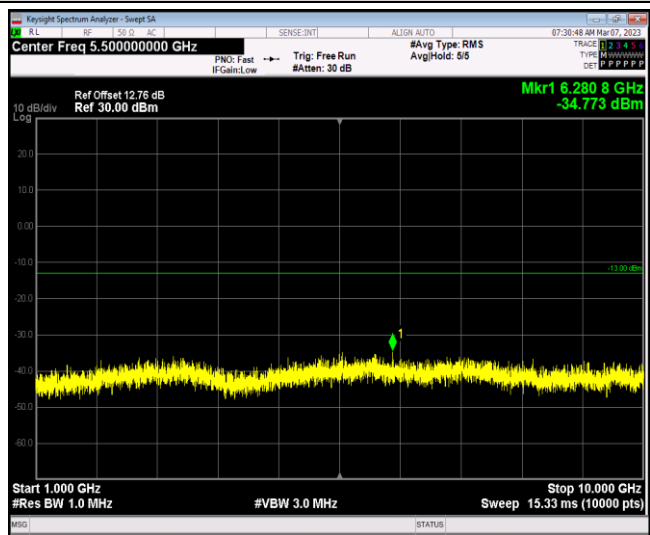
Band13-10MHz-QPSK-23230-1RB#0-Range2:1000~10000MHz
