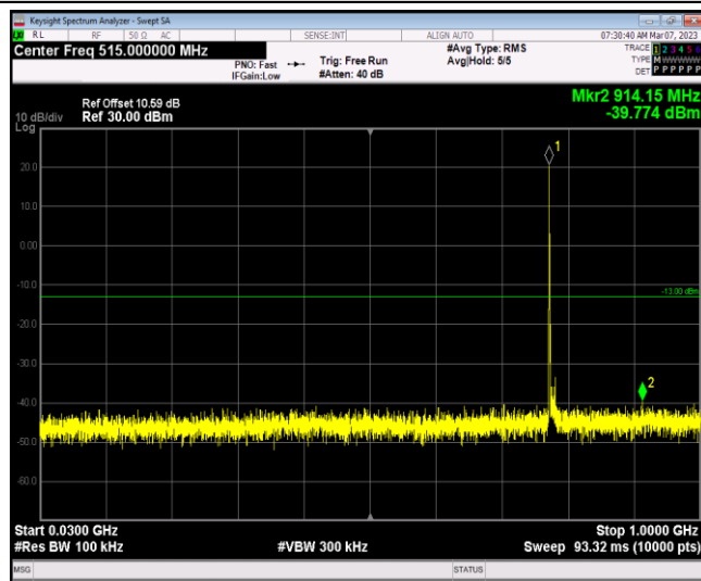
Band13-10MHz-QPSK-23230-1RB#0-Range1:30~1000MHz
