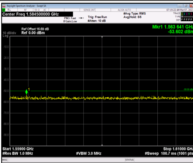
Band13-5MHz-16QAM-23230-1RB#0-Range3:1559~1610MHz
