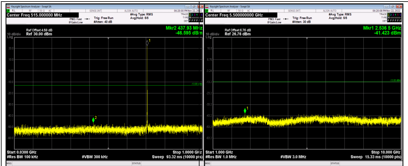
Band12-10MHz-QPSK-23060-1RB#0-Range1:30~1000MHz
