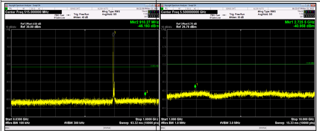
Band12-10MHz-64QAM-23060-1RB#0-Range1:30~1000MHz
