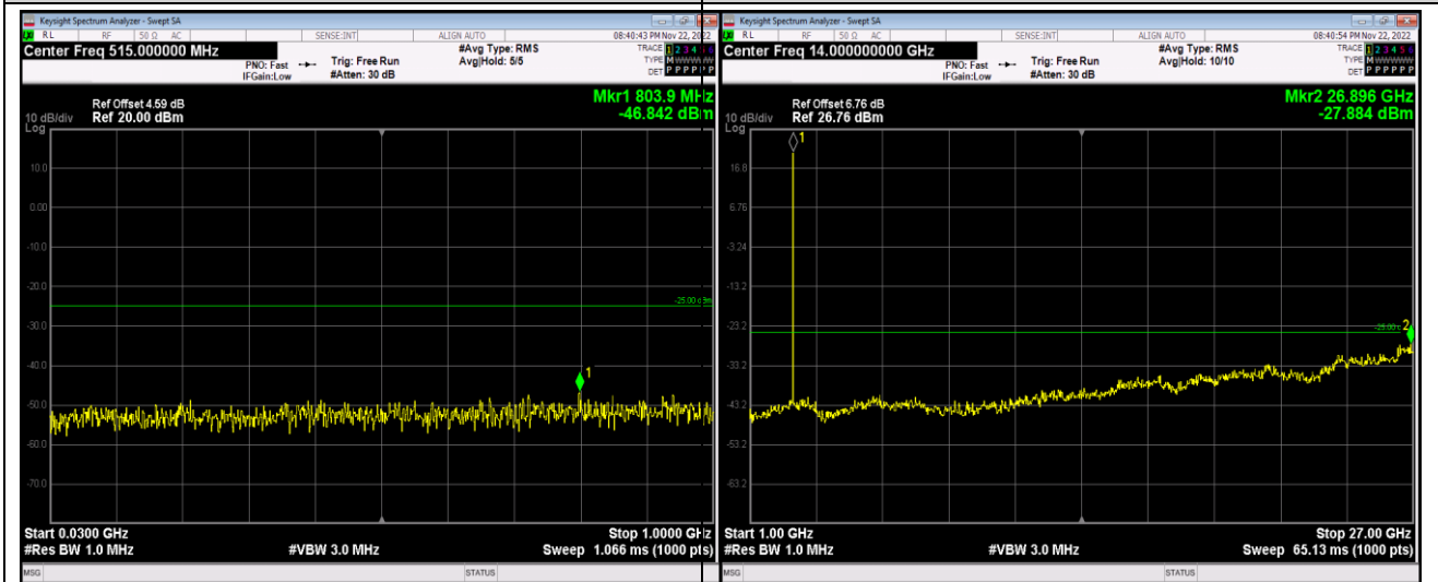
Band41-20MHz-QPSK-39750-1RB#0-Range1:30~1000MHz
