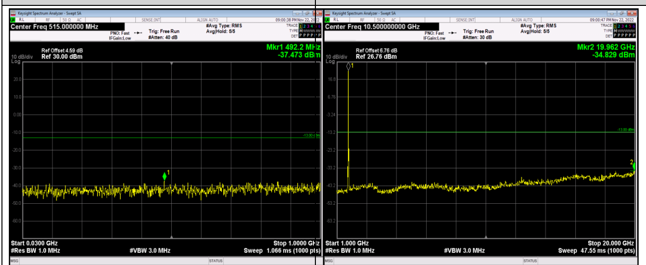
Band66-20MHz-64QAM-132322-1RB#0-Range1:3 0~1000MHz Band66-20MHz-64QAM-132322-1RB#0-Range2:1000 ~20000MHz
