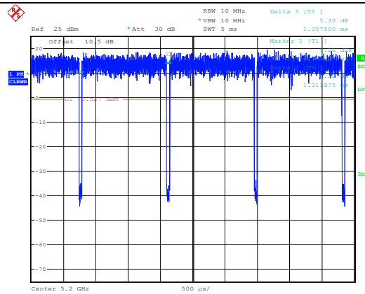
Duty Cycle
