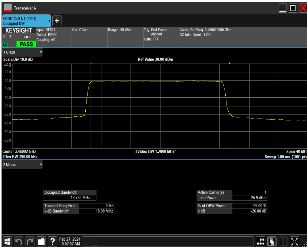
n77(3450-3550) SCS=15kHz DFT_QAM16 BW=20MHz Channel=630668 RB=100@0
