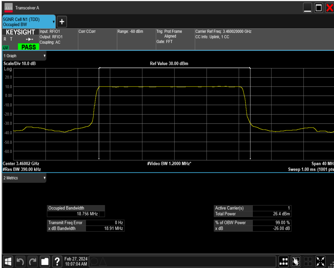
n77(3450-3550) SCS=15kHz DFT_QPSK BW=20MHz Channel=630668 RB=100@0
