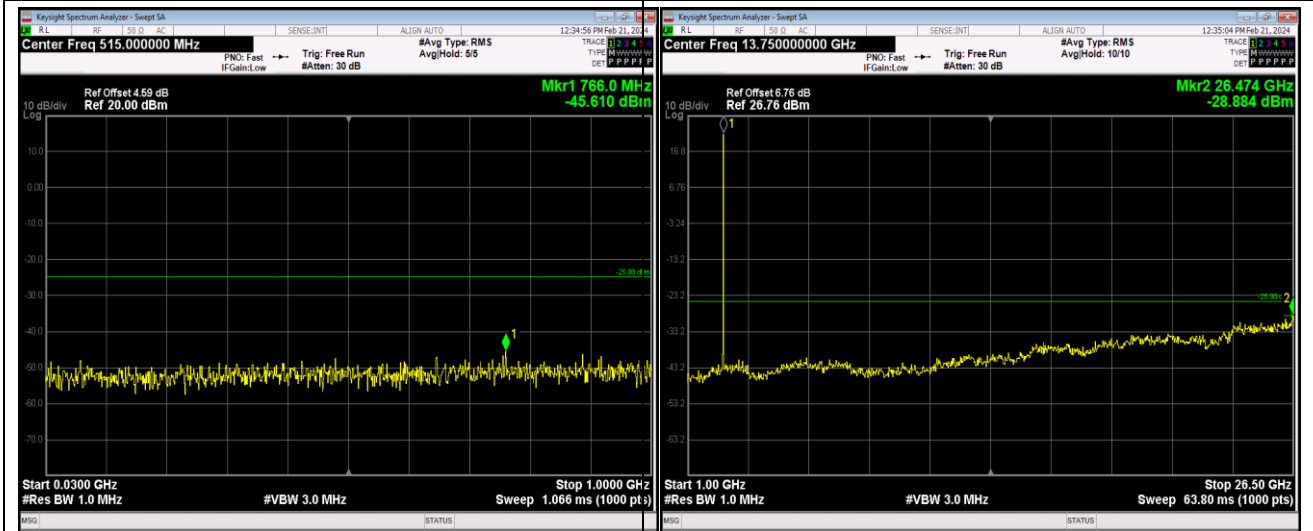
Band41-5MHz-16QAM-40620-1RB#0-Range1:30~1000MHz
