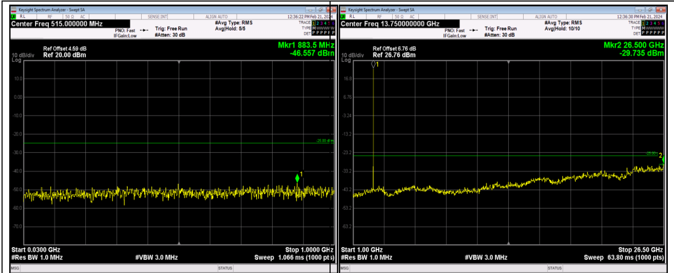
Band41-5MHz-16QAM-39675-1RB#0-Range1:30~1000MHz
