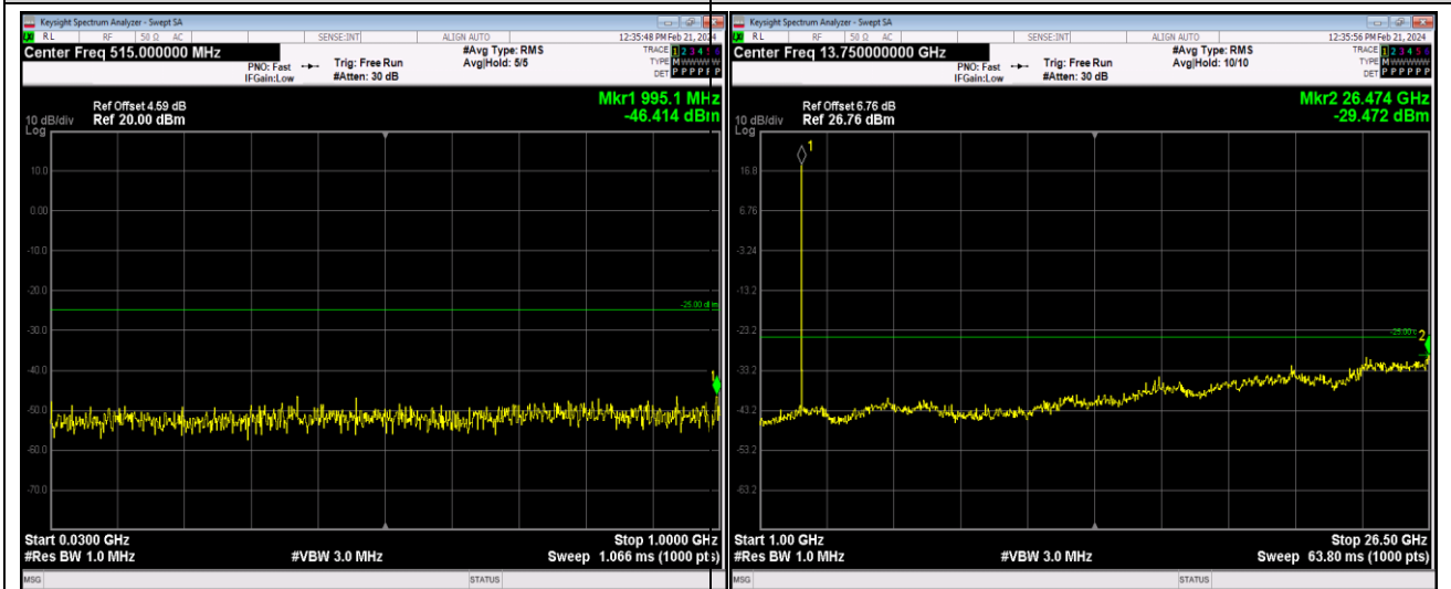
Band41-5MHz-16QAM-41565-1RB#0-Range1:30~1000MHz
