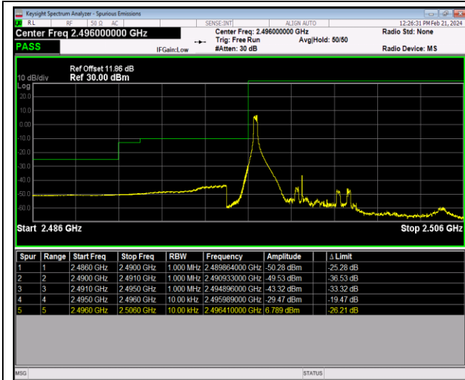
Band41-5MHz-64QAM-39675-25RB#0
