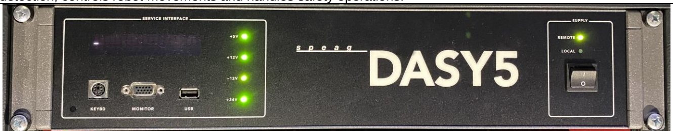
Fig. 8.5 Photo of Server for DASY5
