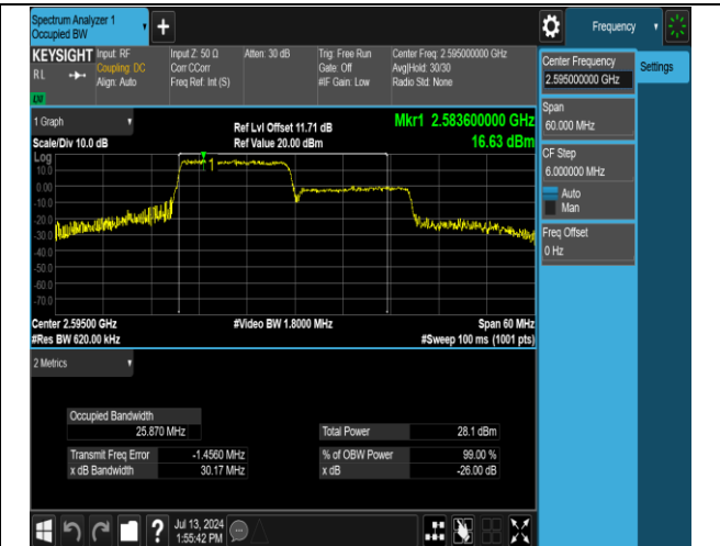
38-38-15MHz-15MHz-16QAM-16QAM-37925-38075-75RB #0-75RB#0-PASS
