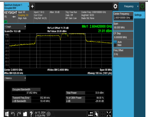
38-38-20MHz-20MHz-QPSK-QPSK-37952-38150-100RB# 0-100RB#0-PASS
