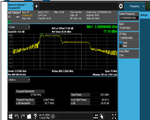
41(2555-2655)-41(2555-2655)-15MHz-20MHz-16QAM-16 QAM-40318-40489-75RB#0-100RB#0-PASS
