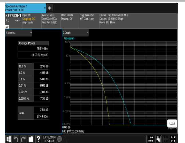
5-5-10MHz-10MHz-QPSK-QPSK-20476-20575-50RB#0-50RB#0-PASS
