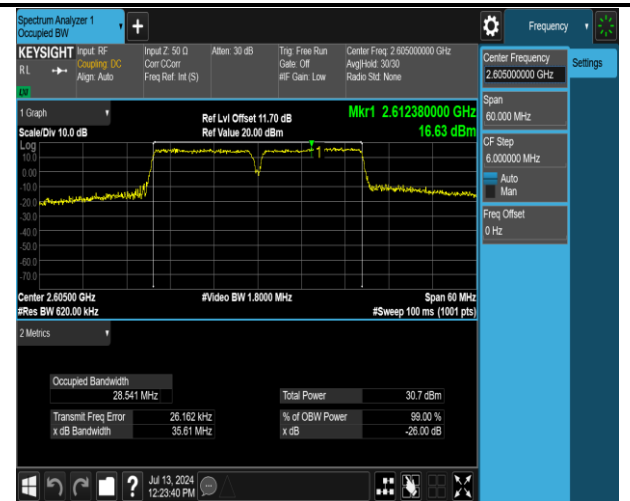
41(2555-2655)-41(2555-2655)-15MHz-15MHz-16QAM-16 QAM-40665-40815-75RB#0-75RB#0-PASS
