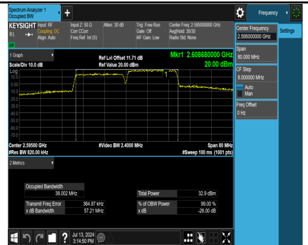
38-38-20MHz-20MHz-16QAM-16QAM-37901-38099-100R B#0-100RB#0-PASS
