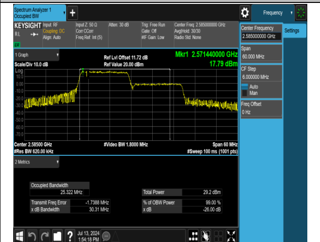
38-38-15MHz-15MHz-QPSK-QPSK-37825-37975-75RB#0 -75RB#0-PASS
