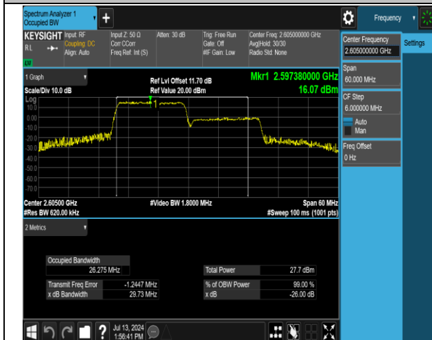
38-38-15MHz-15MHz-16QAM-16QAM-38025-38175-75RB #0-75RB#0-PASS
