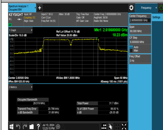
41(2555-2655)-41(2555-2655)-15MHz-15MHz-QPSK-QPS K-40665-40815-75RB#0-75RB#0-PASS
