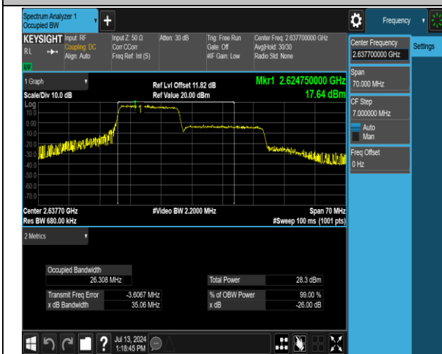
41(2555-2655)-41(2555-2655)-15MHz-20MHz-16QAM-16 QAM-40969-41140-75RB#0-100RB#0-PASS
