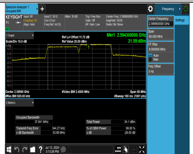
38-38-20MHz-20MHz-QPSK-QPSK-37850-38048-100RB# 0-100RB#0-PASS
