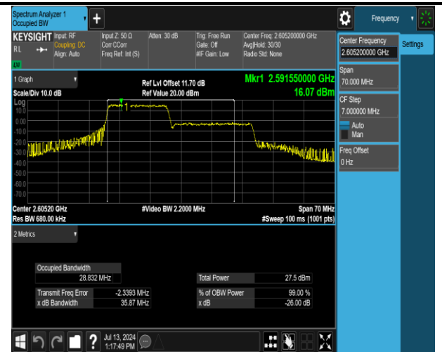
41(2555-2655)-41(2555-2655)-15MHz-20MHz-16QAM-16 QAM-40644-40815-75RB#0-100RB#0-PASS
