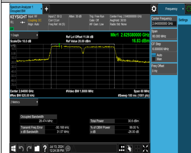
41(2555-2655)-41(2555-2655)-15MHz-15MHz-16QAM-16 QAM-41015-41165-75RB#0-75RB#0-PASS
