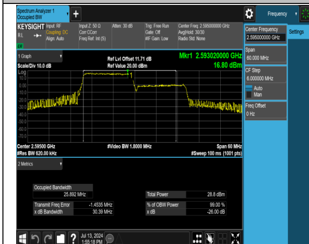
38-38-15MHz-15MHz-QPSK-QPSK-37925-38075-75RB#0 -75RB#0-PASS
