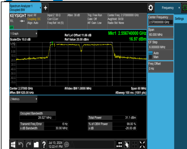
41(2555-2655)-41(2555-2655)-15MHz-15MHz-16QAM-16 QAM-40315-40465-75RB#0-75RB#0-PASS
