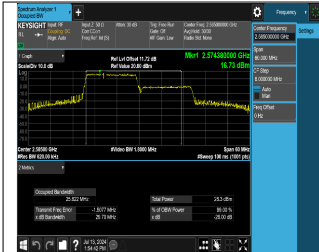
38-38-15MHz-15MHz-16QAM-16QAM-37825-37975-75RB #0-75RB#0-PASS
