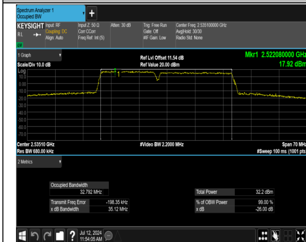
7-7-15MHz-20MHz-QPSK-QPSK-21003-21174-75RB#0-1 00RB#0-PASS
