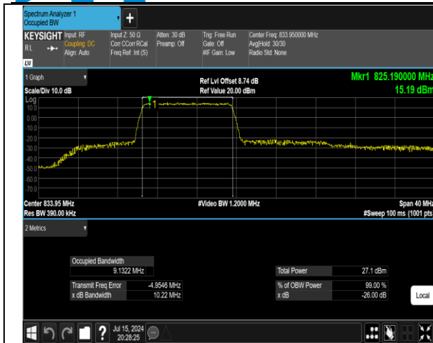
5-5-10MHz-10MHz-16QAM-16QAM-20450-20549-50RB#0 -50RB#0-PASS
