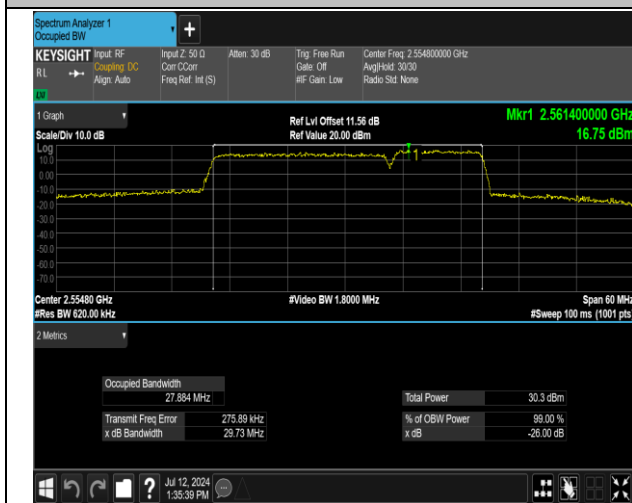
7-7-20MHz-10MHz-16QAM-16QAM-21251-21395-100RB# 0-50RB#0-PASS
