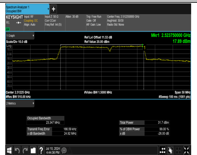
7-7-15MHz-10MHz-QPSK-QPSK-20825-20945-75RB#0-5 0RB#0-PASS
