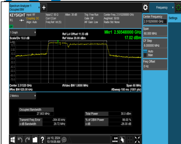
7-7-10MHz-20MHz-16QAM-16QAM-20805-20949-50RB#0 -100RB#0-PASS
