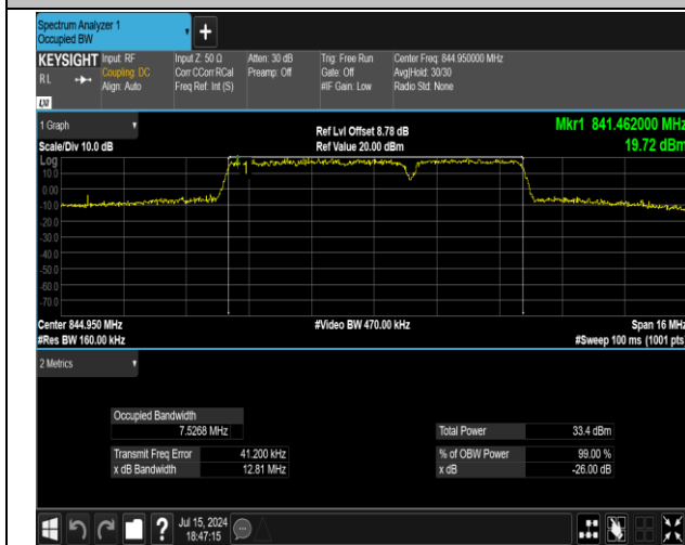
5-5-5MHz-3MHz-16QAM-16QAM-20595-20634-25RB#0-1 5RB#0-PASS
