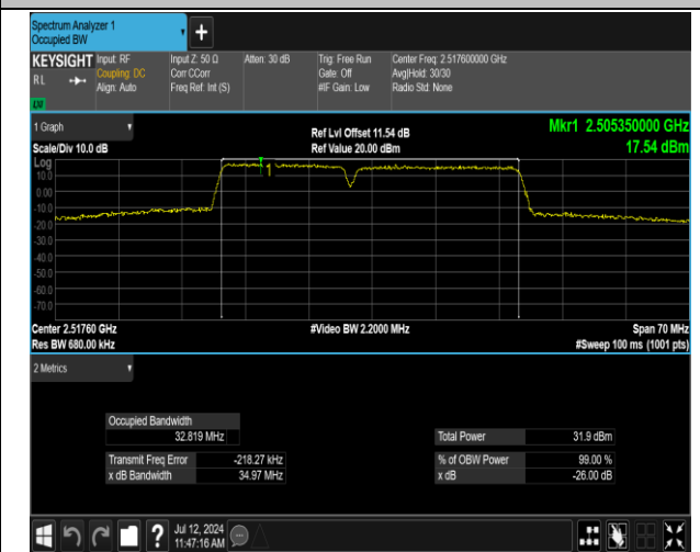
7-7-15MHz-20MHz-QPSK-QPSK-20828-20999-75RB#0-1 00RB#0-PASS
