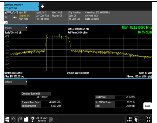
5-5-5MHz-10MHz-16QAM-16QAM-20478-20550-25RB#0-50RB#0-PASS
