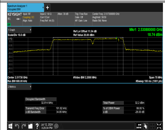
7-7-20MHz-15MHz-QPSK-QPSK-20850-21021-100RB#0- 75RB#0-PASS
