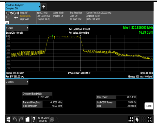
5-5-10MHz-10MHz-QPSK-QPSK-20501-20600-50RB#0-5 0RB#0-PASS
