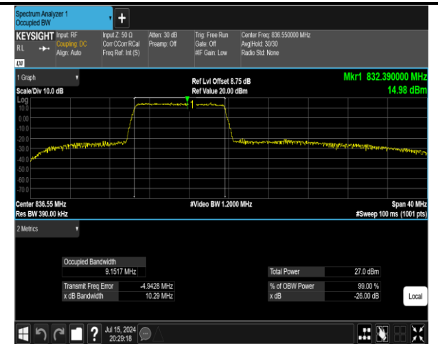
5-5-10MHz-10MHz-16QAM-16QAM-20476-20575-50RB#0 -50RB#0-PASS
