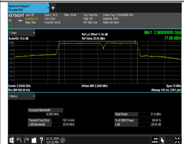
7-7-20MHz-15MHz-QPSK-QPSK-21201-21372-100RB#0- 75RB#0-PASS
