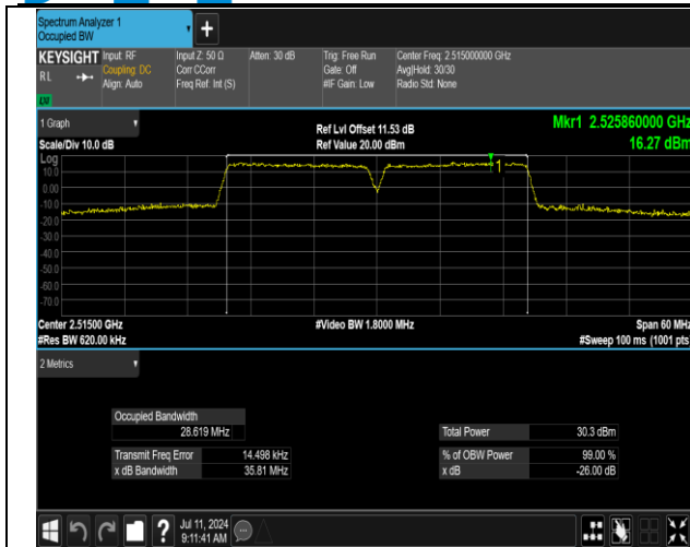
7-7-15MHz-15MHz-16QAM-16QAM-20825-20975-75RB#0 -75RB#0-PASS
