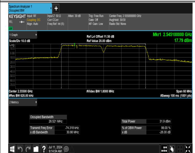
7-7-15MHz-15MHz-QPSK-QPSK-21225-21375-75RB#0-7 5RB#0-PASS
