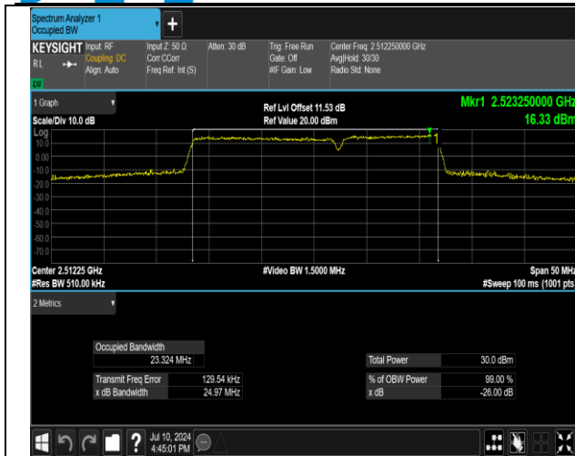
7-7-15MHz-10MHz-16QAM-16QAM-20825-20945-75RB#0 -50RB#0-PASS
