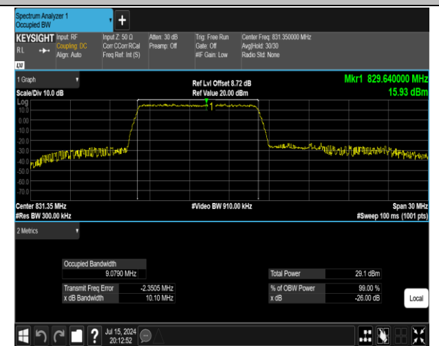
5-5-10MHz-5MHz-QPSK-QPSK-20450-20522-50RB#0-25RB#0-PASS
