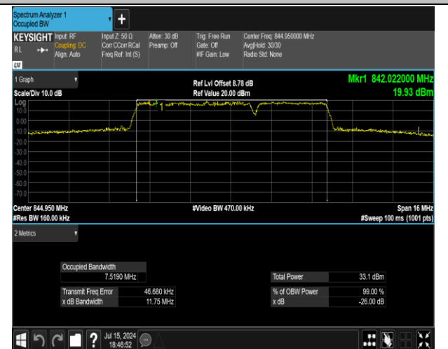
5-5-5MHz-3MHz-QPSK-QPSK-20595-20634-25RB#0-15R B#0-PASS
