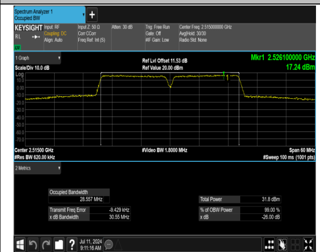
7-7-15MHz-15MHz-QPSK-QPSK-20825-20975-75RB#0-7 5RB#0-PASS
