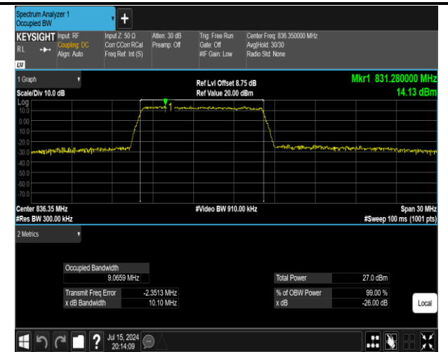
5-5-10MHz-5MHz-16QAM-16QAM-20500-20572-50RB#0-25RB#0-PASS
