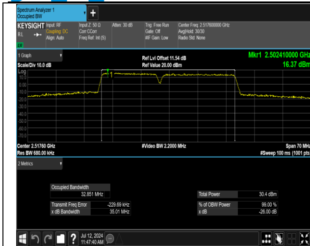
7-7-15MHz-20MHz-16QAM-16QAM-20828-20999-75RB#0 -100RB#0-PASS
