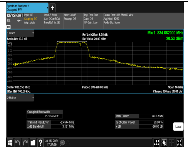
5-5-3MHz-5MHz-16QAM-16QAM-20501-20540-15RB#0-2 5RB#0-PASS
