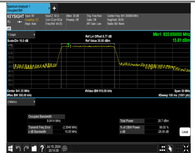
5-5-10MHz-5MHz-QPSK-QPSK-20550-20622-50RB#0-25RB#0-PASS
