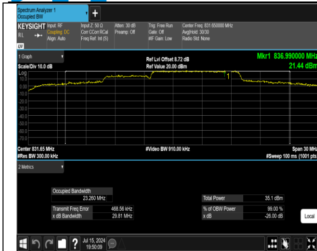
5-5-5MHz-10MHz-16QAM-16QAM-20428-20500-25RB#0-50RB#0-PASS
