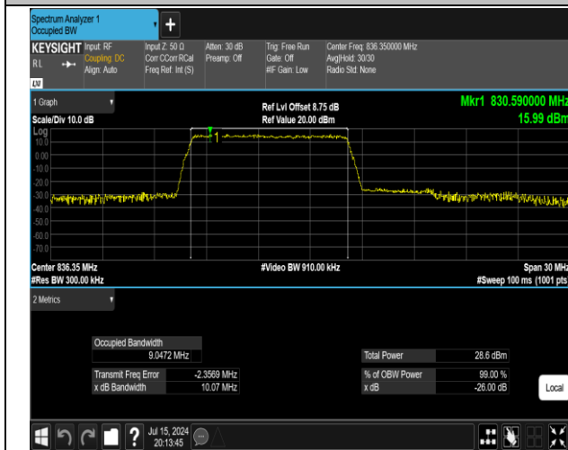
5-5-10MHz-5MHz-QPSK-QPSK-20500-20572-50RB#0-25RB#0-PASS
