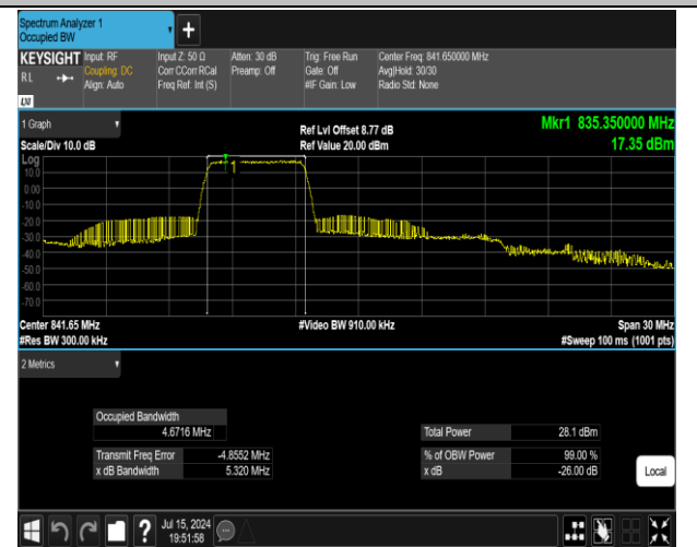
5-5-5MHz-10MHz-QPSK-QPSK-20528-20600-25RB#0-50RB#0-PASS
