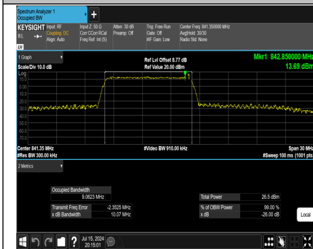
5-5-10MHz-5MHz-16QAM-16QAM-20550-20622-50RB#0-25RB#0-PASS
