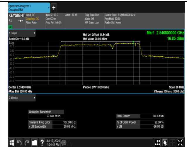
7-7-20MHz-10MHz-16QAM-16QAM-21051-21195-100RB# 0-50RB#0-PASS
