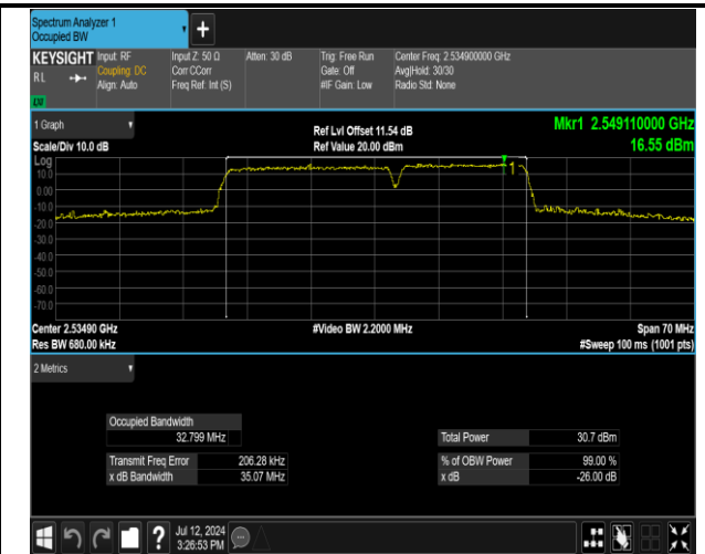
7-7-20MHz-15MHz-16QAM-16QAM-21026-21197-100RB# 0-75RB#0-PASS
