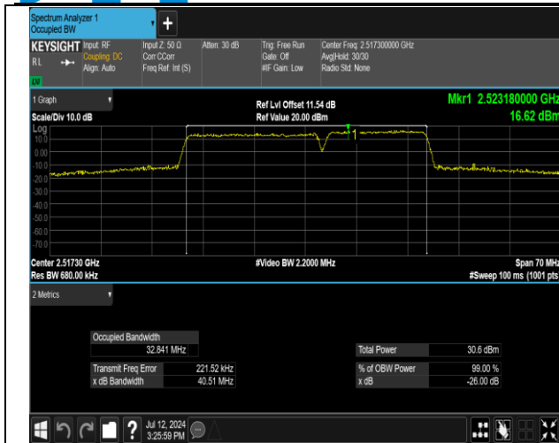
7-7-20MHz-15MHz-16QAM-16QAM-20850-21021-100RB# 0-75RB#0-PASS
