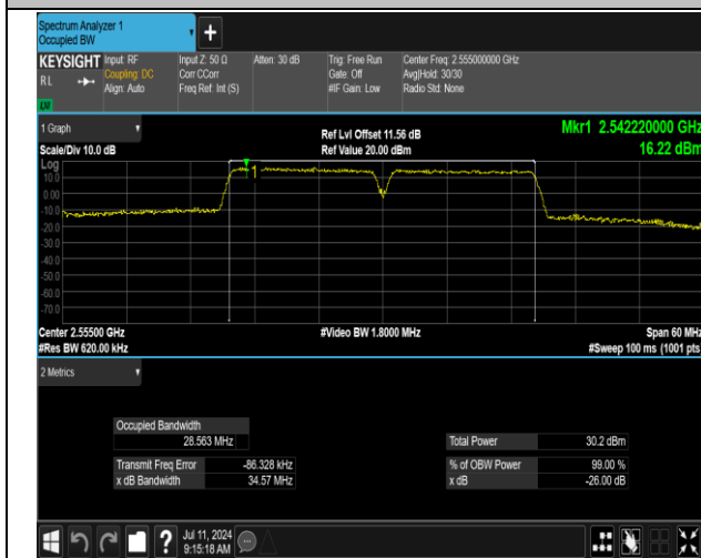
7-7-15MHz-15MHz-16QAM-16QAM-21225-21375-75RB#0 -75RB#0-PASS
