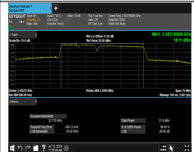
7-7-15MHz-20MHz-QPSK-QPSK-21179-21350-75RB#0-1 00RB#0-PASS
