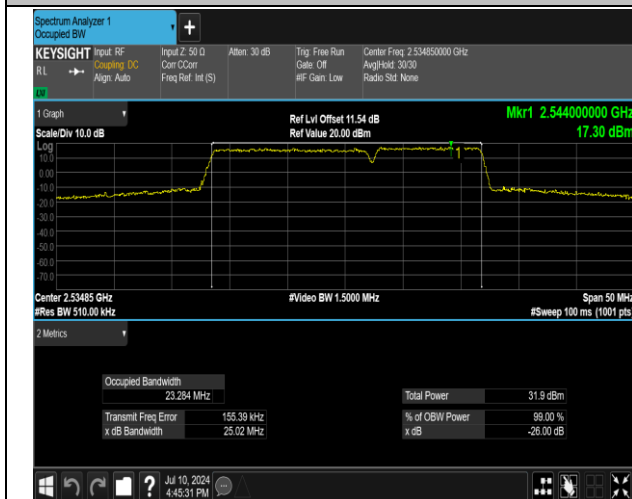
7-7-15MHz-10MHz-QPSK-QPSK-21051-21171-75RB#0-5 0RB#0-PASS
