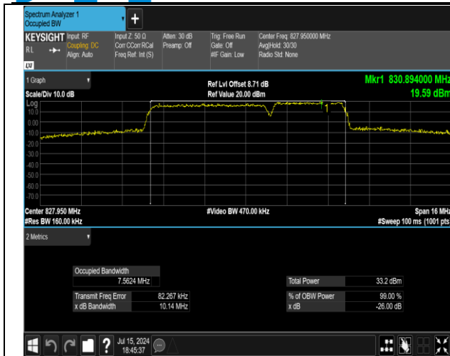
5-5-5MHz-3MHz-16QAM-16QAM-20425-20464-25RB#0-1 5RB#0-PASS
