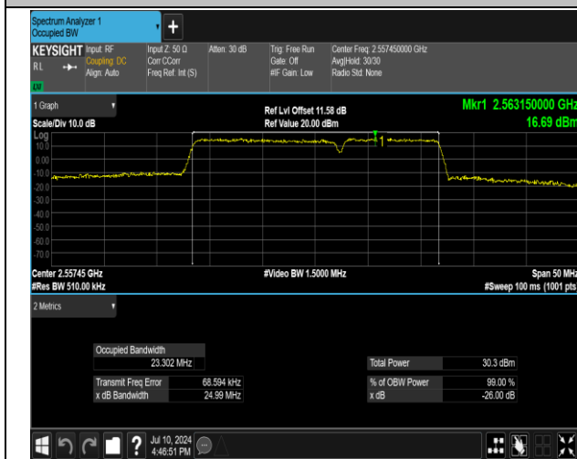
7-7-15MHz-10MHz-16QAM-16QAM-21277-21397-75RB#0 -50RB#0-PASS
