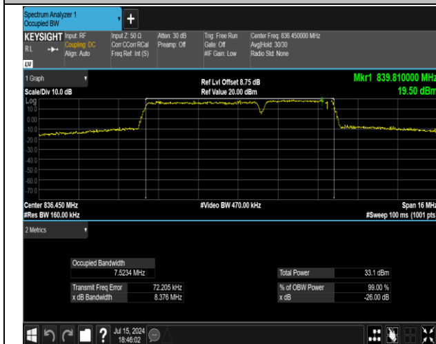
5-5-5MHz-3MHz-QPSK-QPSK-20510-20549-25RB#0-15R B#0-PASS
