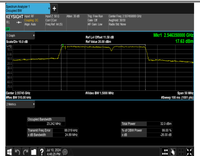
7-7-15MHz-10MHz-QPSK-QPSK-21277-21397-75RB#0-5 0RB#0-PASS
