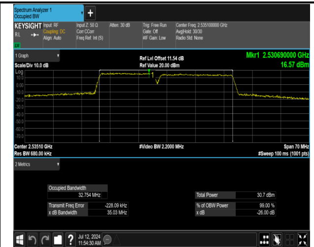
7-7-15MHz-20MHz-16QAM-16QAM-21003-21174-75RB#0 -100RB#0-PASS
