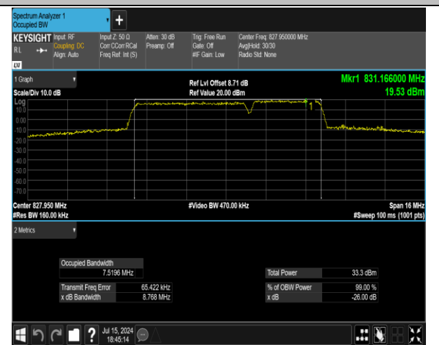
5-5-5MHz-3MHz-QPSK-QPSK-20425-20464-25RB#0-15R B#0-PASS
