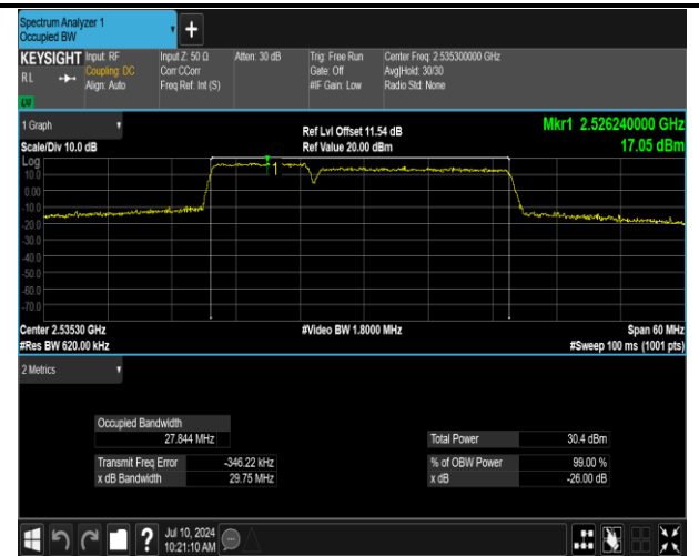
7-7-10MHz-20MHz-16QAM-16QAM-21006-21150-50RB#0 -100RB#0-PASS
