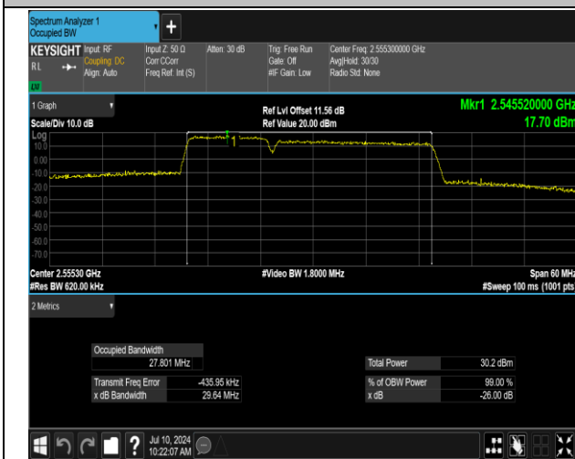
7-7-10MHz-20MHz-16QAM-16QAM-21206-21350-50RB#0 -100RB#0-PASS
