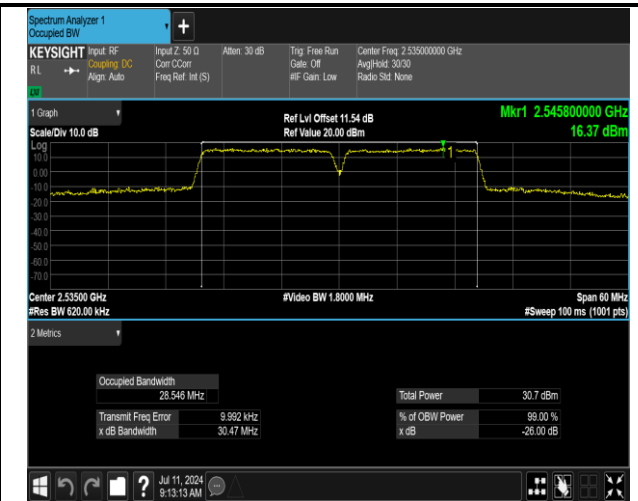
7-7-15MHz-15MHz-16QAM-16QAM-21025-21175-75RB#0 -75RB#0-PASS
