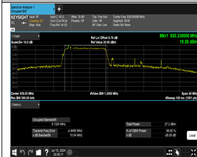
5-5-10MHz-10MHz-16QAM-16QAM-20501-20600-50RB#0 -50RB#0-PASS
