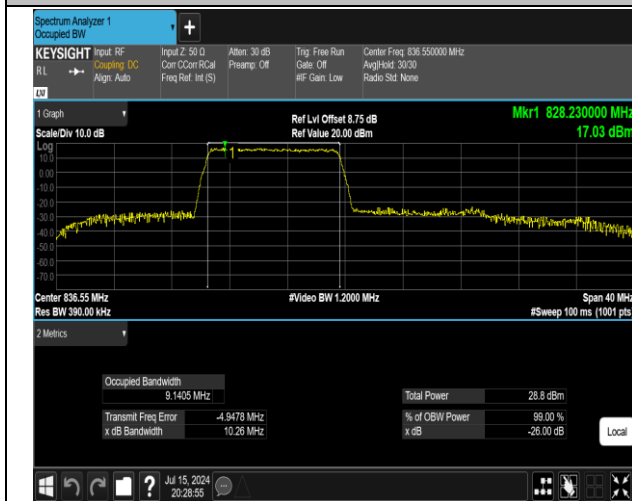
5-5-10MHz-10MHz-QPSK-QPSK-20476-20575-50RB#0-5 0RB#0-PASS
