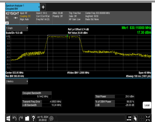
5-5-10MHz-10MHz-QPSK-QPSK-20450-20549-50RB#0-5 0RB#0-PASS
