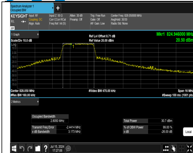
5-5-3MHz-5MHz-16QAM-16QAM-20416-20455-15RB#0-2 5RB#0-PASS
