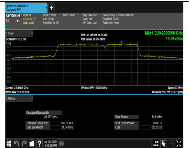
7-7-15MHz-10MHz-16QAM-16QAM-21051-21171-75RB#0 -50RB#0-PASS
