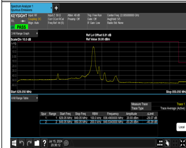
5-5-10MHz-10MHz-QPSK@QPSK-QPSK@QPSK-20501-2 0600-1RB#49@50RB#0-0RB#0@50RB#0-PASS
