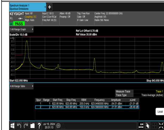
5-5-10MHz-10MHz-QPSK@QPSK-QPSK@QPSK-20450-2 0549-1RB#0@50RB#0-0RB#0@50RB#0-PASS
