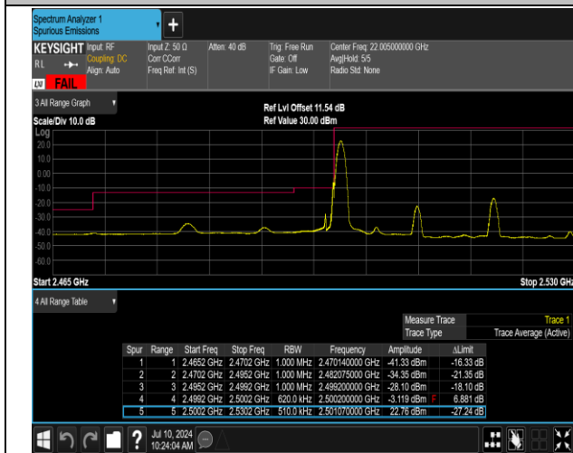
7-7-10MHz-20MHz-16QAM@16QAM-16QAM@16QAM-20 805-20949-1RB#0@50RB#0-0RB#0@100RB#0
