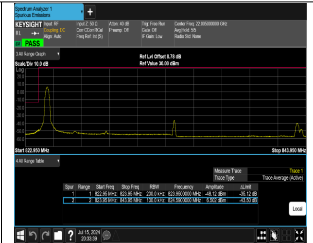
5-5-10MHz-10MHz-16QAM@16QAM-16QAM@16QAM-2 0450-20549-1RB#0@50RB#0-1RB#49@50RB#0-PASS
