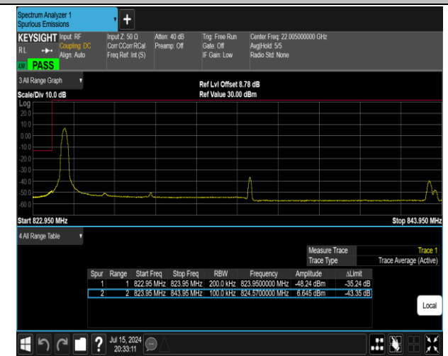
5-5-10MHz-10MHz-QPSK@QPSK-QPSK@QPSK-20450- 20549-1RB#0@50RB#0-1RB#49@50RB#0-PASS
