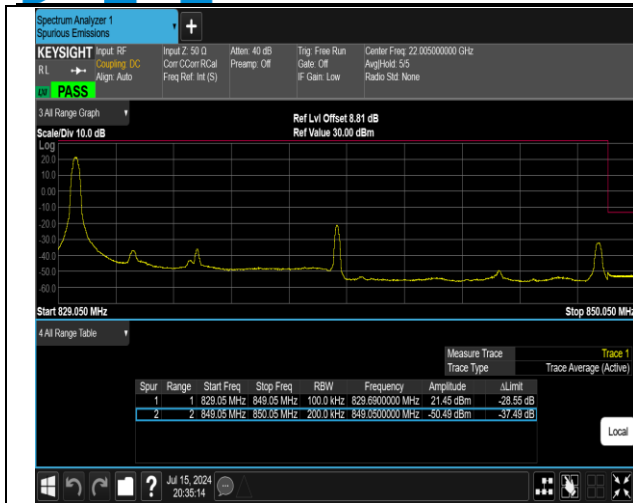
5-5-10MHz-10MHz-QPSK@QPSK-QPSK@QPSK-20501-2 0600-1RB#0@50RB#0-0RB#0@50RB#0-PASS
