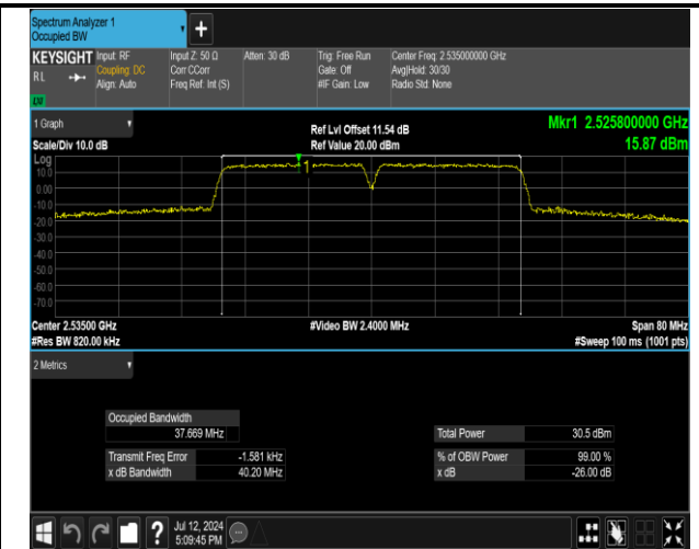
7-7-20MHz-20MHz-16QAM-16QAM-21001-21199-100RB# 0-100RB#0-PASS
