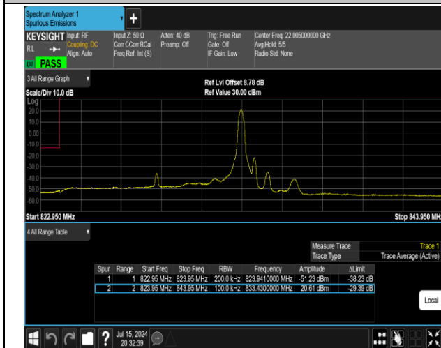
5-5-10MHz-10MHz-16QAM@16QAM-16QAM@16QAM-20 450-20549-1RB#49@50RB#0-0RB#0@50RB#0-PASS
