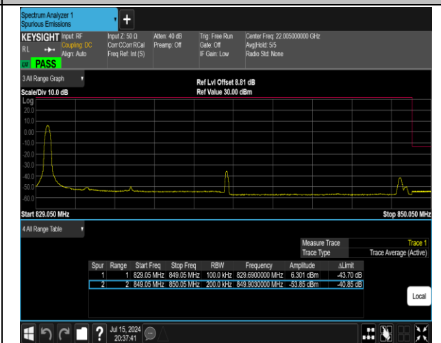
5-5-10MHz-10MHz-16QAM@16QAM-16QAM@16QAM-2 0501-20600-1RB#0@50RB#0-1RB#49@50RB#0-PASS
