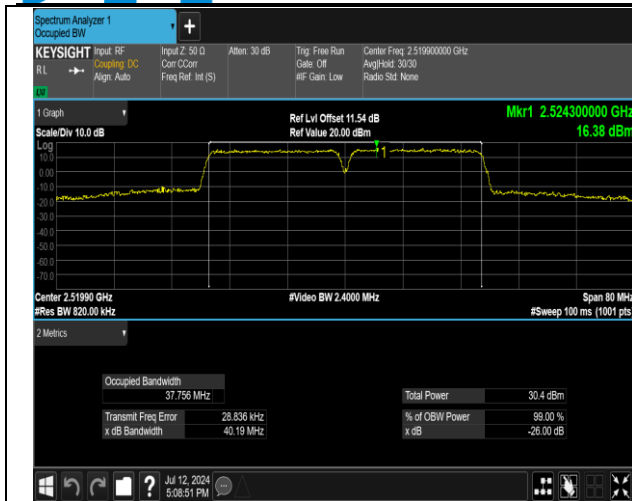
7-7-20MHz-20MHz-16QAM-16QAM-20850-21048-100RB# 0-100RB#0-PASS
