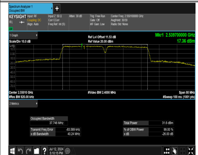
7-7-20MHz-20MHz-QPSK-QPSK-21152-21350-100RB#0- 100RB#0-PASS
