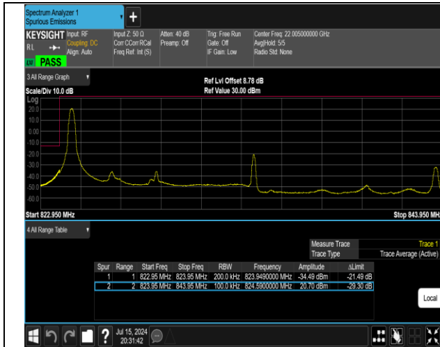
5-5-10MHz-10MHz-16QAM@16QAM-16QAM@16QAM-20 450-20549-1RB#0@50RB#0-0RB#0@50RB#0-PASS
