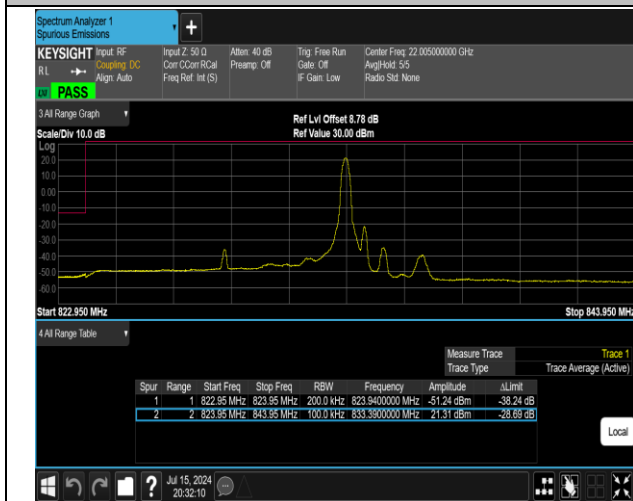
5-5-10MHz-10MHz-QPSK@QPSK-QPSK@QPSK-20450-2 0549-1RB#49@50RB#0-0RB#0@50RB#0-PASS
