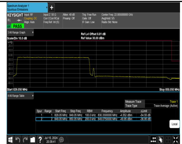
5-5-10MHz-10MHz-16QAM@16QAM-16QAM@16QAM-2 0501-20600-50RB#0@50RB#0-50RB#0@50RB#0-PASS
