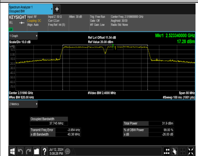
7-7-20MHz-20MHz-QPSK-QPSK-20850-21048-100RB#0- 100RB#0-PASS
