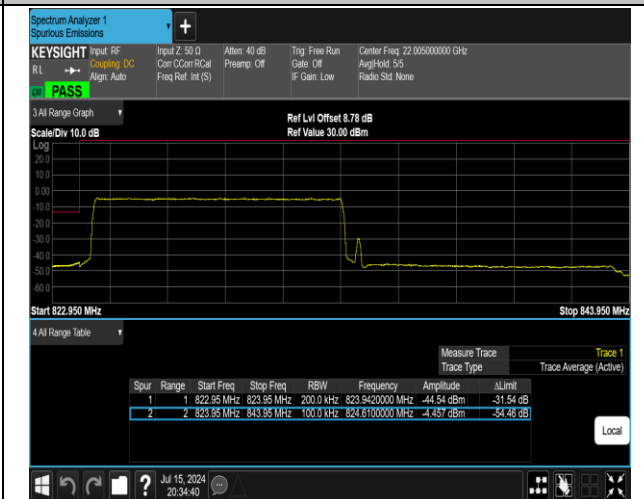
5-5-10MHz-10MHz-16QAM@16QAM-16QAM@16QAM-2 0450-20549-50RB#0@50RB#0-50RB#0@50RB#0-PASS
