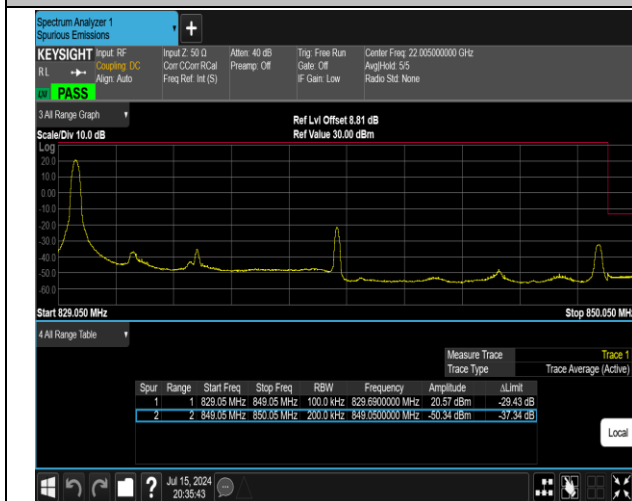
5-5-10MHz-10MHz-16QAM@16QAM-16QAM@16QAM-20 501-20600-1RB#0@50RB#0-0RB#0@50RB#0-PASS
