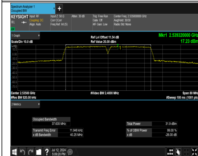
7-7-20MHz-20MHz-QPSK-QPSK-21001-21199-100RB#0- 100RB#0-PASS
