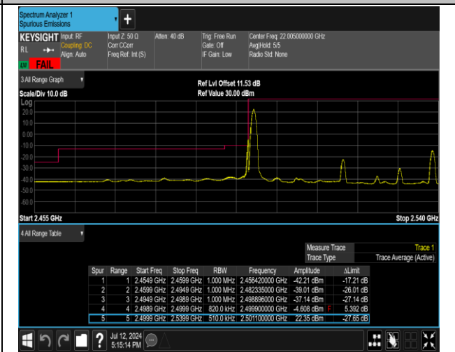
7-7-20MHz-20MHz-16QAM@16QAM-16QAM@16QAM-2 0850-21048-1RB#0@100RB#0-0RB#0@100RB#0-FAIL
