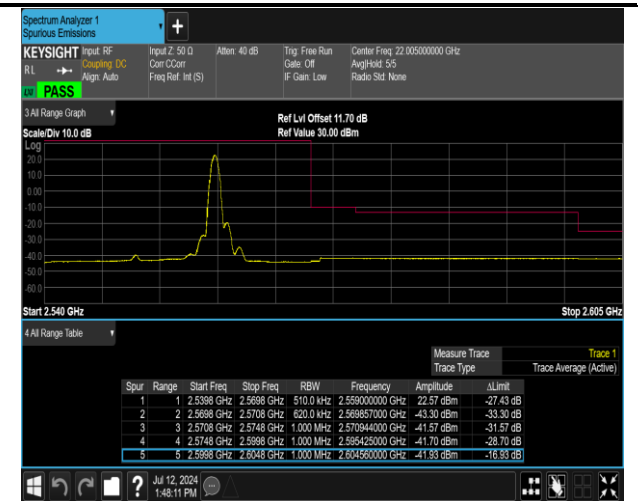
7-7-20MHz-10MHz-16QAM@16QAM-16QAM@16QAM-21251-21395-1RB#99@100RB#0-0RB#0@50RB#0-PASS
