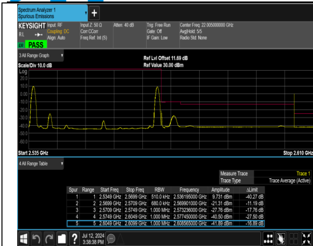
7-7-20MHz-15MHz-QPSK@QPSK-QPSK@QPSK-21201-2 1372-1RB#0@100RB#0-1RB#74@75RB#0-PASS
