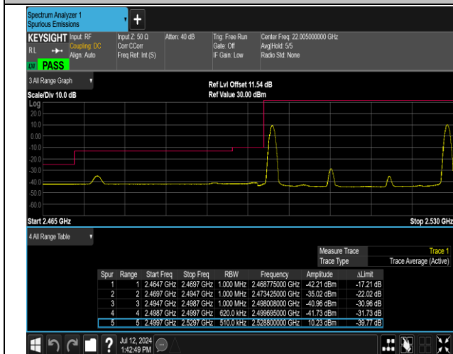
7-7-20MHz-10MHz-QPSK@QPSK-QPSK@QPSK-20850-20994-1RB#0@100RB#0-1RB#49@50RB#0-PASS
