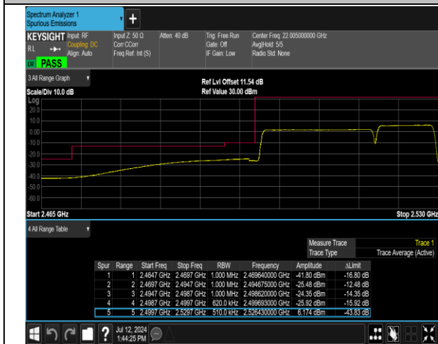
7-7-20MHz-10MHz-QPSK@QPSK-QPSK@QPSK-20850-20994-100RB#0@100RB#0-50RB#0@50RB#0-PASS
