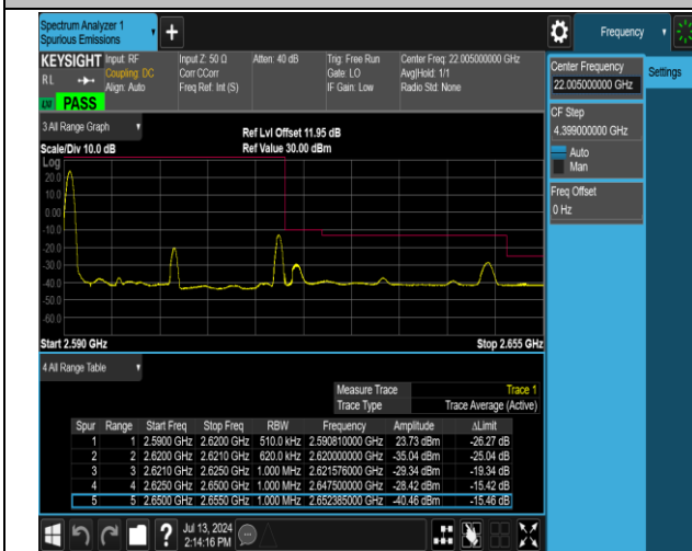
38-38-15MHz-15MHz-QPSK@QPSK-QPSK@QPSK-38025 -38175-1RB#0@75RB#0-0RB#0@75RB#0-PASS
