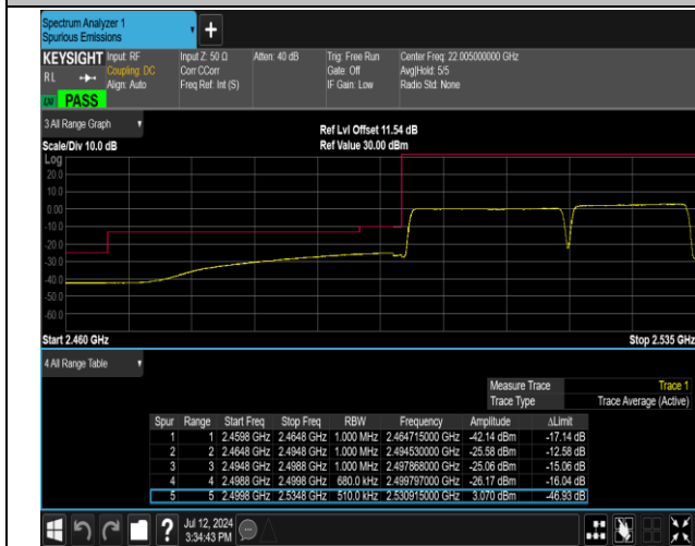
7-7-20MHz-15MHz-16QAM@16QAM-16QAM@16QAM-20850-21021-100RB#0@100RB#0-75RB#0@75RB#0-PASS
