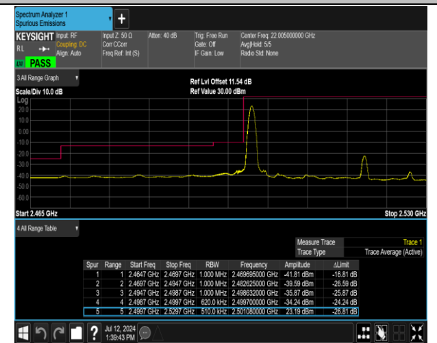
7-7-20MHz-10MHz-QPSK@QPSK-QPSK@QPSK-20850-20994-1RB#0@100RB#0-0RB#0@50RB#0-PASS
