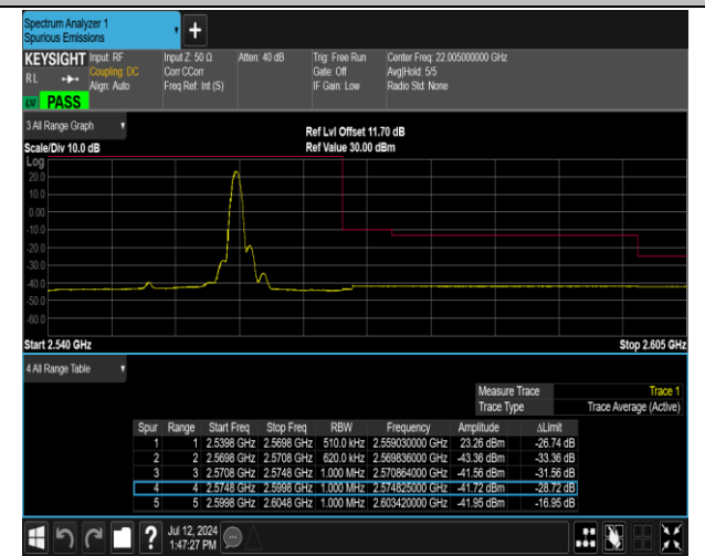
7-7-20MHz-10MHz-QPSK@QPSK-QPSK@QPSK-21251-21395-1RB#99@100RB#0-0RB#0@50RB#0-PASS
