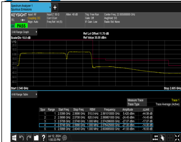
7-7-20MHz-10MHz-QPSK@QPSK-QPSK@QPSK-21251-2 1395-100RB#0@100RB#0-50RB#0@50RB#0-PASS
