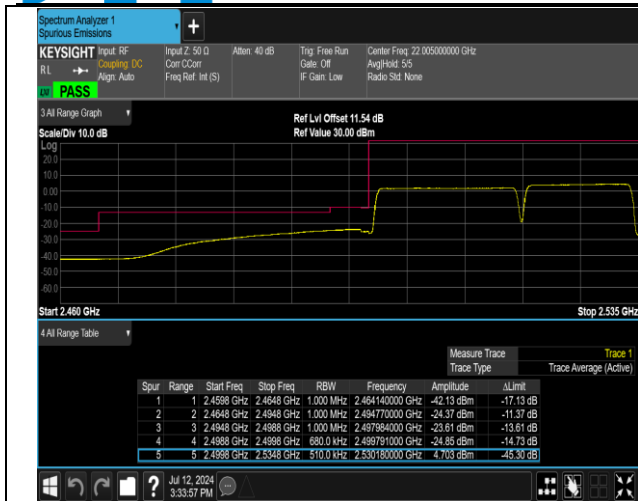
7-7-20MHz-15MHz-QPSK@QPSK-QPSK@QPSK-20850-2 1021-100RB#0@100RB#0-75RB#0@75RB#0-PASS
