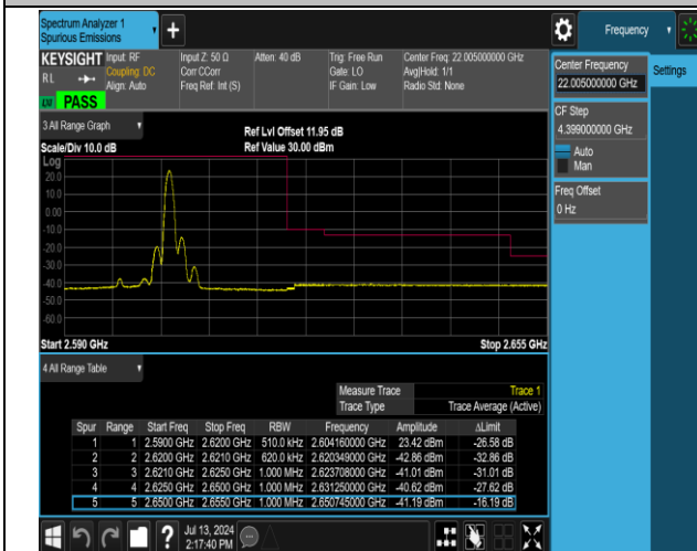
38-38-15MHz-15MHz-QPSK@QPSK-QPSK@QPSK-38025 -38175-1RB#74@75RB#0-0RB#0@75RB#0-PASS
