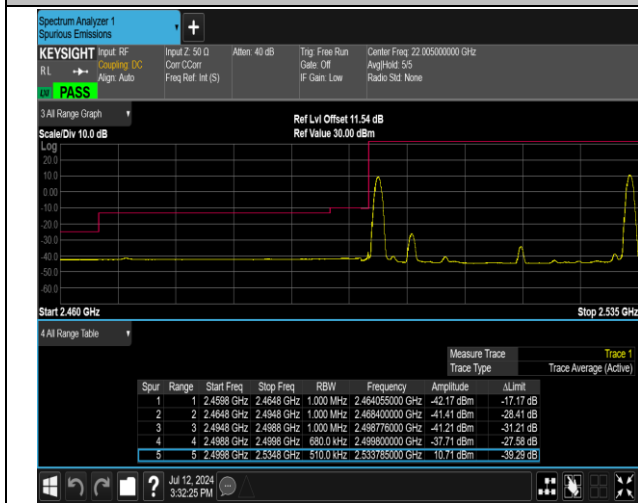
7-7-20MHz-15MHz-QPSK@QPSK-QPSK@QPSK-20850-21021-1RB#0@100RB#0-1RB#74@75RB#0-PASS
