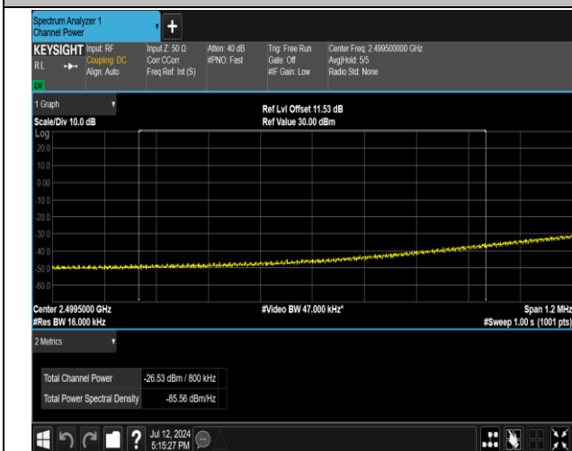
7-7-20MHz-20MHz-16QAM@16QAM-16QAM@16QAM-20 850-21048-1RB#0@100RB#0-0RB#0@100RB#0-PASS_Fi
