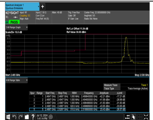
7-7-20MHz-10MHz-QPSK@QPSK-QPSK@QPSK-20850-20994-1RB#99@100RB#0-0RB#0@50RB#0-PASS
