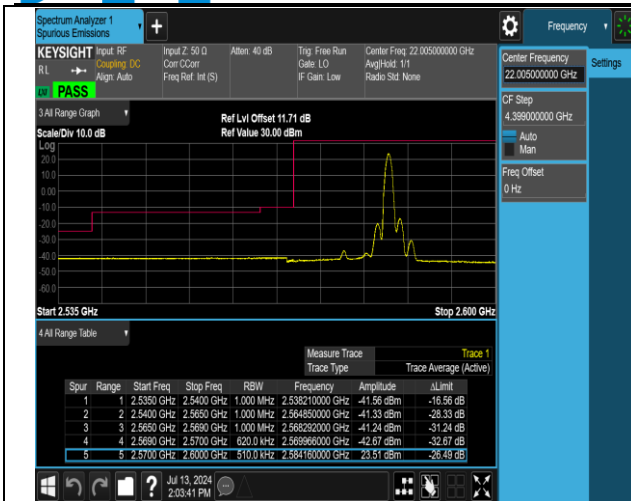
38-38-15MHz-15MHz-QPSK@QPSK-QPSK@QPSK-37825 -37975-1RB#74@75RB#0-0RB#0@75RB#0-PASS
