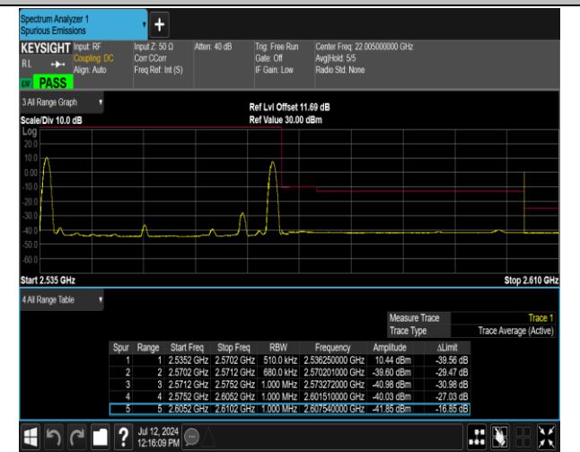
7-7-15MHz-20MHz-QPSK@QPSK-QPSK@QPSK-21179-2 21350-1RB#0@75RB#0-1RB#99@100RB#0-PASS
