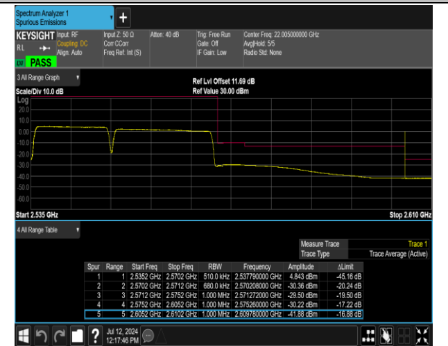
7-7-15MHz-20MHz-QPSK@QPSK-QPSK@QPSK-21179-2 21350-75RB#0@75RB#0-100RB#0@100RB#0-PASS
