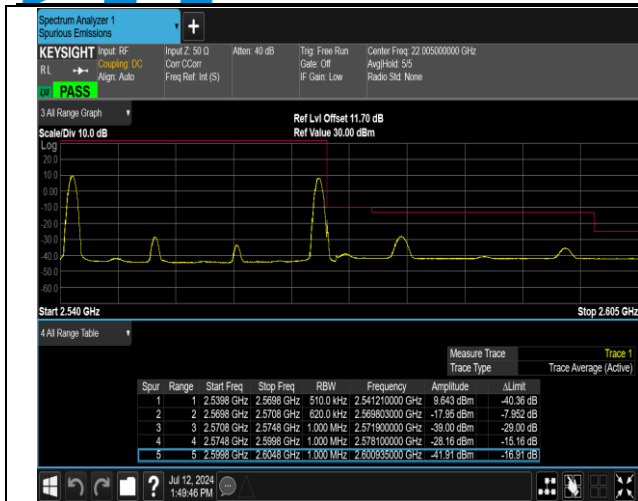
7-7-20MHz-10MHz-16QAM@16QAM-16QAM@16QAM-21251-21395-1RB#0@100RB#0-1RB#49@50RB#0-PASS
