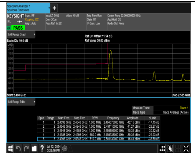
7-7-20MHz-15MHz-QPSK@QPSK-QPSK@QPSK-20850-21021-1RB#0@100RB#0-0RB#0@75RB#0-PASS
