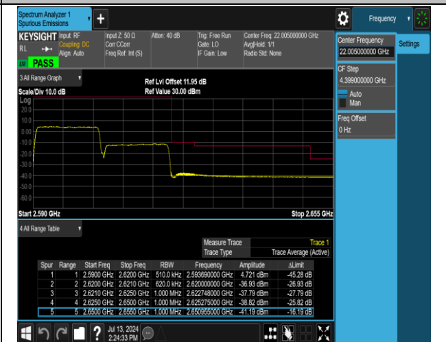
38-38-15MHz-15MHz-QPSK@QPSK-QPSK@QPSK-380 25-38175-75RB#0@75RB#0-75RB#0@75RB#0-PASS
