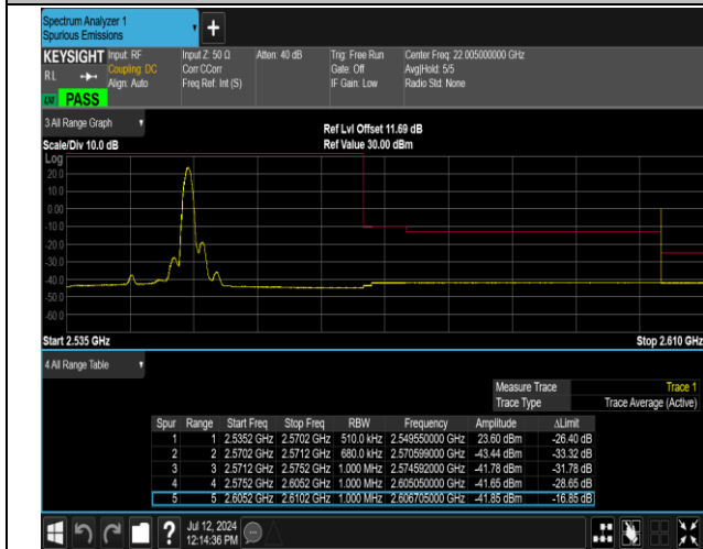
7-7-15MHz-20MHz-QPSK@QPSK-QPSK@QPSK-21179-2 1350-1RB#74@75RB#0-0RB#0@100RB#0-PASS
