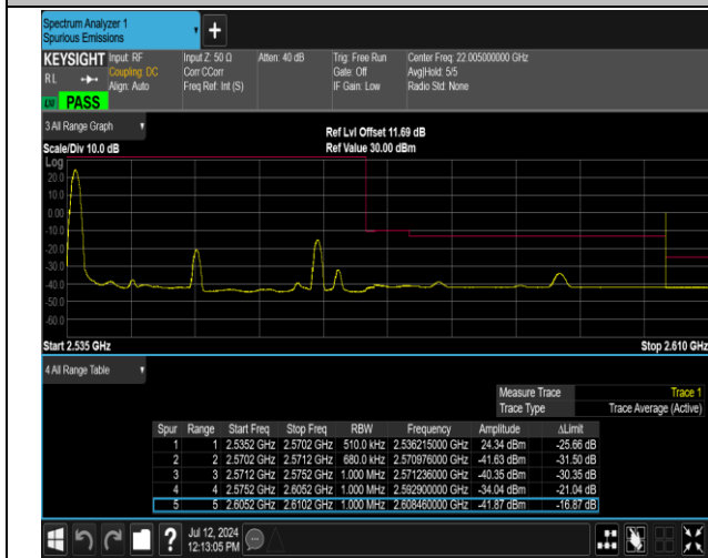
7-7-15MHz-20MHz-QPSK@QPSK-QPSK@QPSK-21179-2 1350-1RB#0@75RB#0-0RB#0@100RB#0-PASS
