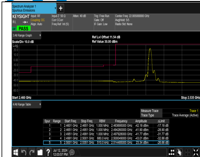
7-7-15MHz-20MHz-QPSK@QPSK-QPSK@QPSK-20828-2 0999-1RB#74@75RB#0-0RB#0@100RB#0-PASS
