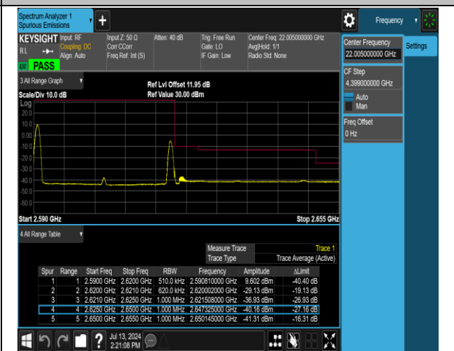
38-38-15MHz-15MHz-QPSK@QPSK-QPSK@QPSK-380 25-38175-1RB#0@75RB#0-1RB#74@75RB#0-PASS
