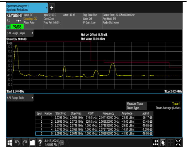
7-7-20MHz-10MHz-QPSK@QPSK-QPSK@QPSK-21251-21395-1RB#0@100RB#0-0RB#0@50RB#0-PASS
