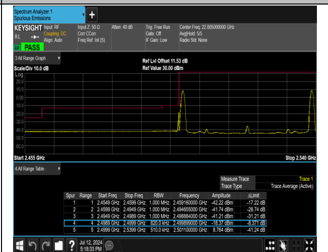
7-7-20MHz-20MHz-16QAM@16QAM-16QAM@16QAM-2 0850-21048-1RB#0@100RB#0-1RB#99@100RB#0-PAS
