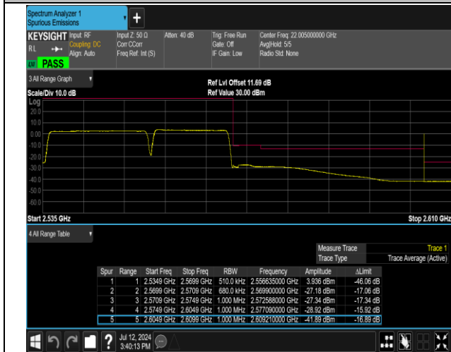
7-7-20MHz-15MHz-QPSK@QPSK-QPSK@QPSK-21201-21372-100RB#0@100RB#0-75RB#0@75RB#0-PASS
