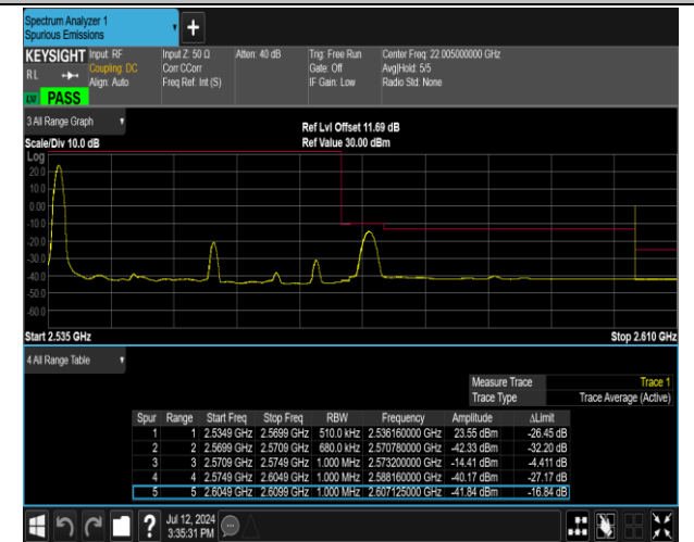
7-7-20MHz-15MHz-QPSK@QPSK-QPSK@QPSK-21201-21372-1RB#0@100RB#0-0RB#0@75RB#0-PASS
