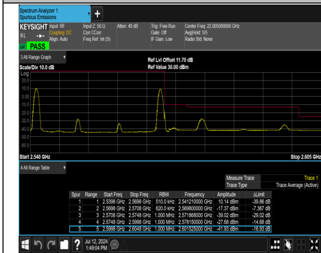
7-7-20MHz-10MHz-QPSK@QPSK-QPSK@QPSK-21251-2 1395-1RB#0@100RB#0-1RB#49@50RB#0-PASS
