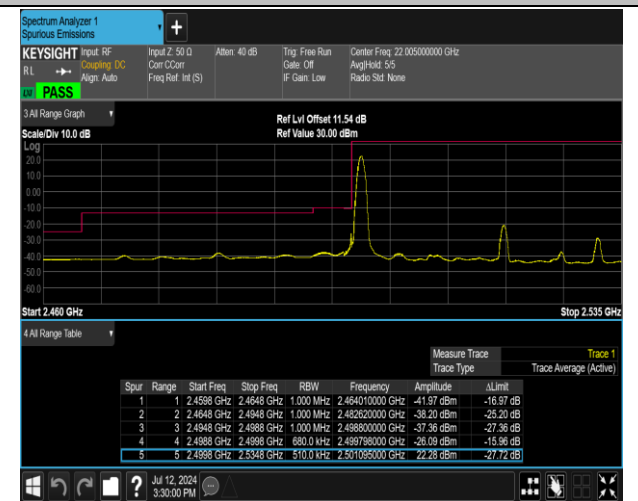
7-7-20MHz-15MHz-16QAM@16QAM-16QAM@16QAM-20850-21021-1RB#0@100RB#0-0RB#0@75RB#0-PASS
