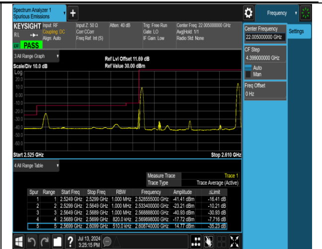
38-38-20MHz-20MHz-QPSK@QPSK-QPSK@QPSK-378 50-38048-1RB#0@100RB#0-1RB#99@100RB#0-PASS
