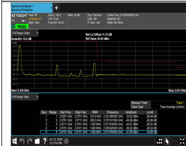
7-7-20MHz-20MHz-QPSK@QPSK-QPSK@QPSK-21152-2 1350-1RB#0@100RB#0-0RB#0@100RB#0-PASS
