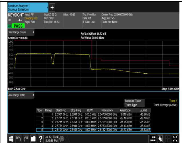
7-7-20MHz-20MHz-QPSK@QPSK-QPSK@QPSK-21152- 21350-100RB#0@100RB#0-100RB#0@100RB#0-PASS
