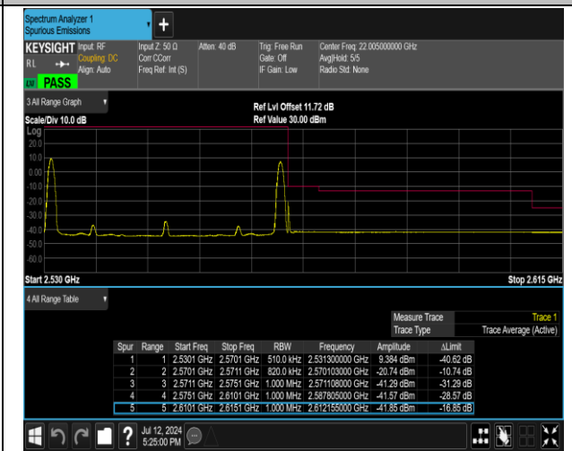
7-7-20MHz-20MHz-QPSK@QPSK-QPSK@QPSK-21152- 21350-1RB#0@100RB#0-1RB#99@100RB#0-PASS
