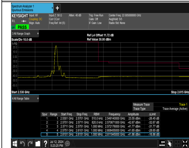
7-7-20MHz-20MHz-QPSK@QPSK-QPSK@QPSK-21152-2 1350-1RB#99@100RB#0-0RB#0@100RB#0-PASS
