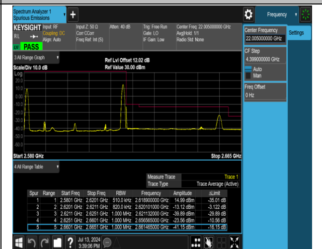
38-38-20MHz-20MHz-QPSK@QPSK-QPSK@QPSK-379 52-38150-1RB#0@100RB#0-1RB#99@100RB#0-PASS
