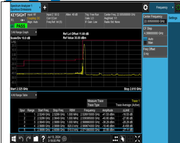
38-38-20MHz-20MHz-QPSK@QPSK-QPSK@QPSK-37850 -38048-1RB#0@100RB#0-0RB#0@100RB#0-PASS
