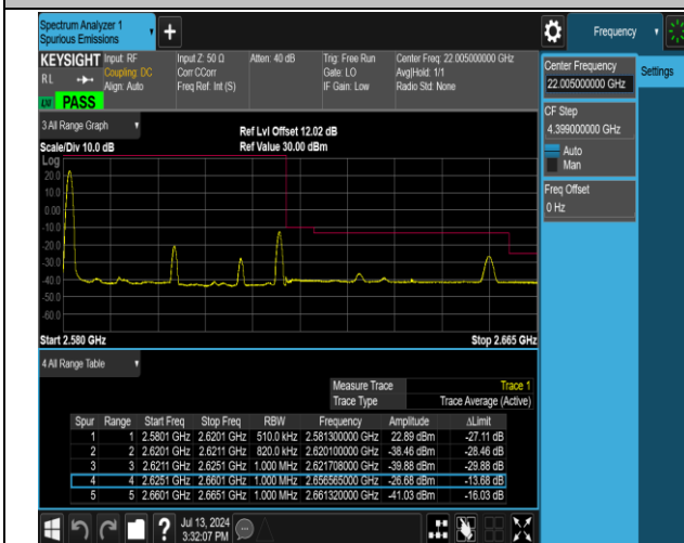
38-38-20MHz-20MHz-QPSK@QPSK-QPSK@QPSK-37952 -38150-1RB#0@100RB#0-0RB#0@100RB#0-PASS
