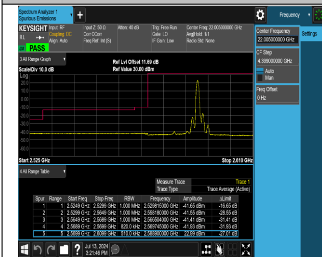
38-38-20MHz-20MHz-QPSK@QPSK-QPSK@QPSK-37850 -38048-1RB#99@100RB#0-0RB#0@100RB#0-PASS
