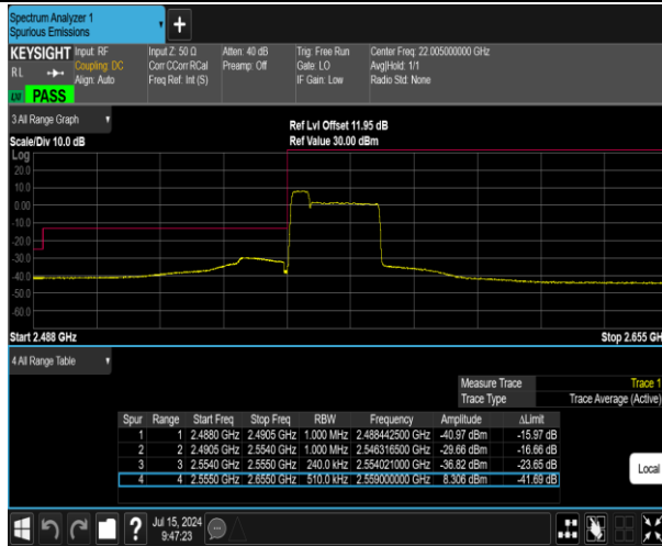
B#99@100RB#0-PASS
