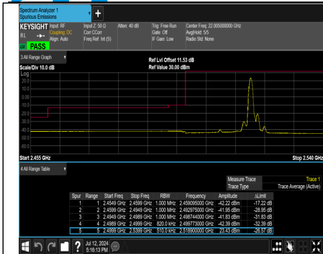
7-7-20MHz-20MHz-QPSK@QPSK-QPSK@QPSK-20850-2 1048-1RB#99@100RB#0-0RB#0@100RB#0-PASS
