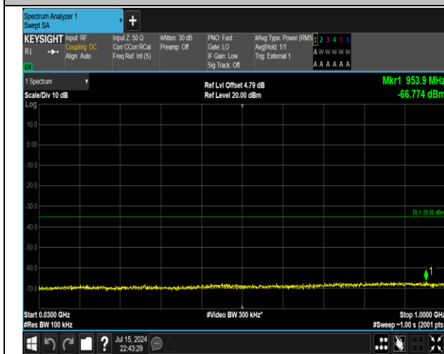
38-38-15MHz-15MHz-16QAM-16QAM-37925-38075-1RB #0-ORB#0-30~1000MHz-PASS
