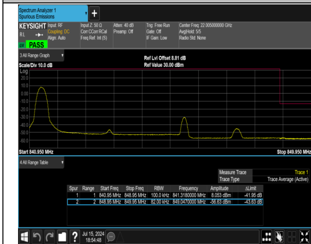
5-5-5MHz-3MHz-QPSK@QPSK-QPSK@QPSK-20595-206 34-1RB#0@25RB#0-1RB#15@15RB#0-PASS
