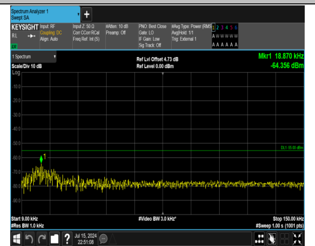
38-38-15MHz-15MHz-16QAM-16QAM-37925-38075-1RB# 0-1RB#74-0.009~0.15MHz-PASS
