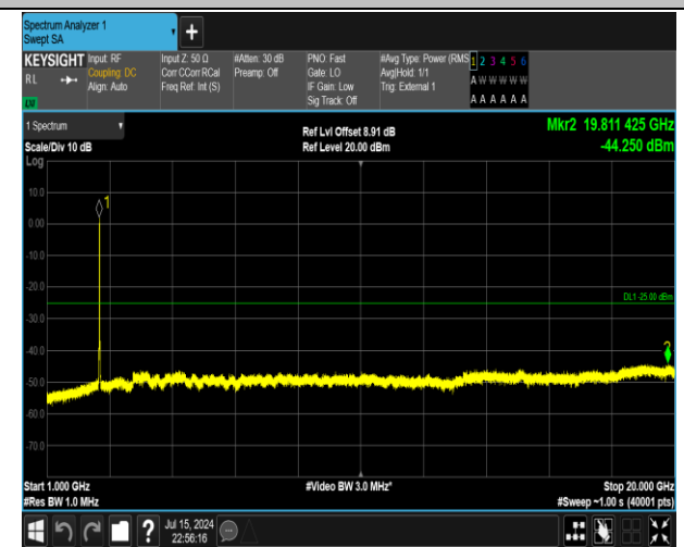
38-38-15MHz-15MHz-16QAM-16QAM-37925-38075-75RB #0-75RB#0-1000~20000MHz-PASS
