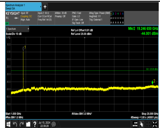
38-38-15MHz-15MHz-16QAM-16QAM-37825-37975-75RB #0-75RB#0-1000~20000MHz-PASS
