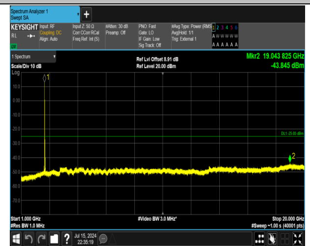
38-38-15MHz-15MHz-16QAM-16QAM-37825-37975-1RB# 0-1RB#74-1000~20000MHz-PASS
