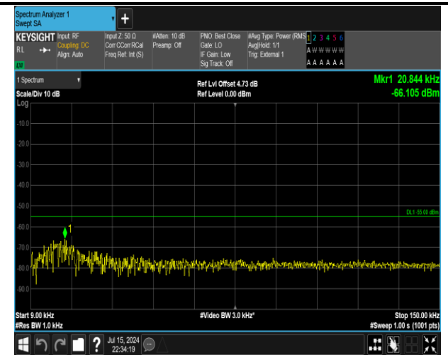
38-38-15MHz-15MHz-16QAM-16QAM-37825-37975-1RB# 0-1RB#74-0.009~0.15MHz-PASS
