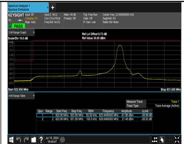
5-5-5MHz-3MHz-QPSK@QPSK-QPSK@QPSK-20425-20 464-1RB#24@25RB#0-0RB#0@15RB#0-PASS
