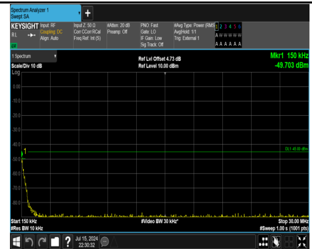
38-38-15MHz-15MHz-16QAM-16QAM-37825-37975-1RB# 74-ORB#0-0.15~30MHz-PASS
