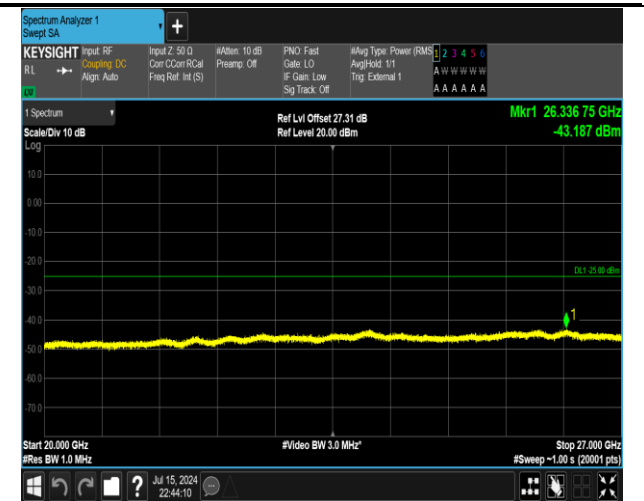
38-38-15MHz-15MHz-16QAM-16QAM-37925-38075-1RB# 0-ORB#0-20000~27000MHz-PASS
