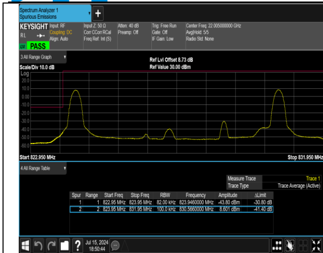
5-5-5MHz-3MHz-QPSK@QPSK-QPSK-20425-204 64-1RB#0@25RB#0-1RB#15@15RB#0-PASS
