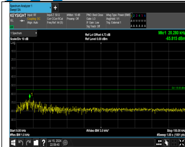
38-38-15MHz-15MHz-16QAM-16QAM-38025-38175-1RB #0-0RB#0-0.009~0.15MHz-PASS
