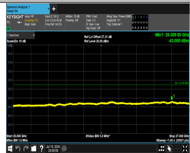
38-38-15MHz-15MHz-16QAM-16QAM-38025-38175-1RB# 0-0RB#0-20000~27000MHz-PASS
