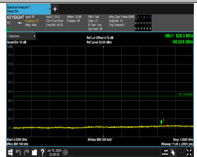
38-38-15MHz-15MHz-16QAM-16QAM-38025-38175-1RB# 0-1RB#74-30~1000MHz-PASS
