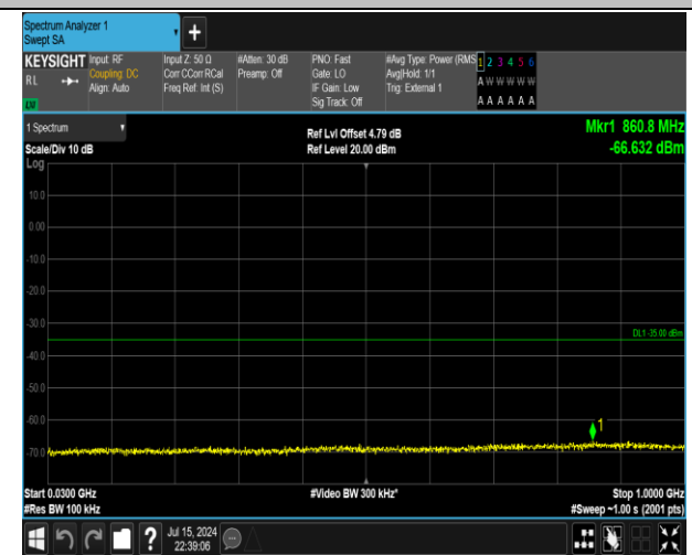
38-38-15MHz-15MHz-16QAM-16QAM-37825-37975-75RB #0-75RB#0-30~1000MHz-PASS
