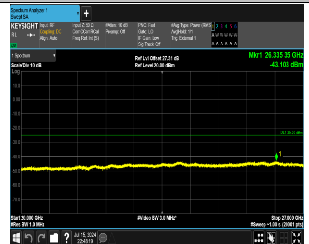
38-38-15MHz-15MHz-16QAM-16QAM-37925-38075-1RB# 74-0RB#0-20000~27000MHz-PASS
