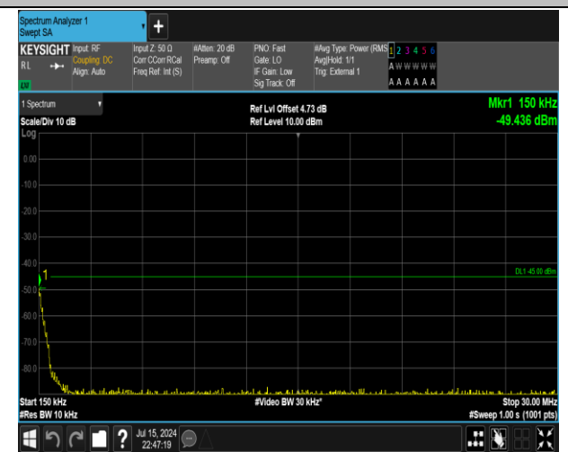
38-38-15MHz-15MHz-16QAM-16QAM-37925-38075-1RB# 74-0RB#0-0.15~30MHz-PASS
