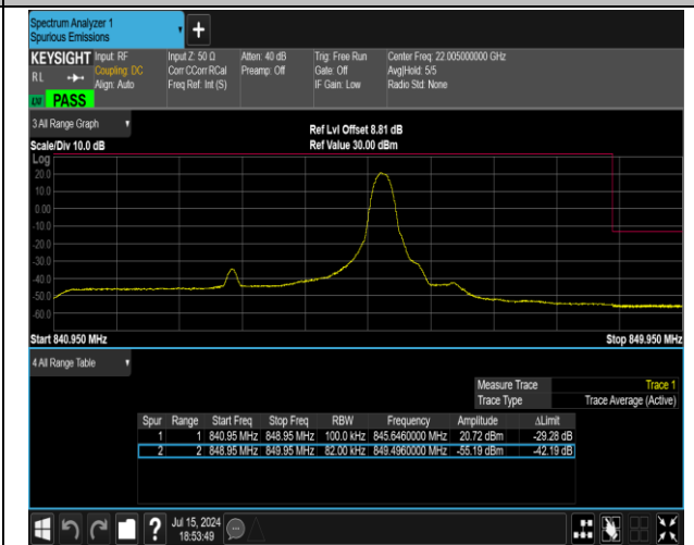
5-5-5MHz-3MHz-QPSK@QPSK-QPSK@QPSK-20595-20 634-1RB#24@25RB#0-0RB#0@15RB#0-PASS
