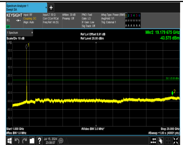
38-38-15MHz-15MHz-16QAM-16QAM-38025-38175-1RB# 0-1RB#74-1000~20000MHz-PASS
