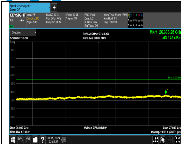
38-38-15MHz-15MHz-16QAM-16QAM-37925-38075-1RB #0-1RB#74-20000~27000MHz-PASS
