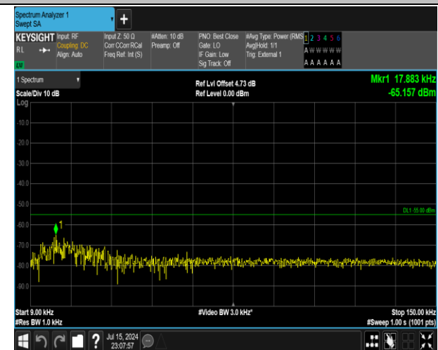
38-38-15MHz-15MHz-16QAM-16QAM-38025-38175-1RB# 0-1RB#74-0.009~0.15MHz-PASS
