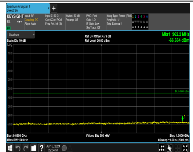
38-38-15MHz-15MHz-16QAM-16QAM-37825-37975-1RB# 0-1RB#74-30~1000MHz-PASS
