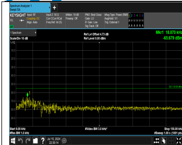
38-38-15MHz-15MHz-16QAM-16QAM-37825-37975-1RB #74-ORB#0-0.009~0.15MHz-PASS
