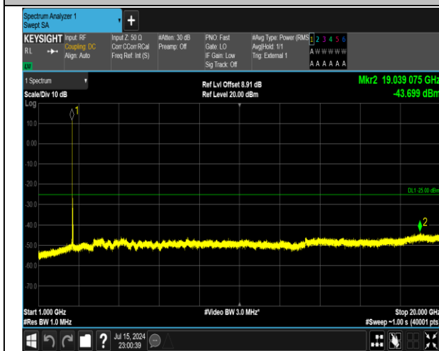
38-38-15MHz-15MHz-16QAM-16QAM-38025-38175-1RB #0-0RB#0-1000~20000MHz-PASS
