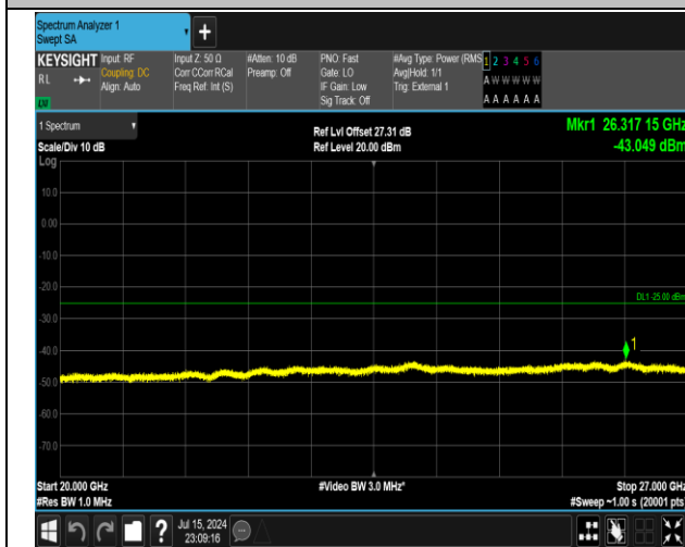
38-38-15MHz-15MHz-16QAM-16QAM-38025-38175-1RB #0-1RB#74-20000~27000MHz-PASS
