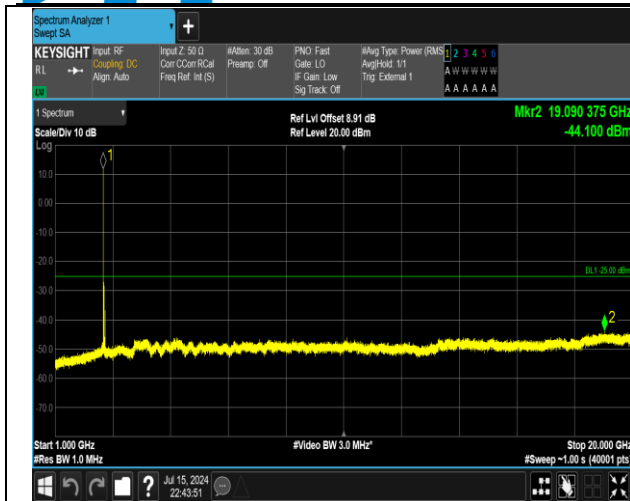
38-38-15MHz-15MHz-16QAM-16QAM-37925-38075-1RB #0-ORB#0-1000~20000MHz-PASS
