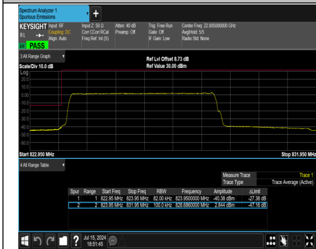
5-5-5MHz-3MHz-QPSK@QPSK-QPSK@QPSK-20425-204 64-25RB#0@25RB#0-15RB#0@15RB#0-PASS
