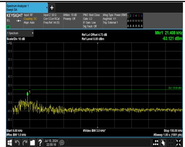
38-38-15MHz-15MHz-16QAM-16QAM-37925-38075-75RB #0-75RB#0-0.009~0.15MHz-PASS
