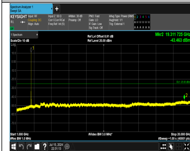
38-38-15MHz-15MHz-16QAM-16QAM-37825-37975-1RB #74-ORB#0-1000~20000MHz-PASS
