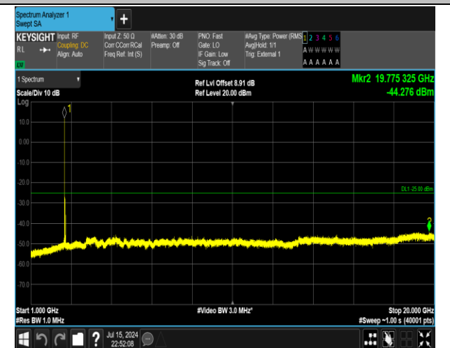
38-38-15MHz-15MHz-16QAM-16QAM-37925-38075-1RB# 0-1RB#74-1000~20000MHz-PASS
