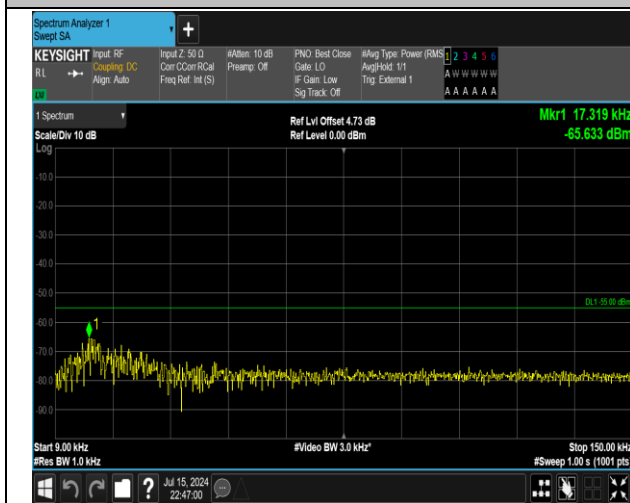
38-38-15MHz-15MHz-16QAM-16QAM-37925-38075-1RB #74-0RB#0-0.009~0.15MHz-PASS
