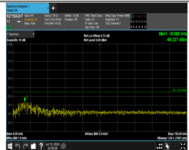
38-38-15MHz-15MHz-16QAM-16QAM-37825-37975-75RB #0-75RB#0-0.009~0.15MHz-PASS
