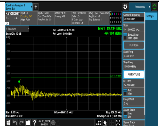
38-38-20MHz-20MHz-QPSK-QPSK-37952-38150-1RB#0-0 RB#0-0.009~0.15MHz-PASS
