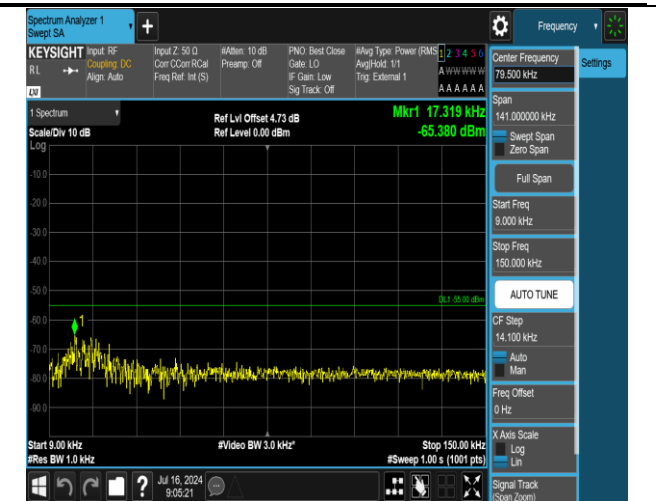
38-38-20MHz-20MHz-QPSK-QPSK-37901-38099-1RB#99-ORB#0-0.009~0.15MHz-PASS
