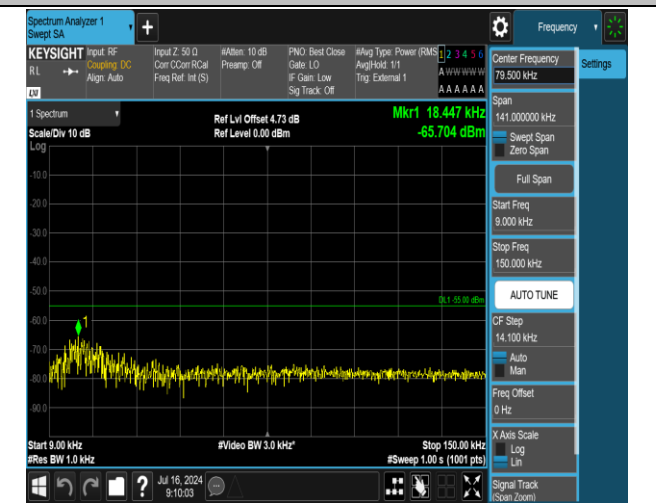
38-38-20MHz-20MHz-QPSK-QPSK-37952-38150-1RB#99- ORB#0-0.009~0.15MHz-PASS
