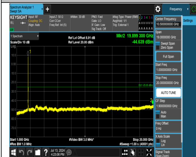
38-38-20MHz-20MHz-QPSK-QPSK-37952-38150-100RB# 0-100RB#0-1000~20000MHz-PASS
