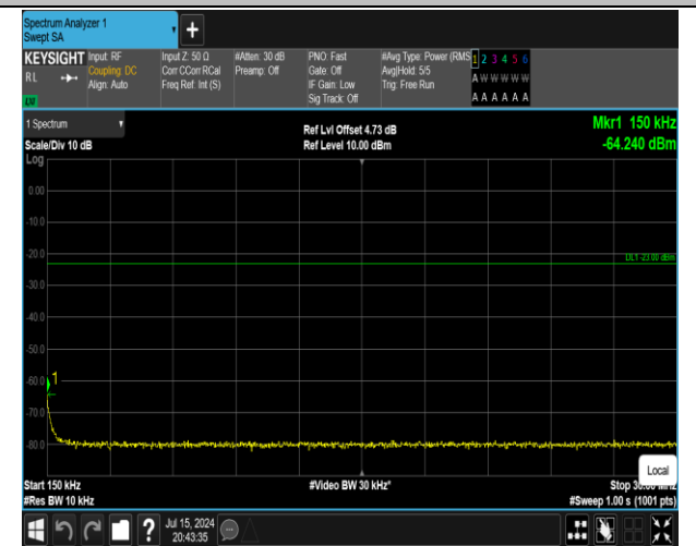
5-5-10MHz-10MHz-16QAM-16QAM-20450-20549-1RB#49-0RB#0-0.15~30MHz-PASS
