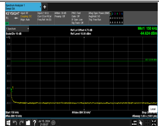
5-5-10MHz-10MHz-16QAM-16QAM-20501-20600-1RB#0- ORB#0-0.15~30MHz-PASS
