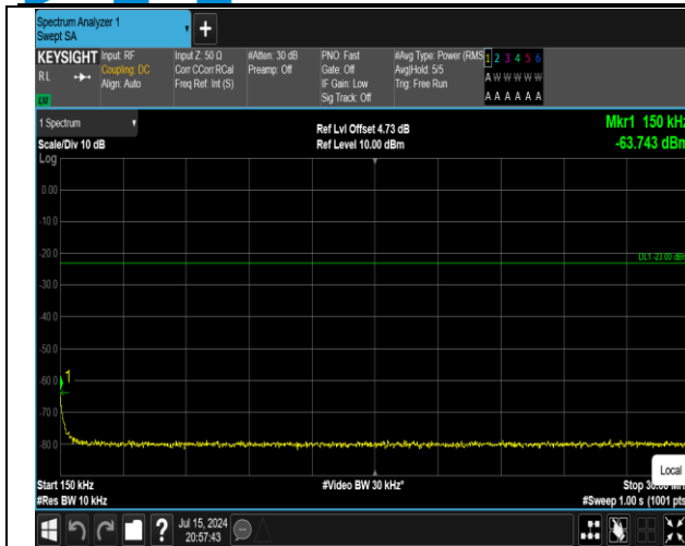
5-5-10MHz-10MHz-16QAM-16QAM-20476-20575-50RB# 0-50RB#0-0.15~30MHz-PASS
