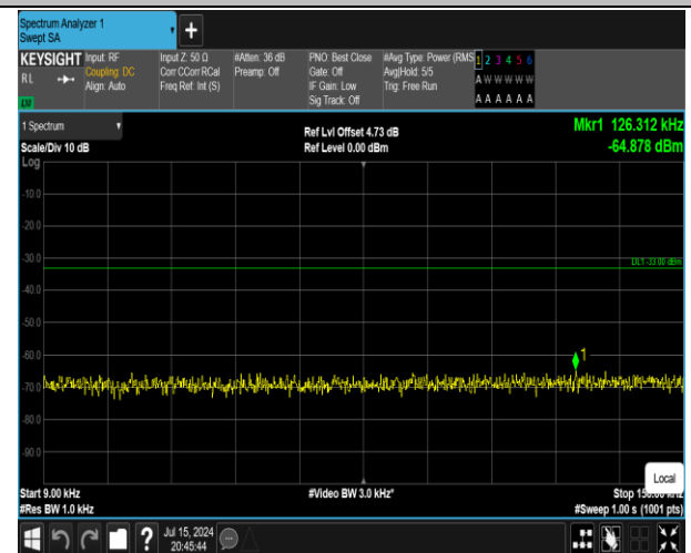
5-5-10MHz-10MHz-16QAM-16QAM-20450-20549-1RB#0- 1RB#49-0.009~0.15MHz-PASS
