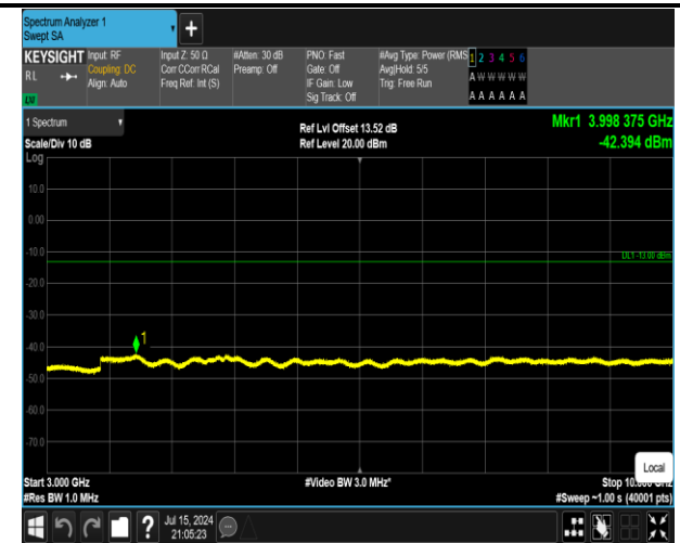
5-5-10MHz-10MHz-16QAM-16QAM-20501-20600-1RB#0-1RB#49-3000~10000MHz-PASS
