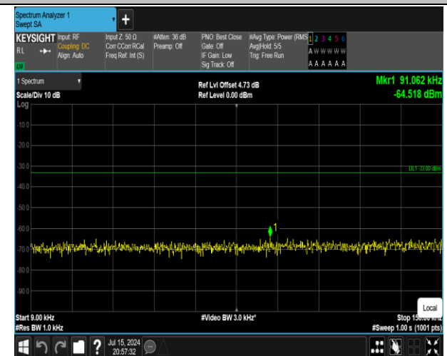
5-5-10MHz-10MHz-16QAM-16QAM-20476-20575-50RB#0 -50RB#0-0.009~0.15MHz-PASS
