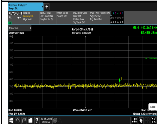
5-5-10MHz-10MHz-16QAM-16QAM-20450-20549-1RB#49-0RB#0-0.009~0.15MHz-PASS
