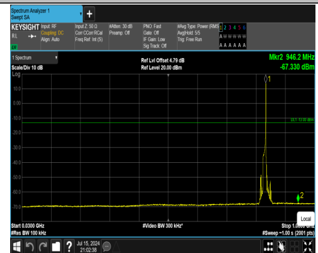
5-5-10MHz-10MHz-16QAM-16QAM-20501-20600-1RB#49-0RB#0-30~1000MHz-PASS
