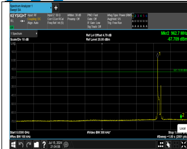
5-5-10MHz-10MHz-16QAM-16QAM-20501-20600-1RB#0-1RB#49-30~1000MHz-PASS
