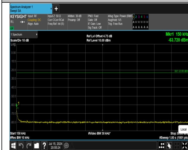
5-5-10MHz-10MHz-16QAM-16QAM-20476-20575-1RB#0- 1RB#49-0.15~30MHz-PASS
