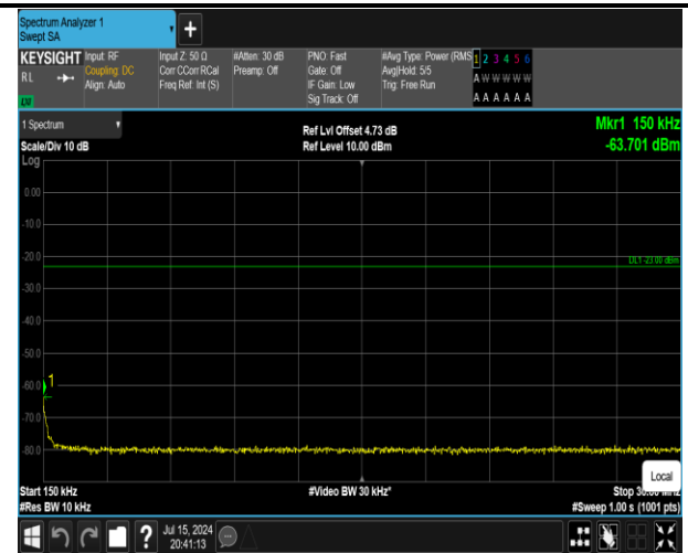
5-5-10MHz-10MHz-16QAM-16QAM-20450-20549-1RB#0- ORB#0-0.15~30MHz-PASS
