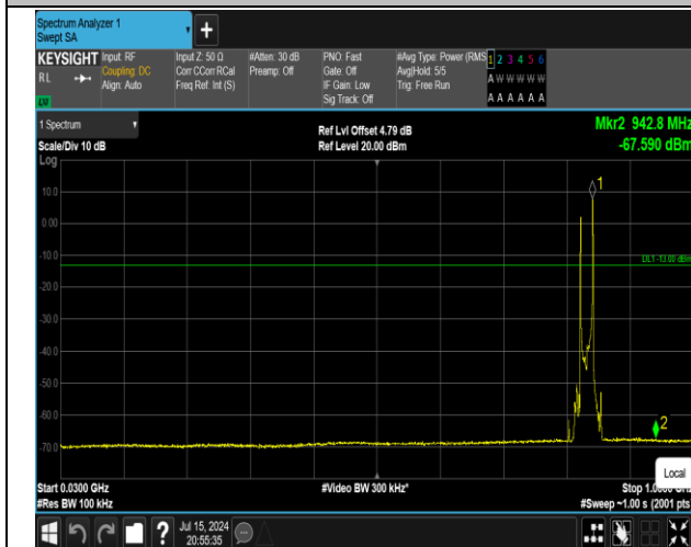
5-5-10MHz-10MHz-16QAM-16QAM-20476-20575-1RB#0- 1RB#49-30~1000MHz-PASS
