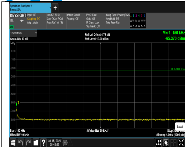
5-5-10MHz-10MHz-16QAM-16QAM-20450-20549-1RB#0-1RB#49-0.15~30MHz-PASS
