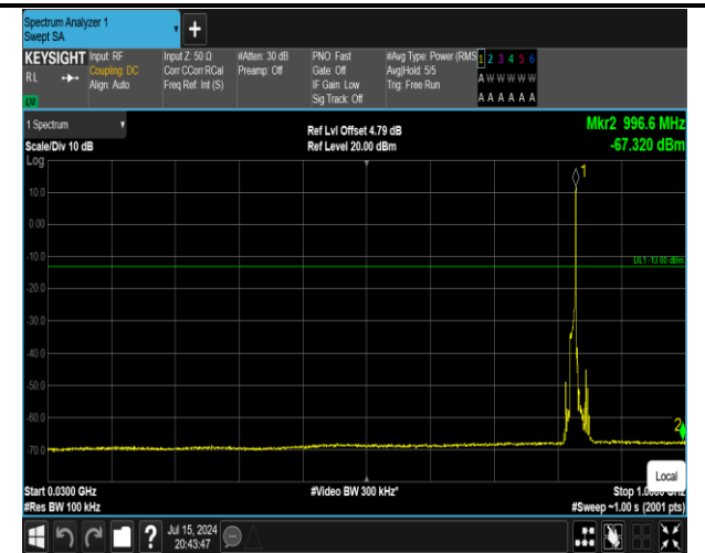
5-5-10MHz-10MHz-16QAM-16QAM-20450-20549-1RB#49 -0RB#0-30~1000MHz-PASS
