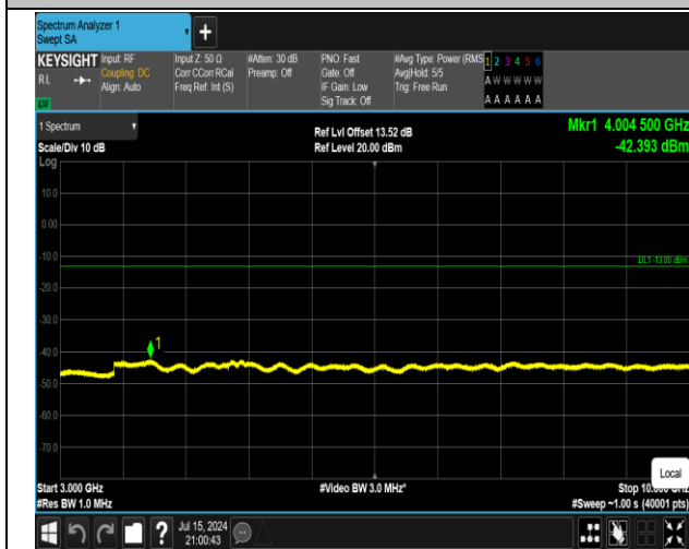
5-5-10MHz-10MHz-16QAM-16QAM-20501-20600-1RB#0-ORB#0-3000~10000MHz-PASS
