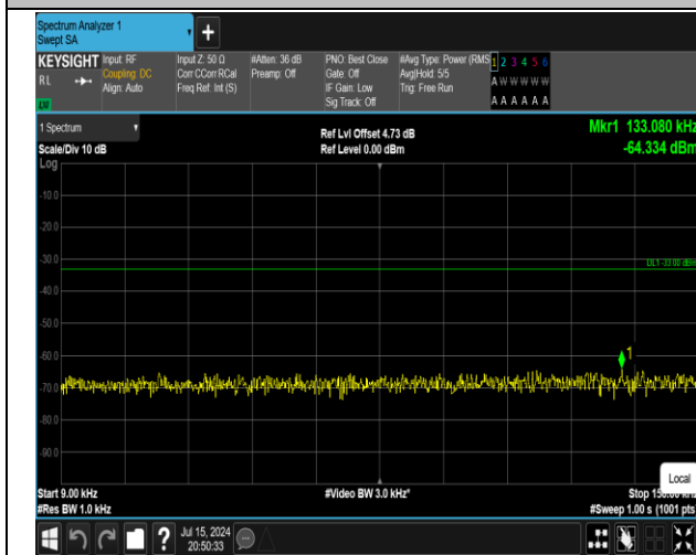
5-5-10MHz-10MHz-16QAM-16QAM-20476-20575-1RB#0- ORB#0-0.009~0.15MHz-PASS
