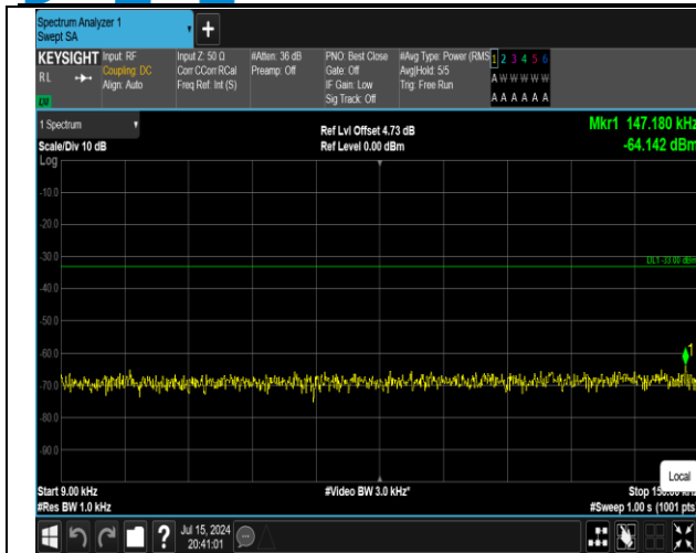
5-5-10MHz-10MHz-16QAM-16QAM-20450-20549-1RB#0- ORB#0-0.009~0.15MHz-PASS
