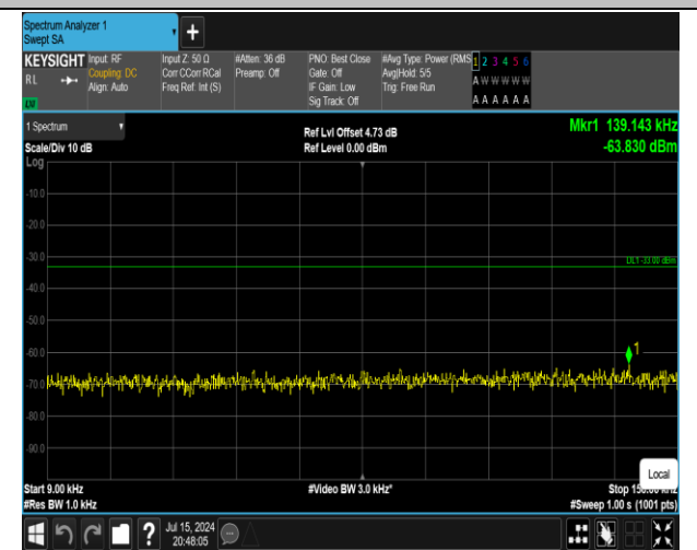
5-5-10MHz-10MHz-16QAM-16QAM-20450-20549-50RB#0 -50RB#0-0.009~0.15MHz-PASS
