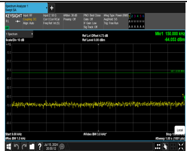
5-5-10MHz-10MHz-16QAM-16QAM-20476-20575-1RB#0- 1RB#49-0.009~0.15MHz-PASS
