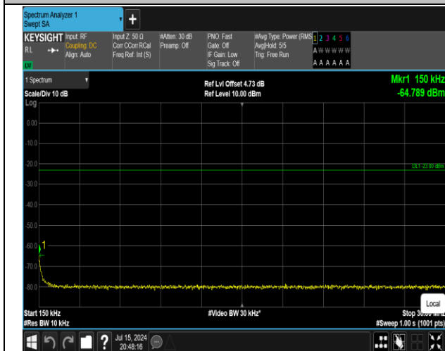
5-5-10MHz-10MHz-16QAM-16QAM-20450-20549-50RB# 0-50RB#0-0.15~30MHz-PASS
