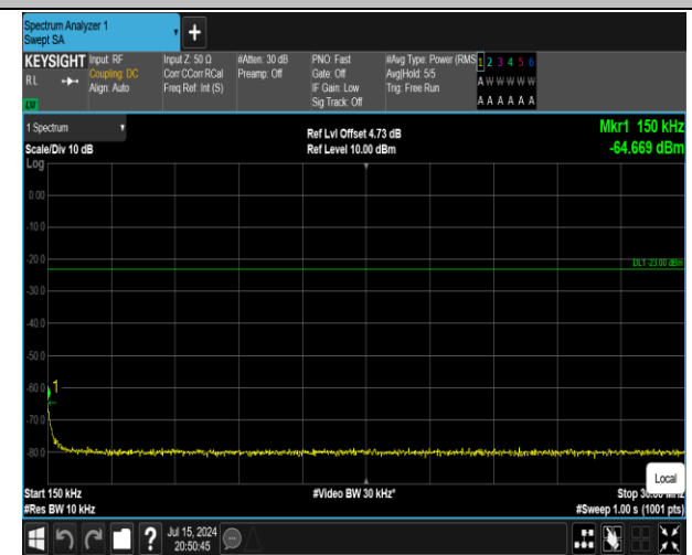
5-5-10MHz-10MHz-16QAM-16QAM-20476-20575-1RB#0- ORB#0-0.15~30MHz-PASS
