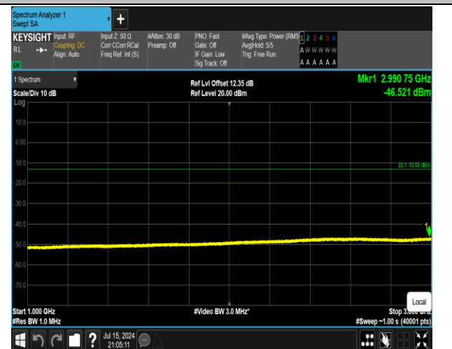
5-5-10MHz-10MHz-16QAM-16QAM-20501-20600-1RB#0-1RB#49-1000~3000MHz-PASS
