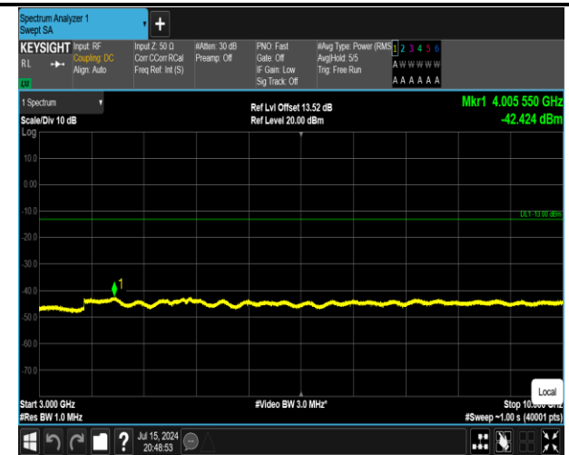
5-5-10MHz-10MHz-16QAM-16QAM-20450-20549-50RB#0 -50RB#0-3000~10000MHz-PASS
