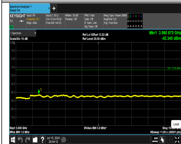
5-5-10MHz-10MHz-16QAM-16QAM-20450-20549-1RB#4 9-0RB#0-3000~10000MHz-PASS
