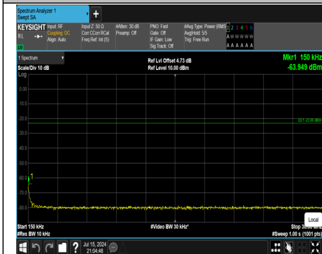
5-5-10MHz-10MHz-16QAM-16QAM-20501-20600-1RB#0-1RB#49-0.15~30MHz-PASS
