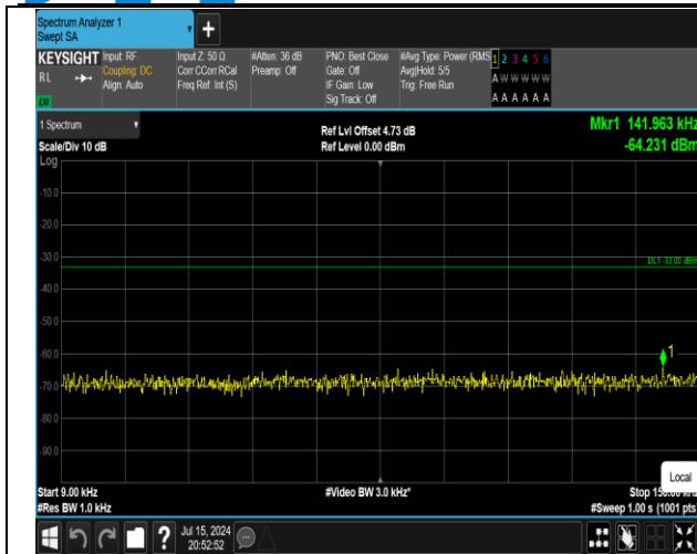
5-5-10MHz-10MHz-16QAM-16QAM-20476-20575-1RB#4 9-ORB#0-0.009~0.15MHz-PASS
