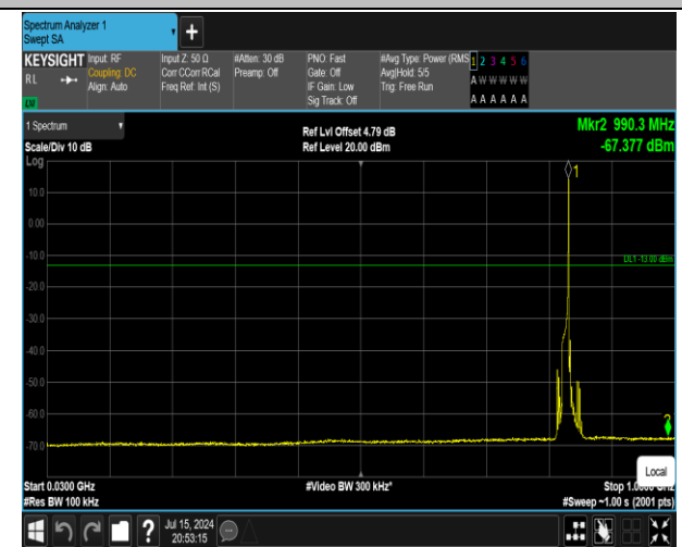
5-5-10MHz-10MHz-16QAM-16QAM-20476-20575-1RB#49 -ORB#0-30~1000MHz-PASS
