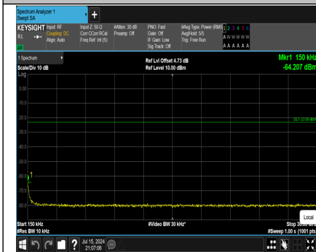
5-5-10MHz-10MHz-16QAM-16QAM-20501-20600-50RB#0 0-50RB#0-0.15~30MHz-PASS
