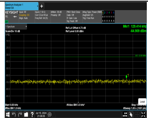
5-5-10MHz-10MHz-16QAM-16QAM-20501-20600-50RB#0 -50RB#0-0.009~0.15MHz-PASS
