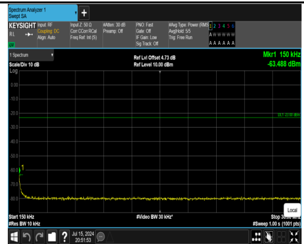
5-5-10MHz-10MHz-QPSK-QPSK-20476-20575-1RB#49-0 RB#0-0.15~30MHz-PASS
