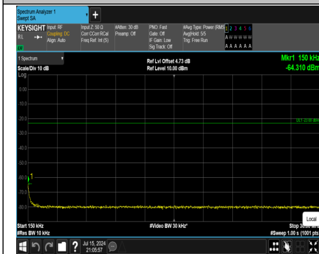
5-5-10MHz-10MHz-QPSK-QPSK-20501-20600-50RB#0-5 ORB#0-0.15~30MHz-PASS
