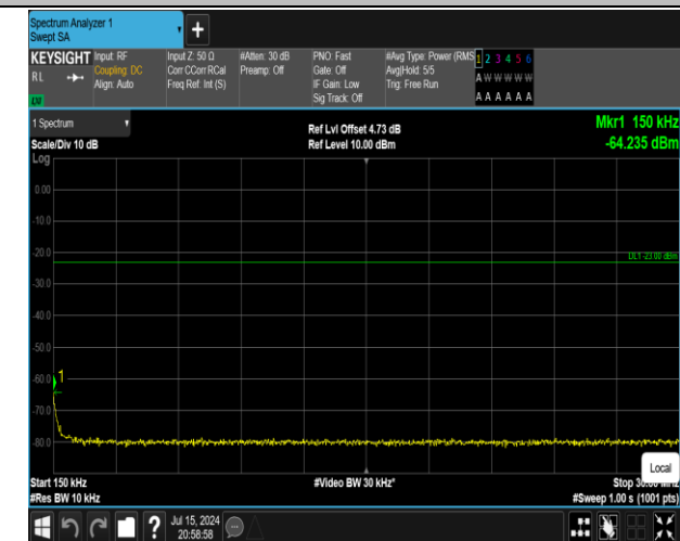
5-5-10MHz-10MHz-QPSK-QPSK-20501-20600-1RB#0-0R B#0-0.15~30MHz-PASS
