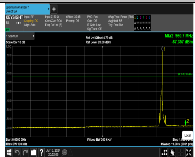
5-5-10MHz-10MHz-QPSK-QPSK-20476-20575-1RB#49-0 RB#0-30~1000MHz-PASS
