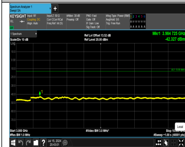
5-5-10MHz-10MHz-QPSK-QPSK-20450-20549-1RB#49-0 RB#0-3000~10000MHz-PASS
