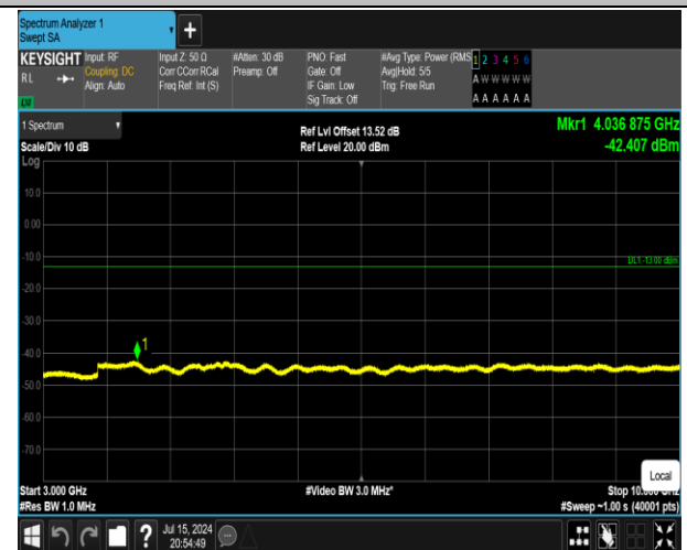
5-5-10MHz-10MHz-QPSK-QPSK-20476-20575-1RB#0-1R B#49-3000~10000MHz-PASS
