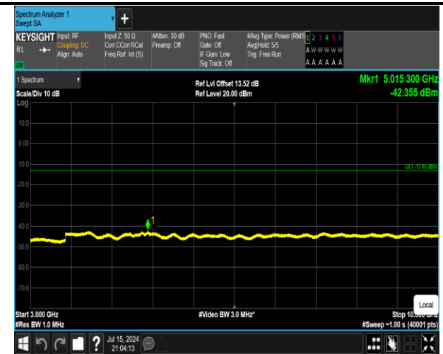
5-5-10MHz-10MHz-QPSK-QPSK-20501-20600-1RB#0-1R B#49-3000~10000MHz-PASS
