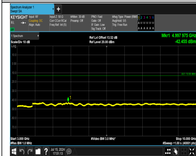
5-5-3MHz-5MHz-16QAM-16QAM-20416-20455-1RB#0-1R B#24-3000~10000MHz-PASS
