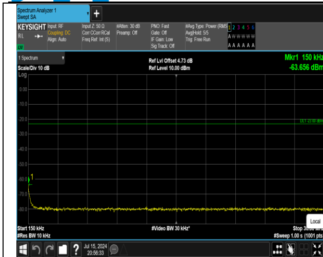
5-5-10MHz-10MHz-QPSK-QPSK-20476-20575-50RB#0-5 ORB#0-0.15~30MHz-PASS
