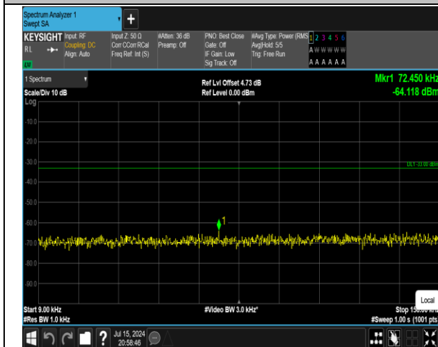
5-5-10MHz-10MHz-QPSK-QPSK-20501-20600-1RB#0-0R B#0-0.009~0.15MHz-PASS
