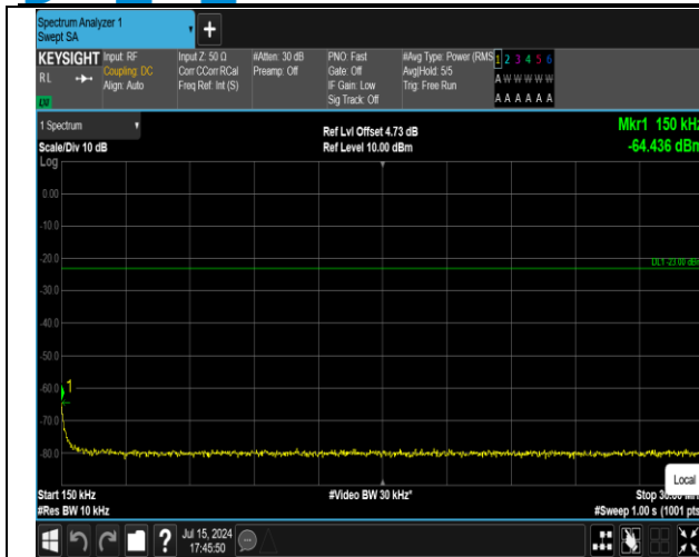
5-5-3MHz-5MHz-16QAM-16QAM-20416-20455-1RB#0-0R B#0-0.15~30MHz-PASS
