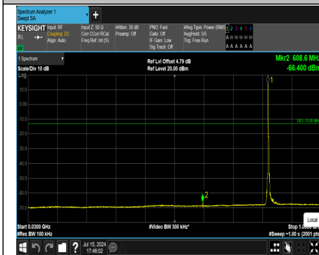
5-5-3MHz-5MHz-16QAM-16QAM-20416-20455-1RB#0-0R B#0-30~1000MHz-PASS
