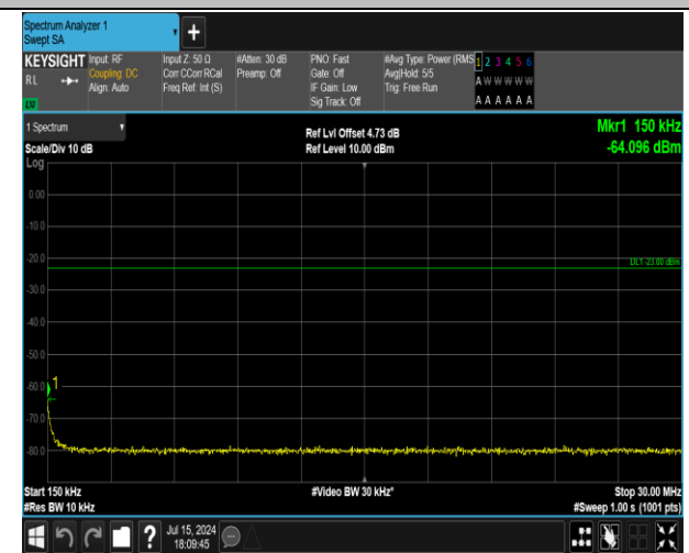
5-5-3MHz-5MHz-16QAM-16QAM-20501-20540-15RB#0-2 5RB#0-0.15~30MHz-PASS
