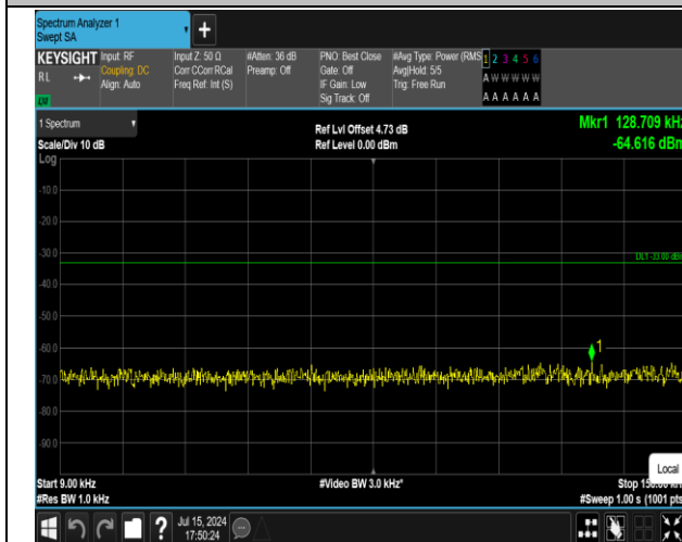
5-5-3MHz-5MHz-16QAM-16QAM-20416-20455-1RB#0-1R B#24-0.009~0.15MHz-PASS
