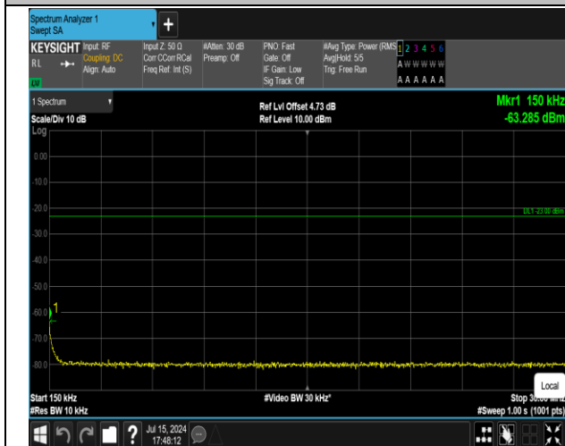
5-5-3MHz-5MHz-16QAM-16QAM-20416-20455-1RB#14-0 RB#0-0.15~30MHz-PASS
