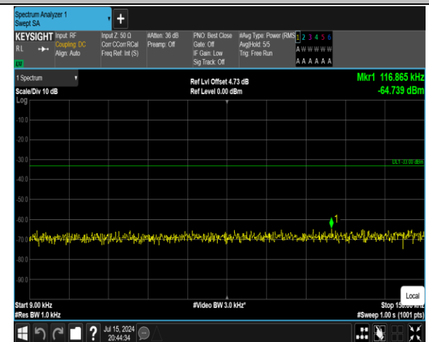
5-5-10MHz-10MHz-QPSK-QPSK-20450-20549-1RB#0-1R B#49-0.009~0.15MHz-PASS
