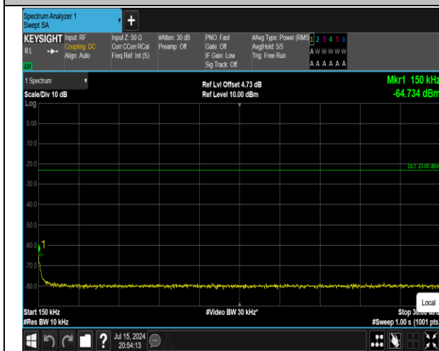
5-5-10MHz-10MHz-QPSK-QPSK-20476-20575-1RB#0-1R B#49-0.15~30MHz-PASS
