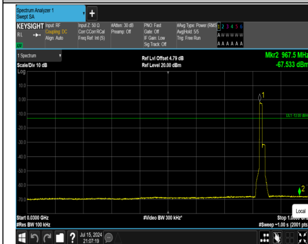
5-5-10MHz-10MHz-16QAM-16QAM-20501-20600-50RB#0 0-50RB#0-30~1000MHz-PASS
