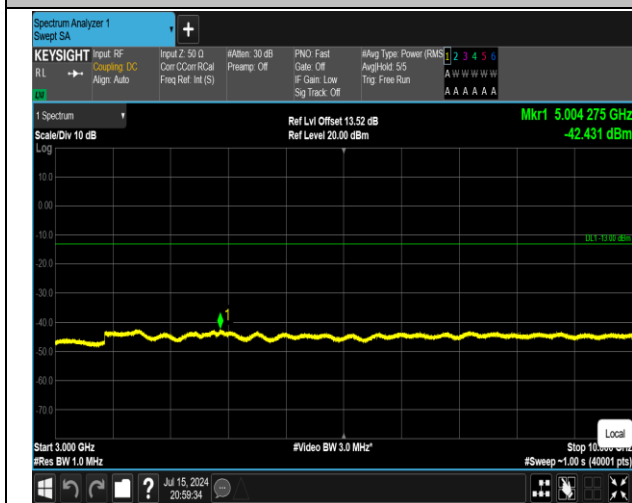
5-5-10MHz-10MHz-QPSK-QPSK-20501-20600-1RB#0-0R B#0-3000~10000MHz-PASS
