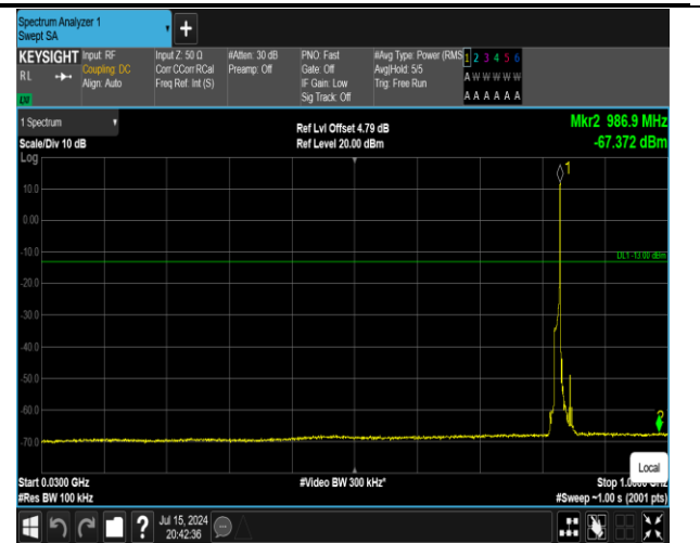
5-5-10MHz-10MHz-QPSK-QPSK-20450-20549-1RB#49-0 RB#0-30~1000MHz-PASS
