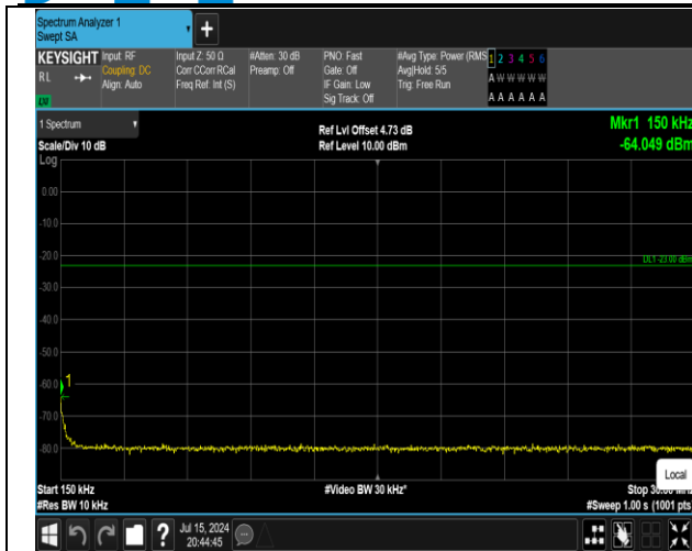
5-5-10MHz-10MHz-QPSK-QPSK-20450-20549-1RB#0-1R B#49-0.15~30MHz-PASS
