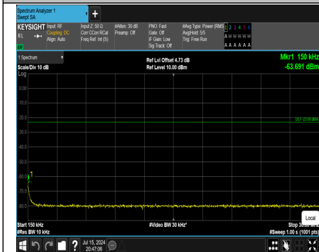
5-5-10MHz-10MHz-QPSK-QPSK-20450-20549-50RB#0-5 ORB#0-0.15~30MHz-PASS
