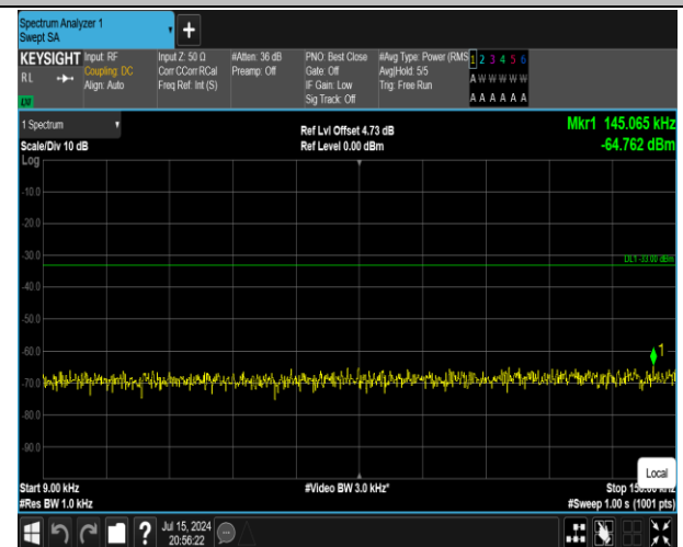
5-5-10MHz-10MHz-QPSK-QPSK-20476-20575-50RB#0-50 RB#0-0.009~0.15MHz-PASS
