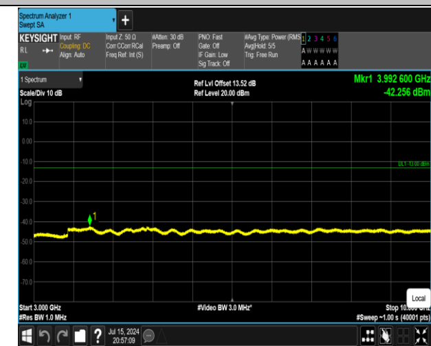
5-5-10MHz-10MHz-QPSK-QPSK-20476-20575-50RB#0-50 RB#0-3000~10000MHz-PASS
