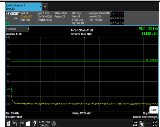
5-5-10MHz-10MHz-QPSK-QPSK-20450-20549-1RB#49-0 RB#0-0.15~30MHz-PASS
