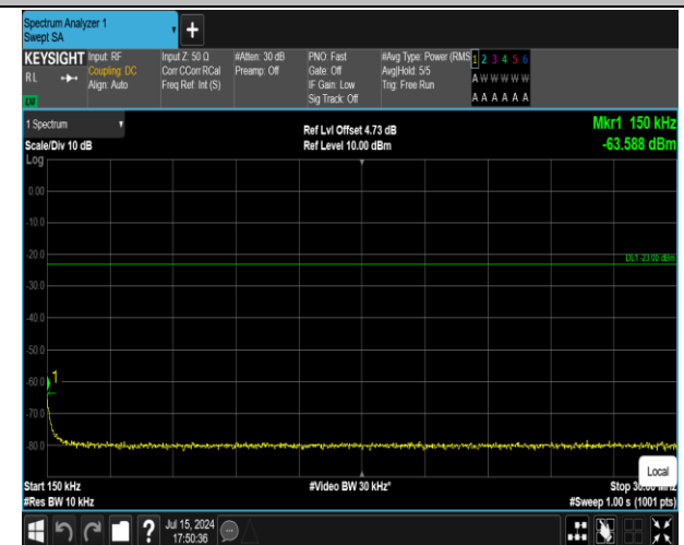
5-5-3MHz-5MHz-16QAM-16QAM-20416-20455-1RB#0-1R B#24-0.15~30MHz-PASS
