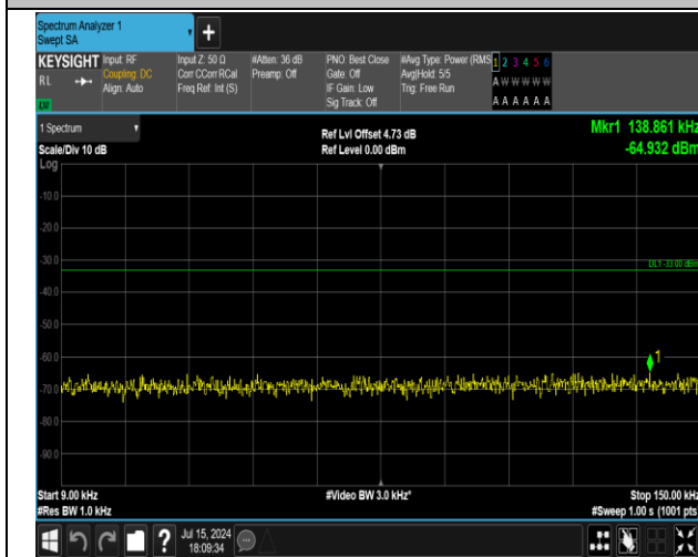
5-5-3MHz-5MHz-16QAM-16QAM-20501-20540-15RB#0-2 5RB#0-0.009~0.15MHz-PASS
