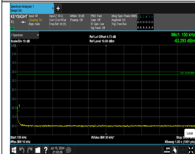
5-5-10MHz-10MHz-QPSK-QPSK-20501-20600-1RB#0-1R B#49-0.15~30MHz-PASS
