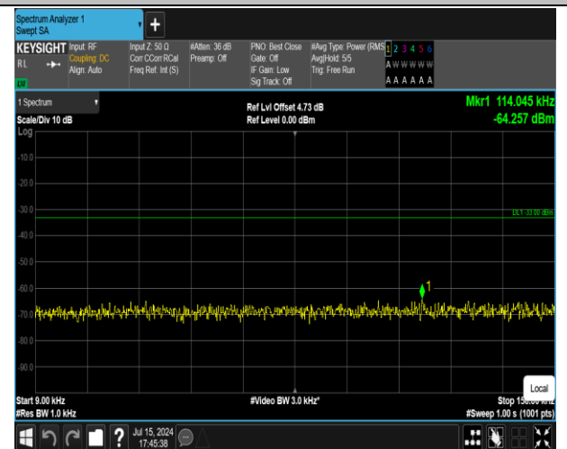
5-5-3MHz-5MHz-16QAM-16QAM-20416-20455-1RB#0-0R B#0-0.009~0.15MHz-PASS
