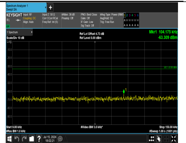
5-5-3MHz-5MHz-16QAM-16QAM-20501-20540-1RB#0-0R B#0-0.009~0.15MHz-PASS
