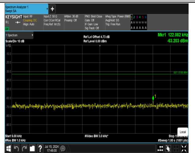
5-5-3MHz-5MHz-16QAM-16QAM-20416-20455-1RB#14-0 RB#0-0.009~0.15MHz-PASS
