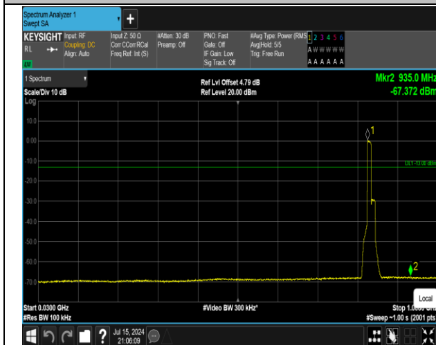
5-5-10MHz-10MHz-QPSK-QPSK-20501-20600-50RB#0-5 ORB#0-30~1000MHz-PASS
