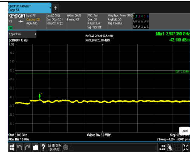
5-5-10MHz-10MHz-QPSK-QPSK-20450-20549-50RB#0-50 RB#0-3000~10000MHz-PASS
