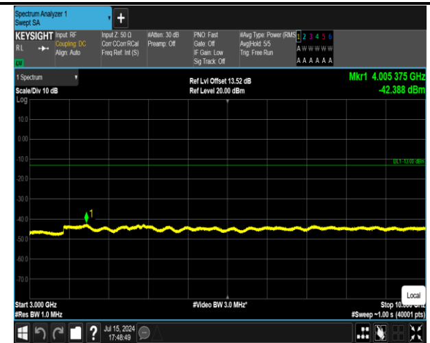
5-5-3MHz-5MHz-16QAM-16QAM-20416-20455-1RB#14-0 RB#0-3000~10000MHz-PASS
