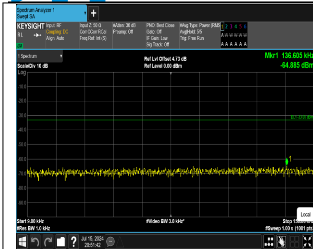
5-5-10MHz-10MHz-QPSK-QPSK-20476-20575-1RB#49-0 RB#0-0.009~0.15MHz-PASS
