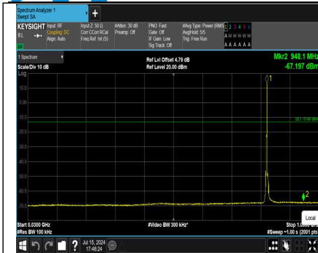
5-5-3MHz-5MHz-16QAM-16QAM-20416-20455-1RB#14-0 RB#0-30~1000MHz-PASS
