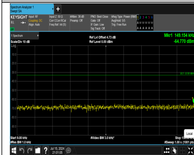
5-5-10MHz-10MHz-QPSK-QPSK-20501-20600-1RB#49-0 RB#0-0.009~0.15MHz-PASS
