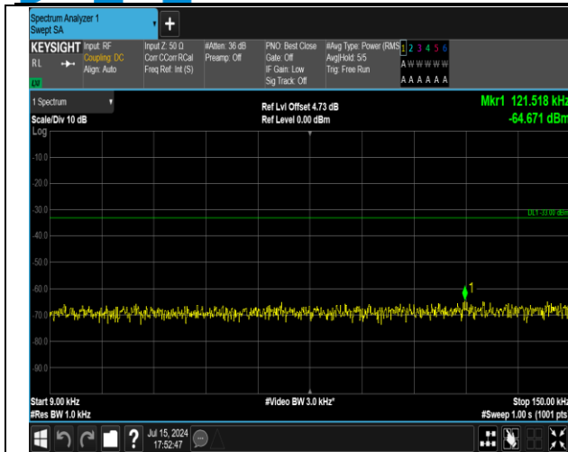
5-5-3MHz-5MHz-16QAM-16QAM-20416-20455-15RB#0-2 5RB#0-0.009~0.15MHz-PASS
