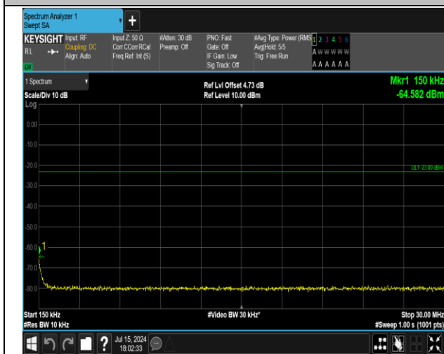
5-5-3MHz-5MHz-16QAM-16QAM-20501-20540-1RB#0-0R B#0-0.15~30MHz-PASS
