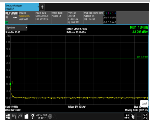
5-5-10MHz-10MHz-QPSK-QPSK-20501-20600-1RB#49-0 RB#0-0.15~30MHz-PASS
