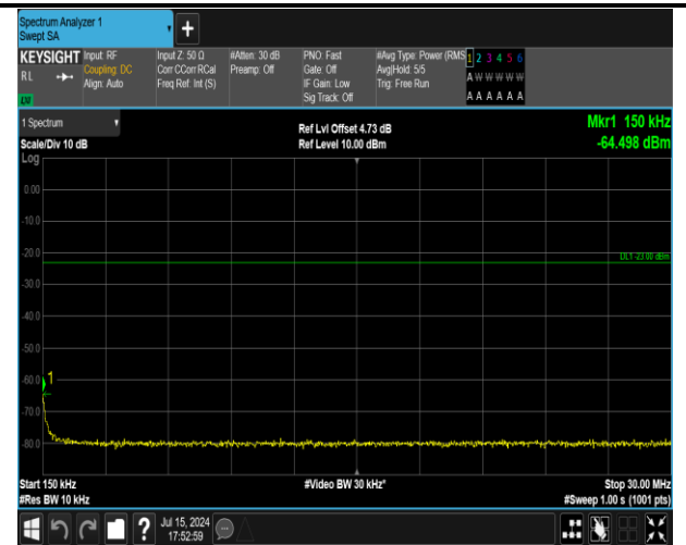
5-5-3MHz-5MHz-16QAM-16QAM-20416-20455-15RB#0-2 5RB#0-0.15~30MHz-PASS
