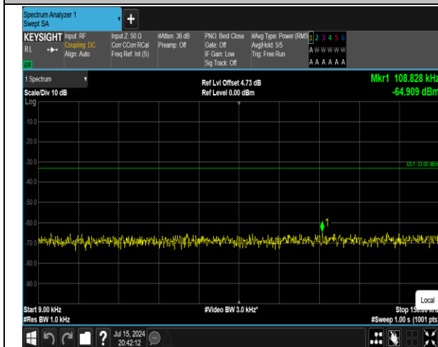
5-5-10MHz-10MHz-QPSK-QPSK-20450-20549-1RB#49-0 RB#0-0.009~0.15MHz-PASS
