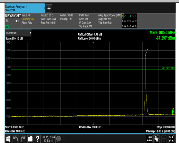
5-5-3MHz-5MHz-16QAM-16QAM-20416-20455-15RB#0-2 5RB#0-30~1000MHz-PASS
