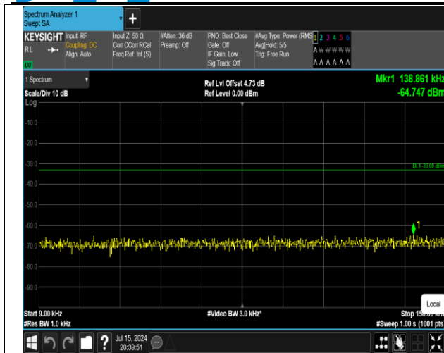
5-5-10MHz-10MHz-QPSK-QPSK-20450-20549-1RB#0-0R B#0-0.009~0.15MHz-PASS
