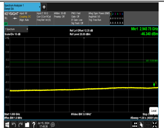
5-5-3MHz-5MHz-16QAM-16QAM-20416-20455-1RB#14-0 RB#0-1000~3000MHz-PASS
