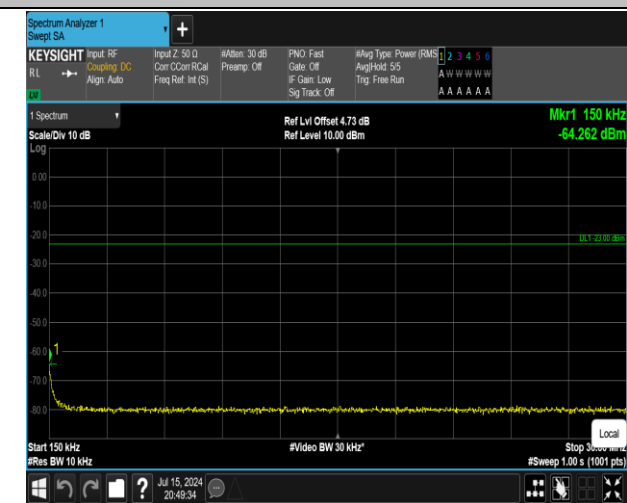
5-5-10MHz-10MHz-QPSK-QPSK-20476-20575-1RB#0-0R B#0-0.15~30MHz-PASS
