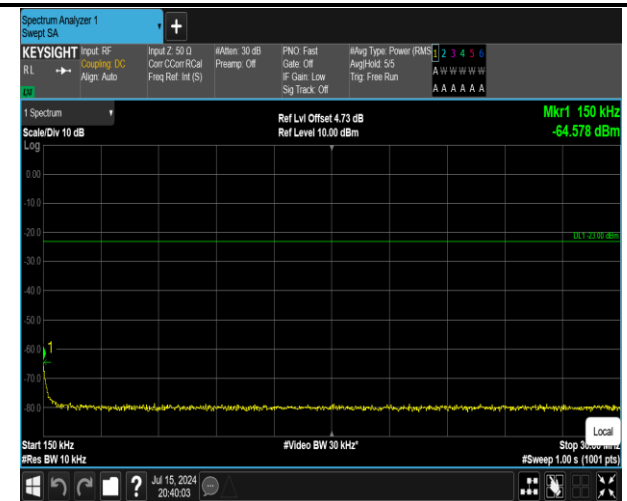
5-5-10MHz-10MHz-QPSK-QPSK-20450-20549-1RB#0-0R B#0-0.15~30MHz-PASS
