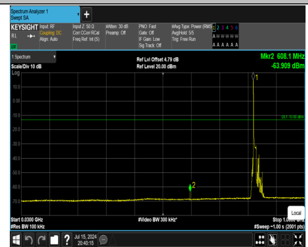
5-5-10MHz-10MHz-QPSK-QPSK-20450-20549-1RB#0-0R B#0-30~1000MHz-PASS
