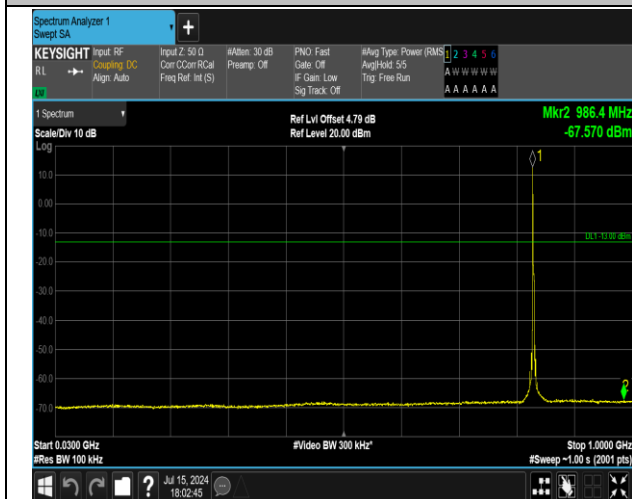
5-5-3MHz-5MHz-16QAM-16QAM-20501-20540-1RB#0-0R B#0-30~1000MHz-PASS
